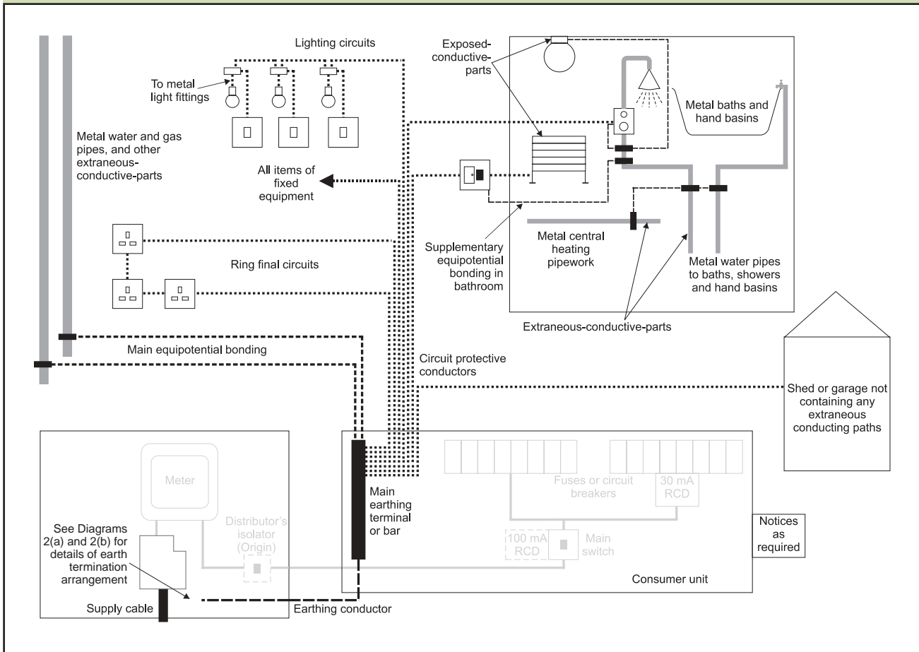
Diagram 1(b): Illustration of the earthing and bonding conductors that might be part of the electrical installation shown in Diagram 1(a)
