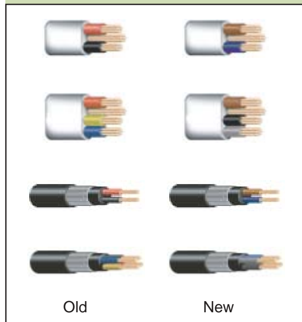
Figure D1: Examples of cables with old and new colours
