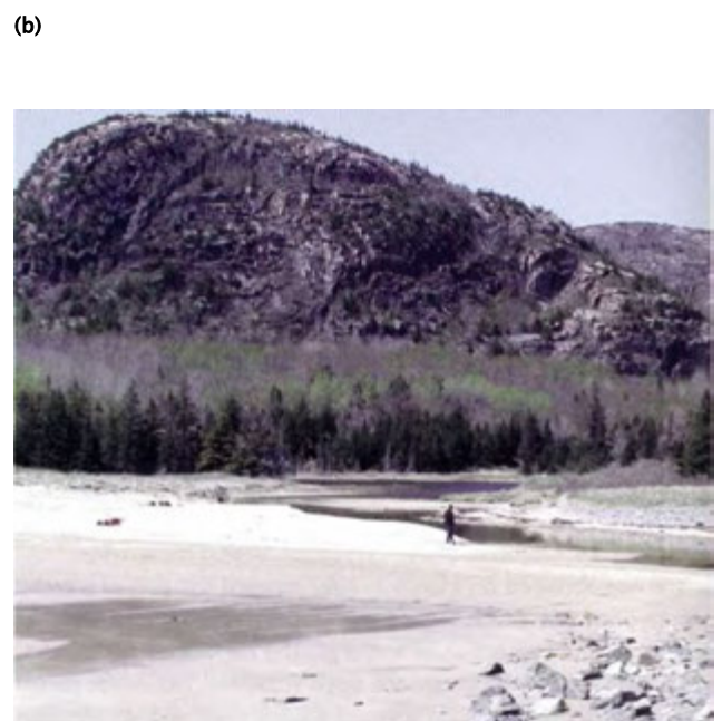
(b) A roche moutonnée known as The Beehive rises above Sand Beach at Acadia National Park in Maine. [Robert E. Nelson, Colby College.]
