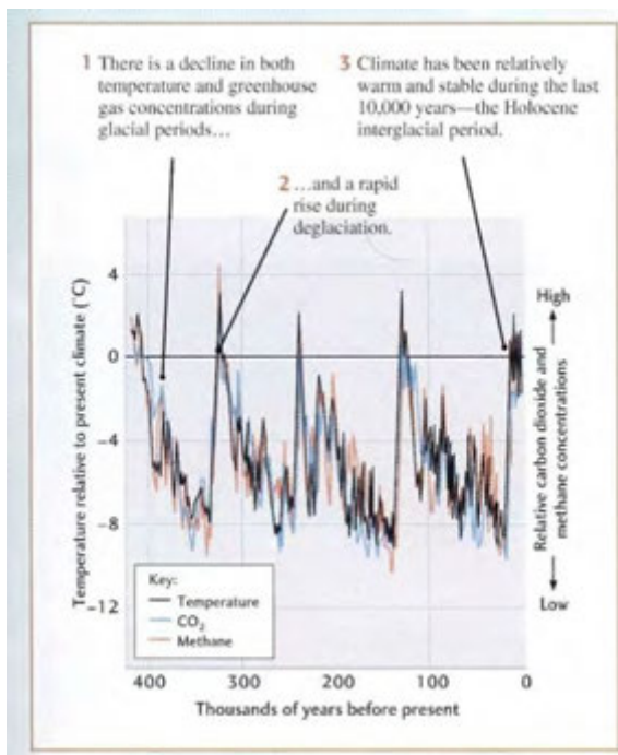
Figure 15.10 A graph showing three types of data recovered from the Vostok ice core in East Antarctica: temperatures inferred from oxygen isotope (black line) and the concentrations of two important greenhouse gases, carbon dioxide (blue line) and methane (red line). The gas concentrations come from measurements of air samples trapped as tiny bubbles within the Antarctic ice. [IPCC, Climate Change 2001: The Scientific Basis ]
