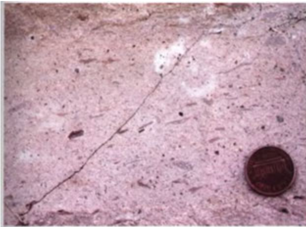
Figure 12.9 (a) Welded tuff from an ash-flow deposit in the Great Basin of northern Nevada. (b) Volcanic breccia. [(a) John Grotzinger. (b) Doug Sokell/Visuals Unlimited.]
