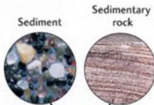
Sedimentary rock
