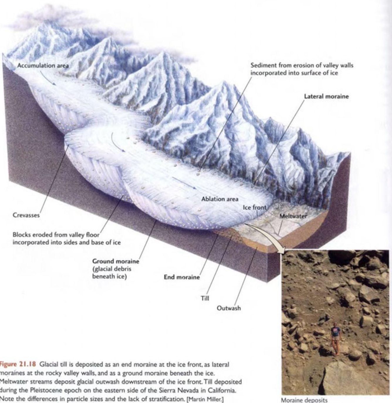
Moraine deposits
