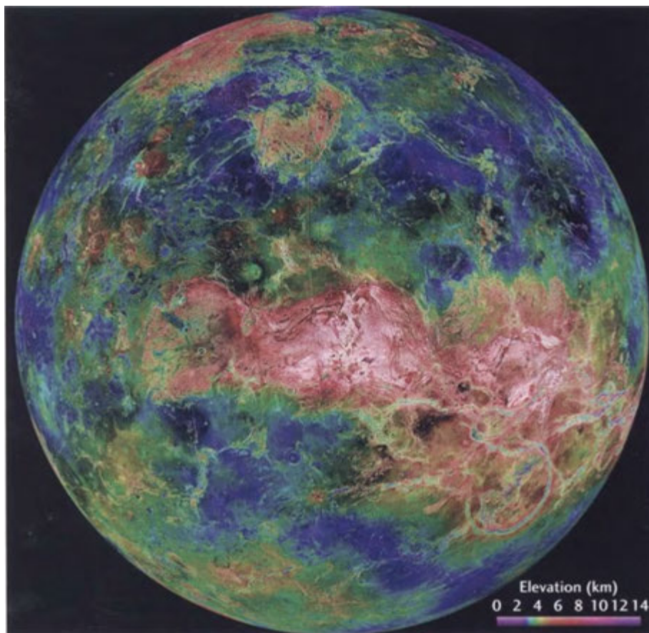
Figure 9.13 This map shows the topography of Venus based on more than a decade of mapping culminating in the 1990–1994 Magellan mission. Regional variations in height are illustrated by the highlands (tan colors), the uplands (green colors), and the lowlands (blue colors). Vast lava plains are found in the lowlands. [NASA/USGS.]
