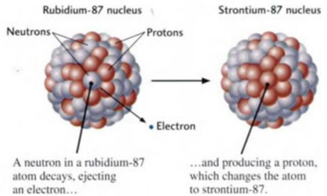
Figure 8.12 The radioactive decay of rubidium to strontium.
