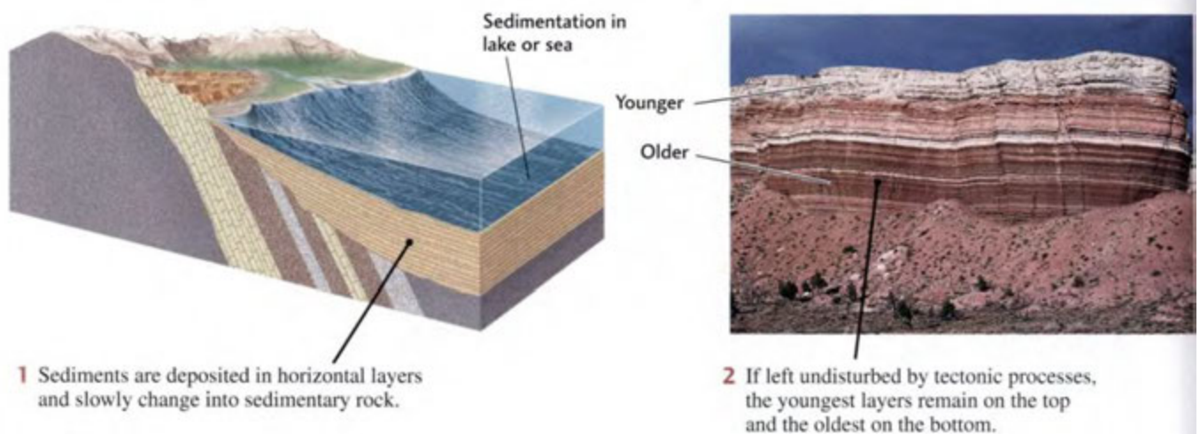
Figure 8.4 Layers of sedimentary rock in Marble Canyon, part of the Grand Canyon. The Grand Canyon was cut by the Colorado River through what is now northern Arizona. These
