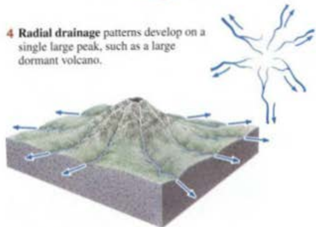
Figure 18.7 Typical drainage networks.
