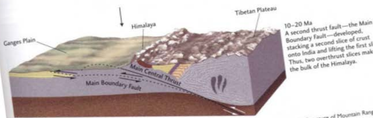
Figure 10.15 Cross sections showing the sequence of events that caused the Himalayan orogeny, simplified and vertically
