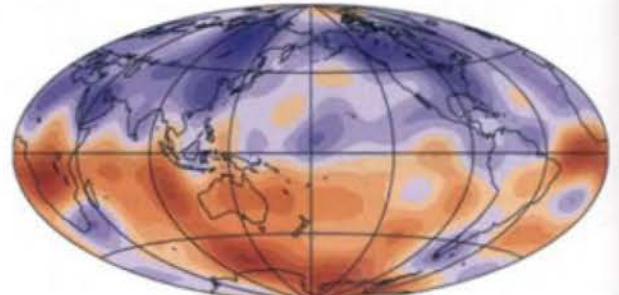
(c) Magnetic field mapped at core-mantle boundary in 2000
