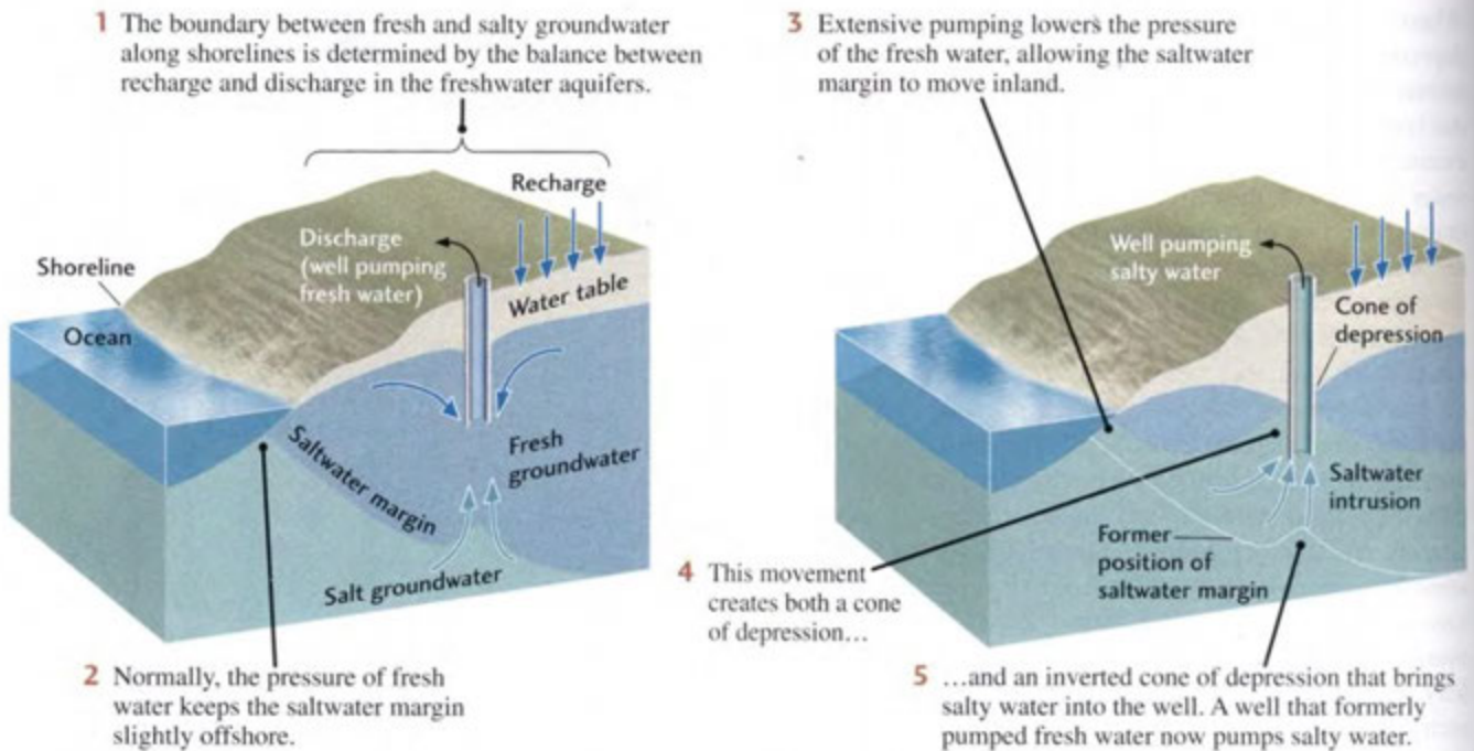
Figure 17.14 The balance between recharge and discharge maintains the freshwater-seawater boundary.
