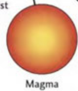
Magma
