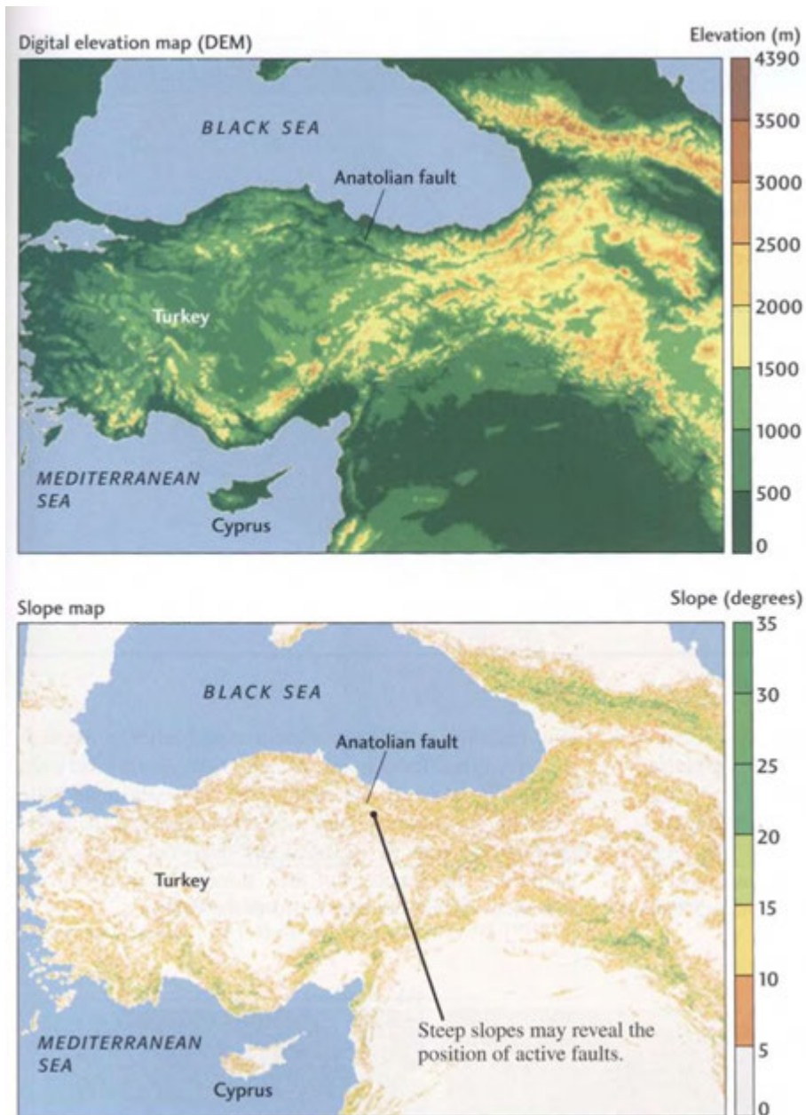
Figure 22.2 Topographic maps for Turkey and adjacent areas. Elevations can be obtained digitally from satellites to produce several types of maps. The top map shows elevation. Because the values are depicted digitally, each pixel representing one elevation value, this type of map is called a Digital Elevation Model, or DEM. In the bottom map, elevation values from the top map are used to calculate the slopes between adjacent pixels. The slopes are then represented by angles measured in degrees from horizontal. A slope map is very useful for identifying places where the changes in topography are particularly abrupt, such as along the front of mountain ranges or along active fault scarps. [Marin Clark.]
