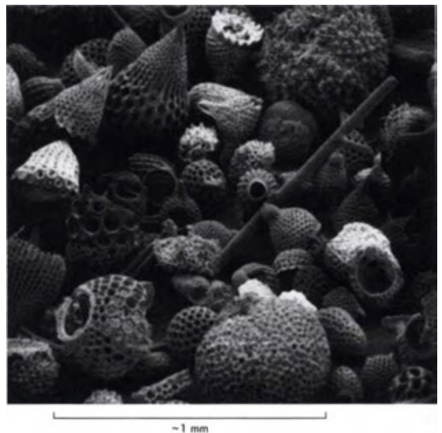
Figure 20.23 Scanning electron micrograph of oceanic ooze. Shown here are shells of both carbonate- and silica-secreting unicellular organisms. [Scripps Institution of Oceanography, University of California, San Diego.]
