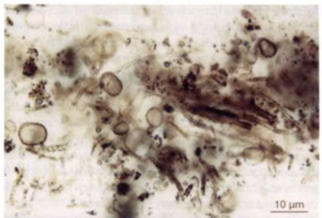
Figure 11.15 (b) By 2.1 Ga, microfossils were well preserved and abundant in the Gunflint formation, southern Ontario, Canada. [Images courtesy of H. J. Hofmann.]
