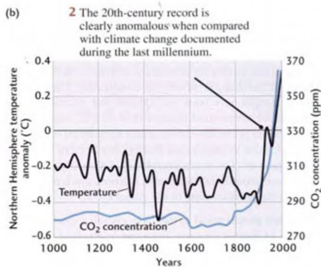
with the increase in CO 2 caused by human activities since the industrial revolution. [IPCC, Climate Change 2001: The Scientific Basis .]
