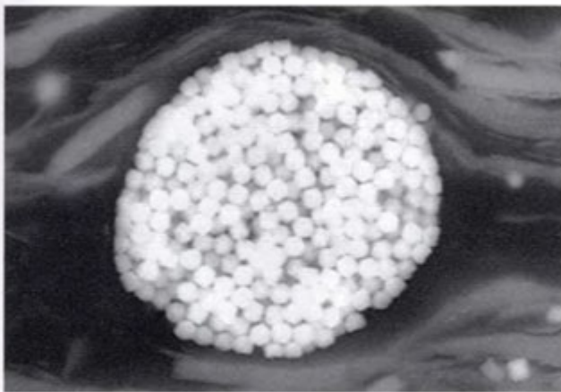
Figure 11.10 Pyrite commonly forms small globules in sediments that have anaerobic pore waters. Microbes use the sulfur in seawater and the iron dissolved from nearby minerals to precipitate pyrite. [Courtesy of Juergen Schieber.]
