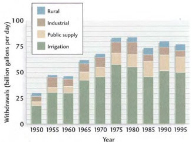
Figure 17.16 Groundwater withdrawals, United States, 1950–1995. [U.S. Geological Survey.]
