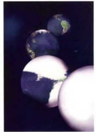
distribution of Permian-Pennsylvanian glacial deposits today. (b) Permian glacial deposits from South Africa. [John Grotzinger.] (c) Late Proterozoic glacial deposits. [John Grotzinger.] (d) The development of a late Precambrian Snowball Earth. Geologists debate the extent to which ice covered the globe, but some think even the oceans became frozen.
