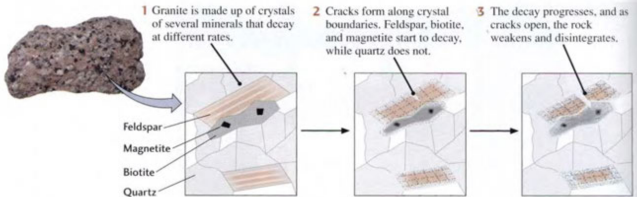
Figure 16.2 Diagrammatic microscopic views of stages in the disintegration of granite. [John Grotzinger/Ramón Rivera-Moreno/Harvard Mineralogical Museum.]
