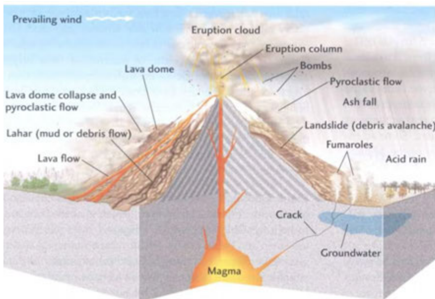
Figure 12.25 Some of the volcanic hazards that can kill people and destroy property. [B. Meyers et al./USGS.]
