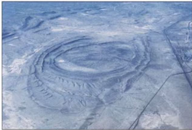
Oldest formation exposed on the surface
