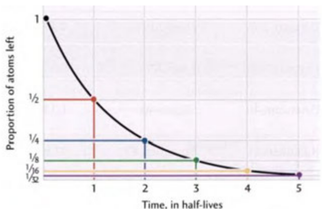
Figure 8.13 The number of radioactive atoms in any mineral declines at a fixed rate over time. This rate of decay is given by the half-life of the isotope.
