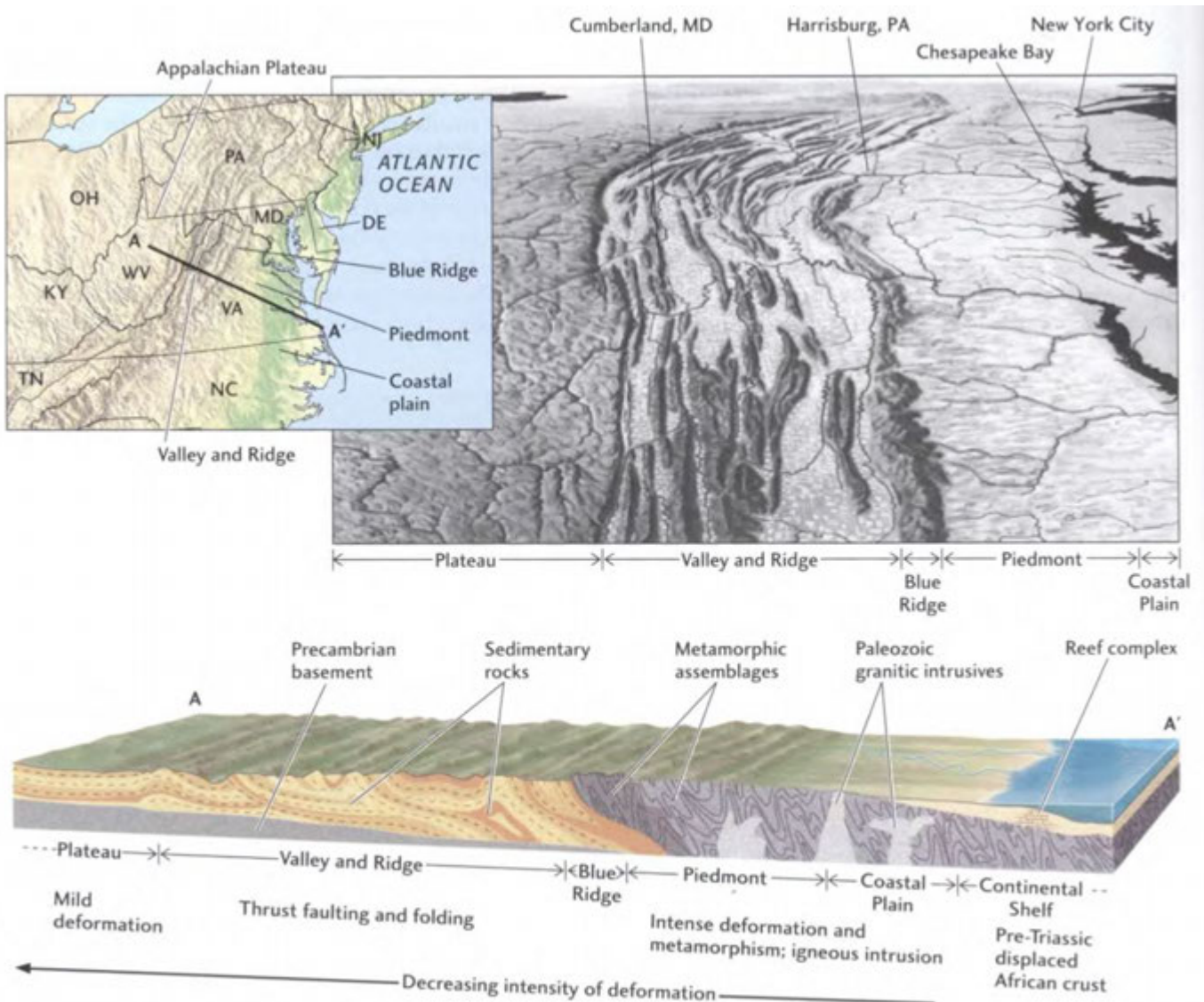
Figure 10.4 The Appalachian Mountain region of the south and central eastern United States, with an aerial view to the northeast and an idealized cross section. The major physiographic
