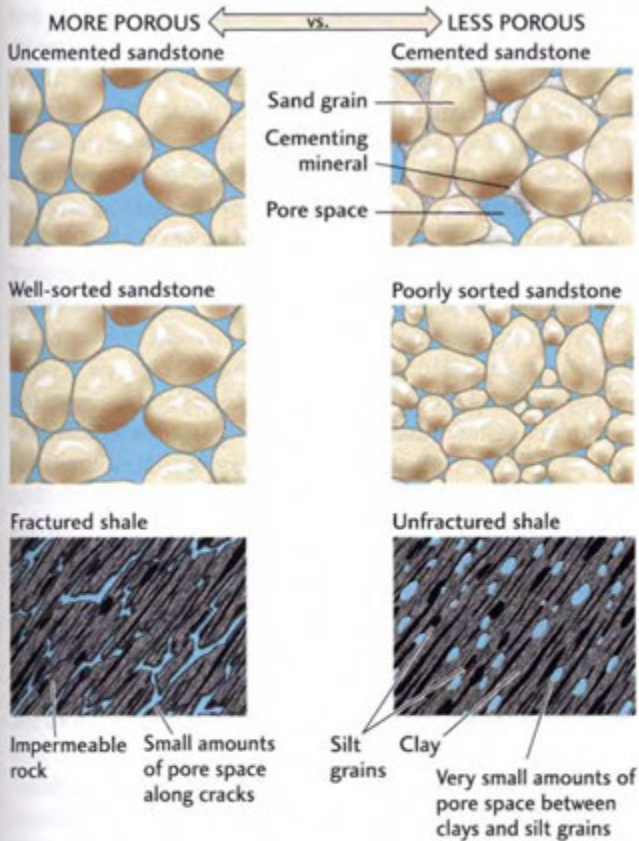
Figure 17.7 Pores in rocks are normally filled partly or entirely with water. (Pores in oil- or gas-bearing sandstones and limestones are filled with oil or gas.)
