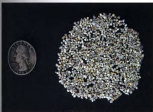
Well-sorted sand
