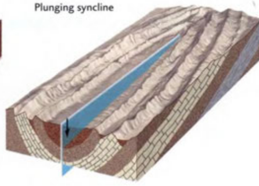
Figure 7.11 The geometry of plunging folds. Note the converging pattern of the layers where they intersect the surface, which you can also see in Figure 7.4.
