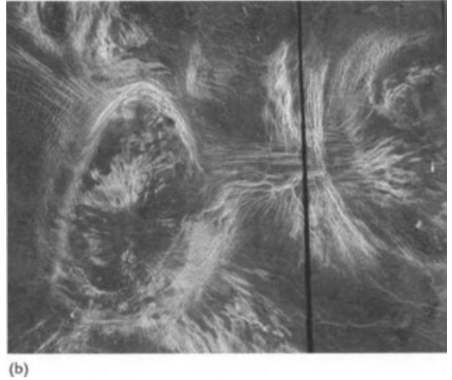
coronae are fractures, faults, and folds produced when a large blob of hot lava collapsed like a fallen soufflé. Each corona is a few hundred kilometers across. [Images from NASA/USGS.]
