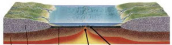
Continental lithosphere
