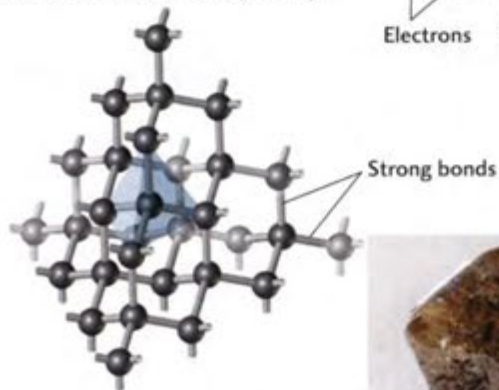
Diamond
