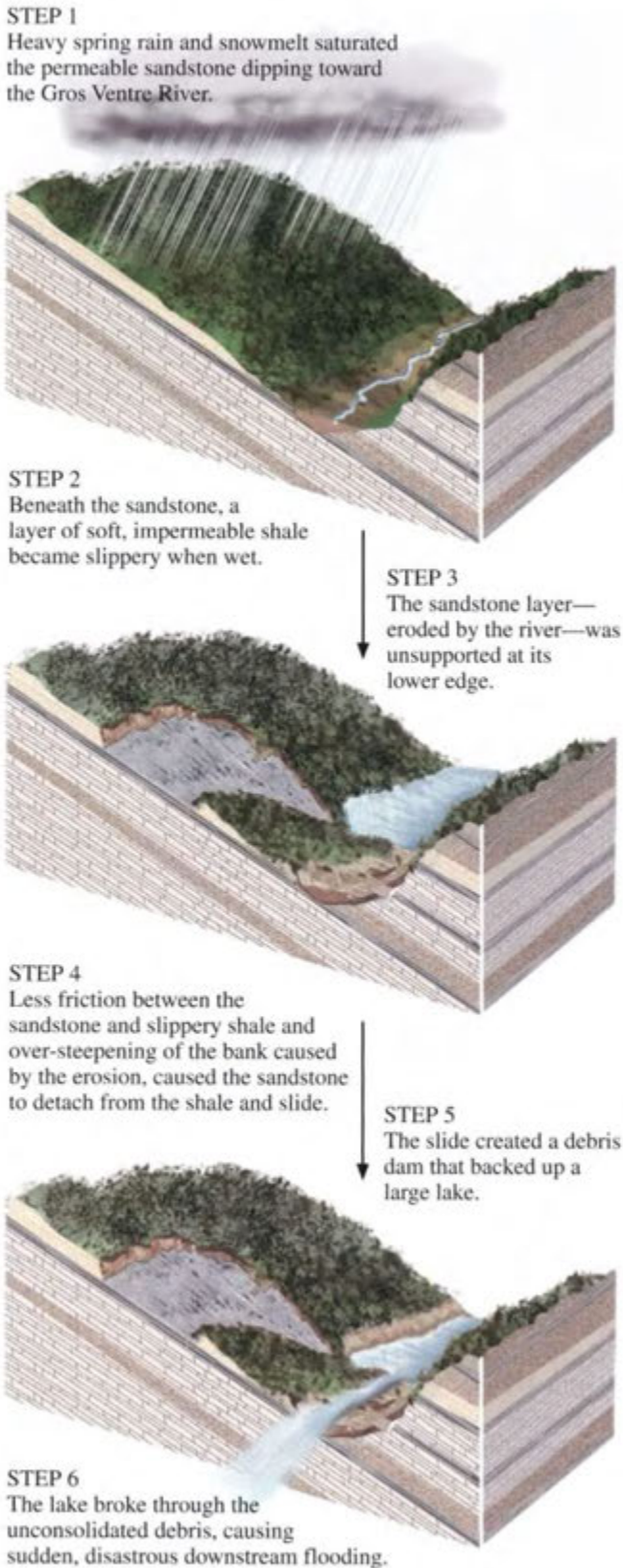
Figure 16.27 The 1925 Gros Ventre slide. [After W. C. Alden, "Landslide and Flood at Gros Ventre, Wyoming," Transactions of the American Institute of Mining, Metallurgical, and Petroleum Engineers (1928): 345–361.] The Gros Ventre landslide, Grand Teton National Park, Wyoming. [Steven Dutch.]
