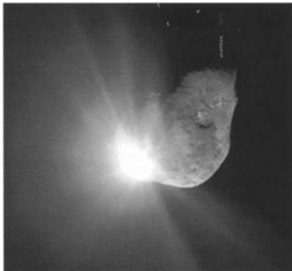
Figure 9.27 The image shows the first moments after Deep Impact's probe collided with comet Tempel 1. The debris from the interior of the comet is expanding from the impact site. [NASA/J PL-Caltech/UMD.]
