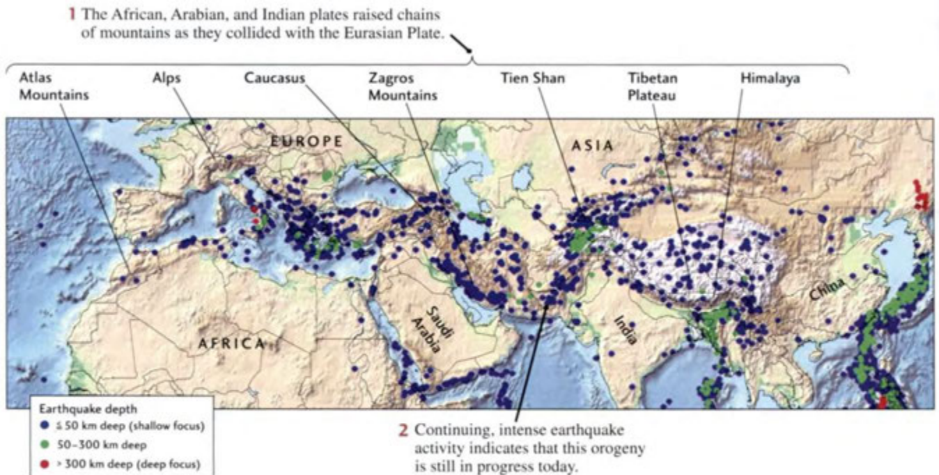
Figure 10.14 The Alpine-Himalayan belt showing the chains of high mountains built by the ongoing collision of the African,
