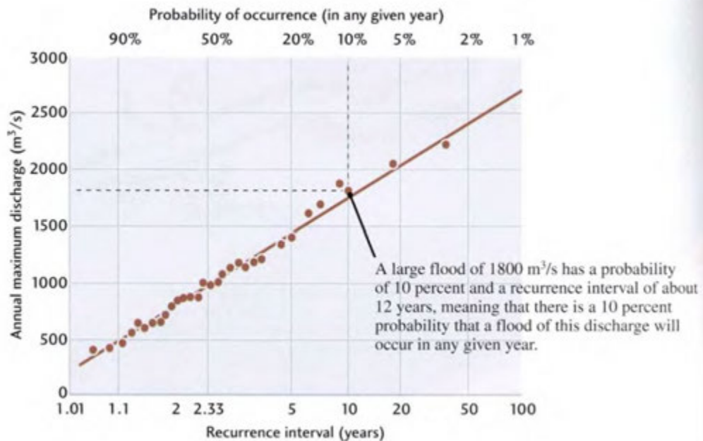
Figure 18.21 The flood-frequency curve for annual floods on the Skykomish River at Gold Bar, Washington. This curve predicts the probability that a flood of a certain discharge will occur in any given year. [After T. Dunne and L. B. Leopold, Water in Environmental Planning . San Francisco: W. H. Freeman, 1978.]
