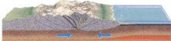
6 As two continents collide, orogeny thickens the crust and builds mountains, forming a new supercontinent.
