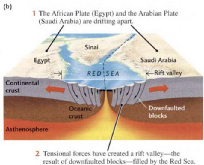
have created a rift valley, filled by the Red Sea. [NASA/TSADO/ Tom Stack.] The diagram shows parallel normal faults bounding the rift valley in the crust beneath the sea.
