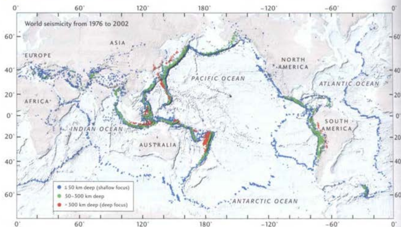
Earth System Figure 13.12 Earthquakes indicate how tectonic plates interact at their boundaries.
