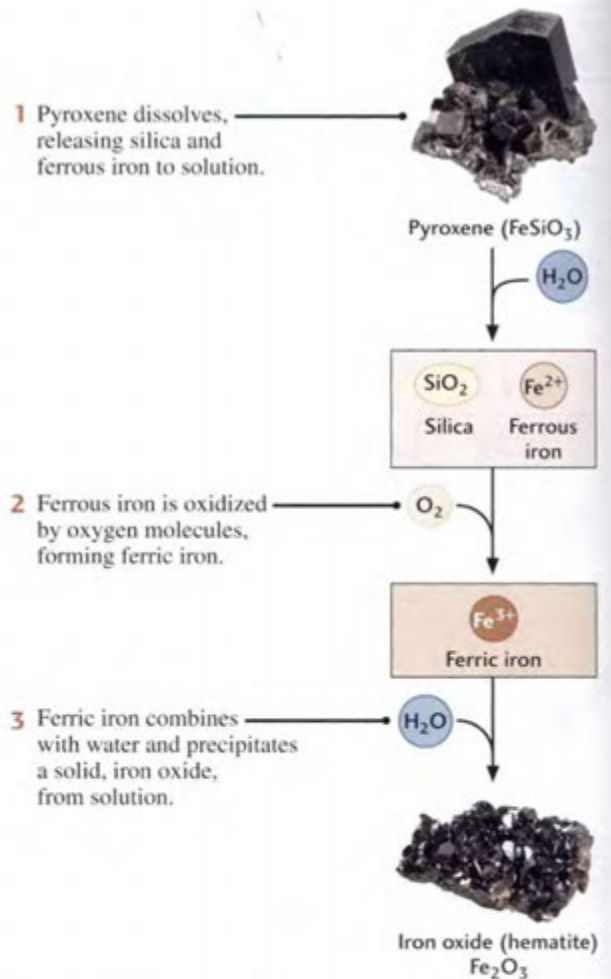
Figure 16.5 The general course of chemical reactions by which an iron-rich mineral, such as pyroxene, weathers in the presence of oxygen and water. [John Grotzinger/Ramón Rivera-Morel/Harvard Mineralogical Museum.]
