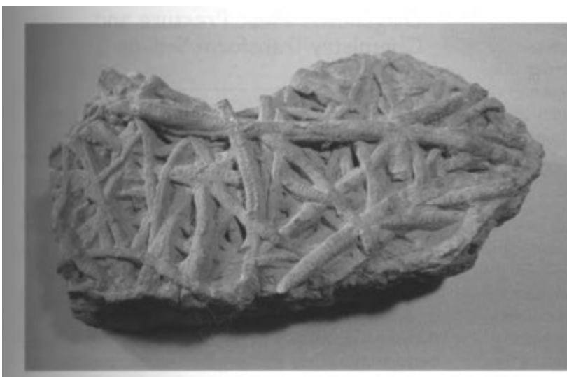
Figure 5.10 Bioturbation structures. This rock is crisscrossed with fossilized tunnels originally made as the organisms burrowed through the mud. [John Grotzinger/Ramon Rivera-Moret/Harvard Mineralogical Museum.]
