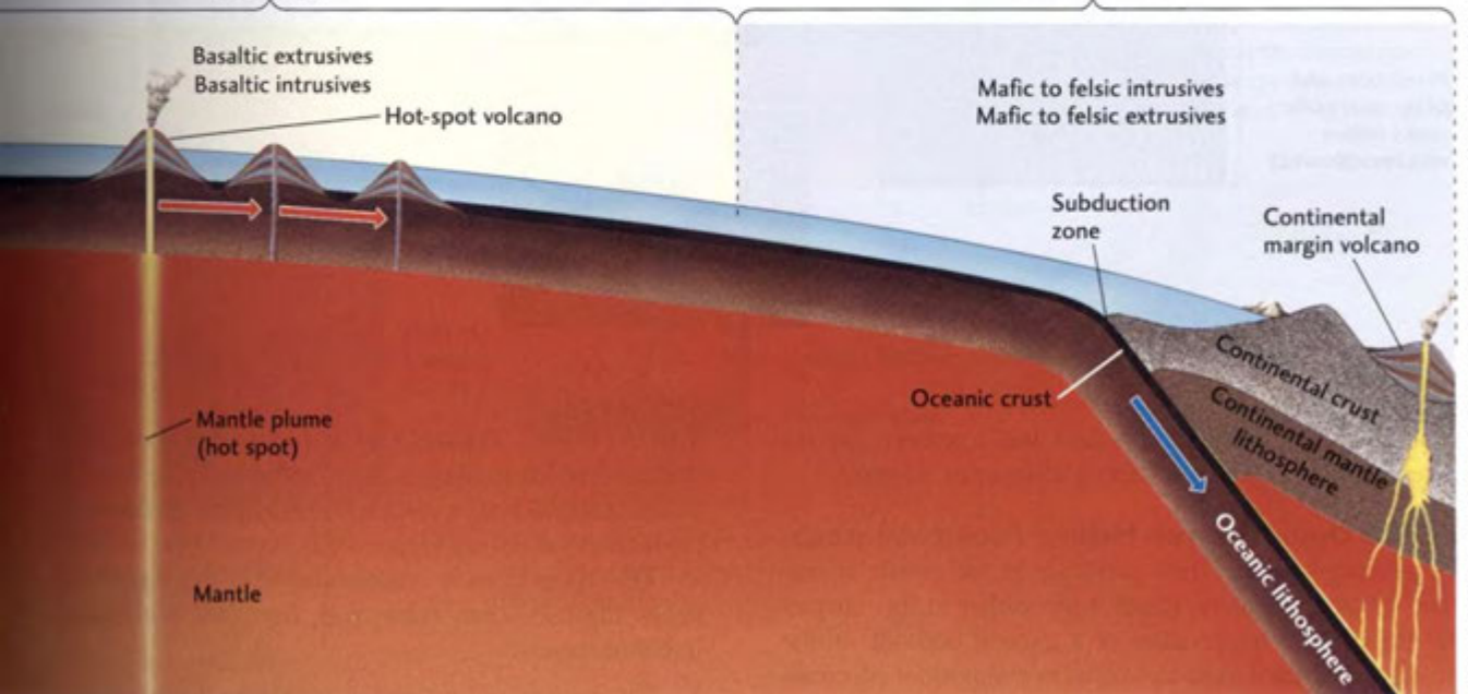
HOT-SPOT VOLCANISM
