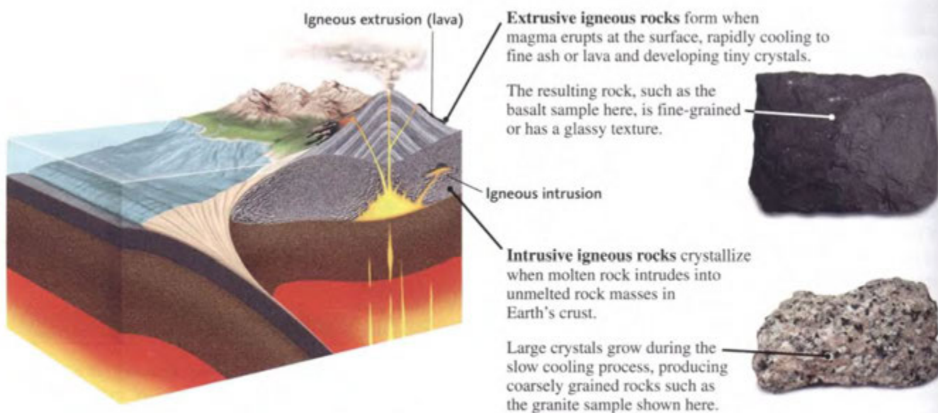
Figure 3.23 The formation of extrusive igneous rocks (basalt is shown here) and intrusive igneous rocks (granite is shown here). [John Grotzinger/Ramón Rivera-Morete/Harvard Mineralogical Museum.]
