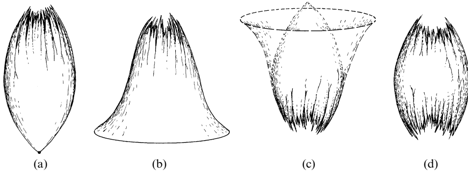
Fig. 27.20 (a) If, in the case K > 0, \Lambda = 0 of Fig. 27.13a, we allow for irregularities, of the type that we see in our actual universe, then instead of the ‘clean’ Big Crunch of the exact Friedmann model, we get a dreadful mess of congealing black-hole singularities of enormously higher entropy ( S \approx 10^{123} ). (b) This is not dependent on \Lambda = 0 , as we could likewise consider corresponding perturbations of the time-reverse of Fig. 27.13d ( K > 0, \Lambda > 0 ) and again we get a similar enormously high entropy mess ( S \approx 10^{123} ) of congealing black holes. (c) A generic Big Bang would look like that of the time-reverse of such a generic collapse (illustrated for K > 0 and either \Lambda = 0 or \Lambda > 0 ). (d) The most ‘probable’ situation (like the curve of Fig. 27.8a)—illustrated in the case K > 0, \Lambda = 0 for clarity—bears no similarity to the actual universe, in its early stages.
