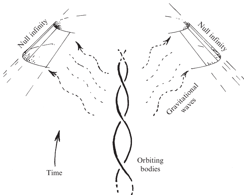
Fig. 19.10 For an isolated system emitting gravitational waves, where it may be assumed that the spacetime is asymptotically flat, there is a precise measure of total mass/energy–momentum and of its loss through gravitational radiation, referred to as the Bondi–Sachs mass/energy conservation law. The relevant mathematical quantities are non-local and defined at ‘null infinity’ (a geometrical notion which will be discussed in §27.12).
