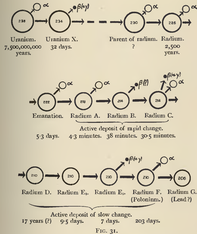
Fig. 31 shows, so far as it is at present known, the complete disintegration series of uranium.
