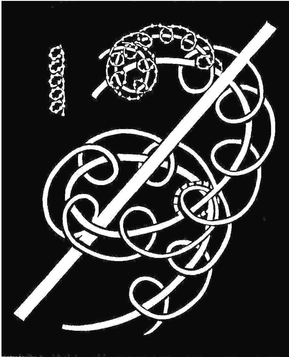
Toroidal winding of 5th-, 6th- and 7th-order spirillae of the UPA (from Occult Chemistry , 3rd ed.)
