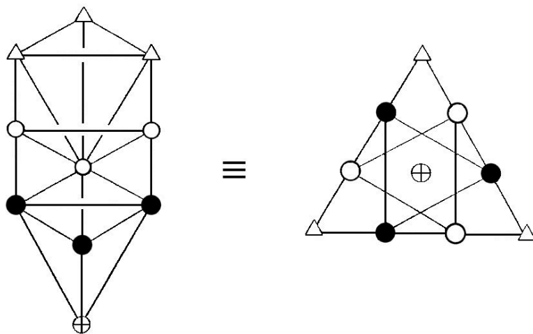
Figure 2. The tetractys.
