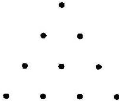
Figure 2. The tetractys.
