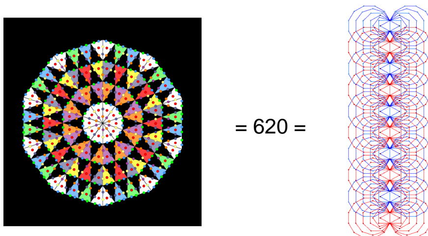
Figure 20. The number value 620 of Kether is the number of corners in the 140 polygons enfolded in 10 Trees of Life that are unshared with their outer form. It is also the number of hexagonal yods in a decagon whose sectors are 2nd-order tetractyses. It is embodied in the 120 Polyhedron built from the number 10 as the sum of its 62 vertices.
