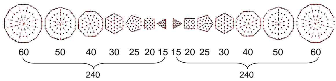
Figure 39. Each set of seven separate polygons, one the mirror image of the other, has 240 hexagonal yods. Each yod denotes a non-zero root of E_8 \times E_8' , the gauge symmetry group of heterotic superstrings. Their counterparts in the 120 Polyhedron are the 240 hexagonal yods (●) in each of the two sets of 30 faces, one the inverted image of the other.
