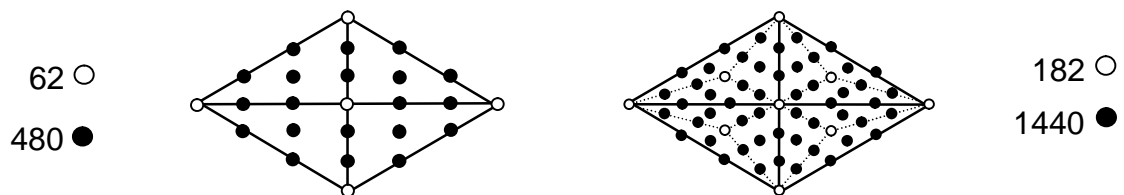
Figure 13. As single tetractyses, the 120 triangular faces of the 120 Polyhedron create 1680 geometrical elements around its axis. As three tetractyses, they generate 2400 elements. 720 elements are added by the conversion.
