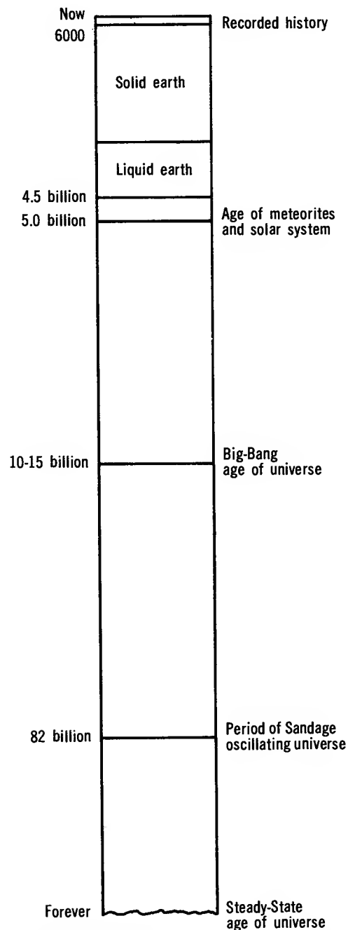
Chart history of the universe.
