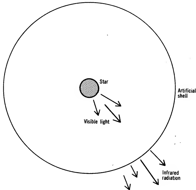
"Tamed" sun proposed by Dyson uses an artificial shell around a star to intercept all radiation, utilize its energy, and re-radiate waste heat from outside shell. The shell might be tens of millions of miles in diameter.
