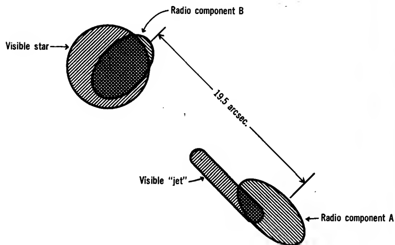
Radio and optical structure of the quasar 3C 273. The radio map was made with the help of three lunar occultations.
