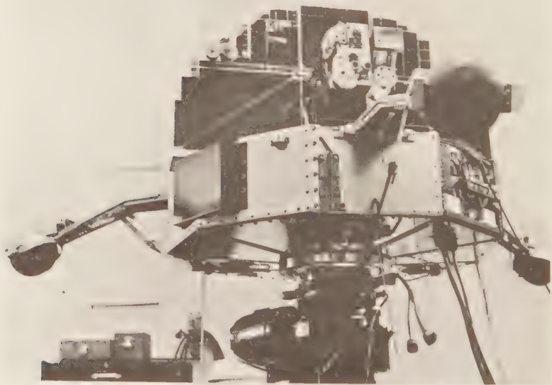
Photograph of an Orbiting Solar Observatory (OSO). Instruments mounted on the "sail" sweep back and forth across the sun's face recording its structure at wavelengths that never reach terrestrial astronomers. Nine-sided base is 112 cm across.
