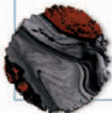
Banded obsidian Obsidian with red hematite
