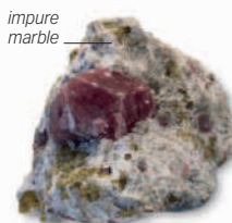
Pink grossular Rounded, pink grossular crystals in marble
