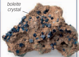
Gypsum with boleite Blue crystals of boleite seen in a matrix of gypsum
