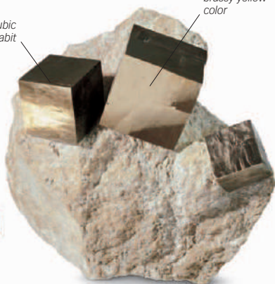
PYRITE
