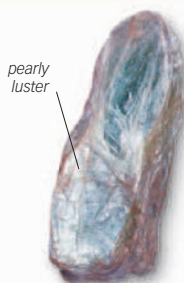
Pearly talc A pearly, toothlike piece of talc
