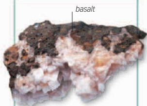
Chabazite in basalt A group of white chabazite crystals in a hollow in basalt
