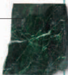
Lilac jadeite A rare and valuable variety of jadeite
