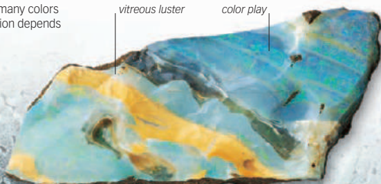
vitreous luster
