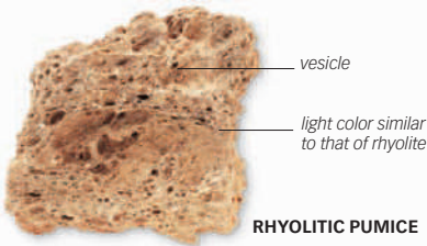
RHYOLITIC PUMICE
