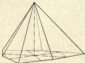
FIG. 198.—The Upper Plus Ditrigonal Hemipyramid ( hk\bar{il} ).
