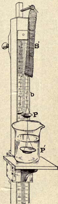
FIG. 374.—Joly Balance.
