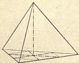
FIG. 199.—Upper Negative Trigonal Hemipyramid of the First Order, ( ohhl ).
