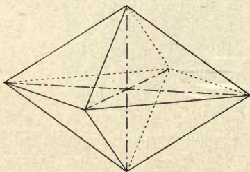
FIG. 52 a.—The Unit Pyramid of Zircon; c = 0.640 .
