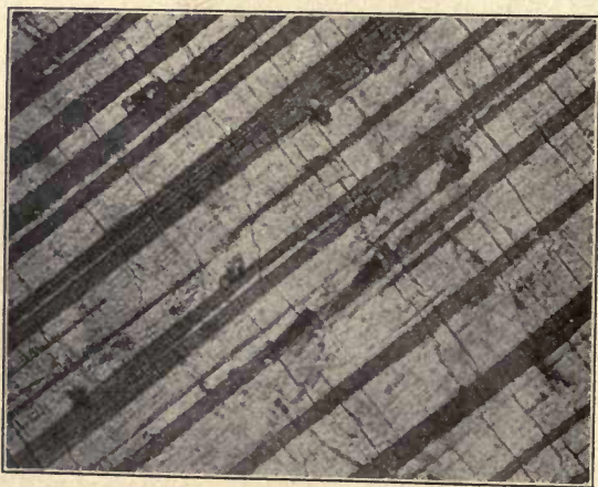
FIG. 281. — Twinning Lamellæ of Plagioclase, between Crossed Nicols. Much enlarged.
