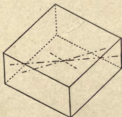
FIG. 183. — The Plus Rhombohedron of the Third Order, (hk\bar{1}l) .
