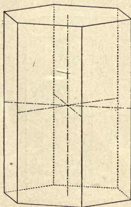
FIG. 157. — Hexagonal Prism of the First Order, a : \infty a : a : \infty c , (ho\bar{1}o) .
