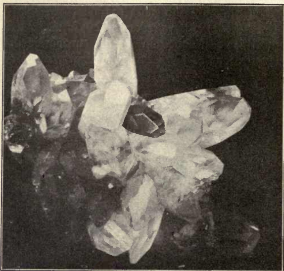
FIG. 440. — Calcite with a Scalenohedral Habit. Cumberland, England.
