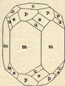
FIG. 178. — Apatite, a Combination of p(10\bar{1}1) , u(12\bar{3}1) , s(11\bar{2}1) , m(10\bar{1}0) .
