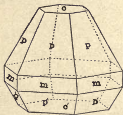
FIG. 189.—Combination of p(10\bar{1}1) , p(10\bar{1}\bar{1}) , m(10\bar{1}0) , c(0001) , c'(000\bar{1}) .
