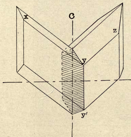
FIG. 278. — Gypsum Twins.
