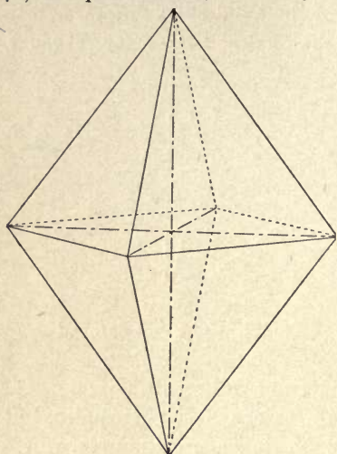
FIG. 56.—The Unit Pyramid of Barite.
