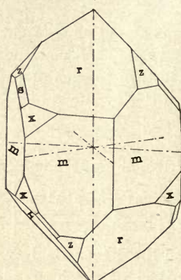
FIG. 211. — Left-handed Quartz, m(10\bar{1}0) , r(10\bar{1}1) , z(01\bar{1}1) , s(21\bar{1}1) , x(6\bar{5}11) .
