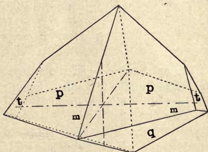
FIG. 257. — Combination of p(111) , q(11\bar{1}) , m(\bar{1}10) , t(\bar{7}71) , z(\bar{1}61) on Clinohedrite.
