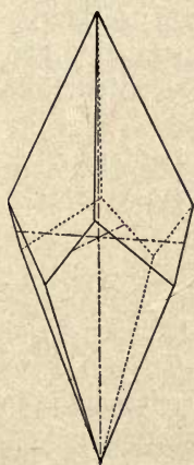
FIG. 139. — The Right Tetragonal Trapezohedron.
