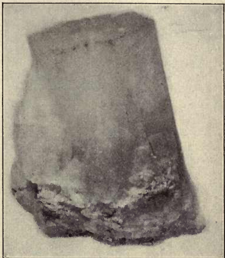
FIG. 449. — Aragonite from Herrengrund, Hungary.
