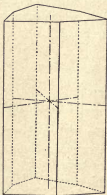
FIG. 194. — Ditrigonal Prism, (hk\bar{i}l) .
