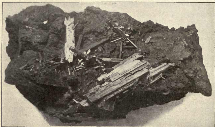
FIG. 520. — Crocoite from Dundas, Tasmania.
