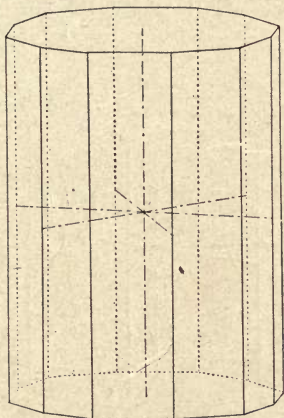
FIG. 156. — Dihexagonal Prism, na : \frac{n}{n-1}a : a : mc , (hk\bar{1}o) .
