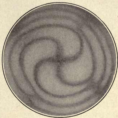
FIG. 345. — Airy's Spirals.
