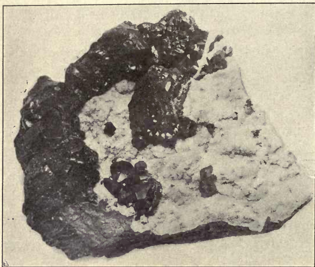
FIG. 399. — Sphalerite and Calcite. Joplin, Missouri.
