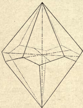
FIG. 181. — The Right Hexagonal Trapezohedron, \tau(hk\bar{l}) .
