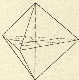
FIG. 193. — Trigonal Pyramid of the First Order, (01\bar{1}1) .
