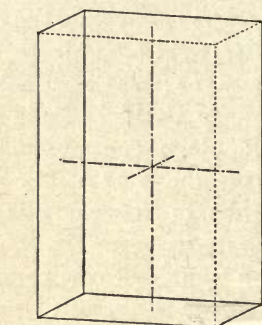
FIG. 225. — Combination of the Three Pinacoids.
