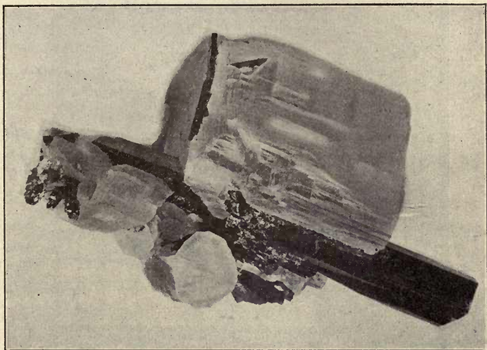
FIG. 439. — Calcite Rhombohedron r , and Epidote from Sulzbachthal, Tyrol.
