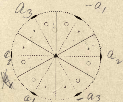
FIG. 161. — Type 19, Dihexagonal Alternating.
