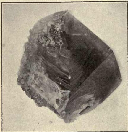
FIG. 381.—A Cube of Fluorite, showing Four Vicinal Faces replacing the Cube Face.
