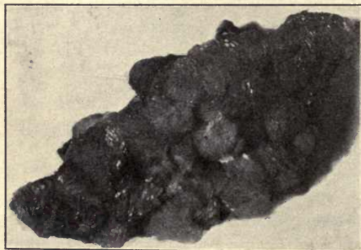
FIG. 496. — Prehnite. Bergen Hill, New Jersey.
