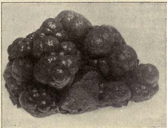
FIG. 433. — Psilomelane from Langenberg, Saxony.
