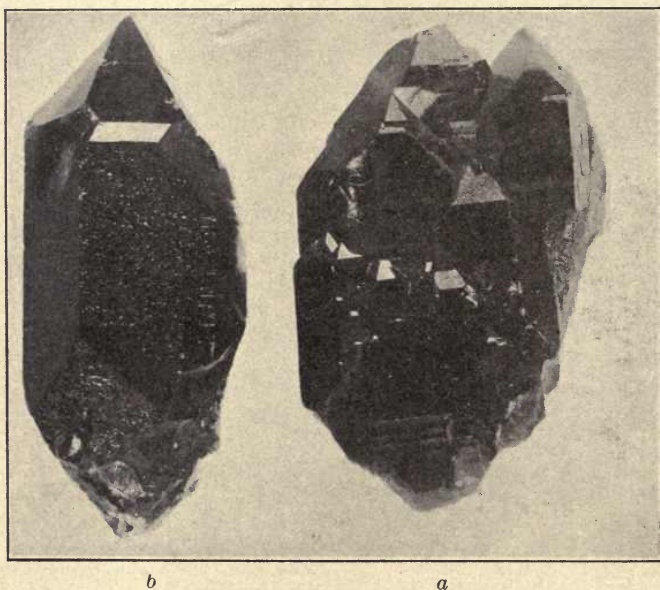
FIG. 272. — Smoky Quartz from Disentis, Switzerland.
