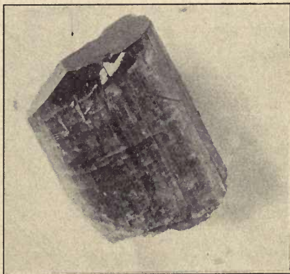
FIG. 274. — Tourmaline from Pala, California, showing Longitudinal Striations on the Prism.
