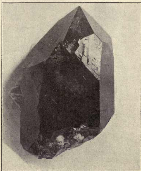
FIG. 424.—Quartz Twinned, composed of Right-hand Individuals. St. Gothard, Switzerland.
