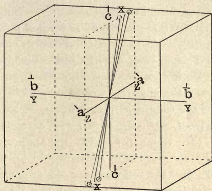
FIG. 321.—Diagram of the Optical Properties of Wollastonite.
