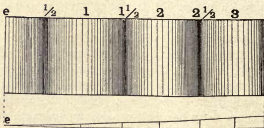
FIG. 333. — Diagram of the Quartz Wedge.
