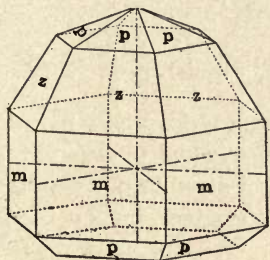
FIG. 171. — Greenockite, a combination of p(10\bar{1}1) , p(101\bar{1}) , m(10\bar{1}0) , z(20\bar{2}1) , c(0001) .
