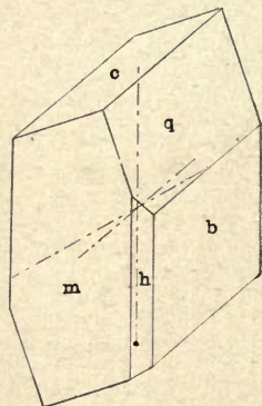
FIG. 267. — Calcium Thio-sulphate: Combinations of c(001), b(010), m(\overline{1}\overline{1}0), q(011), and h(110).
