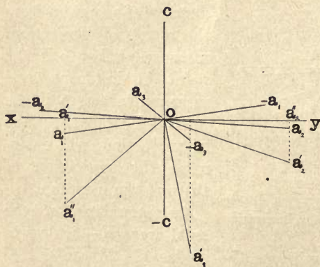
FIG. 53.—Axial Cross of Apatite; c = 0.734+ .
