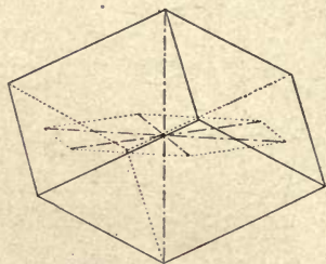
FIG. 185.—Rhombohedron of the Second Order, (hh2hl) .
