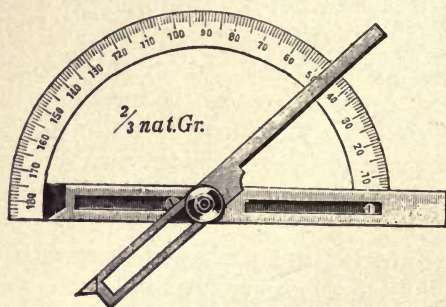
FIG. 301. — Contact Goniometer.
