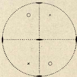
FIG. 232. — Type 6, Digonal Holosaxial.
