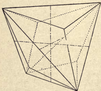
FIG. 92. — The Plus Trigonal Tristetrahedron.
