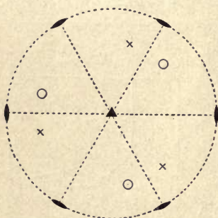
FIG. 207. — Type 10, Trigonal Holohedral.
