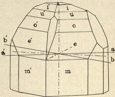
FIG. 31.—Crystal of Topaz in which the Faces c , i , u , o , e , and m are in the Same Zone, the Axis of which is aa' .
