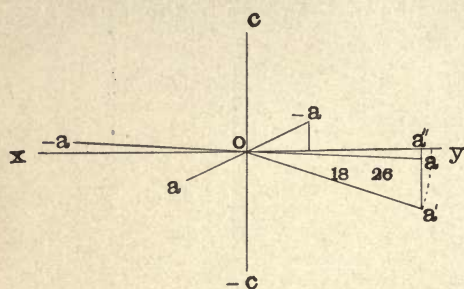
FIG. 52.—Axial Cross of Zircon; \bar{c} = 0.64+ .
