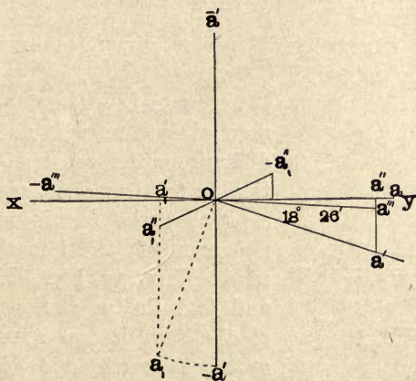
FIG. 51.—The Axial Cross of the Isometric System.
