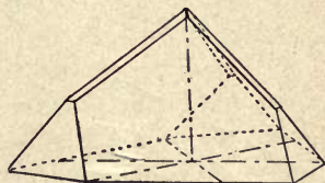
FIG. 215. — Combination of Forms showing the Polar Development of Crystals of Sodium Periodate.
