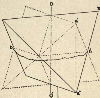
FIG. 18. — Axis of Alternating Symmetry : Chalcopyrite.
