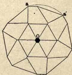
FIG. 17.—Hexagonal Axis of Symmetry: Apatite.
