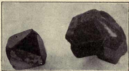
FIG. 435. — Magnetite Crystals from the Tilly Foster Mine, Brewster, New York.
