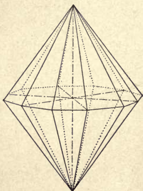
FIG. 153.—Dihexagonal Pyramid,
