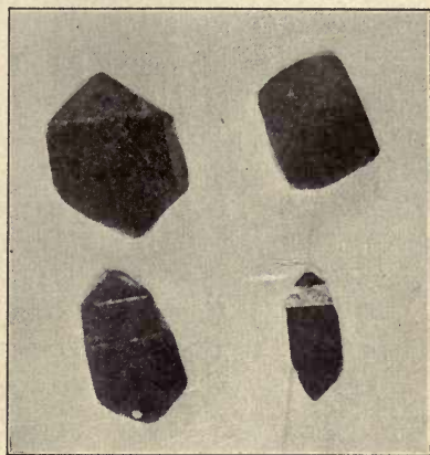
FIG. 490. — Zircon, Buncombe County, North Carolina. The Small Crystal is from Essex County, New York.
