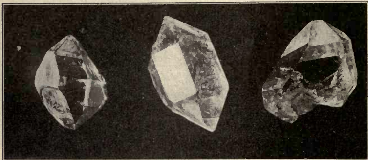
FIG. 8. — Distorted Crystals of Quartz, Herkimer County, New York.
