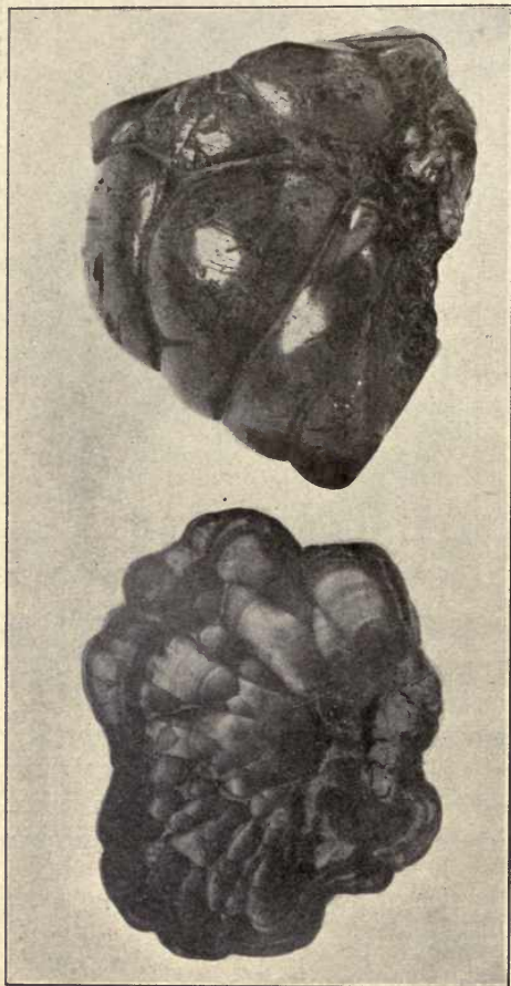
Fig. 452. — Malachite, Austria.
