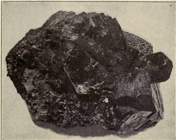
FIG. 508. — Biotite Crystals from Franklin, New Jersey.
