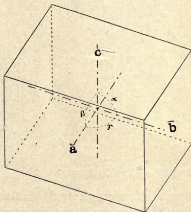
FIG. 265. — Combination of the Three Pinacoids in Rhodonite.
