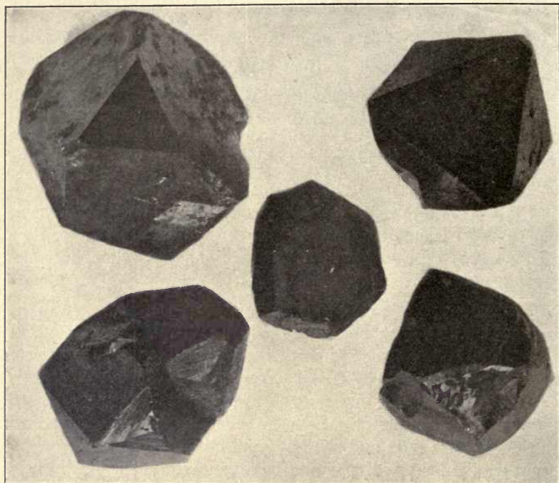
FIG. 402. — Pyrite Crystals.
