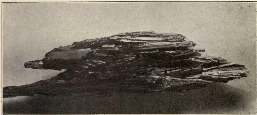
FIG. 396. — Stibnite from Lyo Island, Japan.
