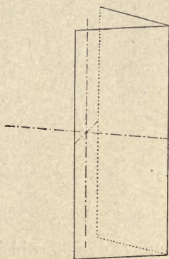
FIG. 248.—Right Hemiprism.
