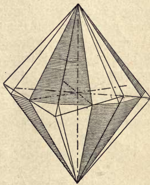
FIG. 162. — The Positive Scalehedron, k ( hhil ).
