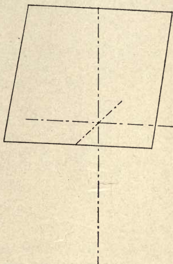
FIG. 256. — The Upper Front Hemiorthodome, (hol) .
