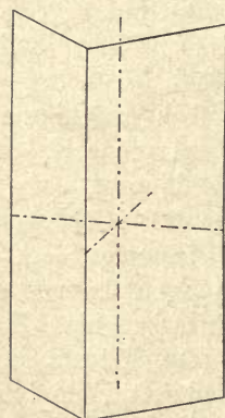
FIG. 254. — Front Hemiprism.
