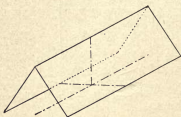
FIG. 230. — The Upper Brachydome.
