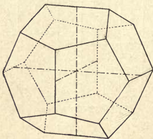
FIG. 101.—The Pyritohedron, \pi(hlo) .
