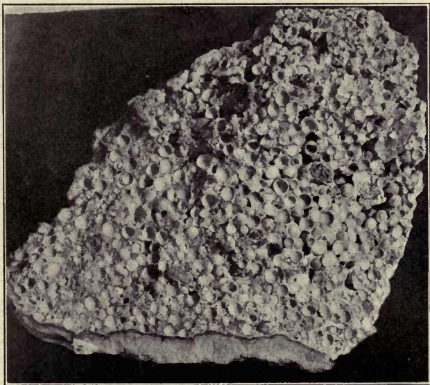
FIG. 388. — Oölitic Calcite. Carlsbad, Bohemia.
