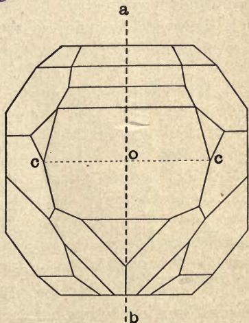
FIG. 13. — Plane of Symmetry.
