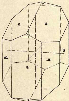
FIG. 244. — Combination of \hat{m}(110) , \hat{a}(100) , \hat{b}(010) , \hat{u}(111) , and \hat{y}(\bar{1}01) , in Augite.
