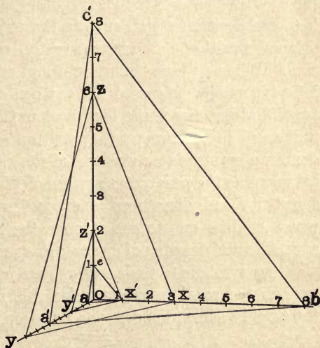
FIG. 22. — Axial Intercepts.
