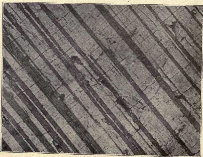
FIG. 462. — Polysynthetic Twinning in Albite, Crossed Nicols.
