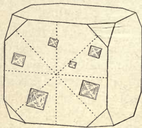
FIG. 106. — Diagram of Etch Figures on Sylvite.
