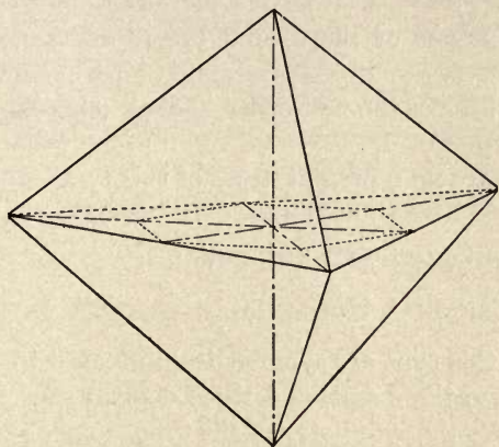
FIG. 204.—The Positive Trigonal Pyramid of the Second Order, (\overline{hh}2\overline{hl}) .
