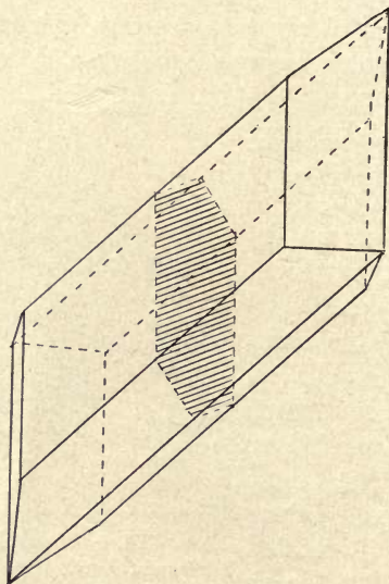
FIG. 276. — Gypsum Crystal showing the Position of the Twinning Plane.
