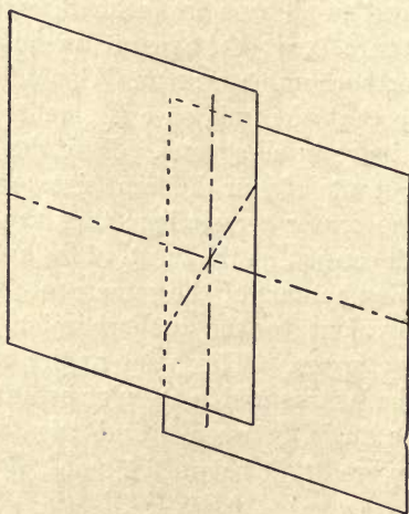
FIG. 261. — Two Faces forming a Triclinic Prism.
