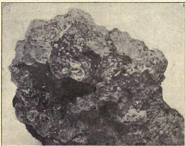
FIG. 434. — Opal Var. Hyalite from Walsch, Bohemia.
