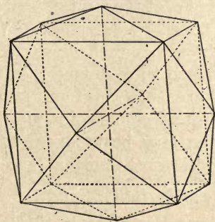
FIG. 74. — The Tetrahexahedron (320), of Fluorite.
