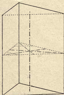
FIG. 206.—The Plus Trigonal Prism of the Second Order, (\overline{hh}2\overline{ho}) .
