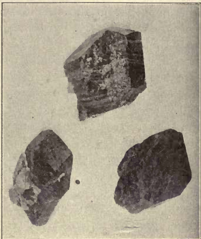
FIG. 472. — Augite from Egausville, Renfrew County, Canada.
