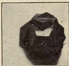
FIG. 283. — Supplementary Twins of Pyrite.
