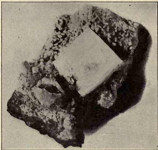
FIG. 501. — Apophyllite with Small Crystals of Albite. Paterson, New Jersey.
