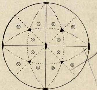
FIG. 107. — The Plus Right Tetartohedral Pentagonal Dodecahedron.
