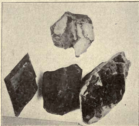
FIG. 507. — Muscovite Crystals from Woodstock, Maine.
