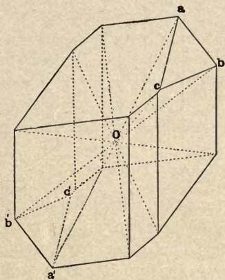
FIG. 19. — Axinite, showing a Center of Symmetry.
