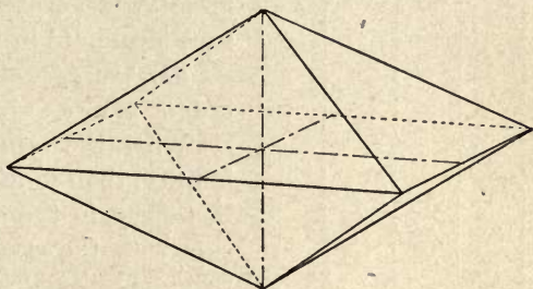
FIG. 115. — Pyramid of the Second Order, (101), of Cassiterite.
