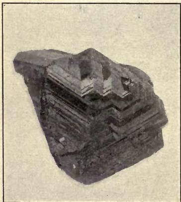
FIG. 286. — Zigzag twins of Rutile.
