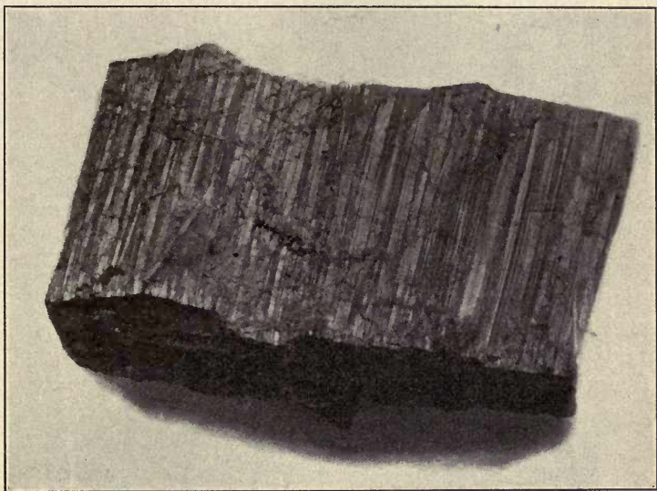
FIG. 380. — Asbestos. Thatford, Quebec, Canada.
