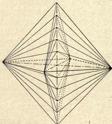
FIG. 220. — The Unit Series of Pyramids.
