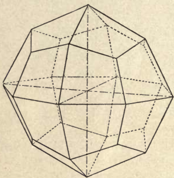
FIG. 76.—The Tetragonal Trisoctahedron, (hhl) .
