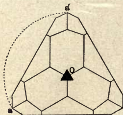
FIG. 15.—Trigonal Axis of Symmetry: Tourmaline.
