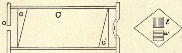
FIG. 338. — Diagram showing the Construction of the Dichroscope.
