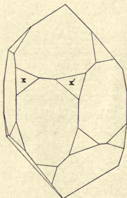
FIG. 296. — Brazilian Twins of Quartz.
