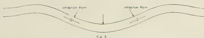
FIGURE 3. Vertical deflection caused by a point load on a beam of infinite length resting on an elastic foundation. Note the marginal uplifts and shearing displacements in the neutral plane at the inflection points.
