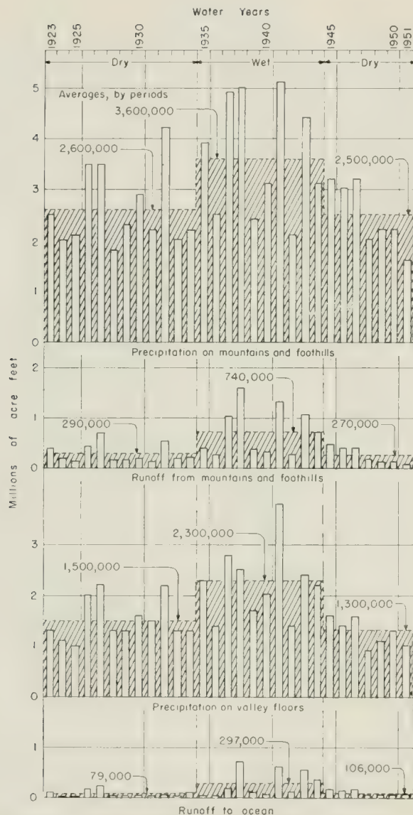
FIGURE 8. Annual precipitation and runoff in the Los Angeles region.
