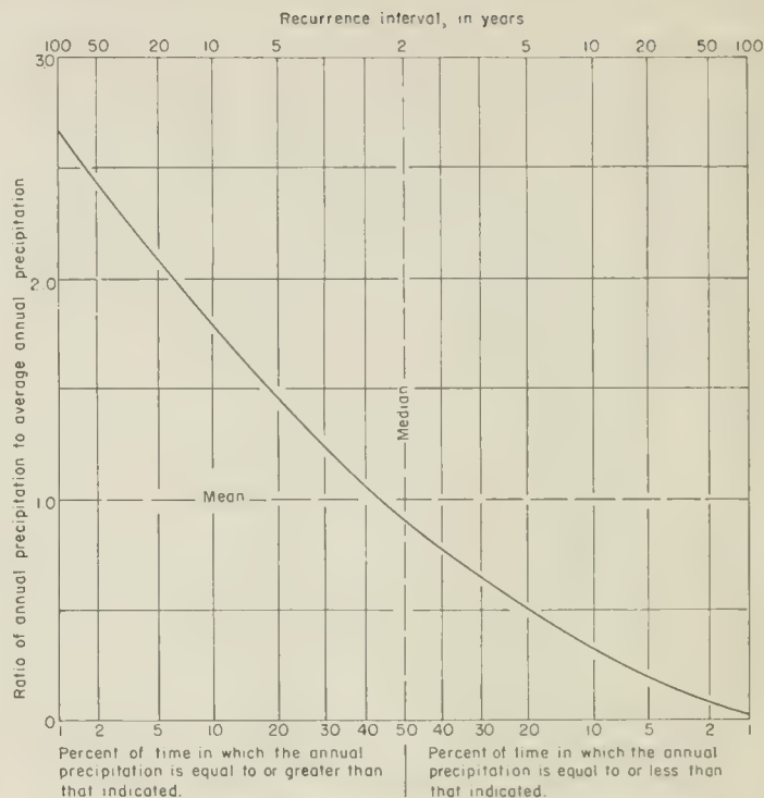
FIGURE 2. Typical frequency distribution of annual precipitation.
