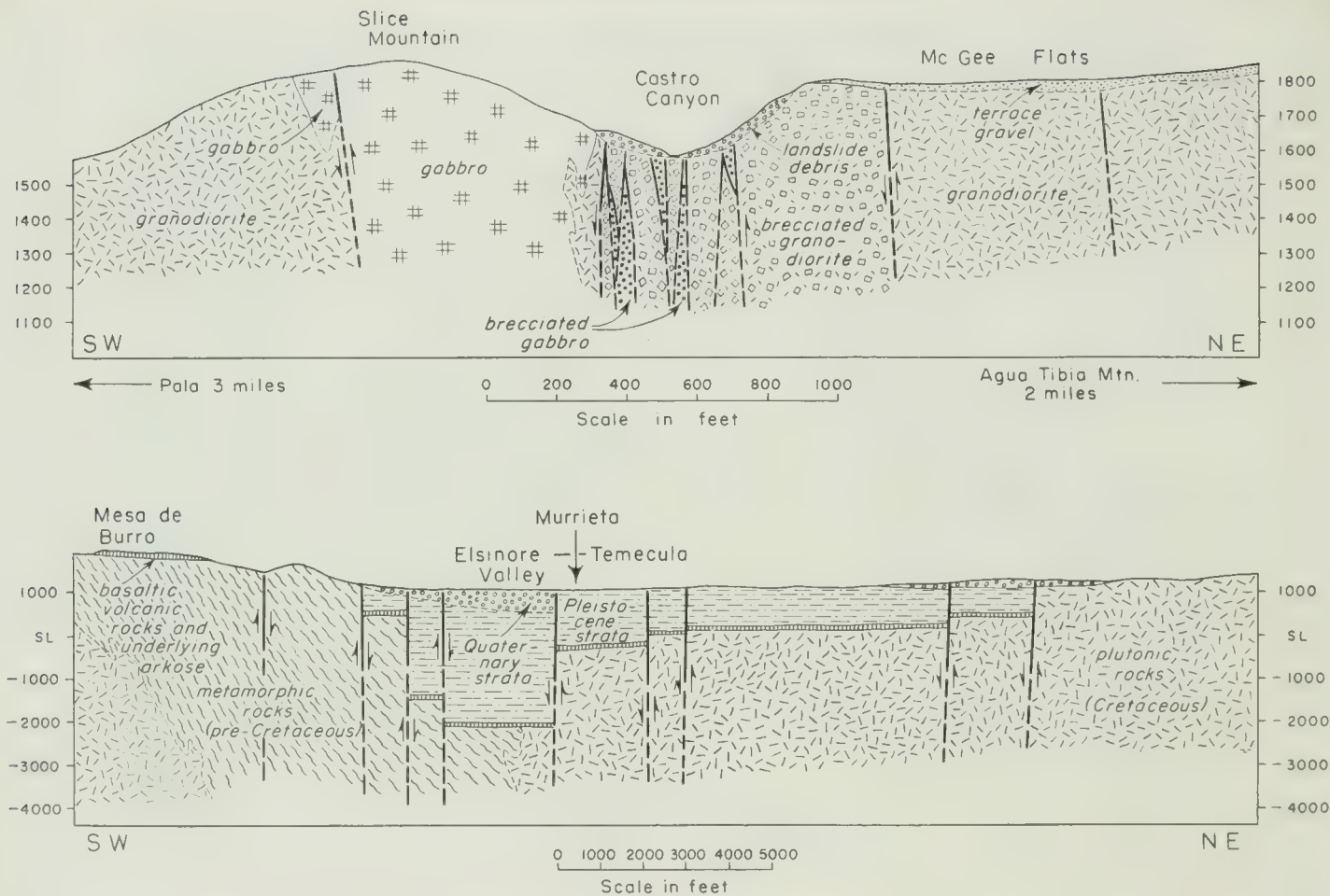
FIGURE 10. Sections across the Elsinore fault zone.
