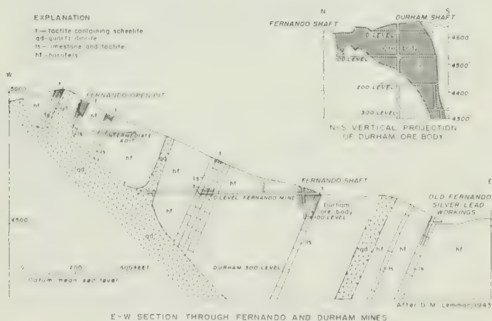
FIGURE 2. Idealized section through Fernando and Durham mines, Darwin district, Inyo County.
