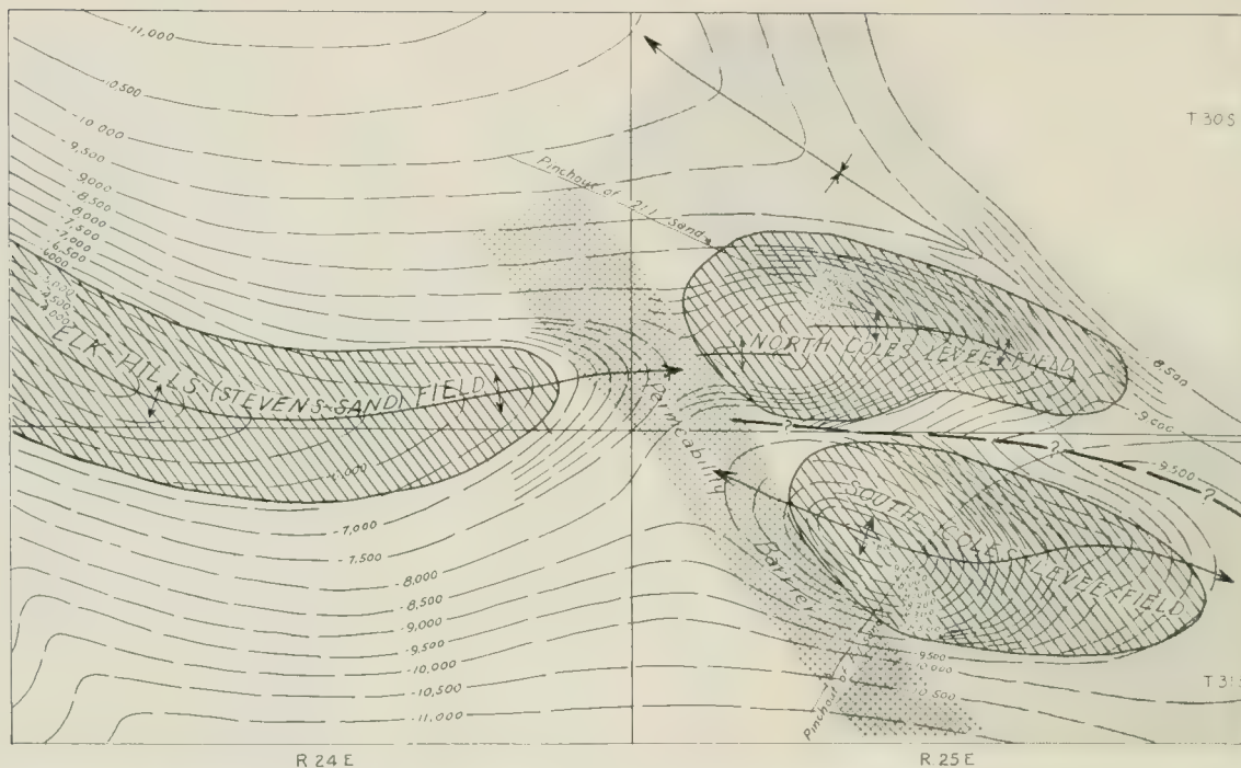
FIGURE 4. Structure-contour map of the Elk Hills-Coles Levee area, showing (1) permeability barrier in main Stevens sand separating the Elk Hills (Stevens sand) field on the west from the North Coles Levee and South Coles Levee fields on the east, (2) pinchout of 21-1 sand lens across North Coles Levee anticline, and (3) pinchout of F-1 sand lens across South Coles Levee anticline.
