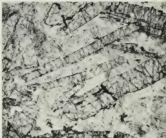
FIGURE 4. Photomicrograph of tabular bastnaesite crystals in calcite matrix. (25x, plane polarized light)
