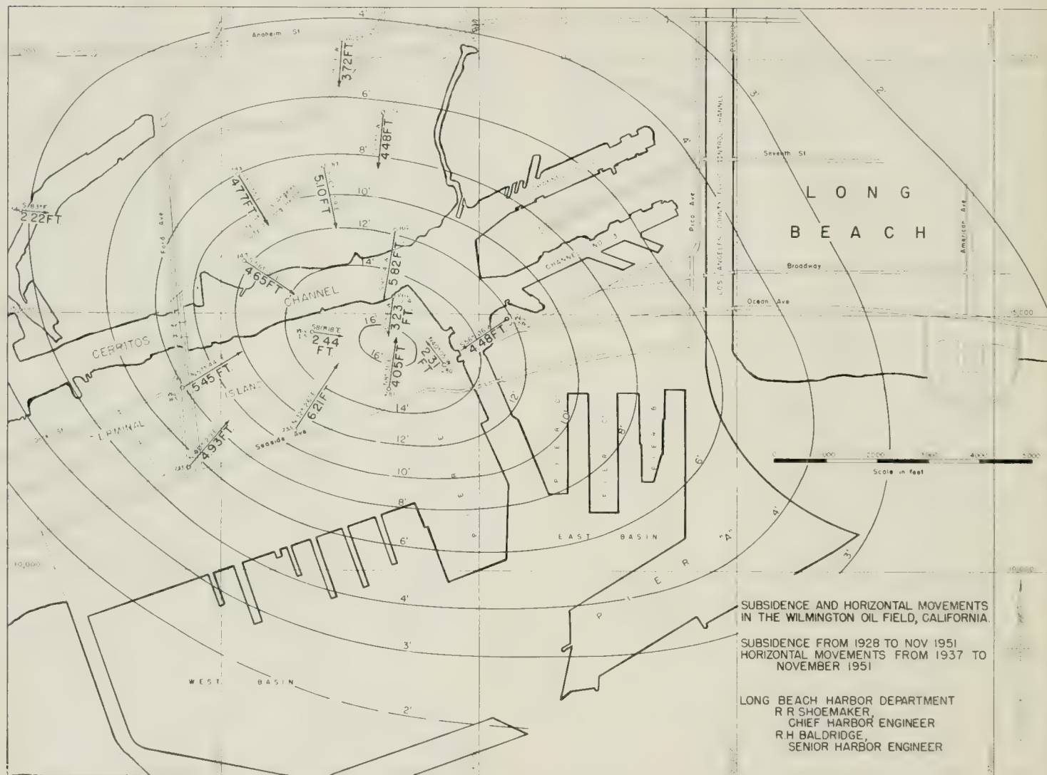
FIGURE 1. Map of Wilmington oil field, showing total subsidence and horizontal movements to November, 1951. Data chiefly from surveys by Long Beach Harbor Department and Office of Los Angeles County Surveyor and Engineer.
