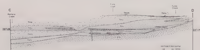
DIAGRAMATIC SOUTHWEST-NORTHEAST SECTION CD
