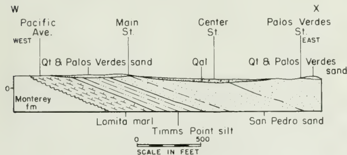
FIGURE 29. Section W-X along Second Street, San Pedro, California.
