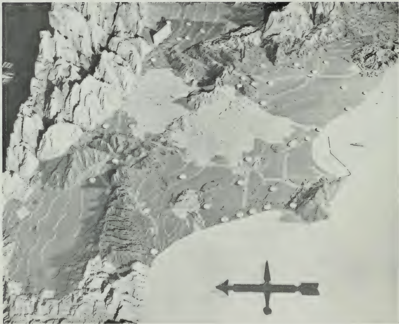
FIGURE 1. Relief map of the Los Angeles basin and adjacent mountains. Palos Verdes Hills in right foreground, Santa Ana Mountains in right background, San Gabriel Mountains in left background, and the Santa Monica Mountains in the left foreground. Map reproduced through the courtesy of the Museum of Science and Industry of California, Exposition Park, Los Angeles. Photograph by Roy V. George.
