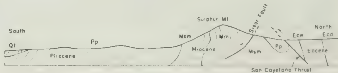
Fig. 14. North-south cross section through Sulphur Mountain.
