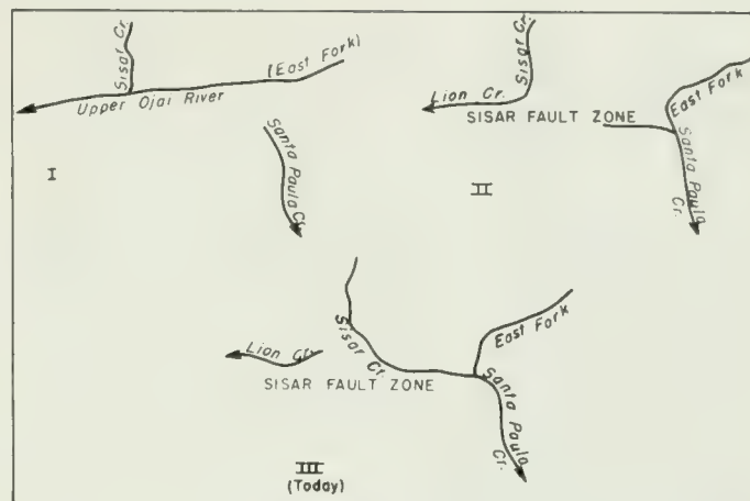
Fig. 17. Stages in capture of Sisar Creek by Santa Paula Creek.
