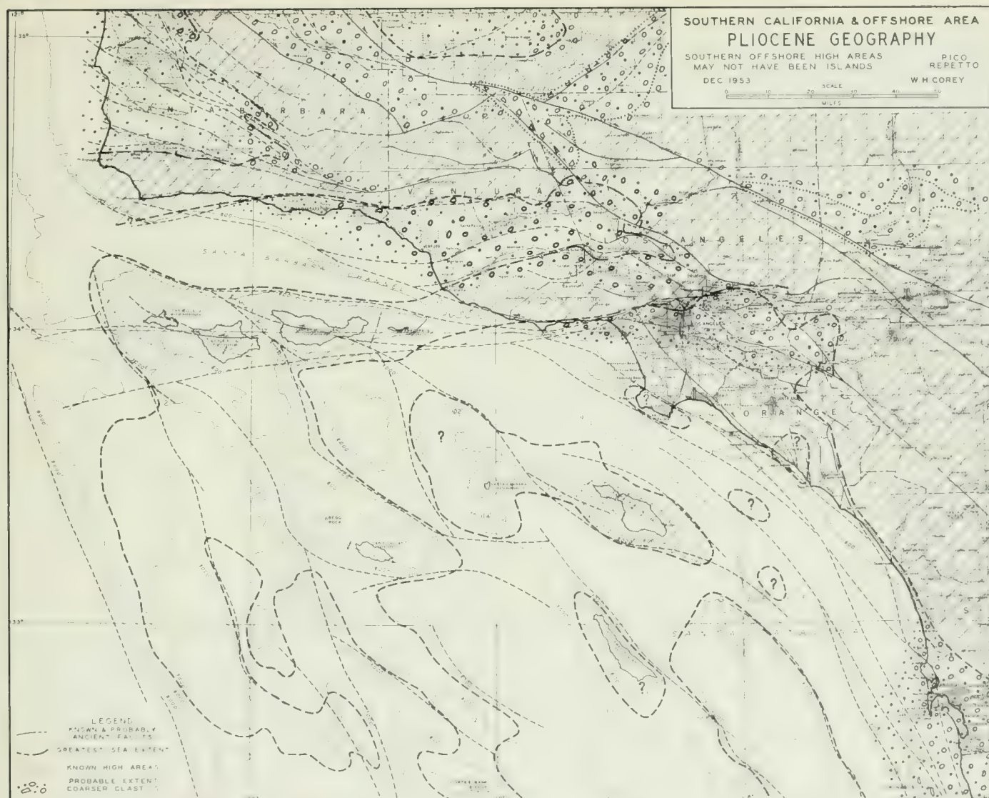
FIGURE 8. Map of a part of southern California, showing general geography and pattern of sedimentation in Pliocene time.
