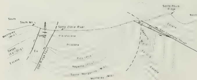
Fig. 11. Section across Santa Clara River Valley.
