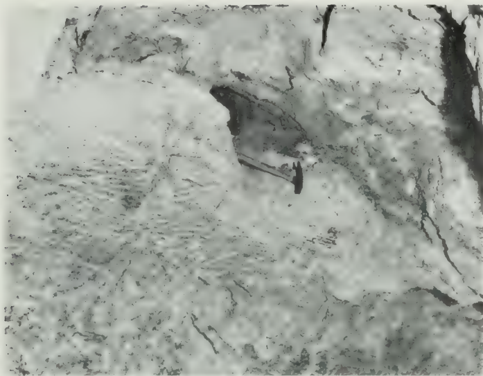
FIGURE 15. Fracture-controlled replacement masses and small fracture fillings of albite (light) in very coarse-grained quartz (dark), Pala Chief mine, Pala district. Above this striped rock is a layer of "pocket pegmatite" that has been worked for gem spodumene, and exposed in the back of the small stope is coarse-grained perthite-quartz pegmatite. Below the striped rock is albite-quartz-perthite pegmatite with subordinate muscovite and schorl.
