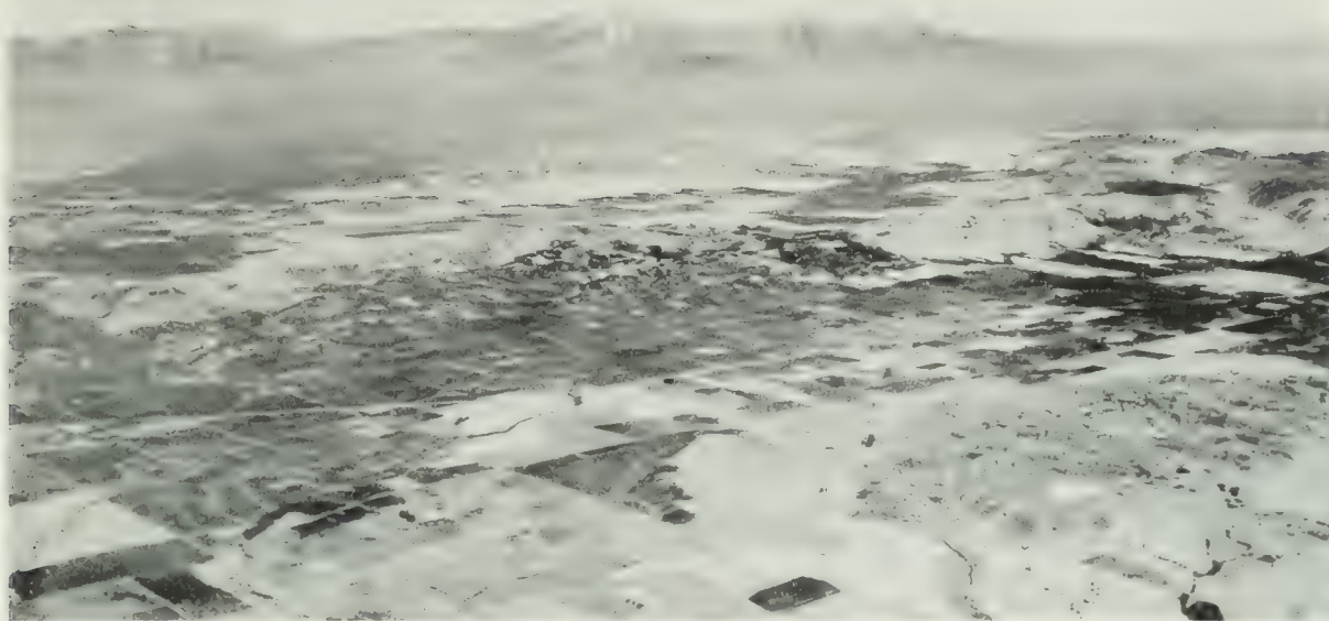
FIGURE 9. Air view northeastward from a point above Buena Park. The West Coyote oil field is at lower right. The Puente Hills extend across the center of the view, and Brea Canyon is at the extreme right. The high peak in the distant San Gabriel Mountains is San Antonio Mountain (Old Baldy Peak), altitude 10,059. Pacific Air Industries photo.
