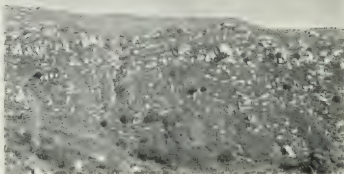
FIGURE 7. Bouldery exposures of granodiorite near the west end of the Agua Tibia Mountains. The rock is broken by two sets of steeply dipping joints, and by a third set of joints that dip gently from right to left.
