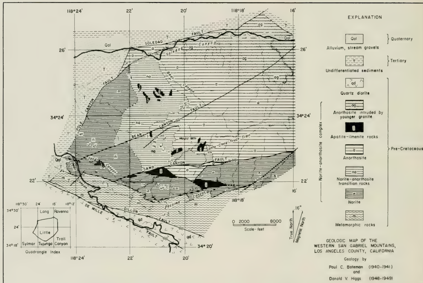
FIGURE 1. Geologic map of the western San Gabriel Mountains, Los Angeles County, California.
