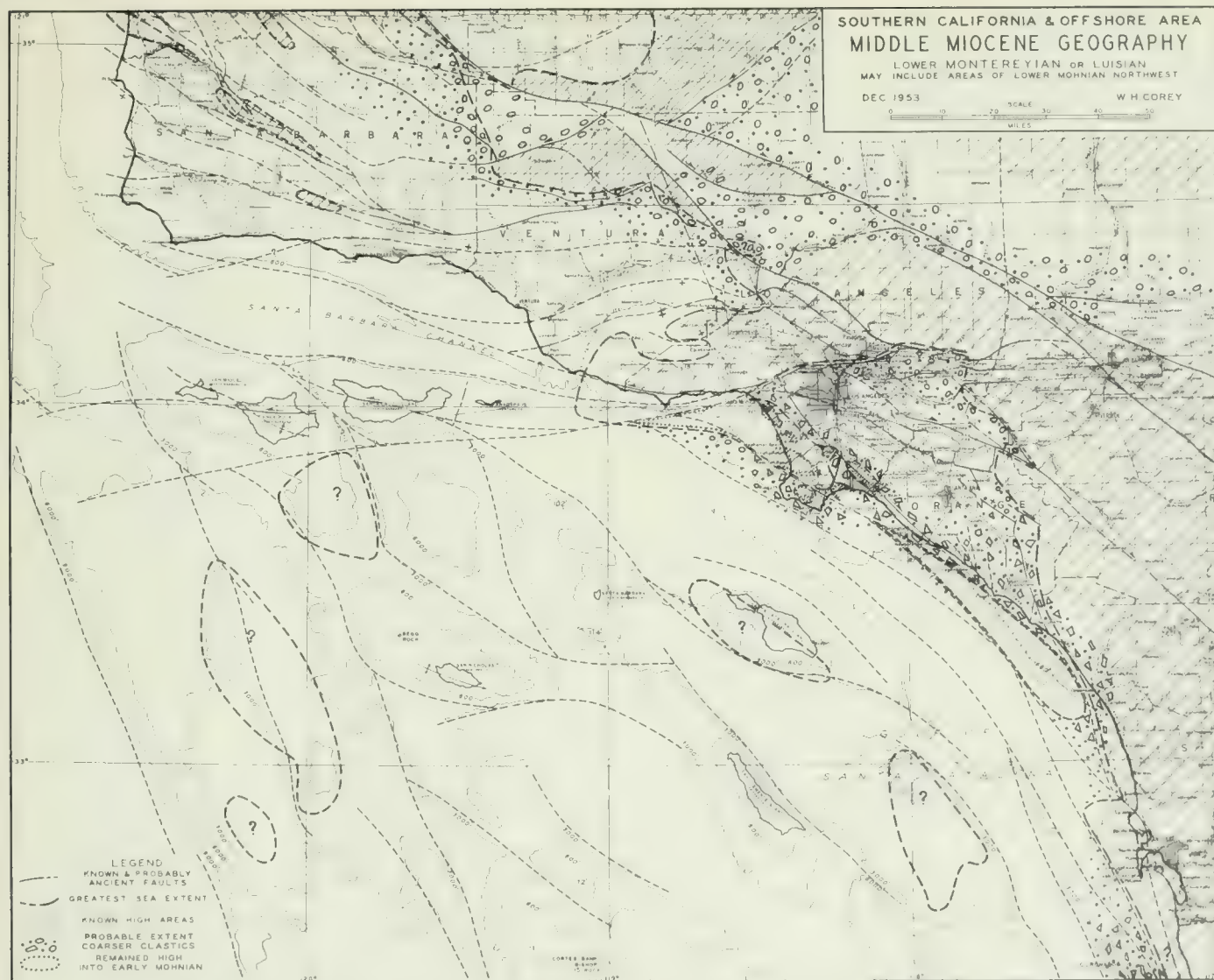
FIGURE 6. Map of a part of southern California showing general geography and pattern of sedimentation in middle Miocene time.
