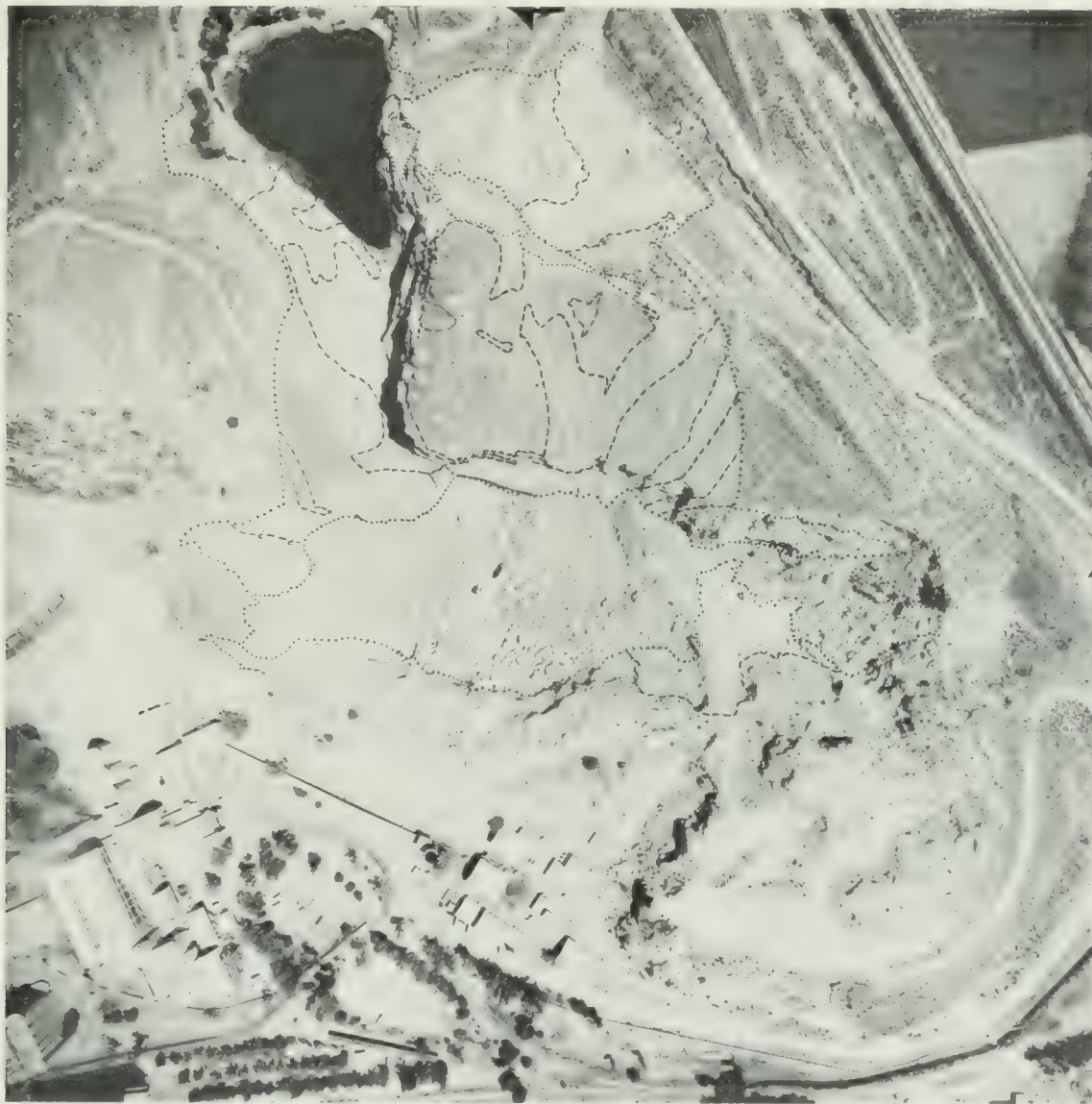
FIGURE 26. Air photograph of the Crestmore Hills and the plant and quarries of the Riverside Portland Cement Company. Contacts between major rock units are shown by means of dashed and dotted lines (see fig. 27). MacPherson Aerial Surveys photo.
