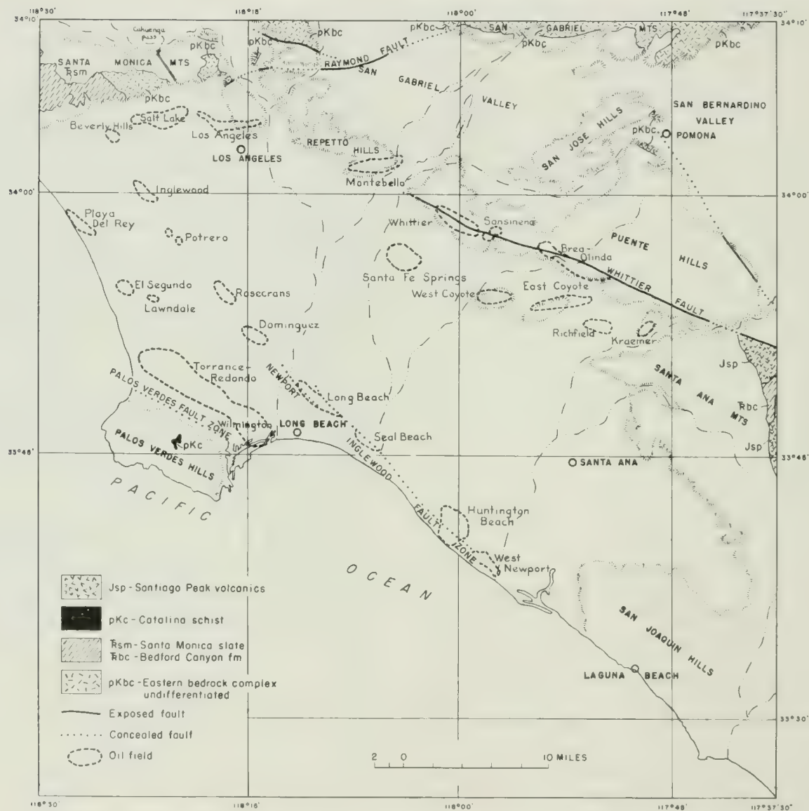
FIGURE 1. Index map of the Los Angeles basin, showing oil fields and distribution of exposed basement rocks.
