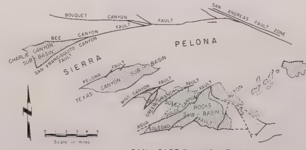
Map showing distribution of major faults, present outcrop areas of the Volcanic formation and associated volcanic rocks, and general positions of sub-basins of Volcanic deposition.
