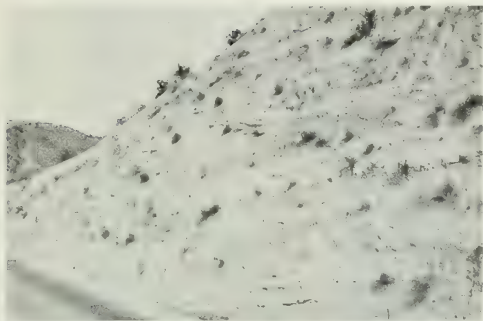
FIGURE 25. Interbedded conglomerate, sandstone, and siltstone of the upper Pliocene San Timoteo formation, U. S. Highway 60 south of San Timoteo Canyon. Note the offsets along faults in the left-hand part of the view.
