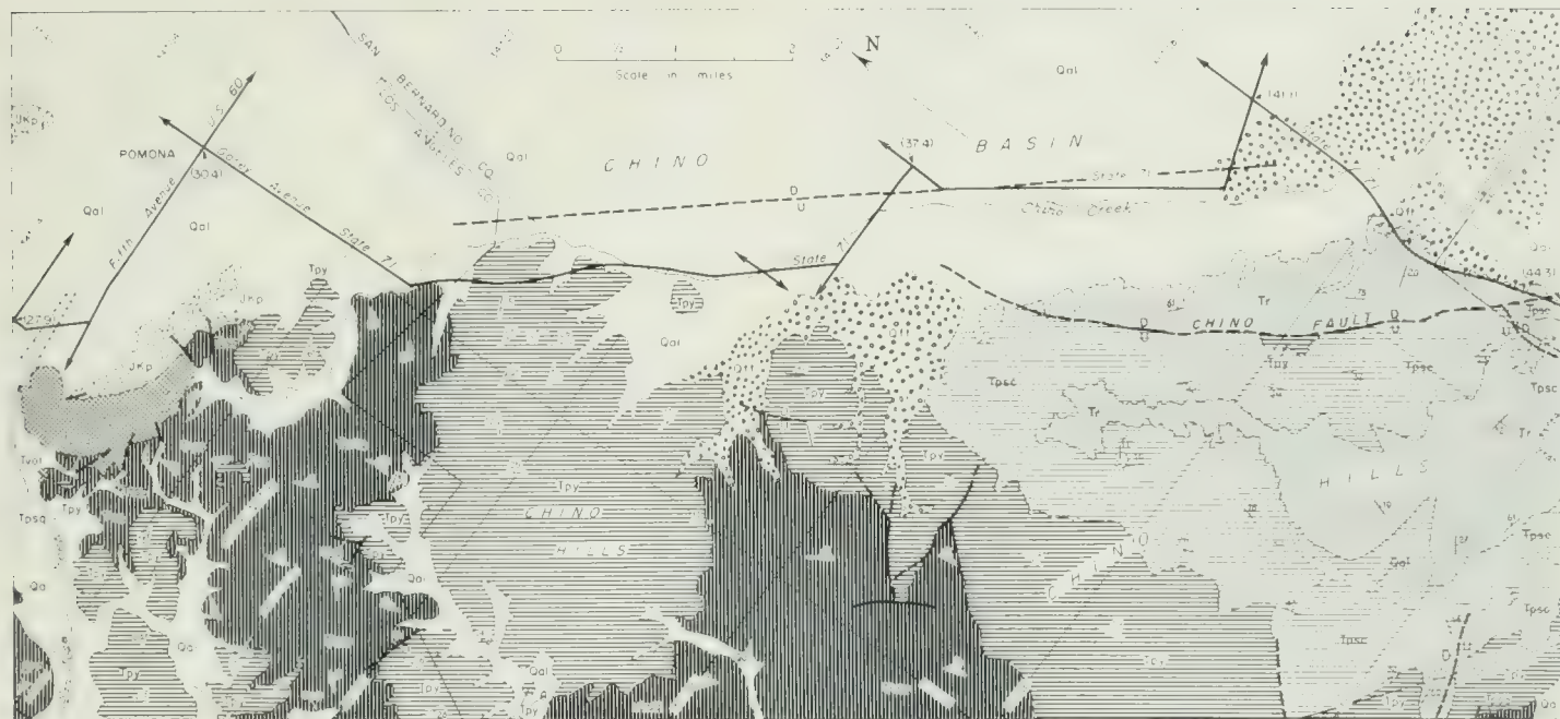
MAP 3. Pomona to Prado Dam. Qal—alluvium; Qol—older alluvial deposits; Tr—Repetto formation; Tpse—Sycamore Canyon member of Puente formation; Tpy—Yorba member of Puente formation; Tpsq—Soquel member of Puente formation; Tvol—volcanic rocks; JKp—plutonic igneous rocks. See Table 1 for stratigraphic relationships and descriptions of these geologic units. Geology after Woodford, et al. (1954).
