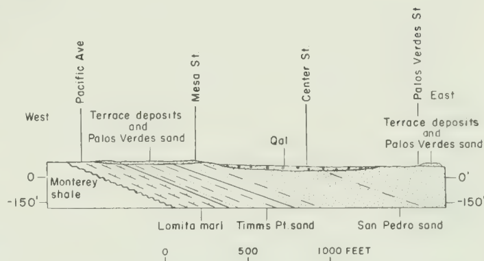
FIGURE 7. Structure section along Second Street, San Pedro.
