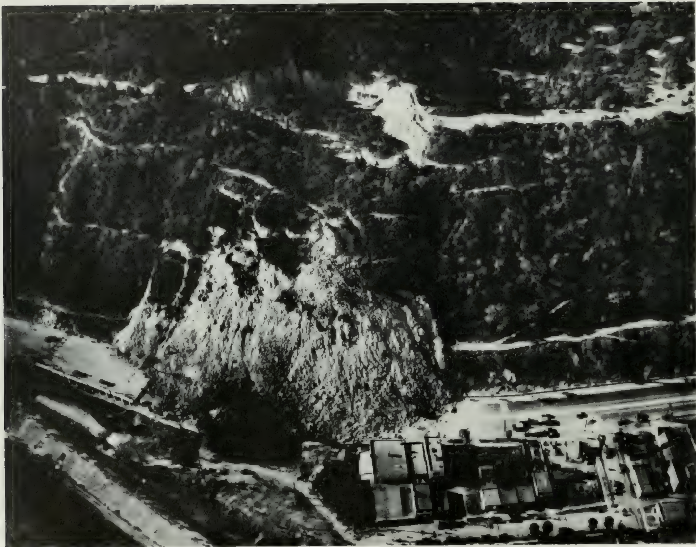
Fig. 4. Elysian Park landslide of November 1937. Riverside Drive in foreground is covered and the viaduct has collapsed beneath the weight of the broken rock. Elysian Park Drive area at the head of the slide subsided to form the steep cliffs. (Map 1.) Photo courtesy of Los Angeles Times.
