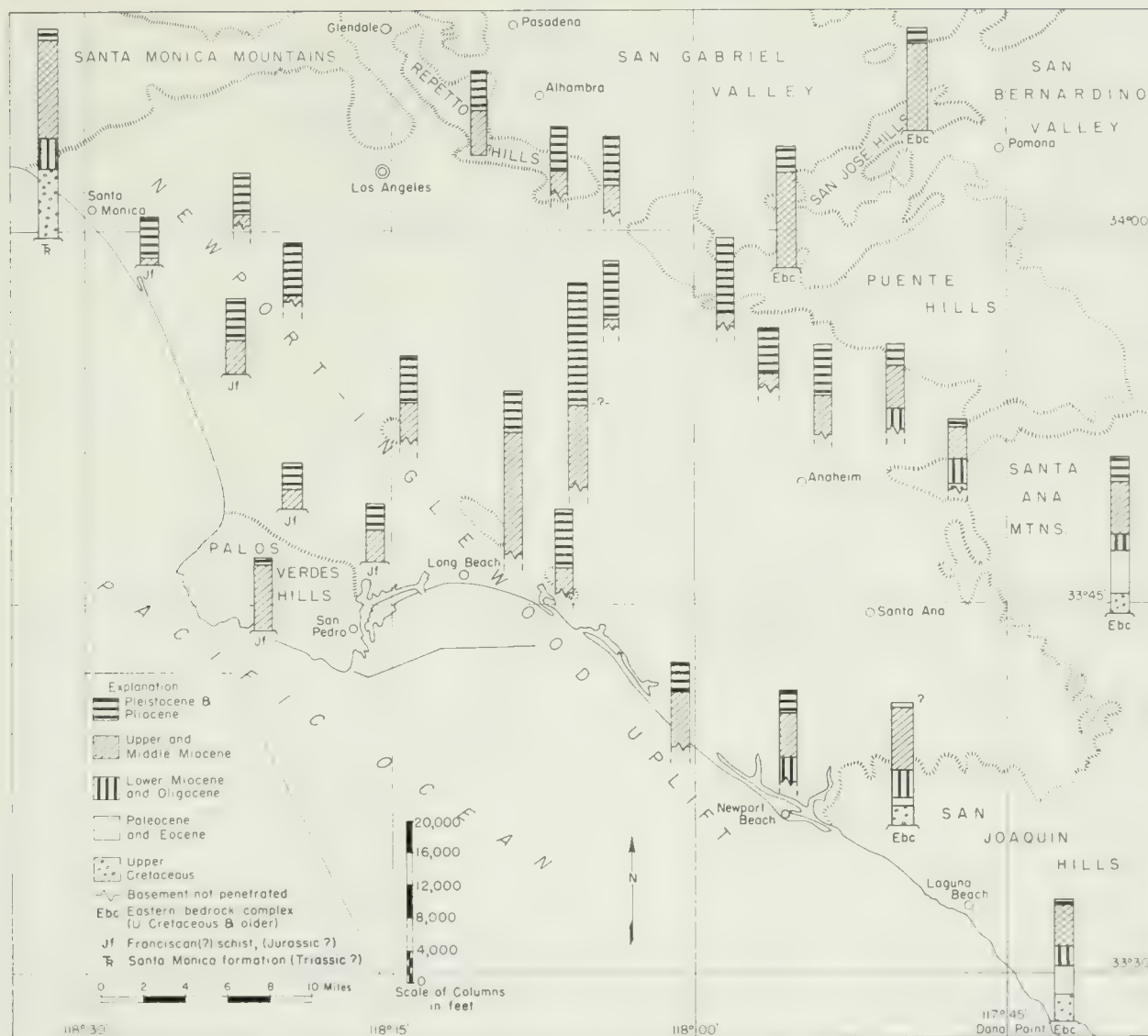
FIGURE 3. Generalized columnar sections in the Los Angeles basin, California.
