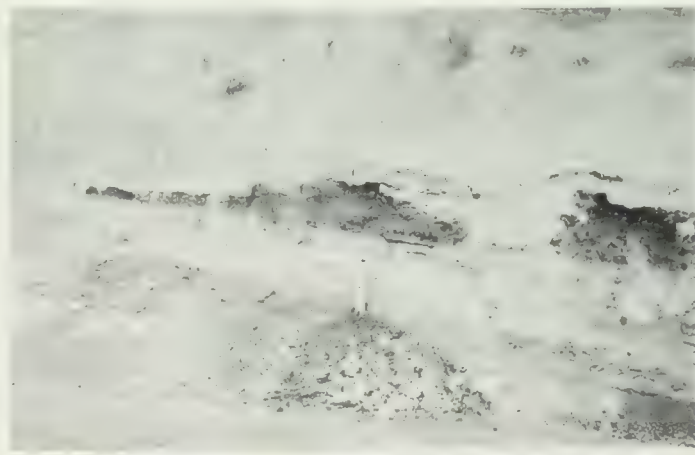
FIGURE 6. Fresh exposure of lignite and clay in upper pit at the Alberhill clay mine. The only bed above the man is overlain by light-colored, blocky clay, and is underlain successively by gray high-alumina clay with conchoidal fracture and by pinkish, dark-appearing clay that is in part of residual origin. All of the exposed material is in the lower part of the Paleocene Silverado formation.
