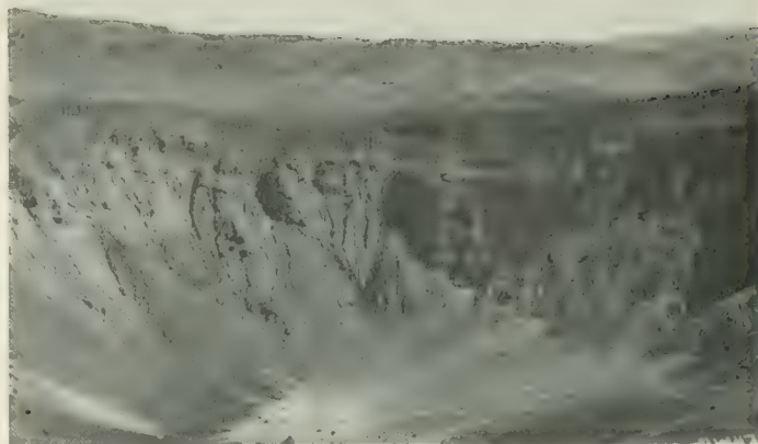
FIGURE 2. Interior of the main Ubehebe crater, in northern Death Valley. View east. The talus slope formed during the glacial epoch is now being destroyed by floods which are building fans below. A distinct unconformity is visible between the cindery material and the thin-bedded Tertiary sediments lower on the crater wall.
