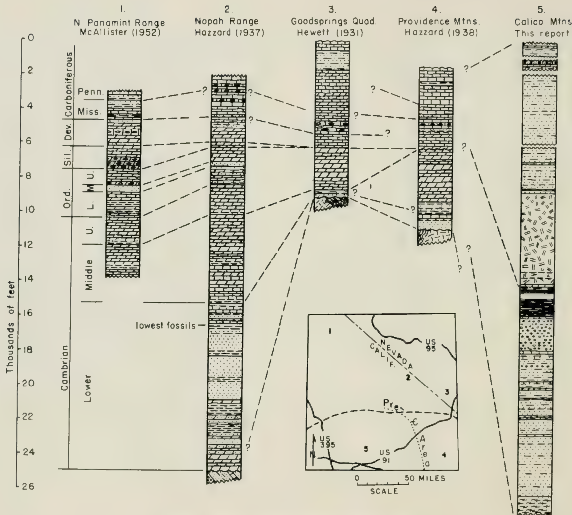
FIGURE 2. Tentative Paleozoic correlations, Mojave Desert.
