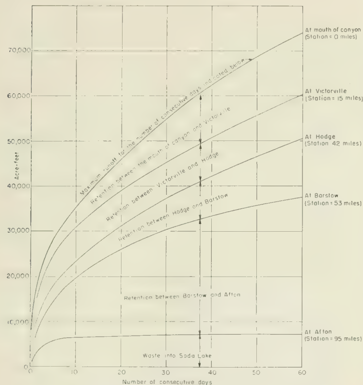
FIGURE 5. Runoff and retention in the Mojave River basin for the 60 consecutive days of greatest runoff in 1932.
