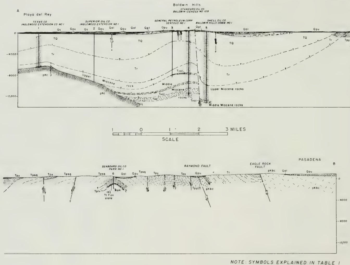
STRUCTURE SECTION A-B, PLAYA DEL REY TO PASADENA
