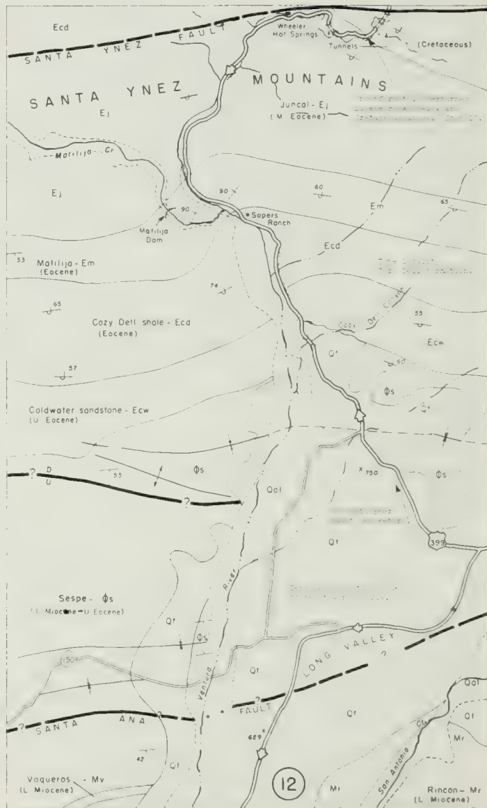
Fig. 18. Rocks exposed in Ojai-Wheeler Hot Springs area.
