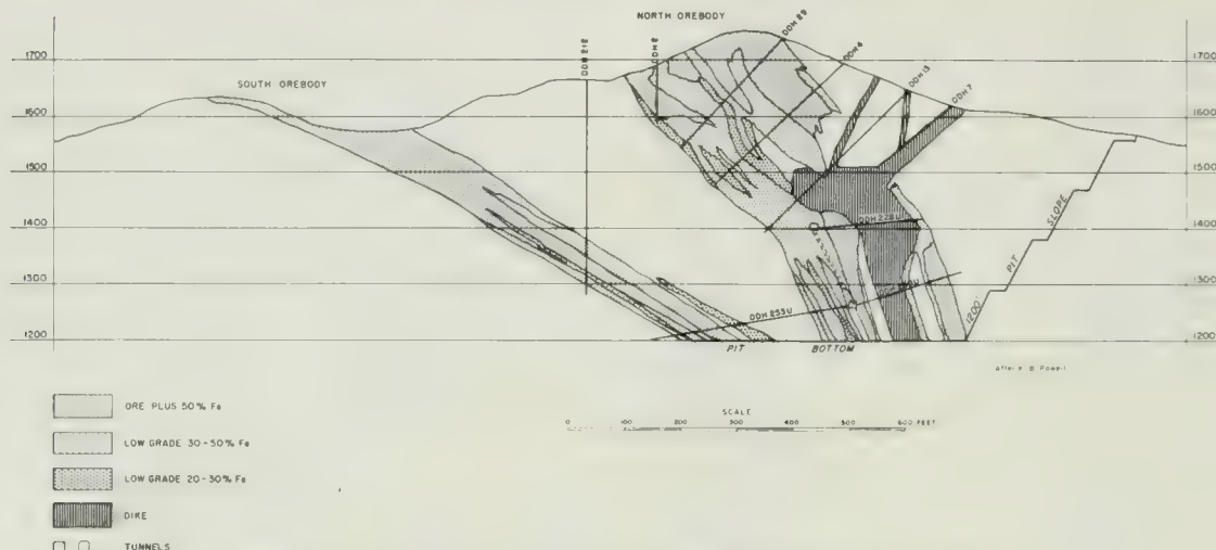
FIGURE 5. Section through the North-South ore bodies, Eagle Mountain iron deposit.
