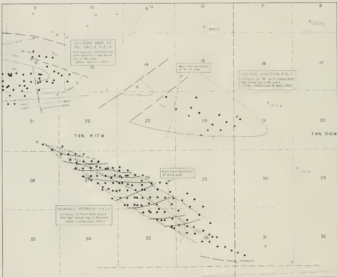
FIGURE 2. Del Valle, Castaic Junction, and Newhall-Potrero fields. Contours in fields, as well as points in selected wildcat wells, are on roughly equivalent horizons. Note accumulation against eastward pinchout in the Newhall-Potrero field, and against westward pinchout in the Castaic Junction field. Much of the Del Valle field is controlled also by westward pinchout. Faults marked "F" control, or at least greatly modify, accumulation in one or more pools. The low point of the basin in this vicinity probably lies near the east quarter corner of sec. 18, T. 4 N., R. 16 W. Data compiled from sources noted, with modifications and additions by writer.
