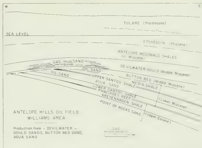
FIGURE 13. Structure section drawn east across Antelope Hills oil field, showing Button Bed unconformity at base of middle Miocene section.
