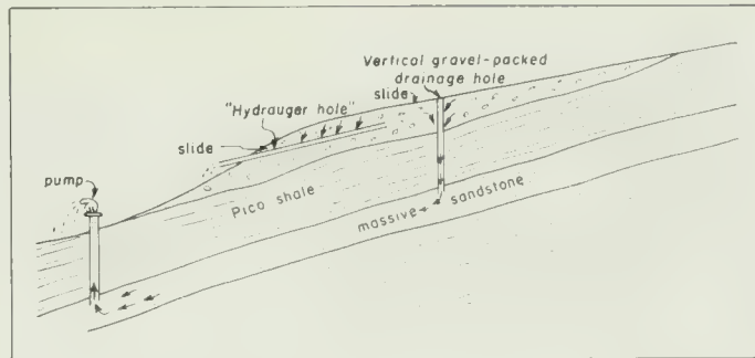
Fig. 20. Diagrammatic sketch showing method by which water in landslide is drained utilizing massive sandstone unit underlying slide.
