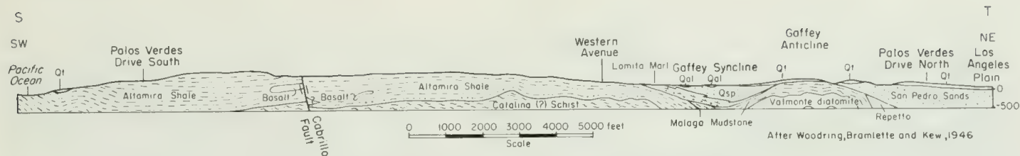
FIGURE 24. Geologic section S-T across the eastern end of the Palos Verdes Hills.
