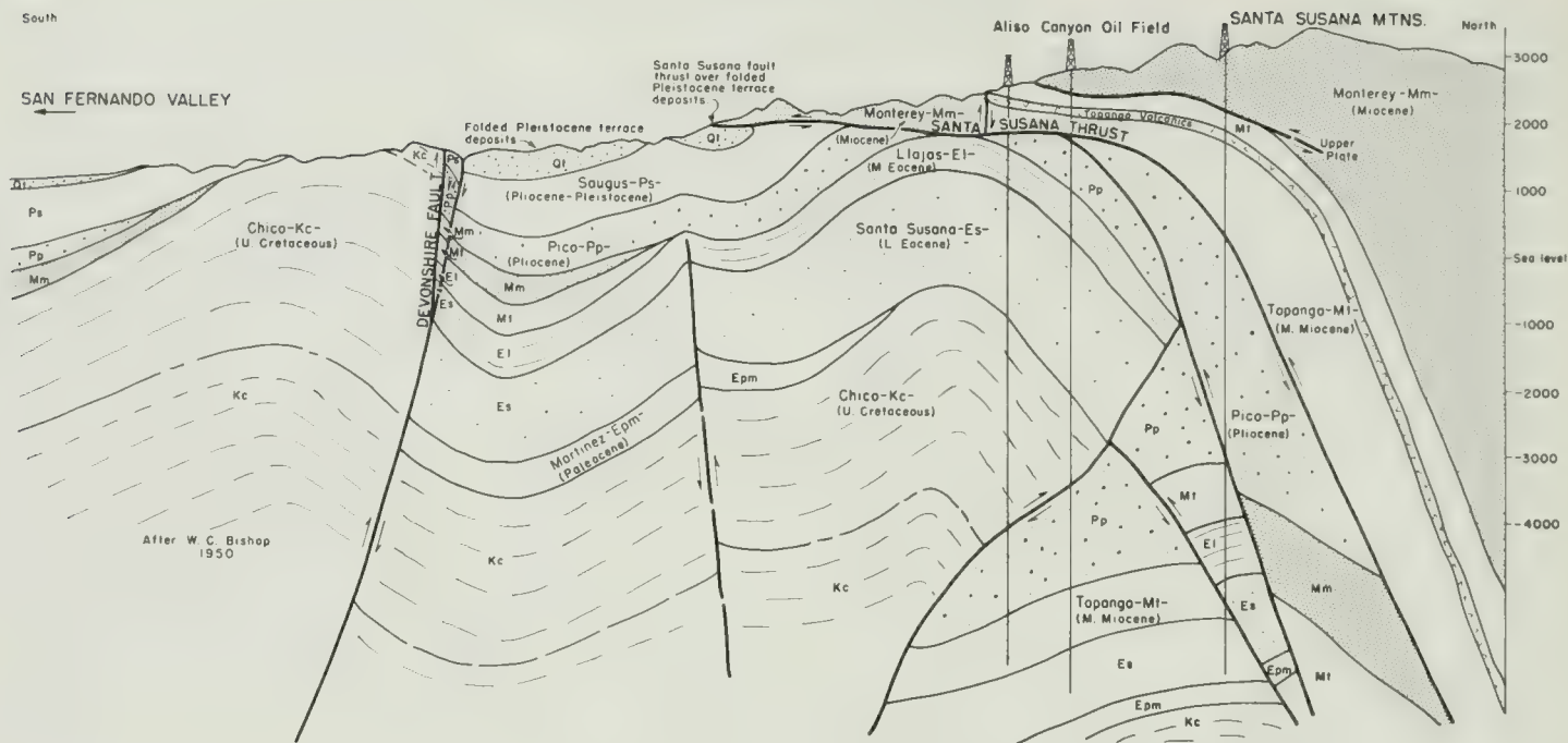
Fig. 28. Cross section through Aliso Canyon oil field.
