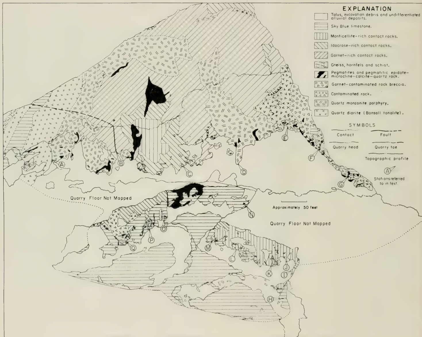
FIGURE 2. Generalized geologic map of faces of the Commercial quarry, Crestmore.
