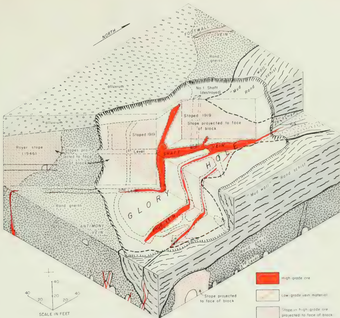
FIGURE 1. Isometric diagram of the Kelly glory hole, Kelly silver mine, San Bernardino County, California. These workings yielded 55,338 tons of ore valued at $3,580,000.
