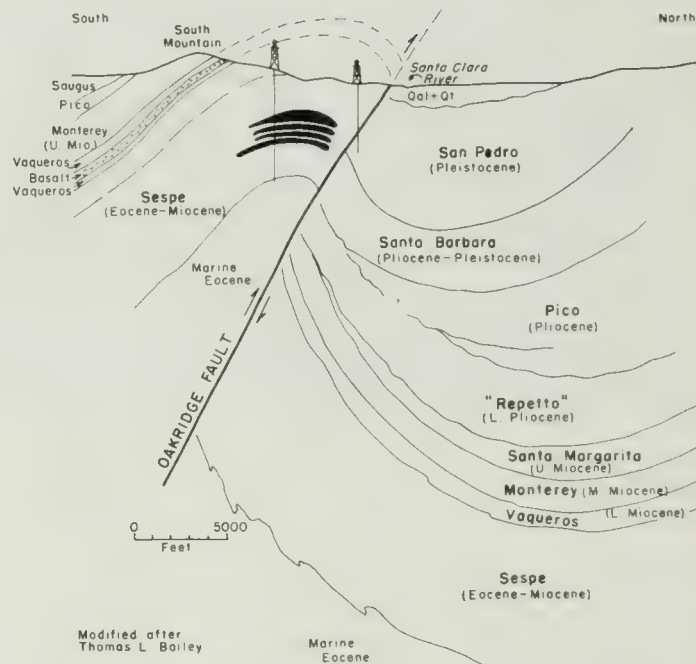
Fig. 26. Cross section through South Mountain oil field.
