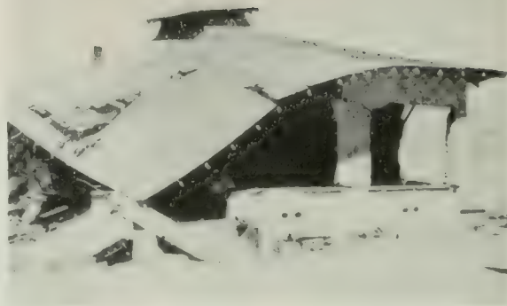
FIGURE 6. Cummings Valley School, west of Tehachapi, 1952. Constructed prior to 1933 of concrete that was nominally but not effectively reinforced. Photo by State Division of Architecture.
