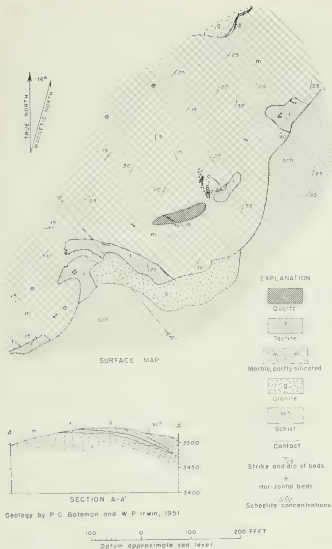
FIGURE 4. Just Associates deposit, Shadow Mountains, San Bernardino County, California.
