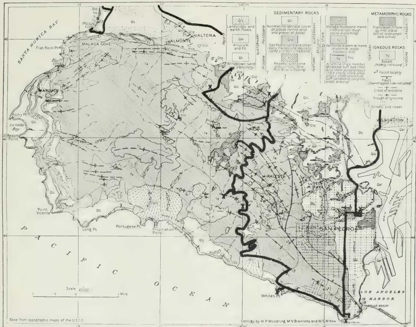
FIGURE 3. Geologic map of the Palos Verdes Hills, showing route of field trip. Map published by permission of the American Association of Petroleum Geologists.
