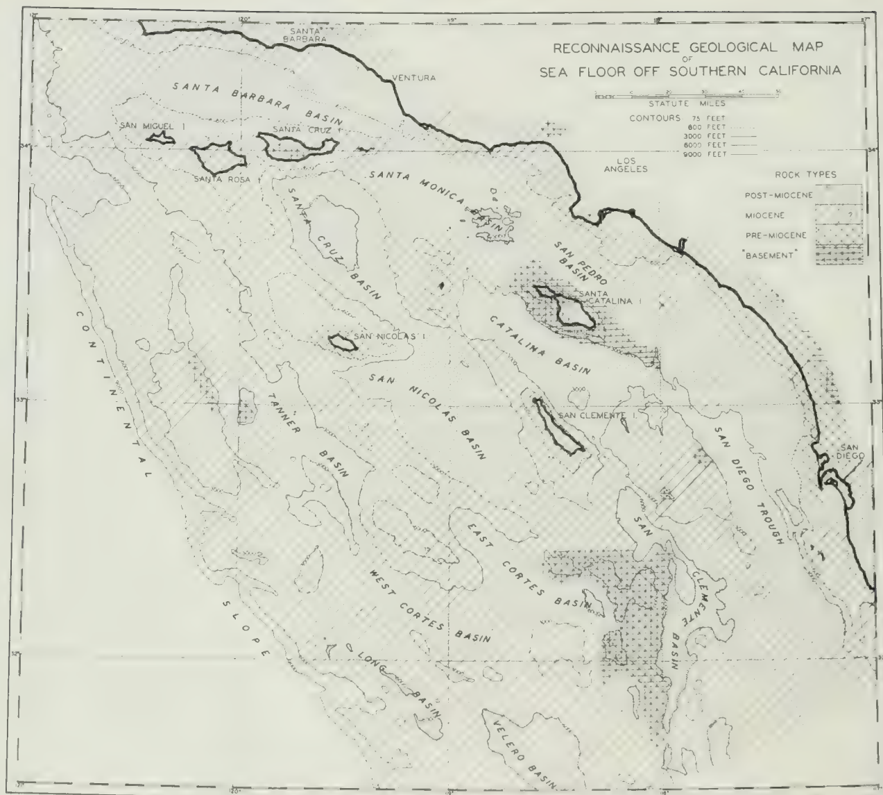
FIGURE 1. Geologic map of sea floor and adjacent land, southern California.
