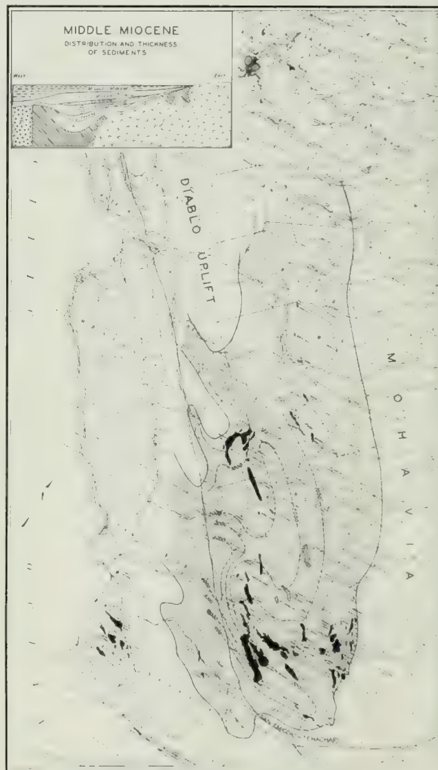
FIGURE 8. Middle Miocene paleogeography.
