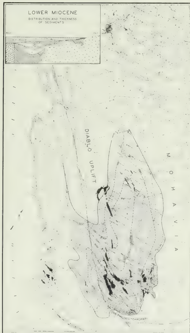
FIGURE 7. Lower Miocene paleogeography.
