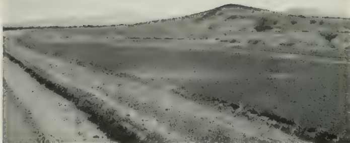
FIGURE 7. Typical desert pavement, blackened by desert lacquer, northeast of Yuma, Arizona.
