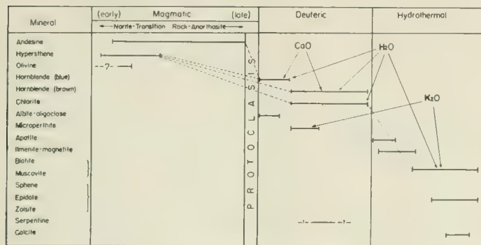
FIGURE 2. Sequence of crystallization of minerals in the norite-anorthosite complex.
