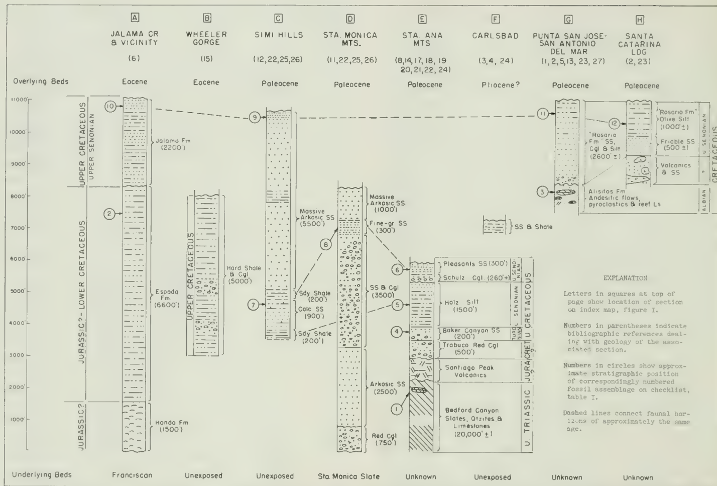
FIGURE 2. Generalized columnar sections of Mesozoic sedimentary rocks in important outcrop areas of southern California and Baja California, Mexico.
