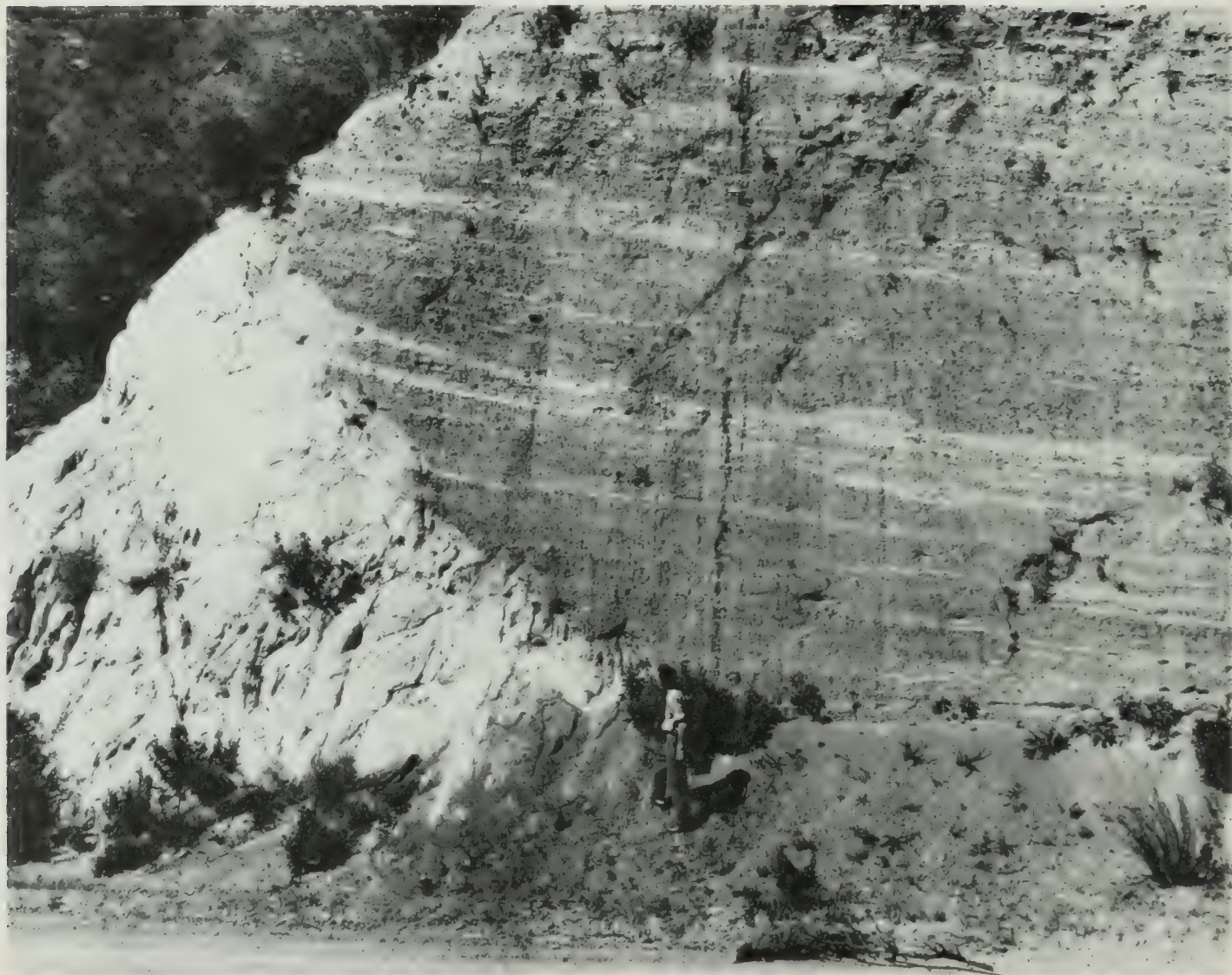
Fig. 7. Quaternary terrace sand and conglomerate deposits against white granodiorite in the San Gabriel Mountains. The overlapping contact exhibits a buttress type of unconformity. (Stop 6, Map 4).
