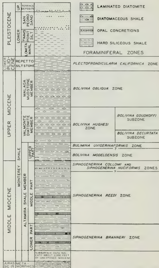
FIGURE 4. Generalized stratigraphic section and related foraminiferal zones of the Palos Verdes Hills. Adapted from Woodring, Bramlette, and Kew, U. S. Geol. Survey Prof. Paper 207.
