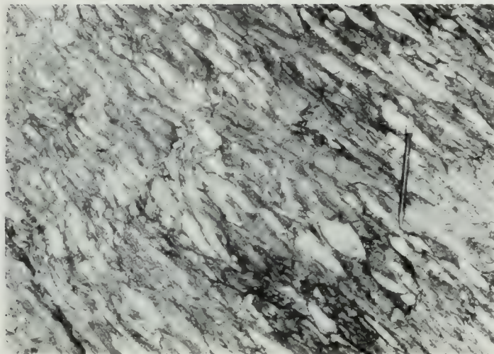
FIGURE 9. Exposure of pre-Cambrian stretched-pebble conglomerate on road between Wildrose Canyon and Harrisburg Flat.
