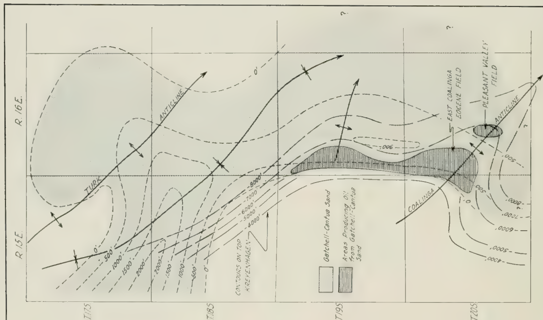
FIGURE 1. Structure-contour map of the Coalina-Cantua Creek area, showing the distribution and thickness of the Gatchell-Cantua sand.
