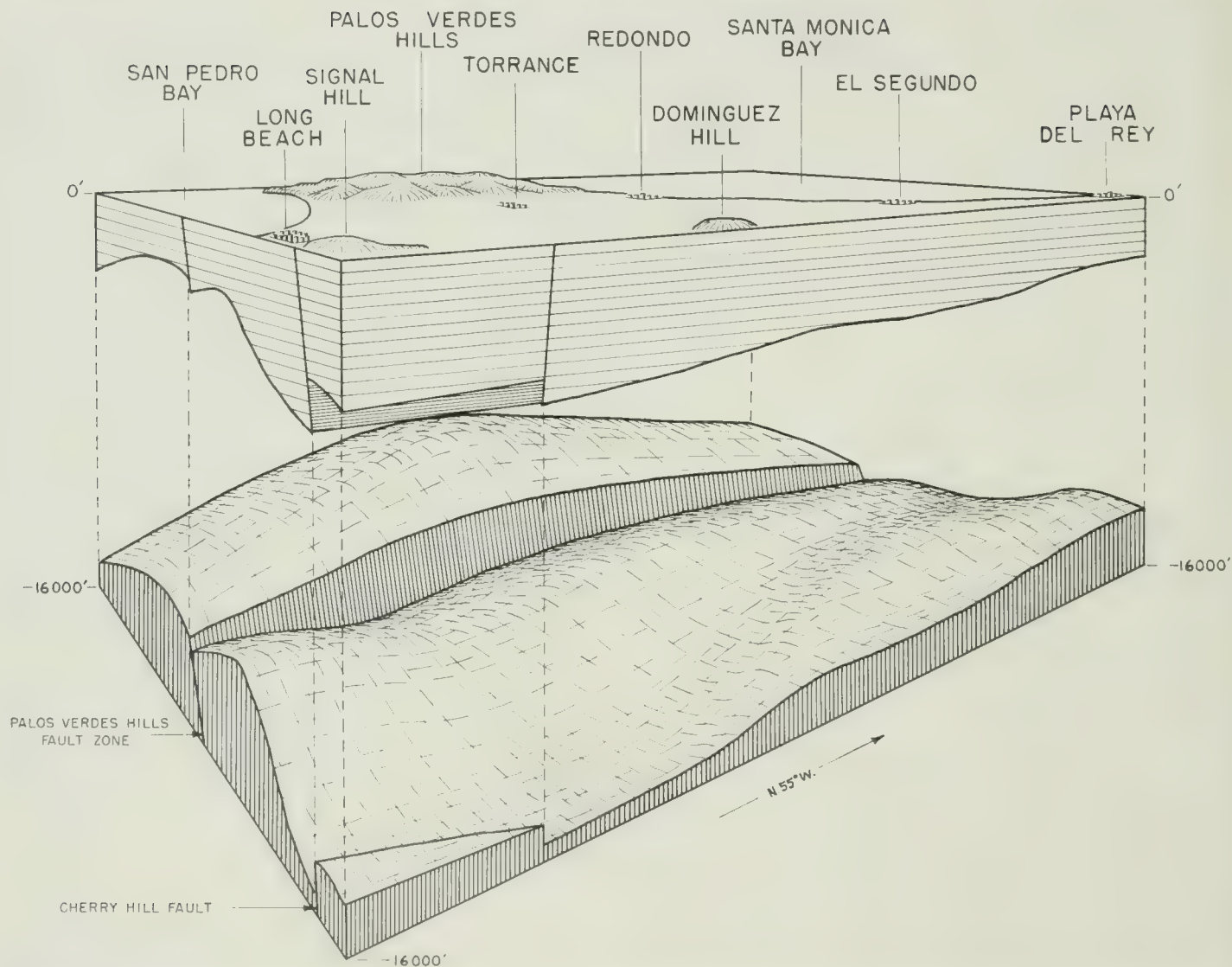
FIGURE 3. Block diagram of west side of Los Angeles basin. The cover of sedimentary rocks is lifted to show the form of the surface on the Catalina schist.
