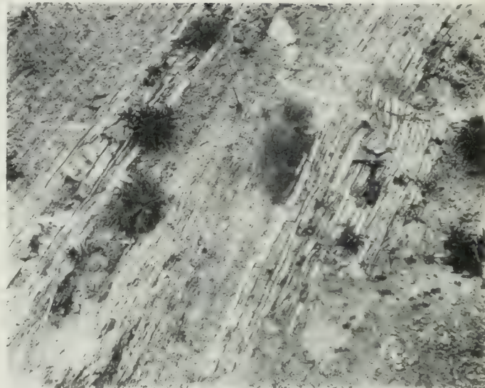
Fig. 29. Rhythmic-bedded siliceous shales of the Modelo (Miocene) formation at Topanga Canyon Road in the Santa Monica Mountains. Note sandstone dikes crossing the bedding planes of the shale. (Stop 26, Map 23).
