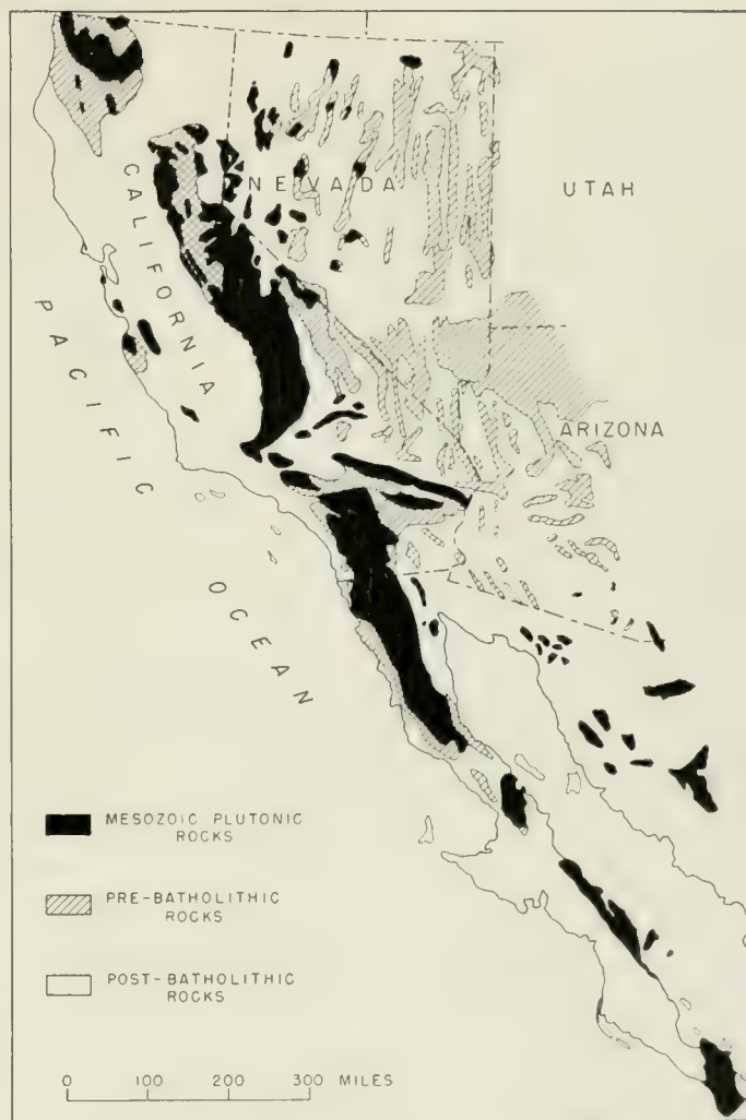
FIGURE 1. Outline map of California and Baja California, showing distribution of plutonic rocks of Mesozoic age
