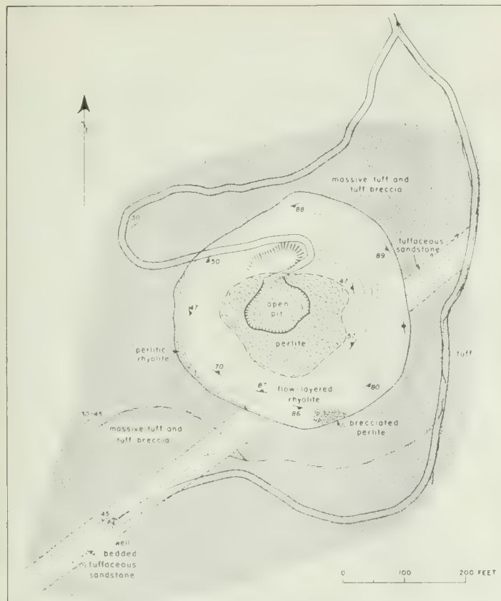
FIGURE 4. Geologic sketch map of the Cedar Top perlite deposit, Castle Mountains, San Bernardino County, California.
