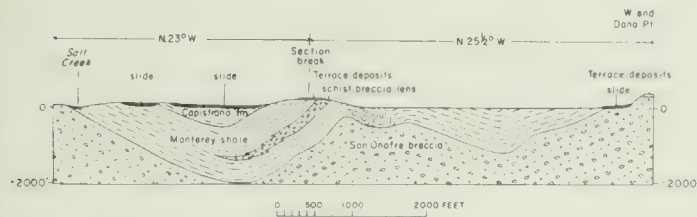
FIGURE 5. Structure section along beach from Salt Creek to Dana Point.
