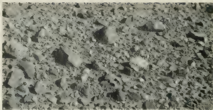
FIGURE 12. A detail of the desert pavement southeast of Stovepipe Wells, in Death Valley, showing numerous wind-carved stones.
