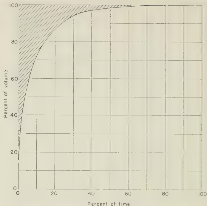
FIGURE 4. Relationship between time and volume of runoff in the Mojave River basin.
