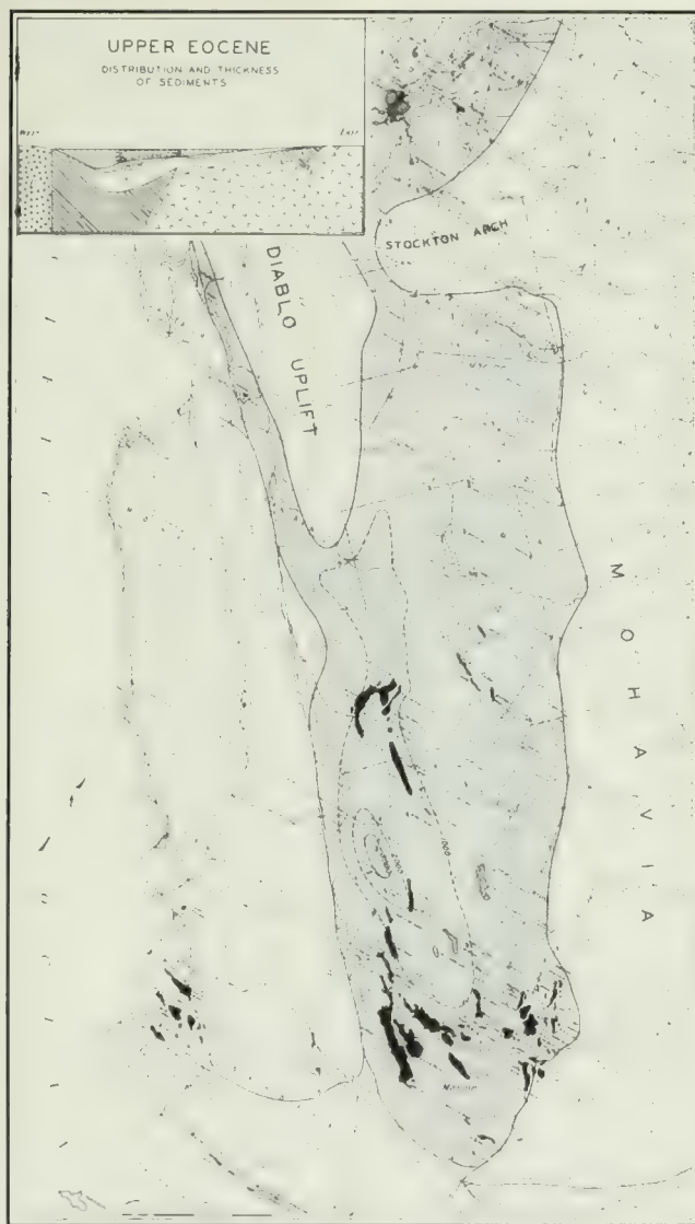
FIGURE 5. Upper Eocene paleogeography.
