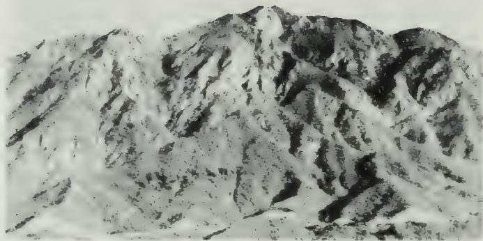
FIGURE 2. View north toward south slope of Josephine Mountain in San Gabriel Mountains. Abundant vegetation above and parallel to road marks trace of San Gabriel fault. Lowe granodiorite above fault; San Gabriel formation below fault. Photo by R. H. Johns.
