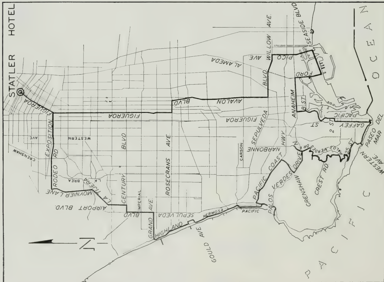
FIGURE 2. Route of field trip through the southwestern part of Los Angeles basin.
