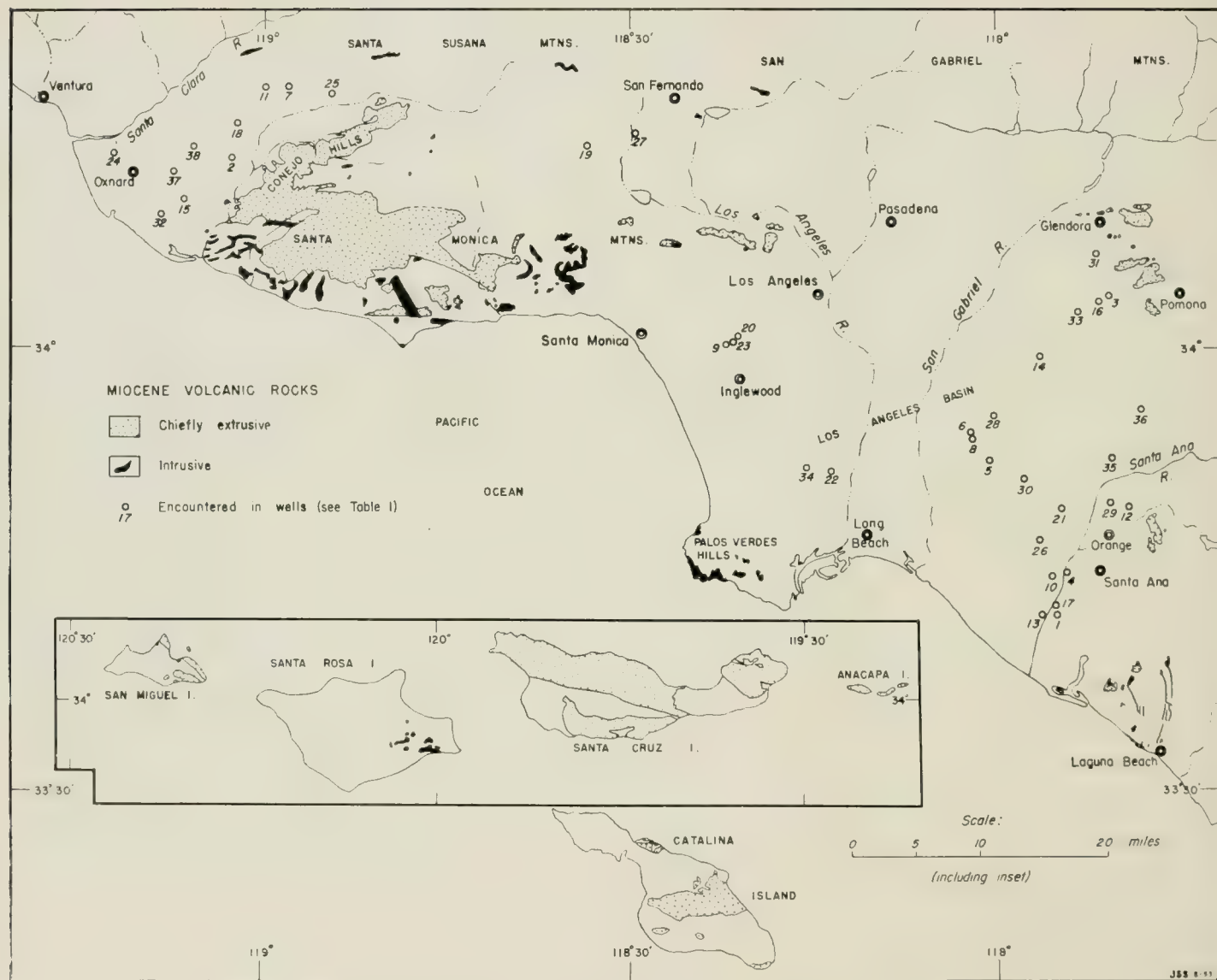
FIGURE 1. Map showing distribution of Miocene volcanic rocks in a part of coastal southern California.
