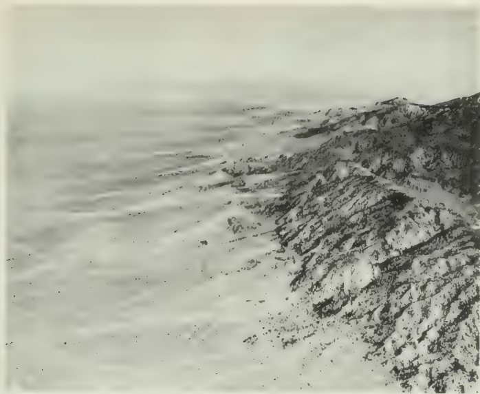
FIGURE 4. Hogbacks (Inface Bluffs) of Quaternary gravel, sand, and silt (Shoemaker gravel) derived from the San Gabriel Mountains; view east toward San Bernardino Mountains. Beds of the Pleistocene Harold formation underlie the low area between the hogbacks and the north slopes of the Table Mountain ridge at right. Mescal Wash in middle distance. Photo by J. S. Shelton and R. C. Frampton.
