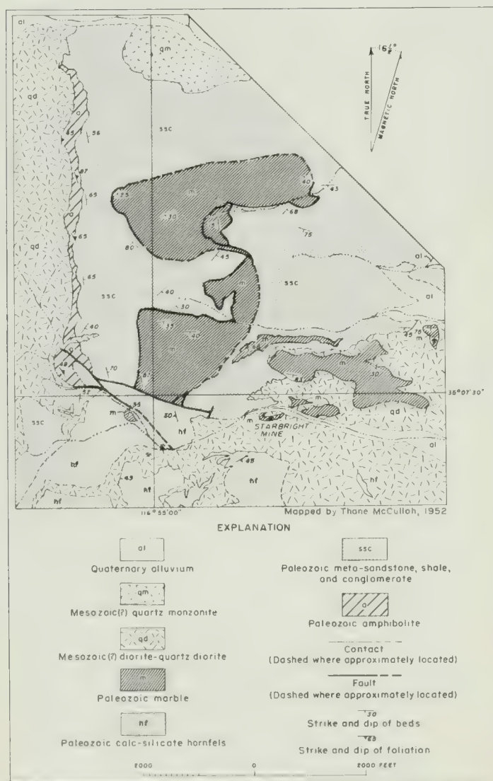
FIGURE 3. Starbright mine area, San Bernardino County, California.
