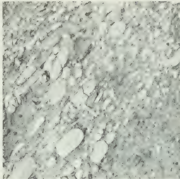
FIGURE 20. Detail of breccia of San Onofre type on wave-cut bench along shore southeast of Salt Creek. Angular fragments are composed of glaucophane schist and related schists.
