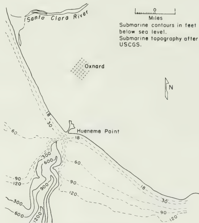
Fig. 22. Hueneme submarine canyon.
