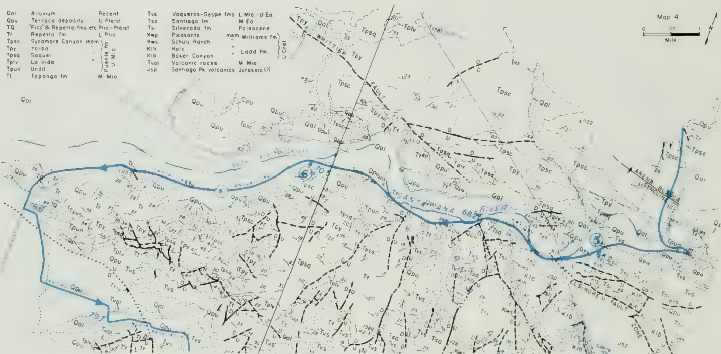
MAP 4. Santa Ana Canyon and western Santa Ana Mountains.
