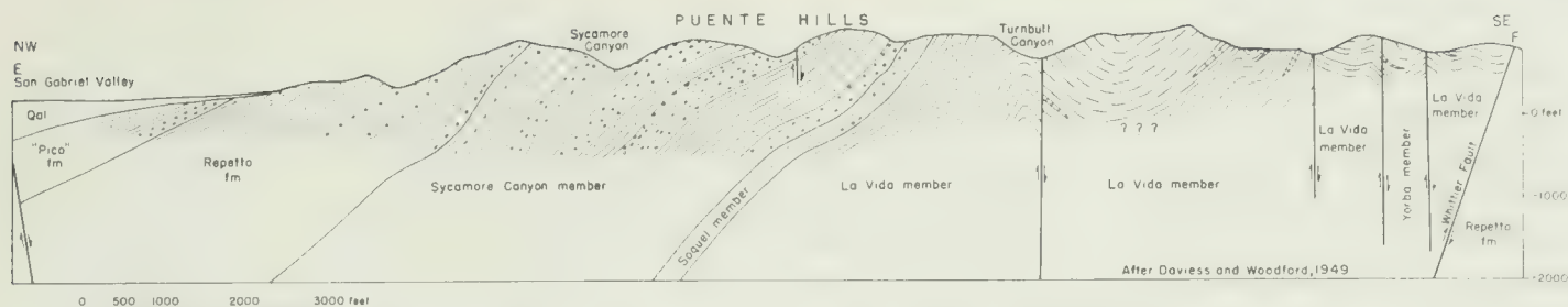
FIGURE 8. Structure section E-F through the Puente Hills north of Whittier, California, showing structure north of the Whittier fault.
