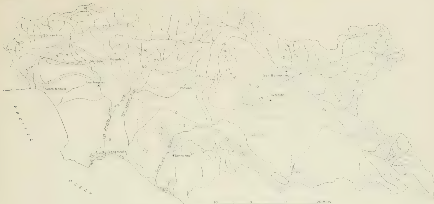
FIGURE 7. Areal distribution of average annual runoff.
