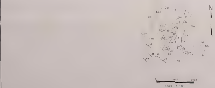
Map showing relations of Mini Canyon, Cosco, Towles, and Saguas formations on hill about one mile south-southwest of Solemnity.
