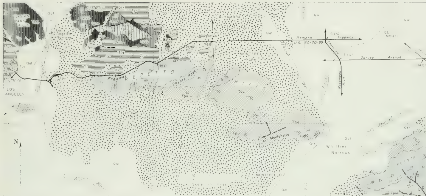
MAP 1. Los Angeles to El Monte. Qal—alluvium; Qft—older alluvial deposits; Tpu—upper Pliocene deposits; Tr—Repetto formation; Tpsc—Sycamore Canyon member of Puente formation; Tpy—Yorba member of Puente formation; Tpsq—Soquel member of Puente formation; Tplv—La Vida member of Puente formation. See Table 1 for stratigraphic relationships and descriptions of these geologic units. Geology after Woodford, et al. (1954).
