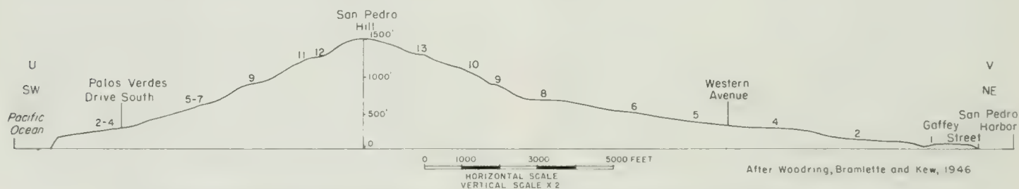
FIGURE 26. Marine terraced profile (section U-V) from Portuguese Bend to northern edge of San Pedro, Palos Verdes Hills.
