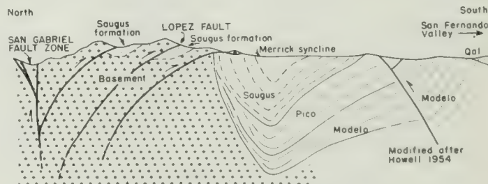
Fig. 5. Cross section through south flank of San Gabriel Mountains to San Fernando Valley.
