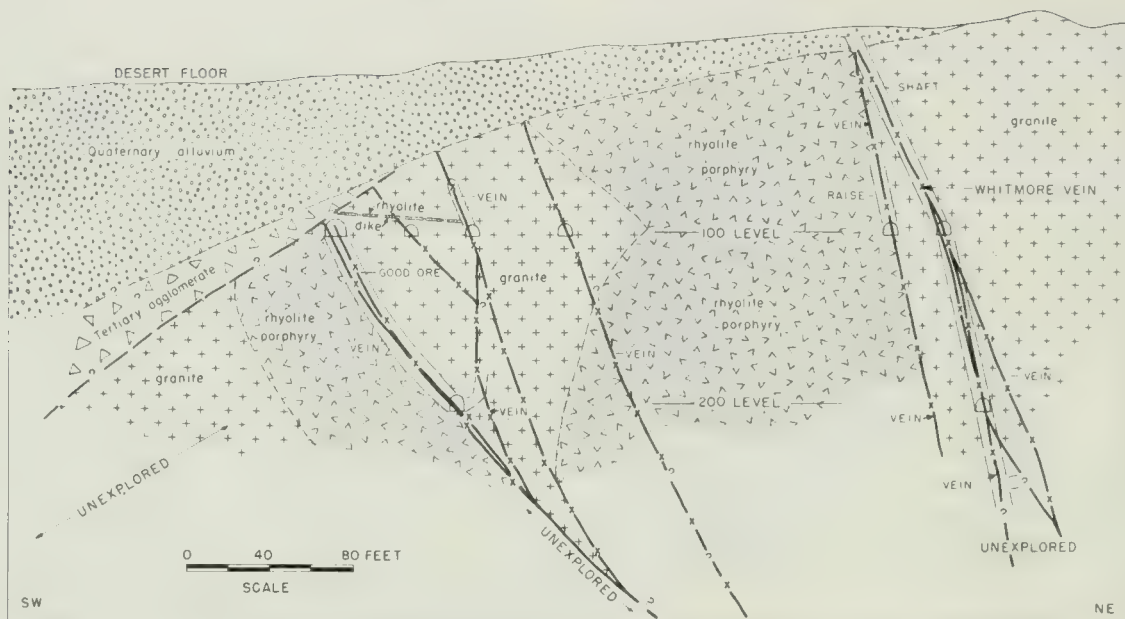
FIGURE 3. Cross sections of the Whitmore mine, Mojave district, Kern County, California.
