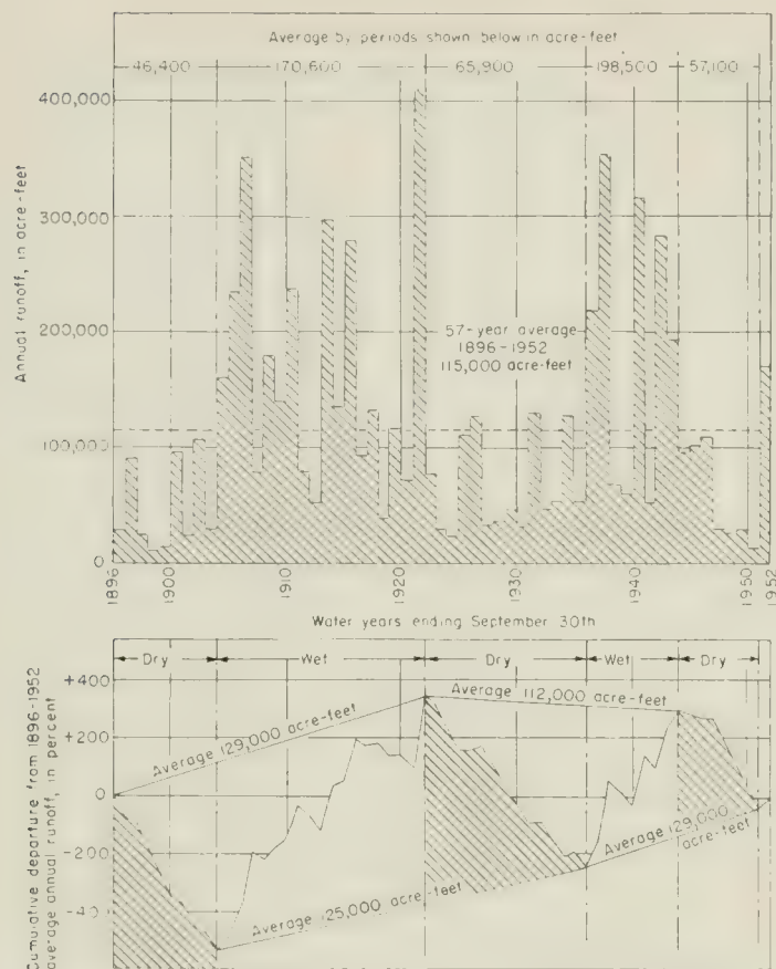
FIGURE 6. Annual runoff of San Gabriel River near Azusa, California, for the period 1896 to 1952.
