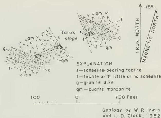
FIGURE 7. Sketch of Birthday Star tungsten prospect, Old Woman Mountains, San Bernardino County, California.
