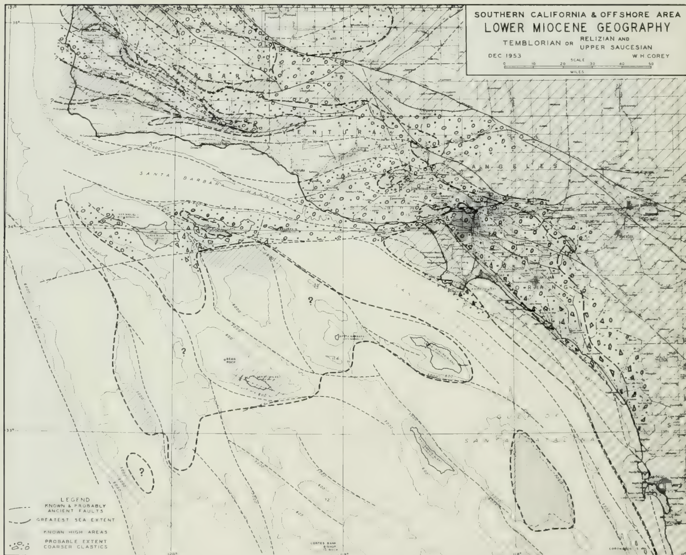
FIGURE 5. Map of a part of southern California, showing general geography and pattern of sedimentation in later early Miocene time.
