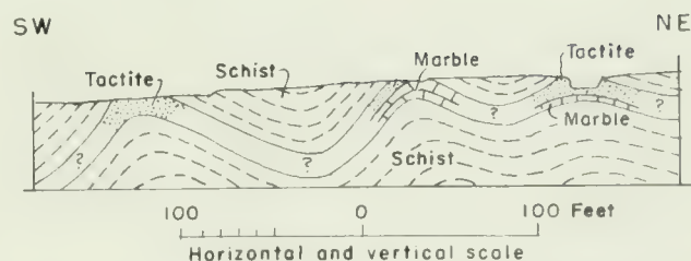
FIGURE 5. Section through Reacon prospect, Shadow Mountains, San Bernardino County, California.
