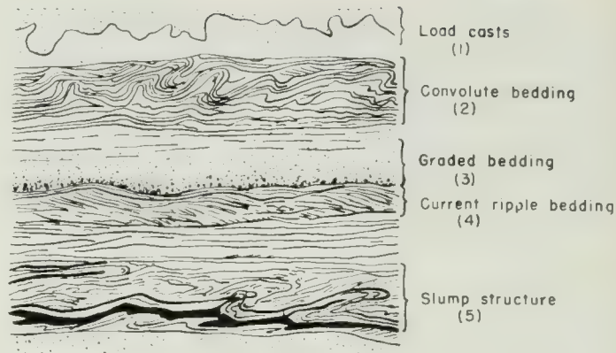
Fig. 13. Diagram showing types of sedimentary structures formed by turbidity currents.
