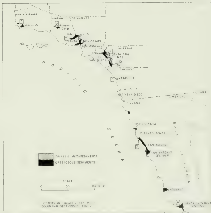
FIGURE 1. Index map of a part of southern California and northern Baja California, Mexico, showing the principal outcrop areas of Mesozoic sedimentary rocks.
