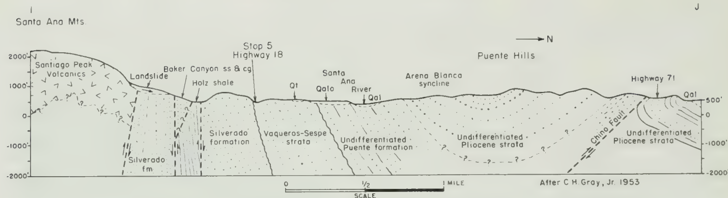
FIGURE 13. Geologic section I-J through the eastern end of the Puente Hills and the northern part of the Santa Ana Mountains.
