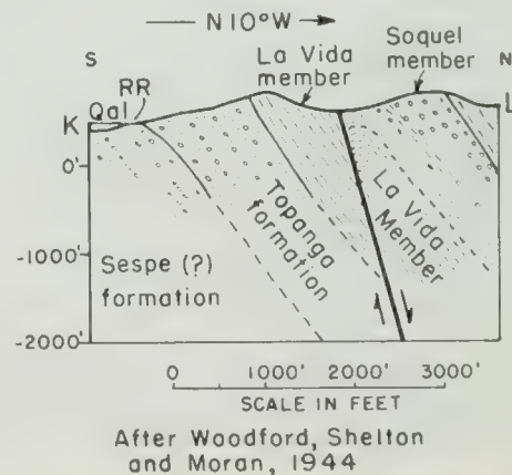
FIGURE 14. Geologic section K-L through Scully Hill west of Stop 5, Santa Ana Canyon.
