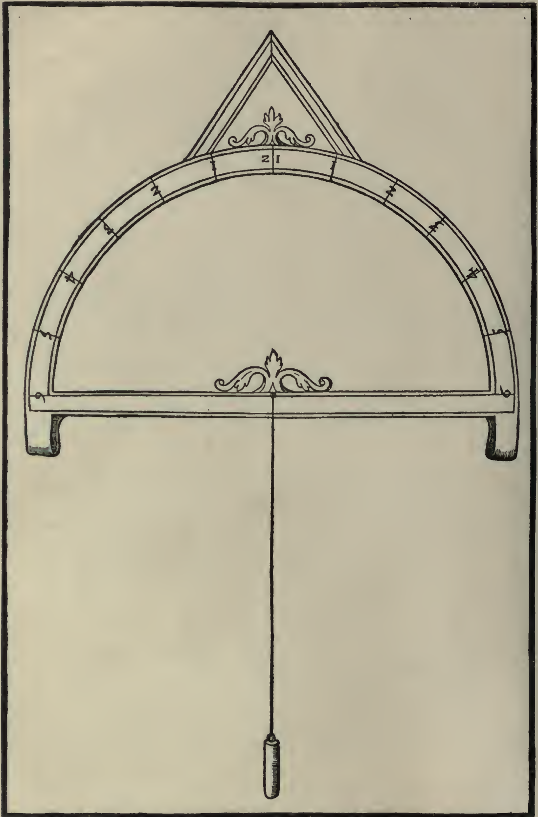
INDICATOR OF A SUSPENDED PLUMMET LEVEL
