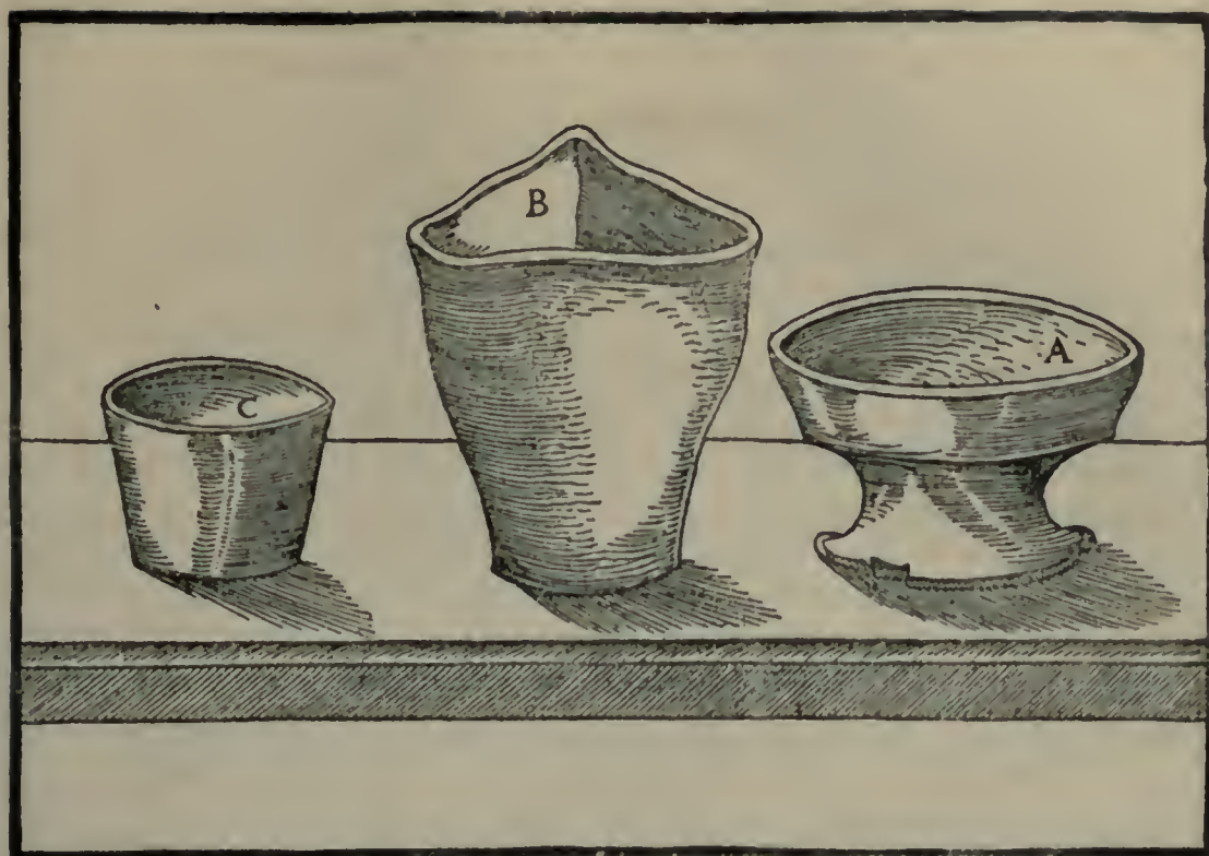
A—SCORIFIER. B—TRIANGULAR CRUCIBLE. C—CUPEL.
