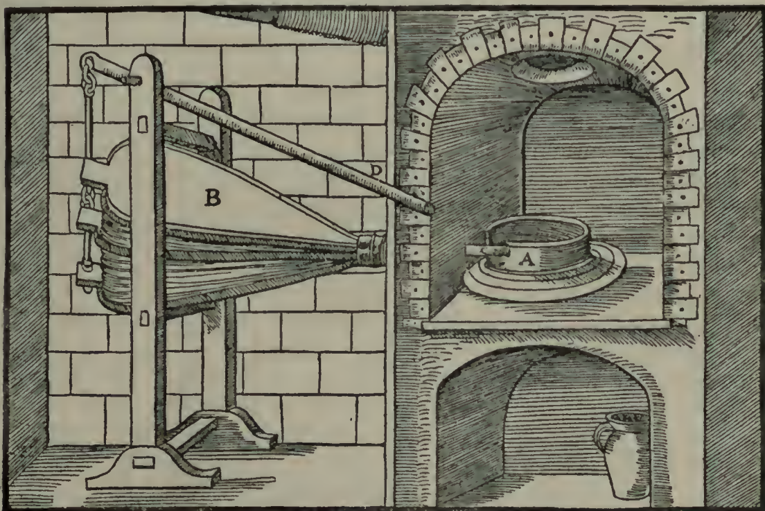
A—IRON HOOP. B—DOUBLE BELLOWS. C—ITS NOZZLE. D—LEVER.
