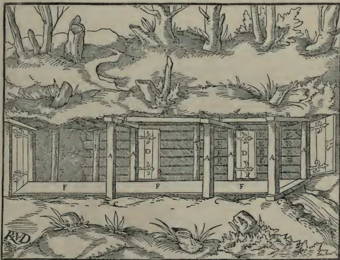
A—POSTS. B—CAPS. C—SILLS. D—DOORS. E—LAGGING. F—DRAINS.
