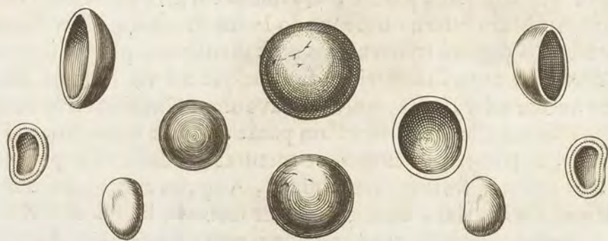
BUFONITES
