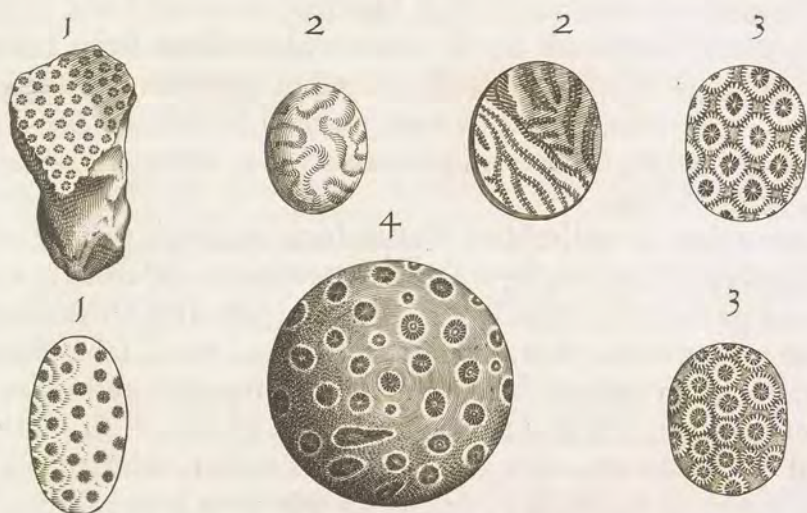
ASTROITES.
