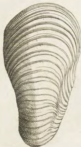
CONCHITES LUNATUS
