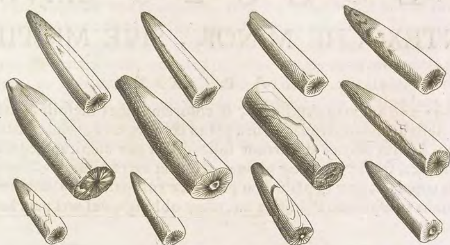
BELEMNITES
