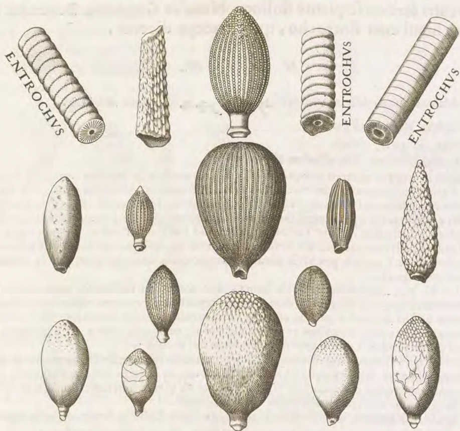
LAPIS IVDAICVS.
