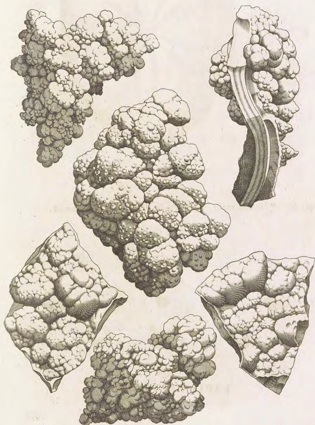
PYRITES BOTRYITES
