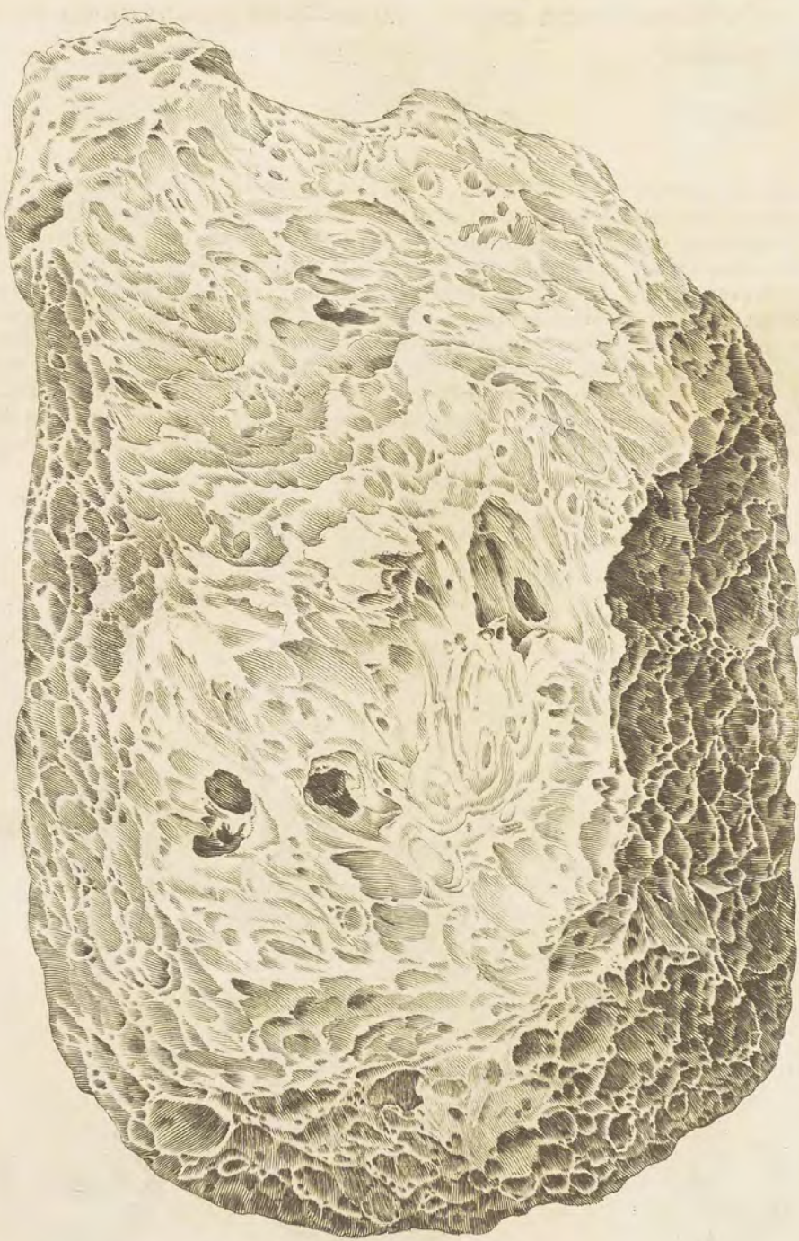
PVMEX SPVMOSVS
