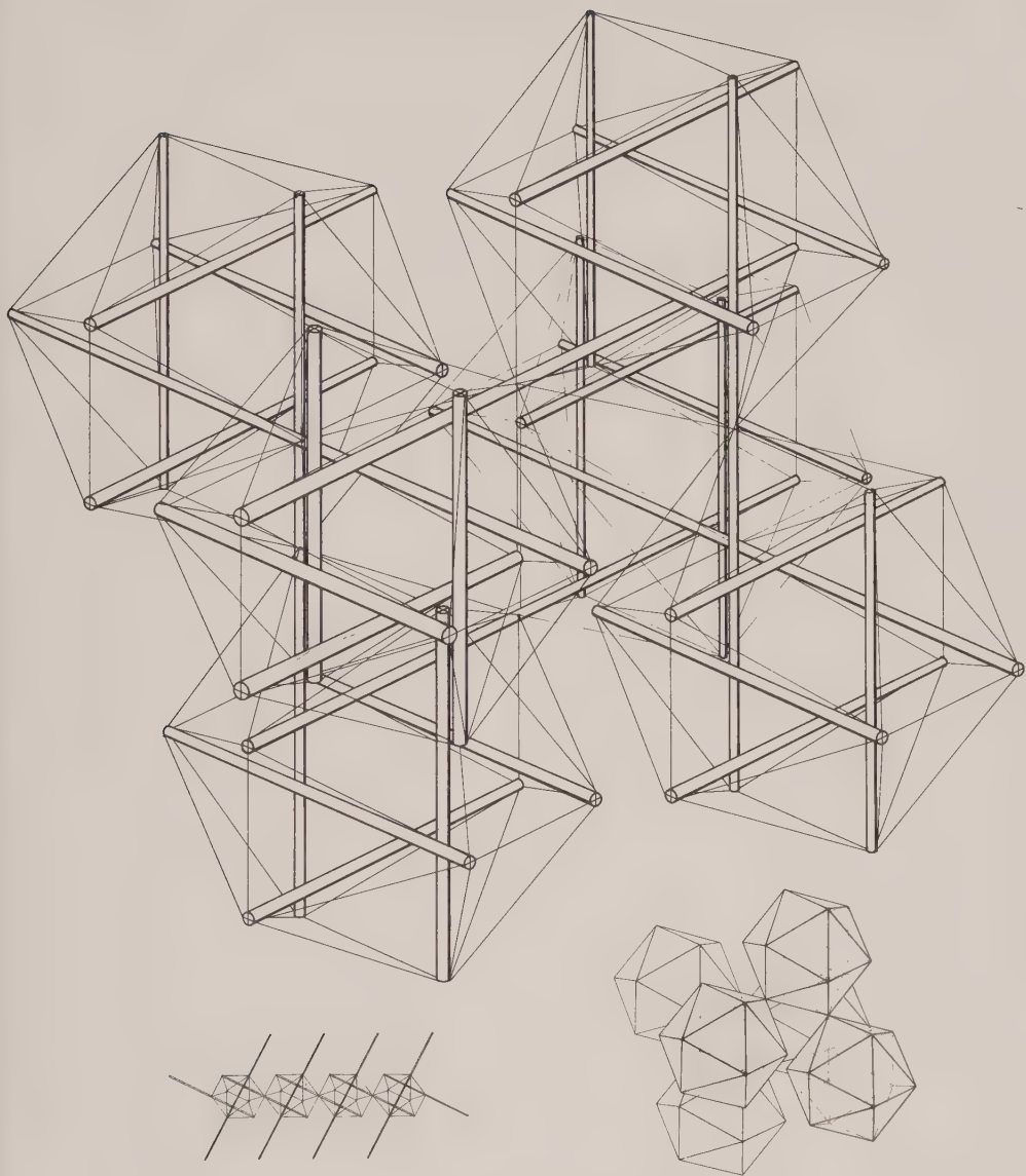
Fig. 784.41 Indefinitely Extensive Array of Tensegrity Icosahedra.
