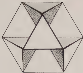
Eight Tetrahedra 8 = 2^3
