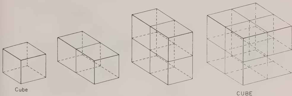
Fig. A11. Filling space with cubes.
