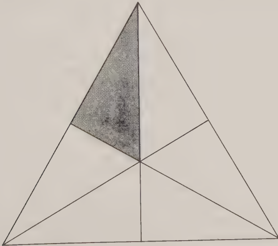
Fig. A21. Subdivision of triangular face into six equal parts.
