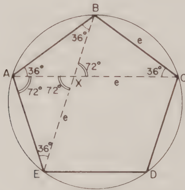
Fig. A5. Regular pentagon and the golden section.
