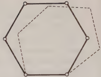
Hexagon
