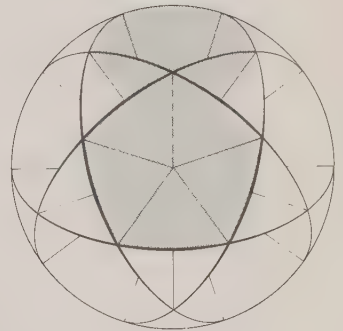
B. The 6-Great-Circle Icosahedron System.
