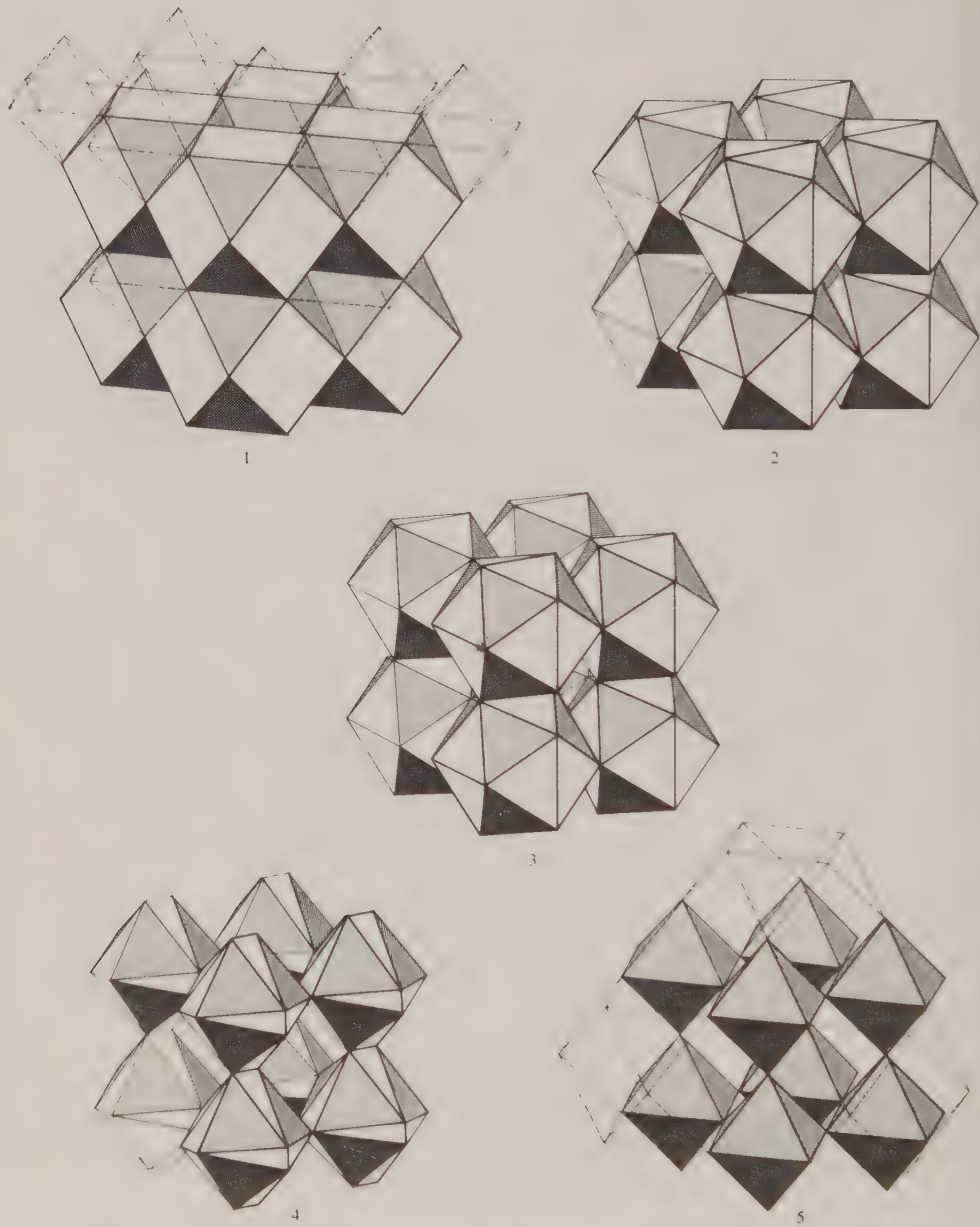
Fig. 470.02C Transformation of Vector Equilibrium and Octahedron as Space-Filling Jitterbug: Because the vector equilibrium and the octahedron will fill space, it is possible to envision a space-filling "jitterbug" transformation. If we combine vector equilibria on their square faces in a space-filling arrangement, the triangular faces form octahedral voids (1). As the vector equilibria contract, just as in the single "jitterbug," they transform through the icosahedron phase (3) and end at the octahedron phase (5).
