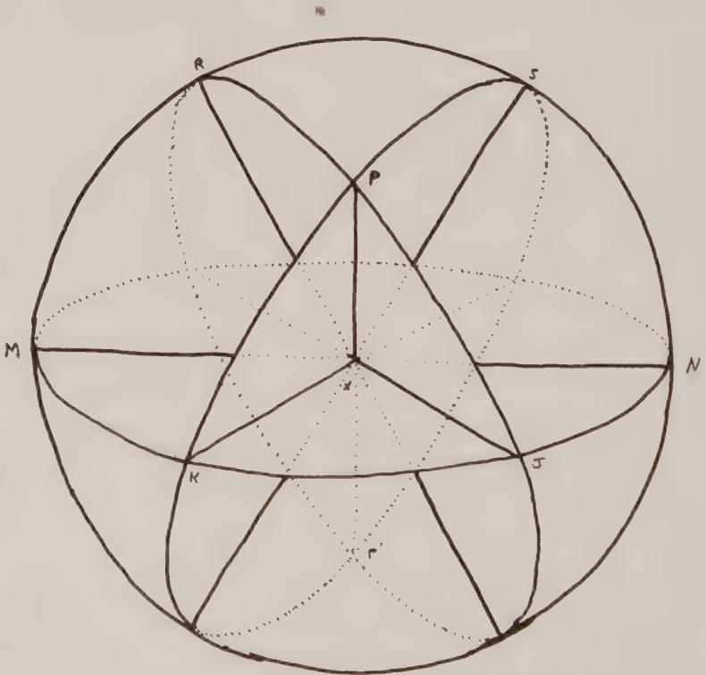
Fig. 841.15A Realization of Four Great Circles of Vector Equilibrium.
