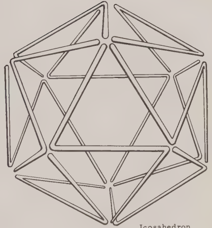
Icosahedron
