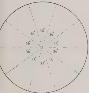
Fig. 458.12 Folding of Great Circles into the Icosahedron System:
