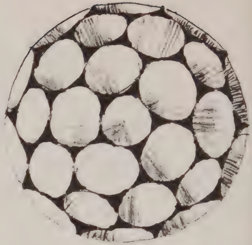
Fig. 541.30H Circular Cornucopia Assembled Around Interior Points to Form a Spherical Array. The tangent circle areas as well as concave triangle interstices constitute the total spherical surface.
