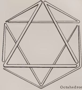
Octahedron
