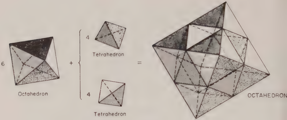
Fig. A13. Scaling the octahedron by a linear factor of two.
