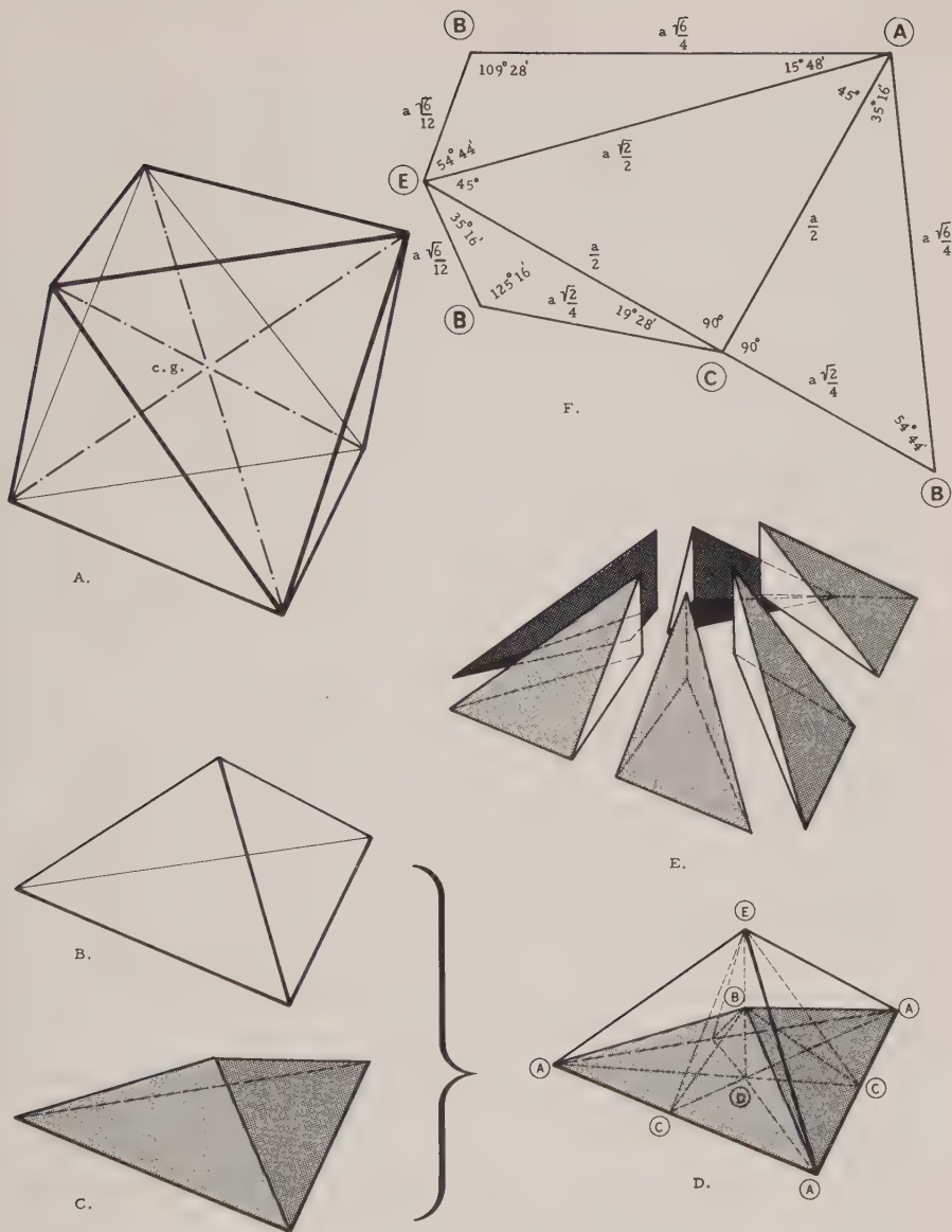
Fig. 916.01 Division of Eighth-Octahedron into Six Parts: B Quanta Module : The regular octahedron (A) is divided into eight identical units (B) equaling \frac{1}{8} of the volume of the octahedron. The quarter tetrahedron as defined by six A Modules (C) is subtracted from the \frac{1}{8} -octahedron (D). This fractional unit is then subdivided into six identical irregular tetrahedra that appear as three right-hand and three left-hand units and are referred to as B Modules. They are equal in volume to the A Modules and are consequently also \frac{1}{24} th of the regular tetrahedron. In (F) is shown the plane net which will fold into either the right or left B Module. Vertex A is at the vertex of the octahedron. Vertex C is at the mid-edge of the octahedron. Vertex E is at the center of gravity of the octahedron.
