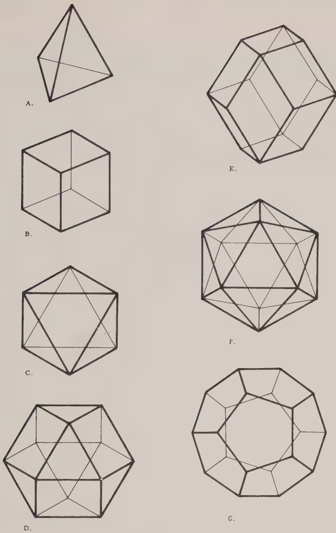
Fig. 400.30 Topological relationships of faces, vertices, and edges of various polyhedra:
