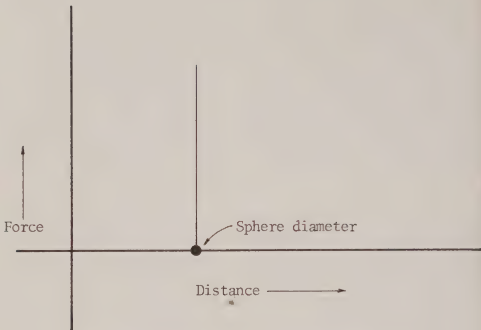
Fig. A35a. Distance-dependence of force between two rigid spheres.
