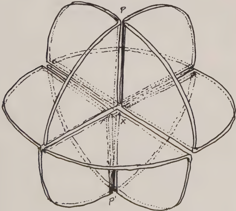
Fig. 835.10 Six Great Circles Folded to Form Octahedron.
