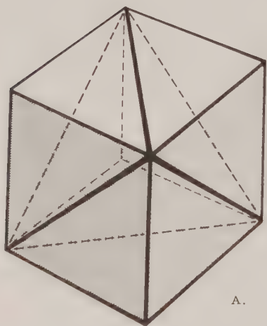
Fig. 415.22 Rational Volumes of Tetrahedroning:
