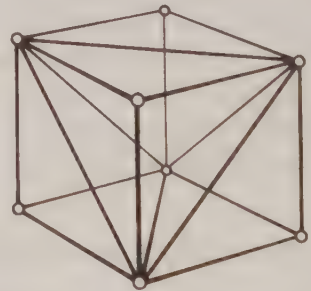
Cube stabilized with tetrahedron
