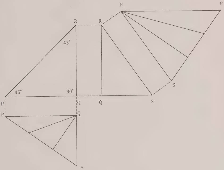
Fig. A25. The AA^*B or A^*AB^* module unfolded.
