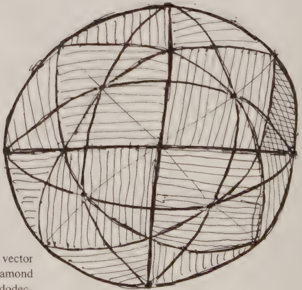
Fig. 454.02 The six great circles of the vector equilibrium disclose the spherical tetrahedra and the spherical cube and their chordal, flat-faceted, polyhedral counterparts.
