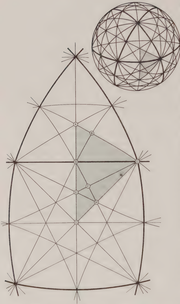
Fig. 453.01 Great Circles of Vector Equilibrium Define Lowest Common Multiple Triangle: 1/48th of a Sphere : The shaded triangle is 1/48th of the entire sphere and is the lowest common denominator (in 24 rights and 24 lefts) of the total spherical surface. The 48 LCD triangles defined by the 25 great circles of the vector equilibrium are grouped together in whole increments to define exactly the spherical surface areas, edges, and vertexes of the spherical tetrahedron, spherical cube, spherical octahedron, and spherical rhombic dodecahedron. The heavy lines are the edges of the four great circles of the vector equilibrium. Included here is the spherical trigonometry data for this lowest-common-denominator triangle of the 25-great-circle hierarchy of the vector equilibrium.
