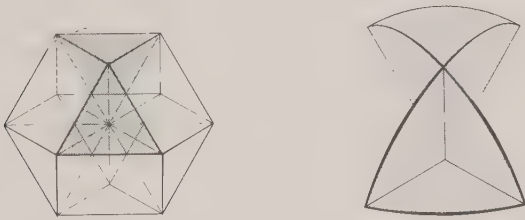
A. The Spherical Cube or Rhombic Dodecahedron.
