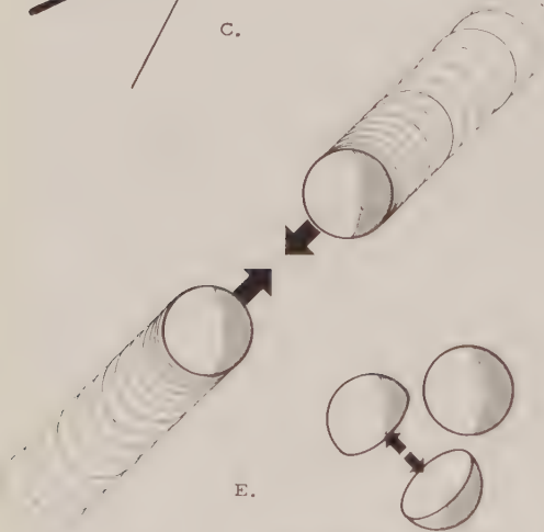
Fig. 517.10 Interference Phenomena: Lines Cannot Go Through the Same Point at the Same Time : Interference phenomena: No two actions can go through the same point at the same time. The consequences of this can be pictured as follows:
