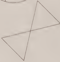
Fig. 831.31 Foldability of Great Circles.
