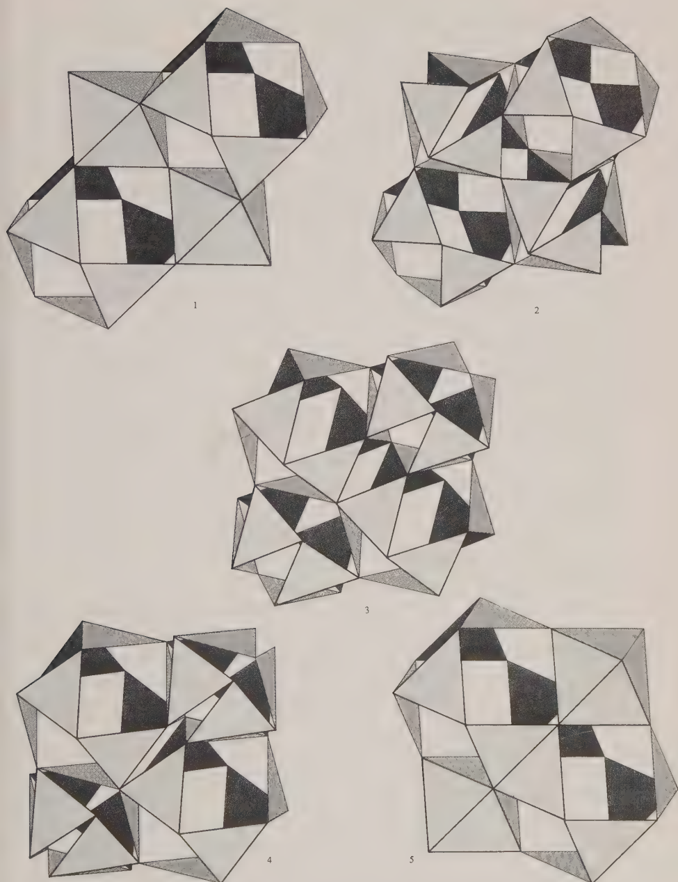
Fig. 470.02D Reciprocity of Vector Equilibrium and Octahedra in Space-Filling Jitterbug : In the space-filling "jitterbug" transformation, the vector equilibria contract to become octahedra, and, because in space filling array there are equal numbers of octahedra and vector equilibria, the original octahedra expand and ultimately become vector equilibria. There is a complete change of the two figures.
