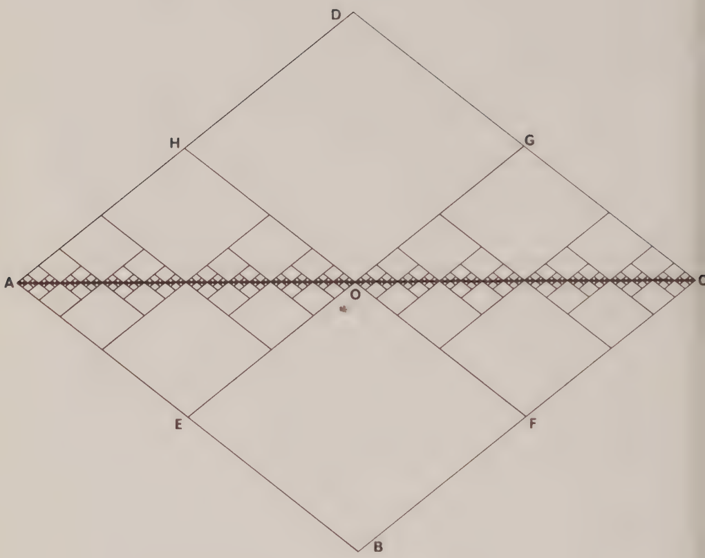
Fig. 522.09 The Deliberately Nonstraight Line : Quasi-''straight'' lines: ABCD A = unit wave; AEOFCGOHA = ABCDA . As we double the frequency and halve the wave-length of positive and negative waves, we approach relative straightness: proof that two deliberately nonstraight lines between points A and C approach relative straightness to more effective degree than attainable by an assumed straight construction.
