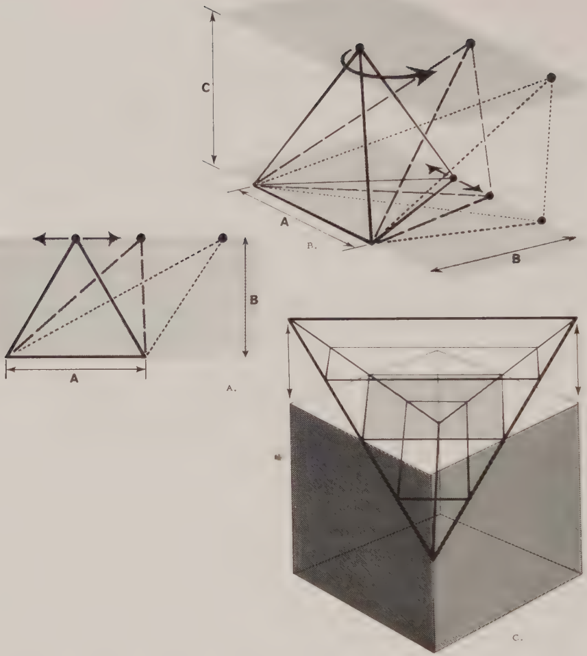
Fig. 621.01 Constant Properties of the Tetrahedron:
