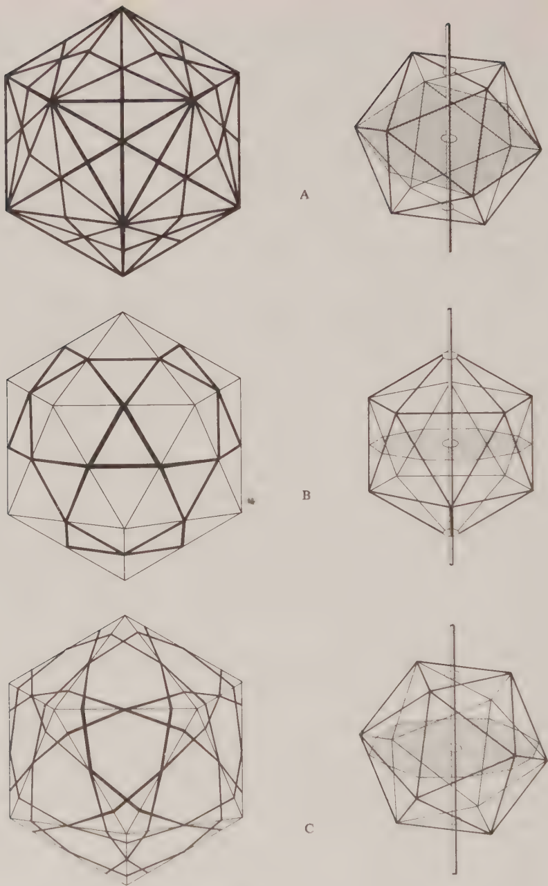
Fig. 457.30A Axes of Rotation of Icosahedron:
