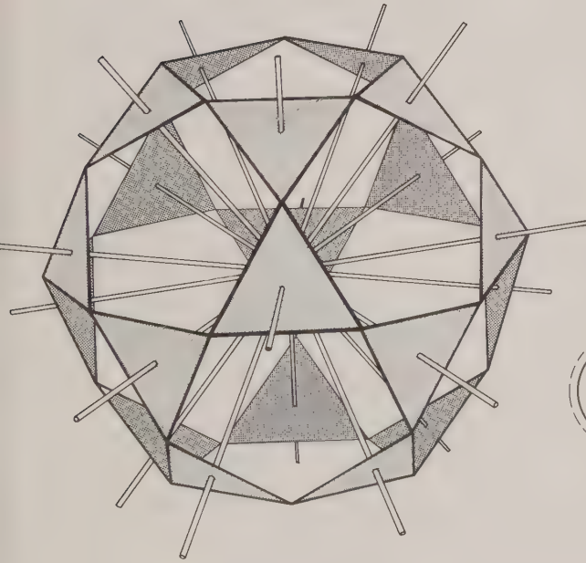
Fig. 465.00 Note that the eight triangular faces of the vector equilibrium are disposed about four-sided openings, i.e. square faces. It is possible to arrange 20 triangles in similar fashion around five-sided openings, i.e. pentagons. The shape is the icosidodecahedron. When a model is constructed with 20 spokes, i.e. ten axes, meeting at its center, which pass through the centers of each triangle, an unexpected behavior results. In the vector equilibrium model the triangles will rotate and contract towards its center, however, with the icosidodecahedron the entire structure remains fixed. It is not capable of contraction due to the fact that there is an odd number of triangles surrounding each opening. The diagrams show clearly why this is so. Any odd-numbered array of interlocked gears will not be free to rotate.
