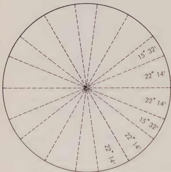
Fig. 455.20 The 12 Great Circles of the Vector Equilibrium Constructed from 12 Folded Units.
