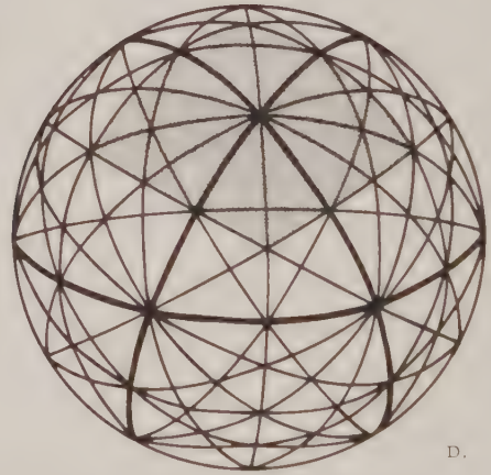
Fig. 454.06 Definition of Spherical Polyhedra in 25-Great-Circle Vector Equilibrium System : The 25 great circles of the spherical vector equilibrium provide all the spherical edges for four spherical polyhedra in addition to the vector equilibrium whose edges are shown here as heavy lines. The shading indicates a typical face of each as follows:
