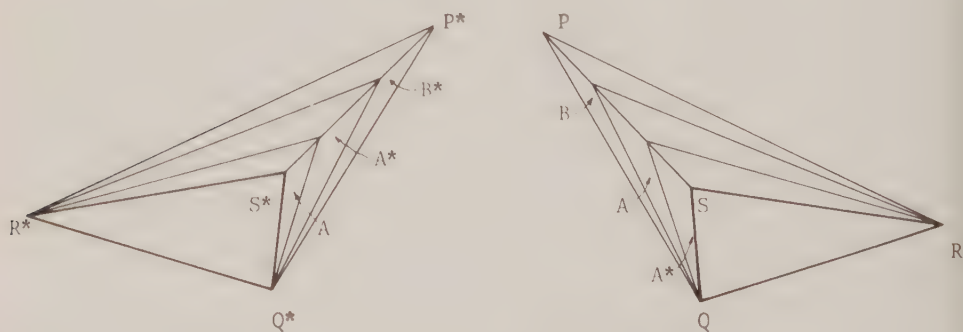
Fig. A24. The alternate arrangement of space filling with AA^*B and A^*AB^* modules.
