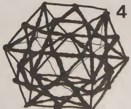
Fig. 450.11 Edge Lines Described by Twenty-five Great Circles of Vector Equilibrium : Each system corresponds with illustration 450.10.
