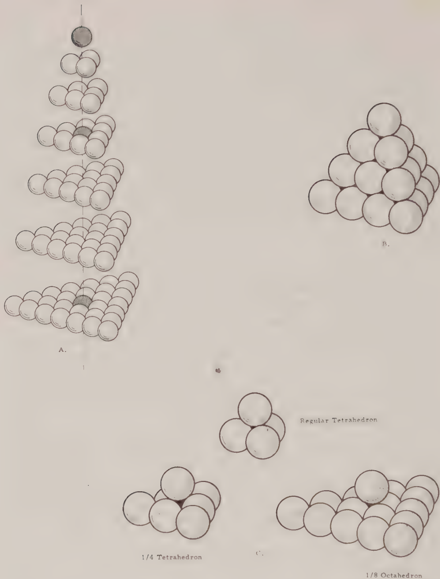
Fig. 415.55 Tetrahedral Closest Packing of Spheres: Nucleus and Nestable Configurations:
