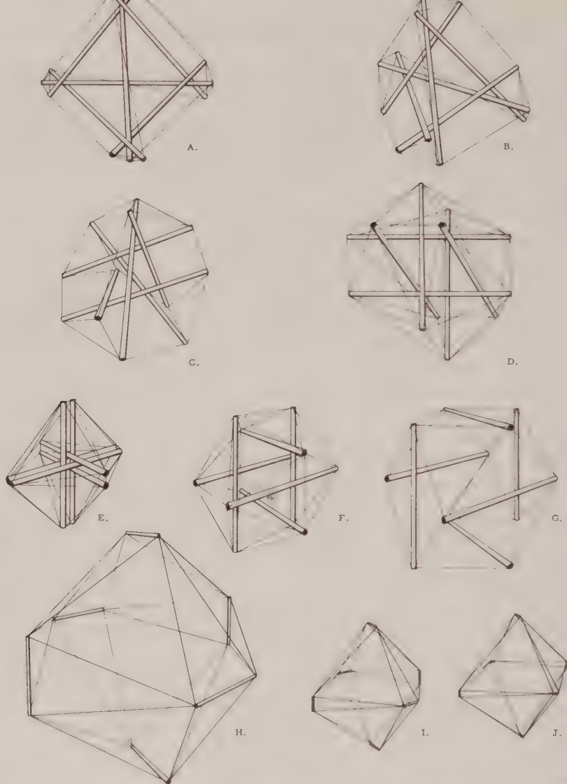
Fig. 725.02 Transformation of Six-Strut Tensegrity Structures : A six-strut tensegrity tetrahedron (A) can be transformed by changing the distribution and relative lengths of its tension members (B, C) to the six-strut icosahedron (D). A theoretical three-way coordinate expansion can be envisioned with three parallel pairs of constant-length struts in which a stretching of tension members is permitted as the struts move outwardly from a common center. Starting with a six-strut octahedron (E), the structure expands outwardly going through the icosahedron phase (F) to the vector-equilibrium phase (G). When the structure expands beyond the vector equilibrium, the six struts become the edges of figure H. They consequently lose their structural function (assuming the original distribution of tension and compression members remains unchanged). As the tension members become substantially longer than the struts, the struts tend to approach relative zero and the overall shape of the structure approaches a super octahedron (I, J).
