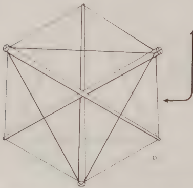
Fig. 724.30 Behavior of Tensegrity Icosahedron.
