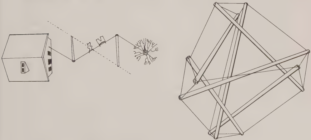
Fig. 712.01 Tensegrity Behavior.
