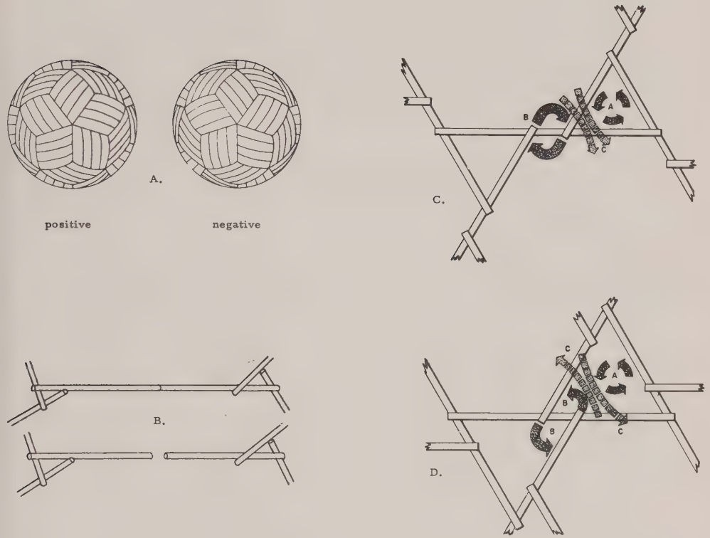
Fig. 770.11 System Turbining in Tensegrity Structures:
