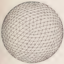
Regular Geodesic Nine-Frequency Icosahedron
