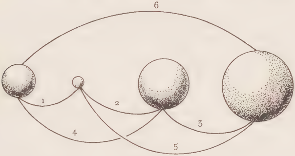
Fig. 2. Linear Tetrahedron. (A) A linear tetrahedron has six relationships. (B) Four unique frequencies (sizes) of entities, or particles; comprise the tetrahedron.
