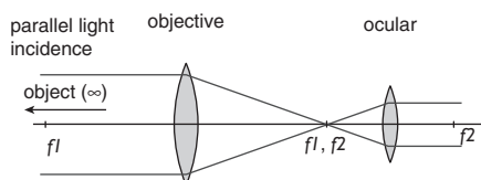
(b) Kepler telescope
