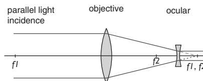
(c) Galilei telescope
