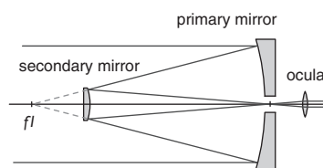
(e) Cassegrain telescope
