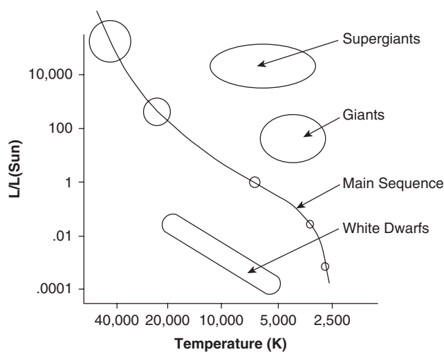
Figure 1 Hertzsprung-Russell diagram
