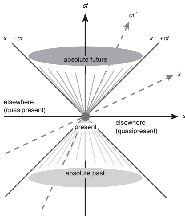
Figure 1 Minkowski diagram
