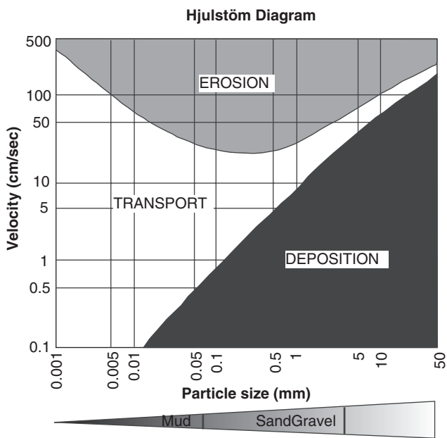
Figure 1 Hjulstöm's curve
