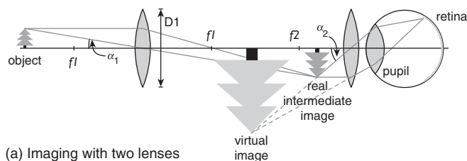
(a) Imaging with two lenses
