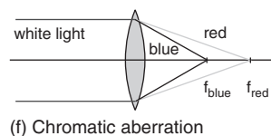
(f) Chromatic aberration
