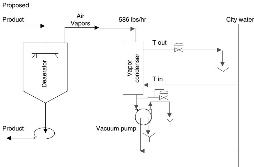
Fig. 5 Proposed equipment configuration.
