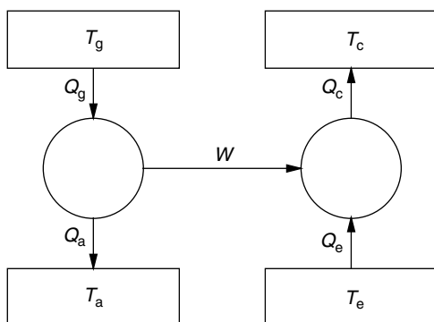
Fig. 4 Thermodynamic model of absorption heat pump.
