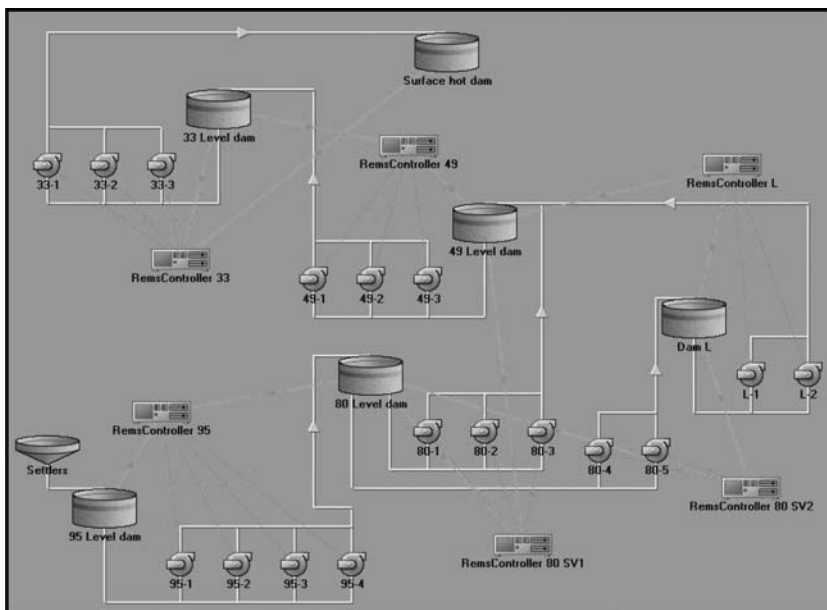
Fig. 7 Schematic layout of a typical intelligent pump scheduling system. Source: From HVAC International.
