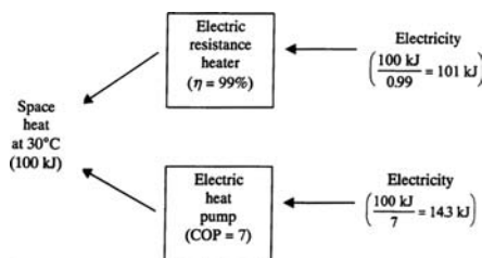
Fig. 1 Comparison of the quantity of electricity required to provide 100 kJ of space heat using two different heating devices: (a) an electric resistance heater and (b) an electric heat pump. Here, \eta denotes energy efficiency and COP coefficient of performance.
