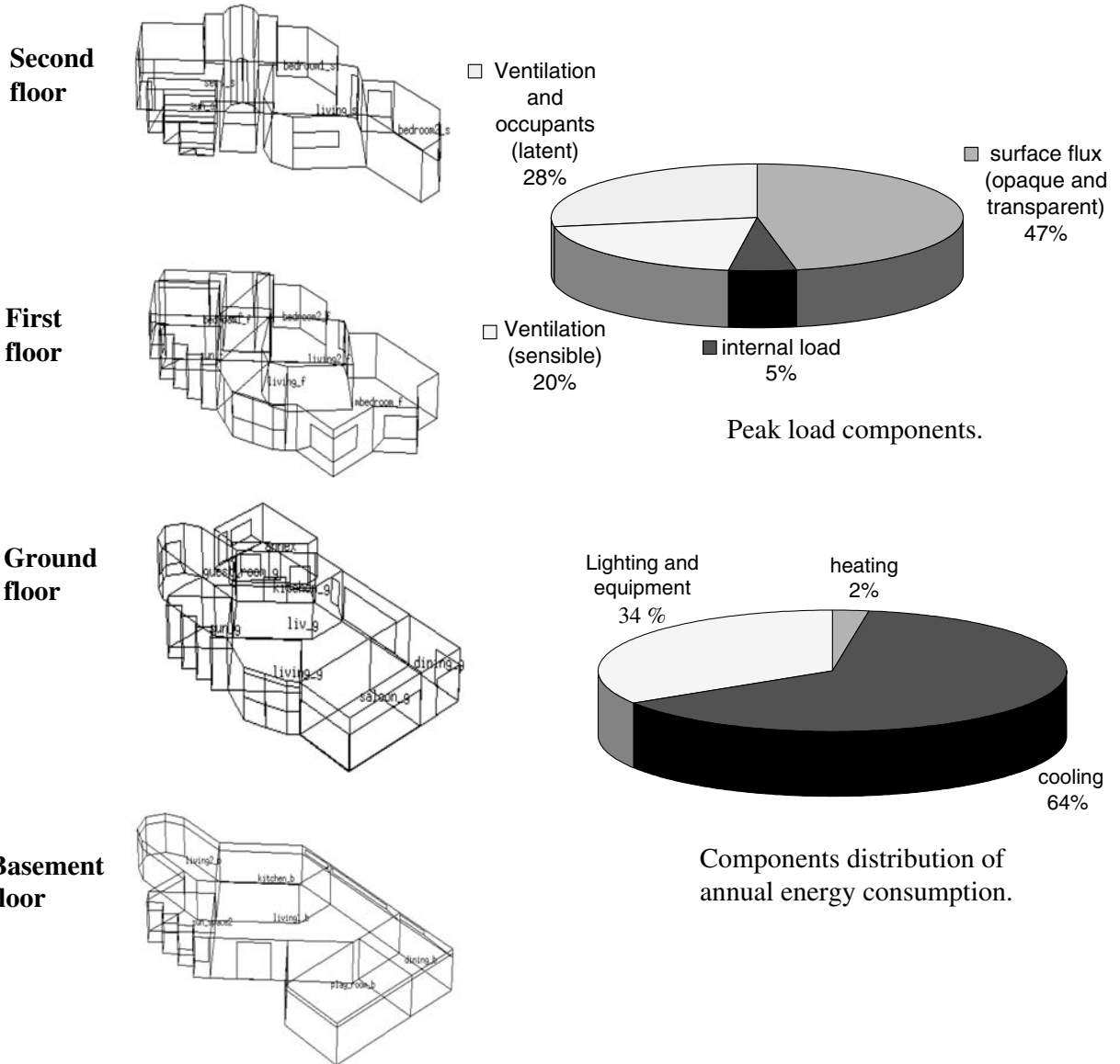
Wire-frame representation of each floor in the villa.
