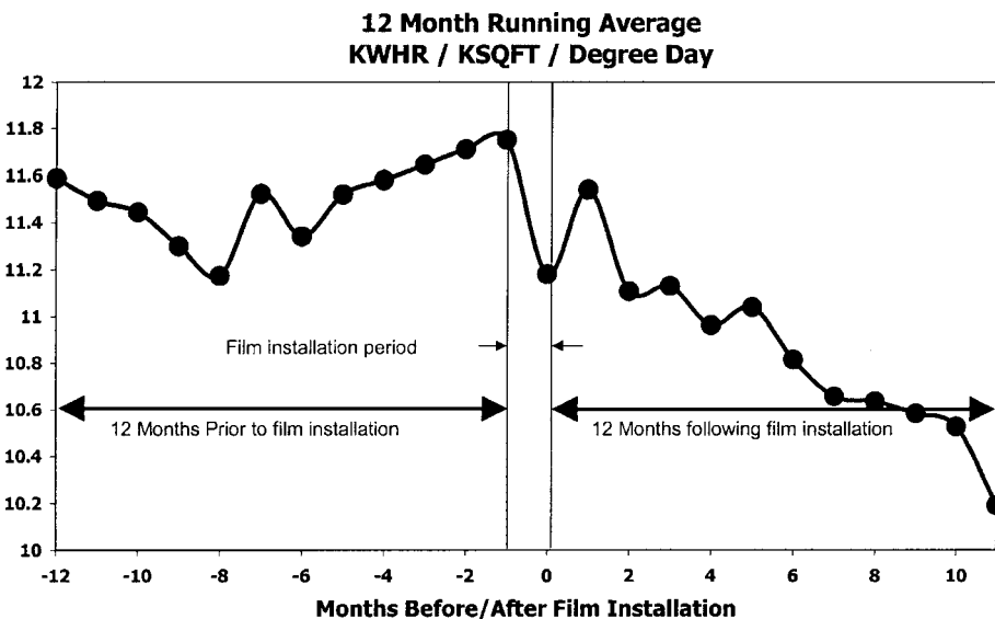
Fig. 3 Building energy use—before and after film installation.
