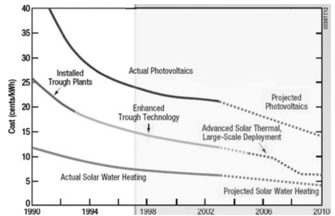
Fig. 2 The cost roadmap of solar energy technology. Source: From U.S. Department of Energy (see Ref. 11).
