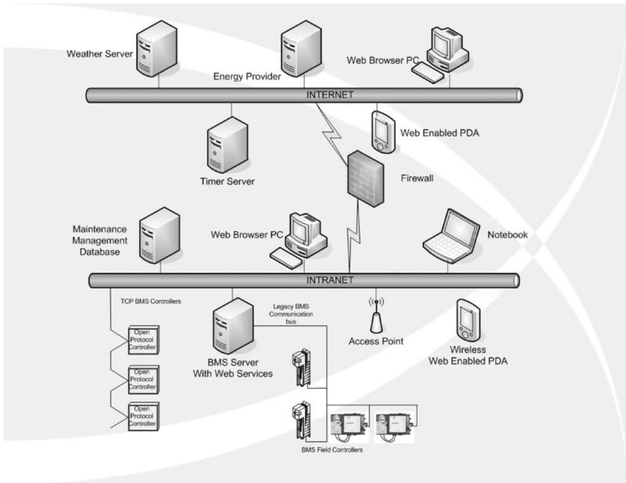
Fig. 1 Future building automation systems (BAS) network schematic.
