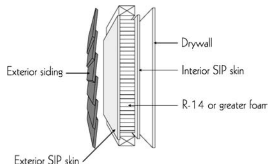
Fig. 12 Structural insulated panels (SIP).
