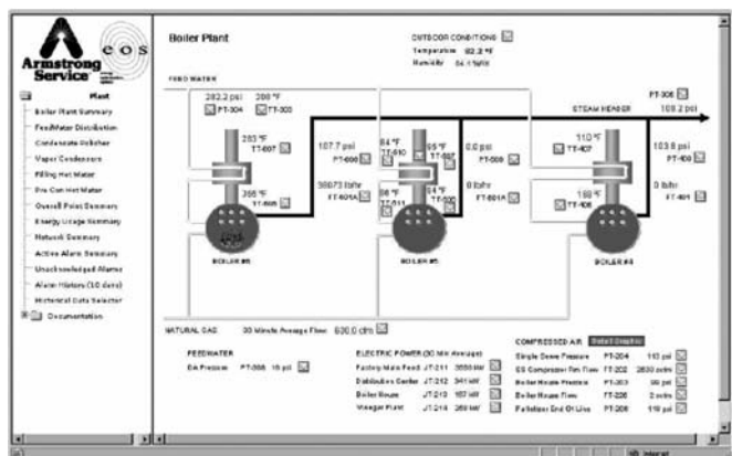
Fig. 2 Proposed economizer.
