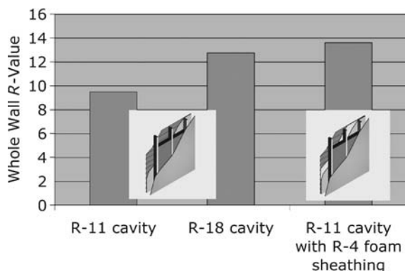
Fig. 4 Whole wall R -values for wood-framed (nominal 2×4) walls on 16-in. centers with interior gypsum and exterior wood siding in a one-story ranch house.
