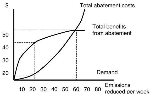
Fig. 3 Total benefits and total cost of abatement.
