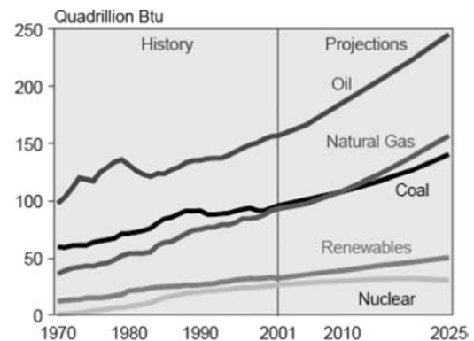
Fig. 6 World marketed energy consumption by energy source, 1970–2025. Source: From Washington Times Corporation (see Ref. 25).
