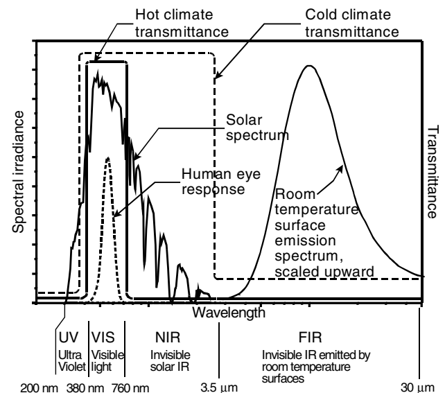
Fig. 7 Spectral irradiances of solar radiation and the infrared emission irradiance from a blackbody at room temperature. The blackbody curve is scaled so that its maximum value is the same as the solar spectrum maximum. Also shown are idealized spectral transmittances of both high and low solar gain low-e coatings.
