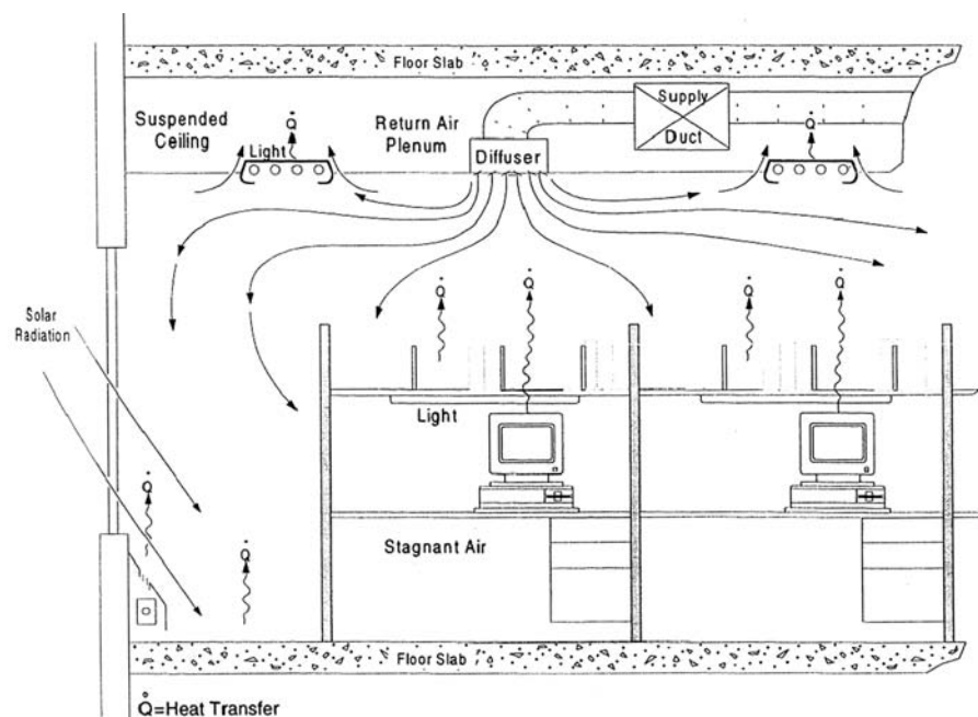
Fig. 3 Overhead system.
