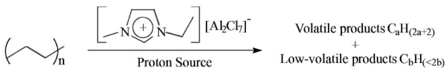
Figure 5.1-4: The products from the ionic liquid cracking of high-density polyethylene at 120 °C and at 200 °C.
