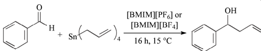
Scheme 5.1-25: Allylation of aldehydes in [BMIM][PF 6 ] or [BMIM][BF 4 ].
