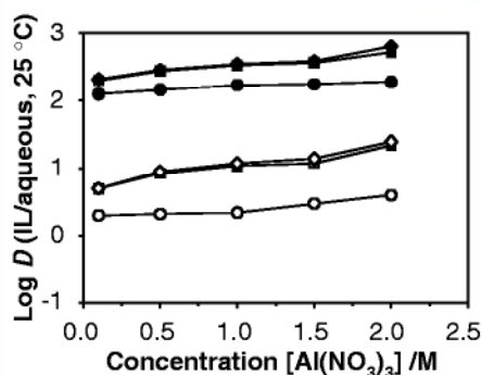
Figure 3.3-3: Distribution ratios for \text{Sr}^{2+} (closed symbol) and \text{Cs}^{+} (open symbol) with dibenzo-18-crown-6 (0.1 M) as extractant in IL/aqueous systems ( [\text{BMIM}][\text{PF}_6] (●), [\text{HMIM}][\text{PF}_6] (■), [\text{OMIM}][\text{PF}_6] (◆)) as a function of increasing aqueous phase concentrations of [\text{Al}(\text{NO}_3)_3] (M). From reference [7].
