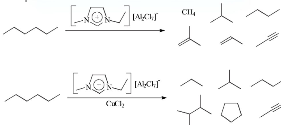
Scheme 5.1-69: The cracking of hexane in [EMIM]Cl/AlCl 3 ( X(\text{AlCl}_3) = 0.67 ) with and without added copper(II) chloride.
