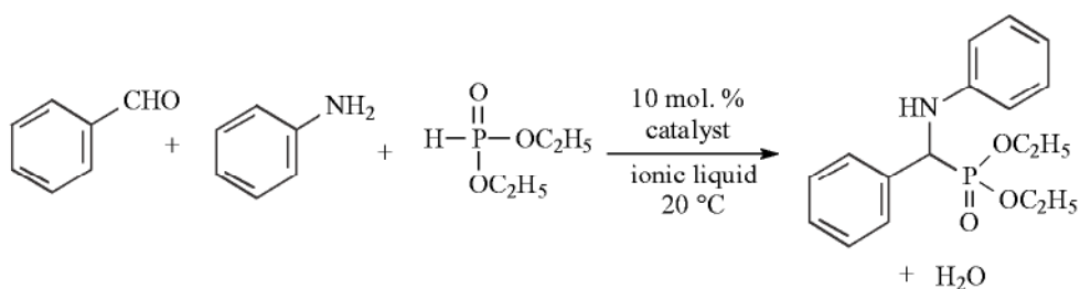
Scheme 5.1-43: Three-component reaction of benzaldehyde, aniline, and diethyl phosphonate in ionic liquids, catalyzed by lanthanide triflates and indium(III) chloride.
