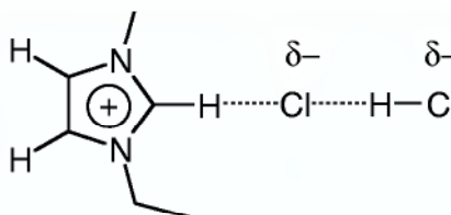
Figure 4.1-3: Proposed structure of the asymmetric [\text{HCl}_2]^- ion bound to the [\text{EMIM}]^+ cation in a binary mixture of \text{HCl}/[\text{EMIM}]\text{Cl} . The figure has been redrawn from reference 10 with permission.
