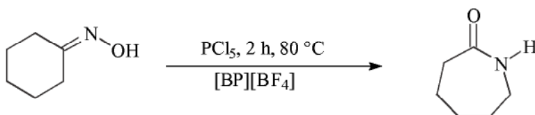
Scheme 5.1-31: The Beckmann rearrangement in ionic liquids.
