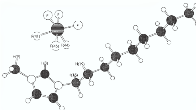
Figure 4.2-2: Molecular structure of [NMIM][PF 6 ] (MP2/6-31G(d,p)). C-H-F distances are: 2.355 Å (H9-F1), 2.198 Å (H8-F41), 2.636 Å (H8-F46), 2.164 Å (H8-F44), 2.439 Å (H15-F44), 2.403 Å (H19-F46), and 2.582 Å (H19-F44). All H-F distances are less than the H-F van der Waals distance of 2.67 Å (see ref. [18]).
