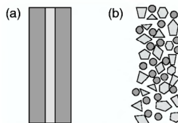
Figure 4.1-9: Schematic of the sample preparation methods used to study liquid EXAFS: (a) thin liquid film sandwich between low atomic weight plates, and (b) the liquid (circles) dispersed in a low atomic number matrix (polyhedrons). The figure has been redrawn from reference 40 with permission.
