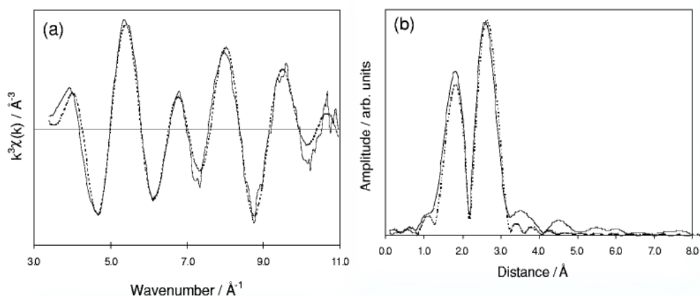
Figure 4.1-12: The experimental (solid line) and fitted (dashed line) U L III -edge (a) EXAFS data and (b) pseudo -radial distribution function after anodization of uranium in [\text{EMIM}]\text{Cl} . The figure has been redrawn from reference 48 with permission.
