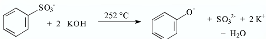
Scheme 5.1-1: The reaction of benzenesulfonates with fused KOH.
