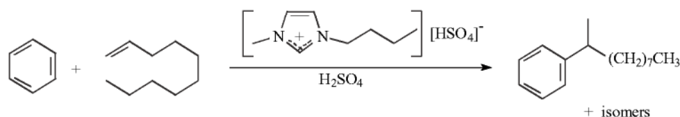
Scheme 5.1-54: The sulfuric acid-catalyzed alkylation of benzene in a hydrogensulfate ionic liquid.
