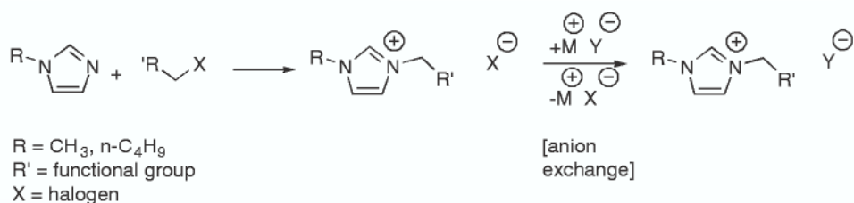
Scheme 2.3-1: General synthesis of task-specific ionic liquids from 1-alkylimidazoles. The preparation of functionalized pyridinium, phosphonium, etc. cations may be accomplished in like fashion.
