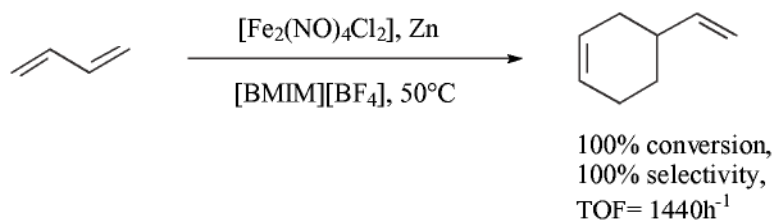
Scheme 5.2-24: Biphasic, Fe-catalyzed cyclotrimerization of butadiene in [BMIM][BF 4 ].
