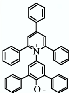
Figure 3.5-1: Reichardt's Dye.
