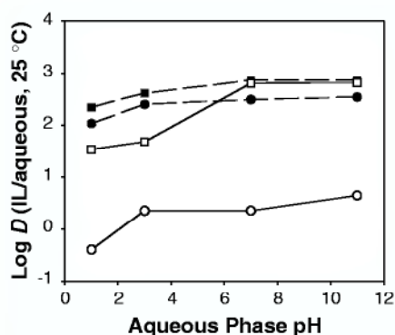
Figure 3.3-5: \text{Hg}^{2+} (■) and \text{Cd}^{2+} (○) distribution ratios between IL and aqueous phase with 1:1 [BMIM][PF 6 ] and urea-appended (dashed lines) or thiourea-appended (solid lines) TSILs as the extracting phase.
