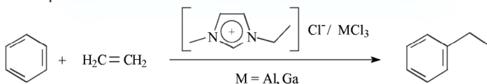
Scheme 5.1-51: The alkylation of aromatic compounds in chloroaluminate(III) or chlorogallate(III) ionic liquids.
