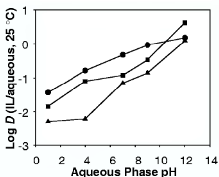
Figure 3.3-4: Metal ion distribution ratios for \text{Fe}^{3+} (●), \text{Cd}^{2+} (▲), and \text{Co}^{2+} (■) with 0.1 mM PAN in [\text{HMIM}][\text{PF}_6] /aqueous systems as a function of aqueous phase pH. From reference [8].
