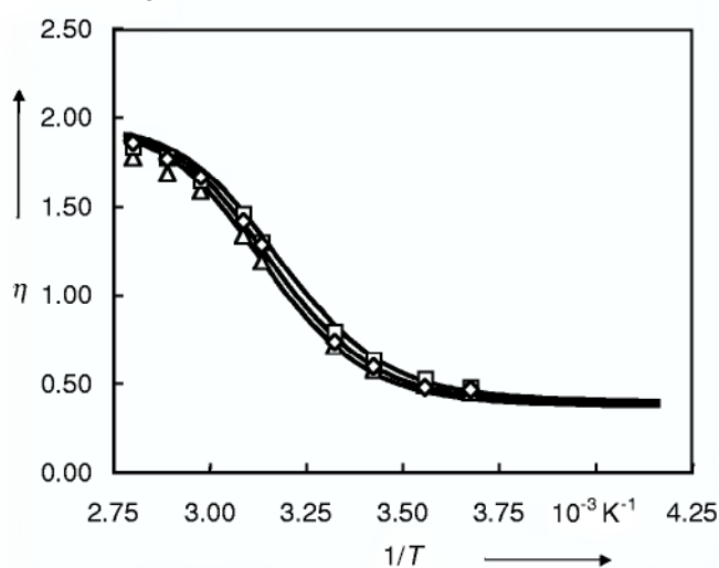
Figure 4.5-2: \{^1\text{H}\}\text{-}^{13}\text{C} NOE factors \eta for [BMIM][PF 6 ] in the neat liquid as a function of reciprocal temperature T ( \Delta : C2, \square and \diamond : C4 and C5, lines: functions calculated with the fitted parameters).
