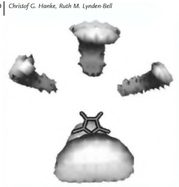
Figure 4.3-3: Three-dimensional distribution function of chloride ions relative to dimethylimidazolium ions.
