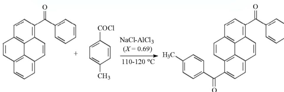
Scheme 5.1-59: The acylation of 1-benzoylpyrene in NaCl/AlCl 3 ( X(\text{AlCl}_3) = 0.69 ).
