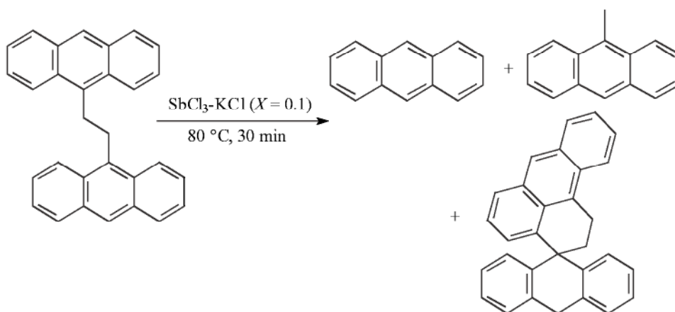
Scheme 5.1-12: The cyclisation of 1,2-bis-(9-anthryl)-ethane in antimony(III) ionic liquids.
