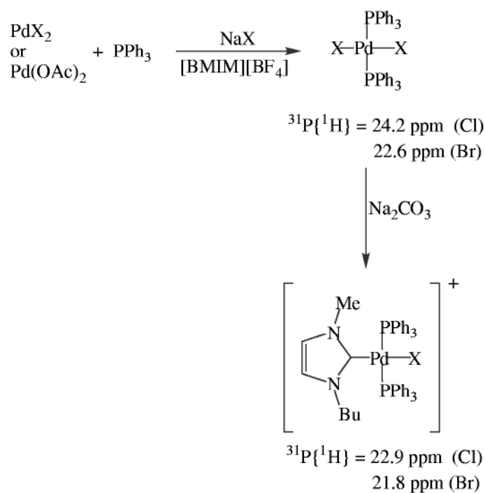
Scheme 6.1-4: The formation of (1-butyl-3-methylimidazolyidene)bis(triphenylphosphine)palladium(II) chloride in [BMIM][BF 4 ].
