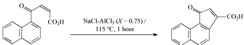
Scheme 5.1-47: The intramolecular cyclization of an alkene.
