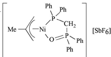
Figure 5.2-7: The cationic Ni-complex [(\text{mall})\text{Ni}(\text{dppmo})][\text{SbF}_6] as used for the biphasic oligomerization of ethylene to \alpha -olefins in, for example, [\text{BMIM}][\text{PF}_6] .
