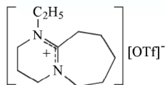
Figure 5.1-2: The structure of 1-ethyl-1,8-diazabicyclo[5,4,0]undec-7-enium trifluoromethanesulfonate [EDBU][OTf].
