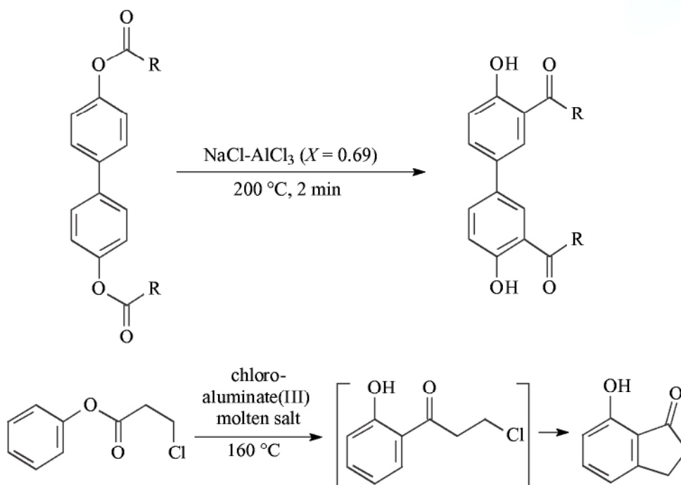
Scheme 5.1-61: The Fries rearrangement in chloroaluminate(III) molten salts.
