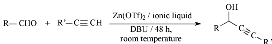
Scheme 5.1-27: The zinc triflate-catalyzed coupling of alkynes with aldehydes to give propargyl alcohols in an ionic liquid.
