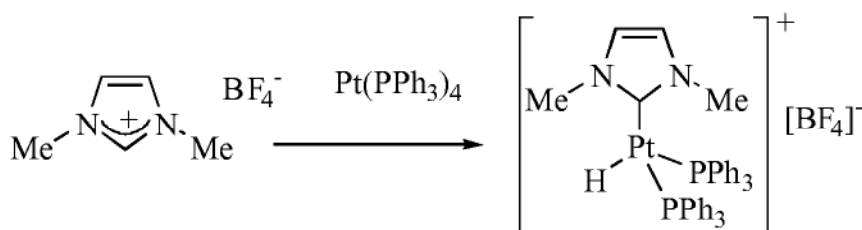
Scheme 5.3-3: Formation of carbene complexes by oxidative addition to Pt(0).
