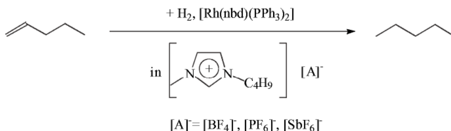
Scheme 5.2-7: Biphasic hydrogenation of 1-pentene with the cationic "Osborn complex" [Rh(nbd)(PPh 3 ) 2 ][PF 6 ] (nbd = norbornadiene) in ionic liquids with weakly coordinating anions.
