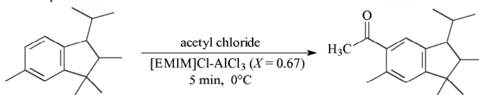
Scheme 5.1-63: The acetylation of 1,1,2,6-tetramethyl-3-isopropylindane in [EMIM]Cl/AlCl 3 ( X(\text{AlCl}_3) = 0.67 ).
