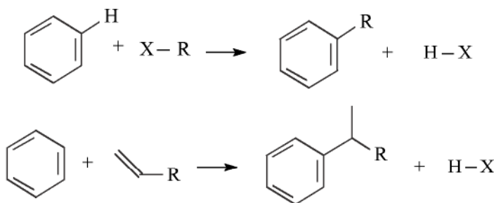
Scheme 5.1-44: The Friedel–Crafts alkylation reaction (R = alkyl, X = leaving group).
