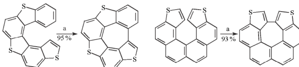
Scheme 5.1-9: The Scholl reactions of two helicenes. (a = NaCl/AlCl 3 (X(AlCl 3 ) = 0.69) at 140 °C).
