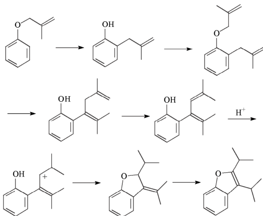
Scheme 5.1-42: Proposed mechanism for the formation of 2,3-diisopropylbenzo[ b ]furan.
