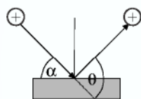
Scattered ions
