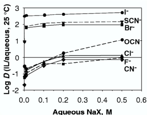
Figure 3.3-2: \text{Hg}^{2+} distribution ratios with increasing aqueous halide concentrations in [\text{BMIM}][\text{PF}_6] /aqueous systems. From reference [8].
