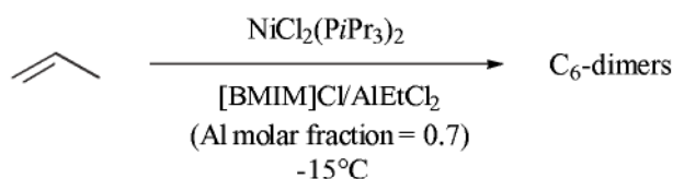
Scheme 5.2-1: Early examples of transition metal catalysis in ionic liquids.
