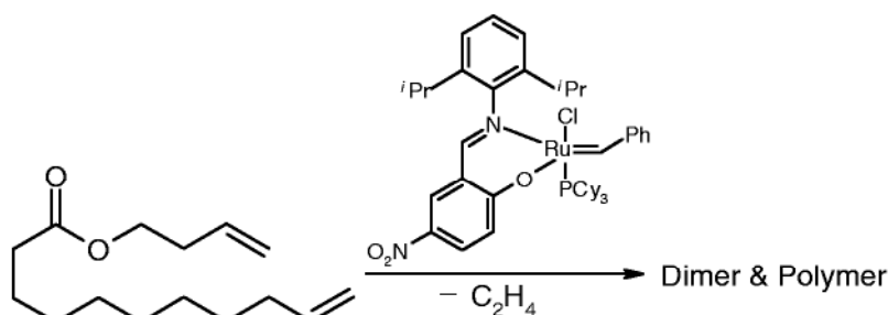
Figure 7.4-2: Acyclic diene metathesis polymerization (ADMET) reaction carried out in the neutral ionic liquid [EMIM]Cl/AlCl 3 ( X(\text{AlCl}_3) = 0.5 ) [52].
