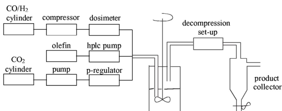
Figure 5.4-1: Continuous flow apparatus as used for the hydroformylation of 1-octene in the biphasic system [\text{BMIM}][\text{PF}_6]/sc\text{CO}_2
