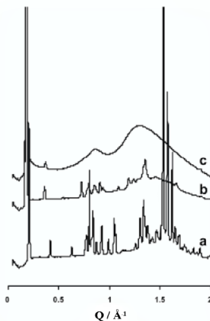
Figure 4.1-6: Small-angle X-ray diffraction data from [cetyltrimethylammonium] 2 [ZnCl 4 ] at (a) room temperature (solid), (b) 90 °C ( S C phase) and (c) 200 °C ( S A phase). Reproduced from reference 25 with permission.
