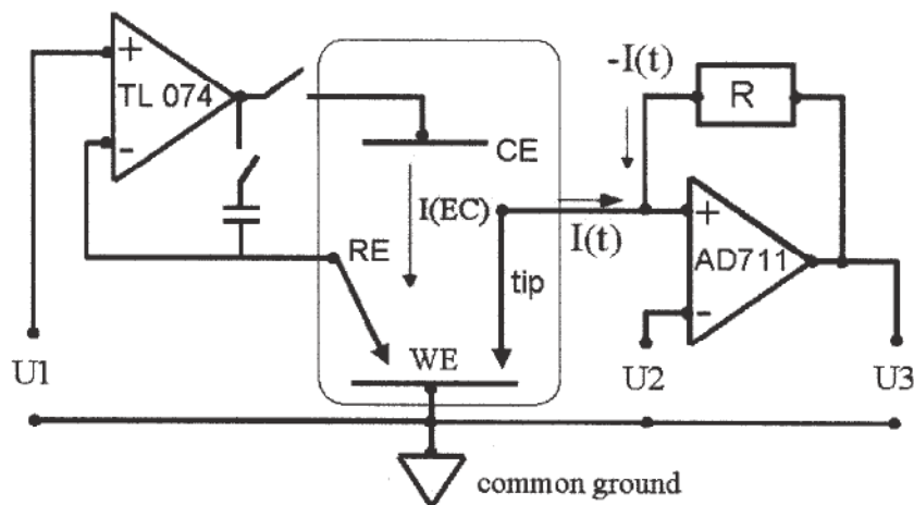
Figure 6.2-2: Simplified circuit of an electrochemical STM setup. In addition to the potentiostat (see Figure 6.2.1), an STM preamplifier is added, to which the tip is connected. U_1 : potentiostatic setpoint, U_2 : tunneling voltage, I(t) : tunneling current, U_3 = -R I(t) .
