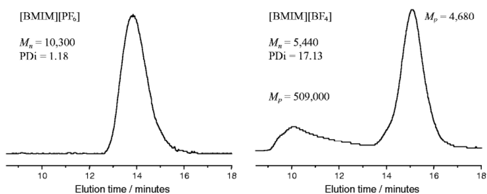
Figure 7.4-3: SEC traces for the Cu(I)Br-mediated living radical polymerization of MMA in the ionic liquids [BMIM][X] (X = [PF 6 ] or [BF 4 ] [44].
