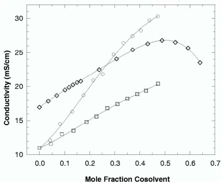
Figure 3.6-5: Change in the conductivity of [EMIM]Cl/AlCl 3 ionic liquids with the mole fraction of co-solvent: (□) benzene or (○) CH 2 Cl 2 added to a 55.56–44.44 mol % [EMIM]Cl/AlCl 3 ionic liquid, and (◇) benzene added to a 40.00–60.00 mol % [EMIM]Cl/AlCl 3 ionic liquid.
