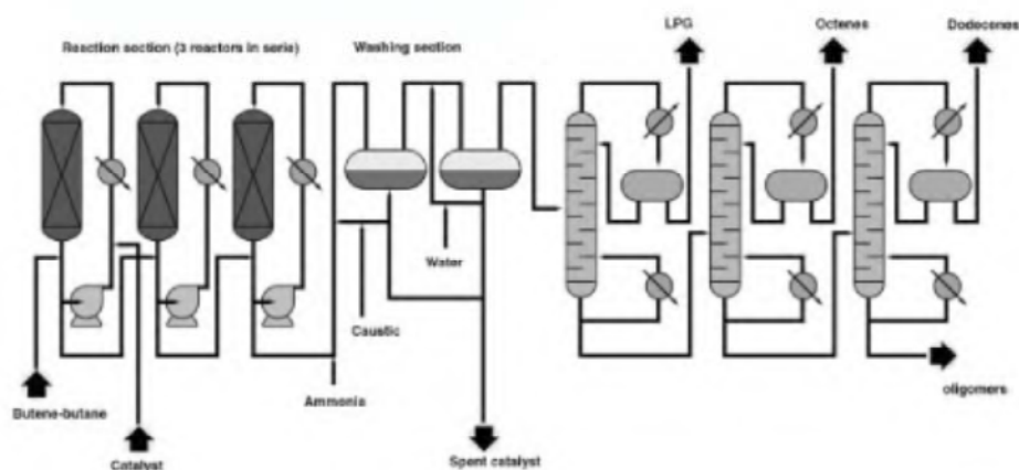
Figure 5.3-5: Dimersol process.
