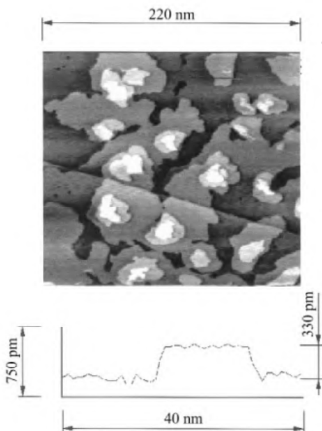
Figure 6.2-14: Bulk deposition of Ge on Au(111) in dry [BMIM] + PF 6 - at -2000 mV terraces with an average height of 330 \pm 30 pm, indicative of Ge(111) bilayers, are obtained.
