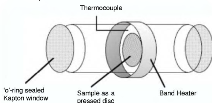
Figure 4.1-10: Schematic of transmission EXAFS cell. Reproduced from reference 36 with permission.
