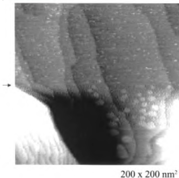
Figure 6.2-13: UPD phenomena of Ge on Au(111) in dry [BMIM] + PF 6 - : two-dimensional islands with an average height of 250 \pm 20 pm start growing upon a potential step from the open circuit potential to -500 mV vs. the Pt quasi reference electrode (picture from [59] – with permission of the Pccp owner societies).
