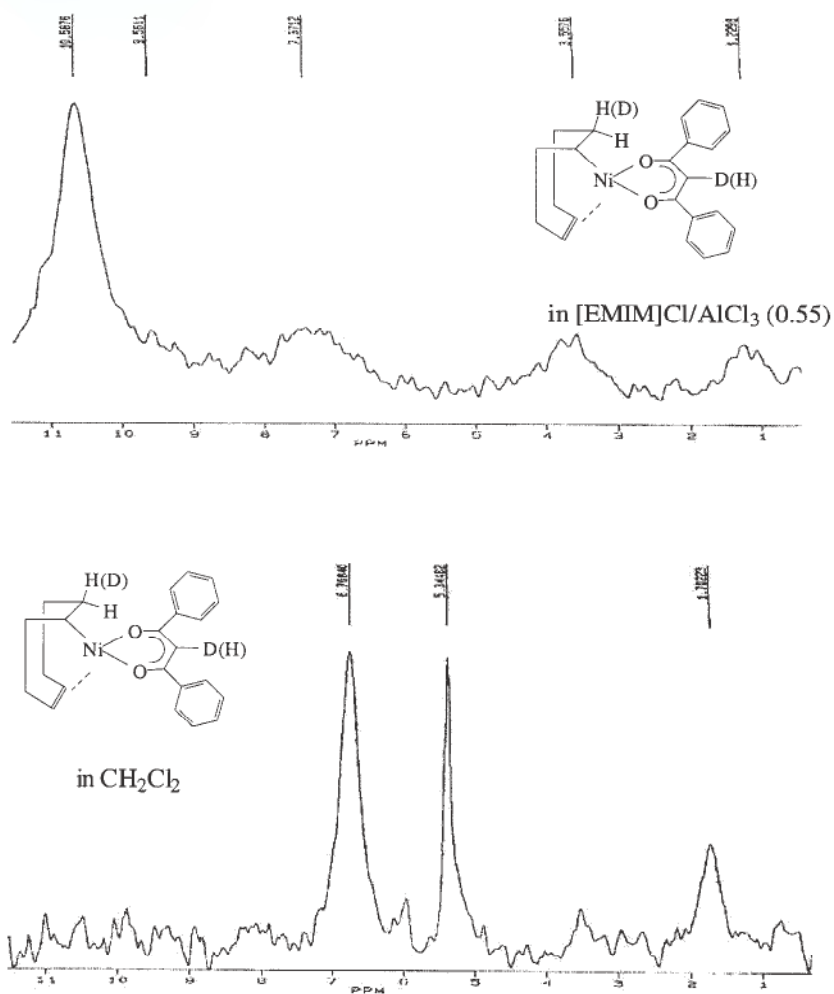
Figure 5.2-3: ^2\text{H} NMR spectra of the deuterated analogue of the square planar Ni-complex ( \eta -4-cycloocten-1-yl)(1,5-diphenyl-2,4-pentanedionato-O,O')nickel recorded [\text{EMIM}]\text{Cl}/\text{AlCl}_3 [ X(\text{AlCl}_3) = 0.55 ] and in \text{CH}_2\text{Cl}_2 .
