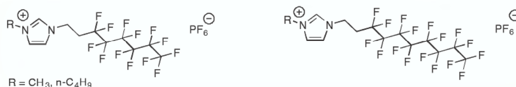
Figure 2.3-5: Imidazolium-based task-specific ionic liquids with cation-appended fluorinated tails.
