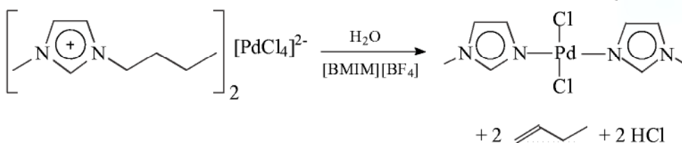
Scheme 5.2-5: Formation of the active Pd-catalyst from [\text{BMIM}]_2 \text{PdCl}_4 for the hydrodimerization of 1,3-butadiene.
