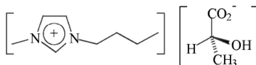
Figure 5.1-1: An example of a chiral ionic liquid used in the Diels-Alder reaction.
