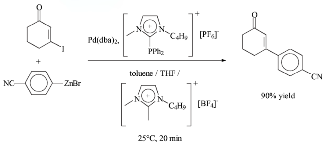
Scheme 5.2-20: Pd-catalyzed cross-coupling of organozinc compounds (Negishi cross-coupling) in [\text{BMMIM}][\text{BF}_4] .
