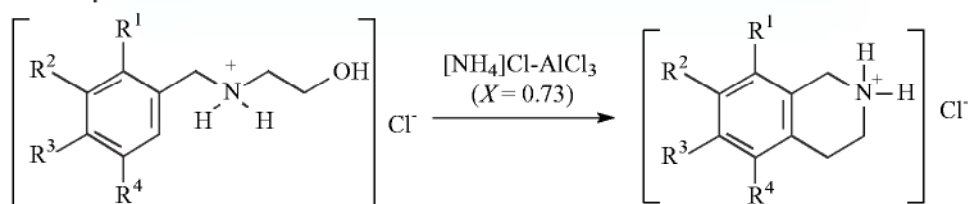
Scheme 5.1-48: The cyclodehydration of N -benzylethanolamine chloride.
