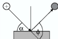
Sputtered(recoiled) ions
