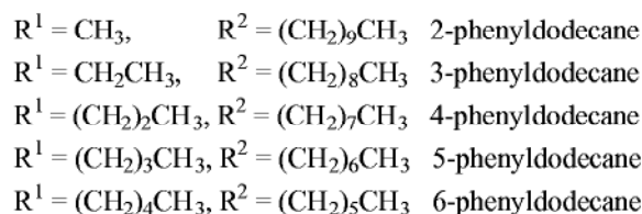
Scheme 5.1-56: The alkylation of benzene with dodecene with an ionic liquid on a solid support.
