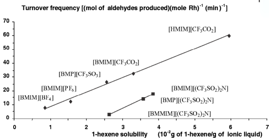
Figure 5.3-4: Turnover frequency of Rh-catalyzed hydroformylation as a function of 1-hexene solubility in ionic liquids. Reactions conditions: Rh(CO) 2 (acac) 0.075 mmol, 1-hexene/Rh = 800, TPPTS/Rh = 4, heptane as internal standard, CO/H 2 = 1 (molar ratio), P = 2 MPa, T = 80 °C, TOF determined at 25 % conversion of 1-hexene ([BMP] = N,N -butylmethylpyrrolidinium; [BMMIM] = 1-butyl-2,3-dimethylimidazolium)
