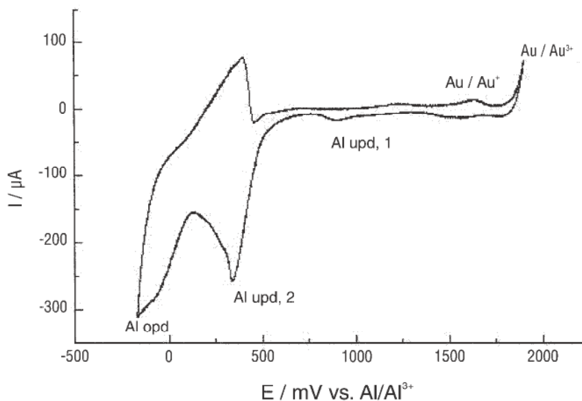
Figure 6.2-3: Cyclic voltammogram of acid [\text{BMIM}]^+\text{Cl}^-/\text{AlCl}_3 on Au(111): Au oxidation begins at electrode potentials > +1.2 V vs. \text{Al}/\text{AlCl}_3 . UPD processes are observed at about +900 and +400 mV before bulk deposition of Al starts (see also [65]).
