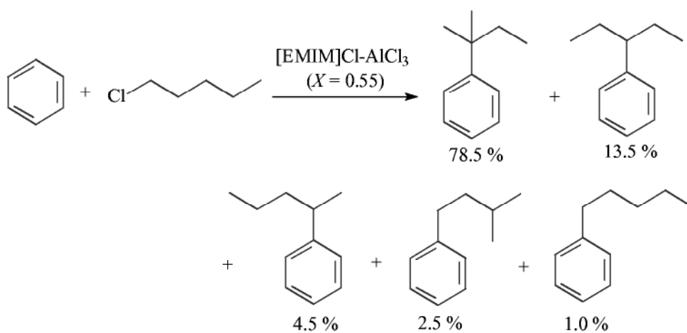
Scheme 5.1-50: The reaction between 1-chloropentane and benzene in [\text{EMIM}]\text{Cl}/\text{AlCl}_3 ( X(\text{AlCl}_3) = 0.55 ).
