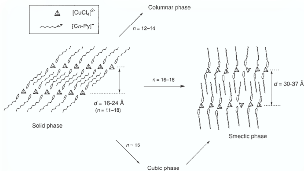
Figure 4.1-5: Schematic showing the changes in structure of N -alkylpyridinium tetrachlorocuprate salts with varying alkyl chain lengths. Reproduced from reference 23 with permission.
