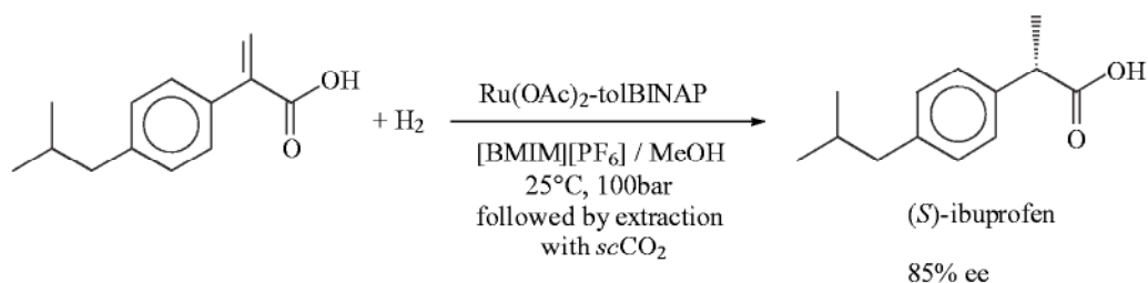
Scheme 5.2-11: Ru-catalyzed asymmetric hydrogenation of isobutylatropic acid, followed by extraction of the product ibuprofen with sc CO 2 .
