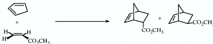
Figure 3.5-2: Diels–Alder cycloaddition between cyclopentadiene and methyl acrylate.
