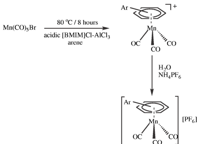
Scheme 6.1-7: The synthesis of [\text{Mn}(\text{CO})_3(\eta^6\text{-arene})]^+ “piano stool” complexes in [\text{BMIM}]\text{Cl}/\text{AlCl}_3 .
