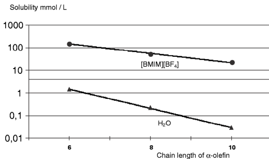
Figure 5.3-2: Comparison of the solubilities of \alpha -olefins with different numbers of carbon atoms in water and in [BMIM][BF 4 ].
