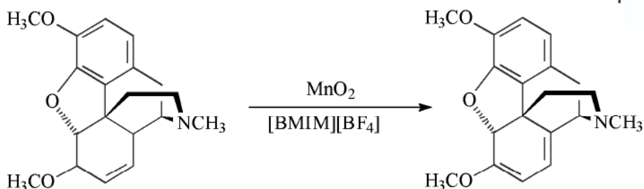
Scheme 5.1-35: The oxidation of CME to thebaine in [BMIM][BF 4 ].
