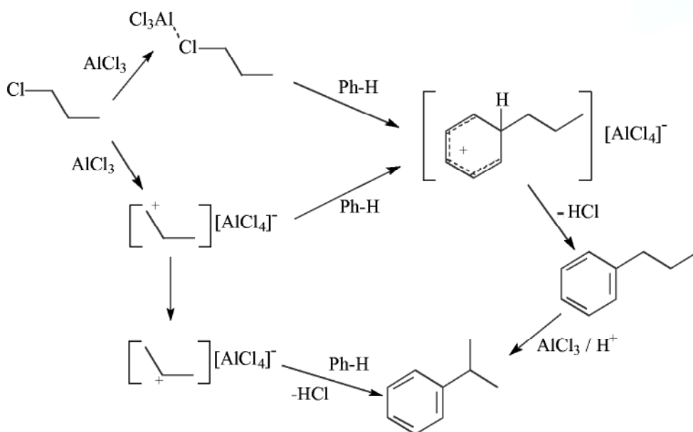
Scheme 5.1-45: The reaction between 1-chloropropane and benzene under Friedel-Crafts conditions.
