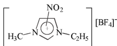
Scheme 5.1-36: The nitration of toluene with [\text{NO}_2][\text{BF}_4] in [\text{EMIM}][\text{BF}_4] .
