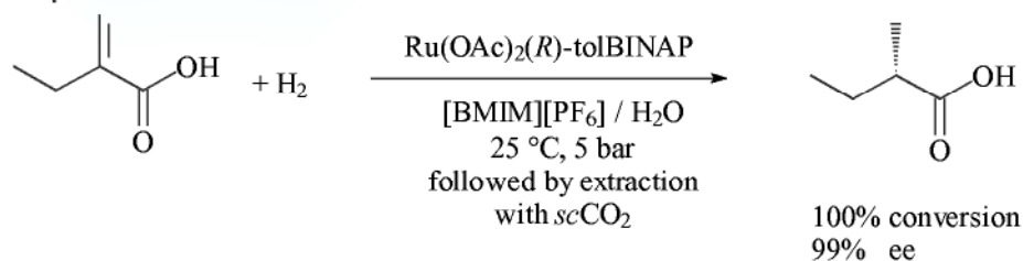
Scheme 5.2-10: Ru-catalyzed asymmetric hydrogenation of tiglic acid, followed by product extraction with sc CO 2 .
