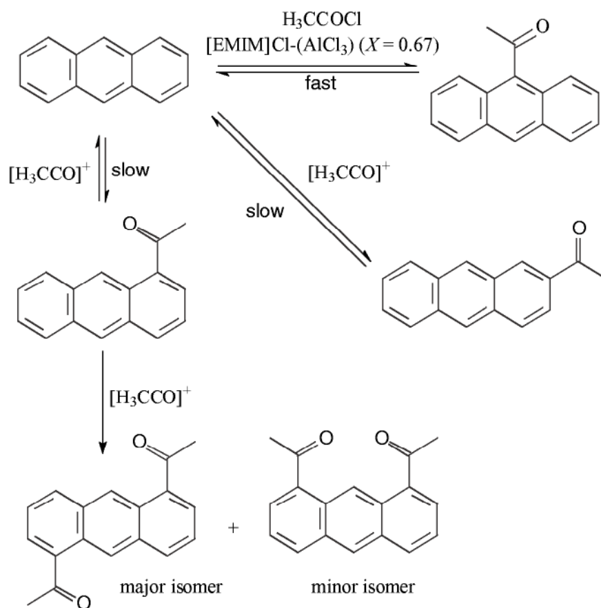
Scheme 5.1-64: The acetylation of anthracene in [EMIM]Cl/AlCl 3 ( X(\text{AlCl}_3) = 0.67 ).
