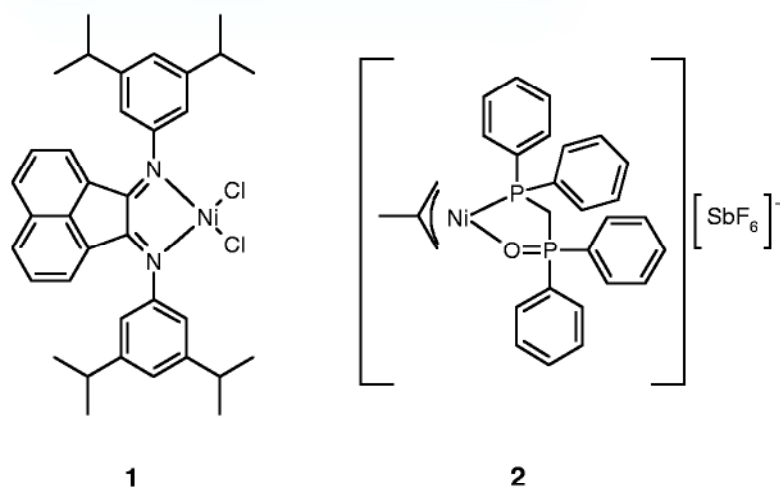
Figure 7.4-1: Nickel catalysts used for the polymerization and oligomerization of ethylene in ambient-temperature ionic liquids [48, 49].
