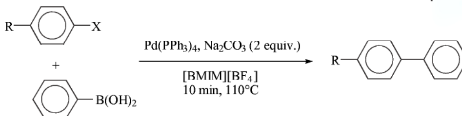
Scheme 5.2-18: Pd-catalyzed Suzuki cross-coupling reaction in a [BMIM][BF 4 ] ionic liquid.
