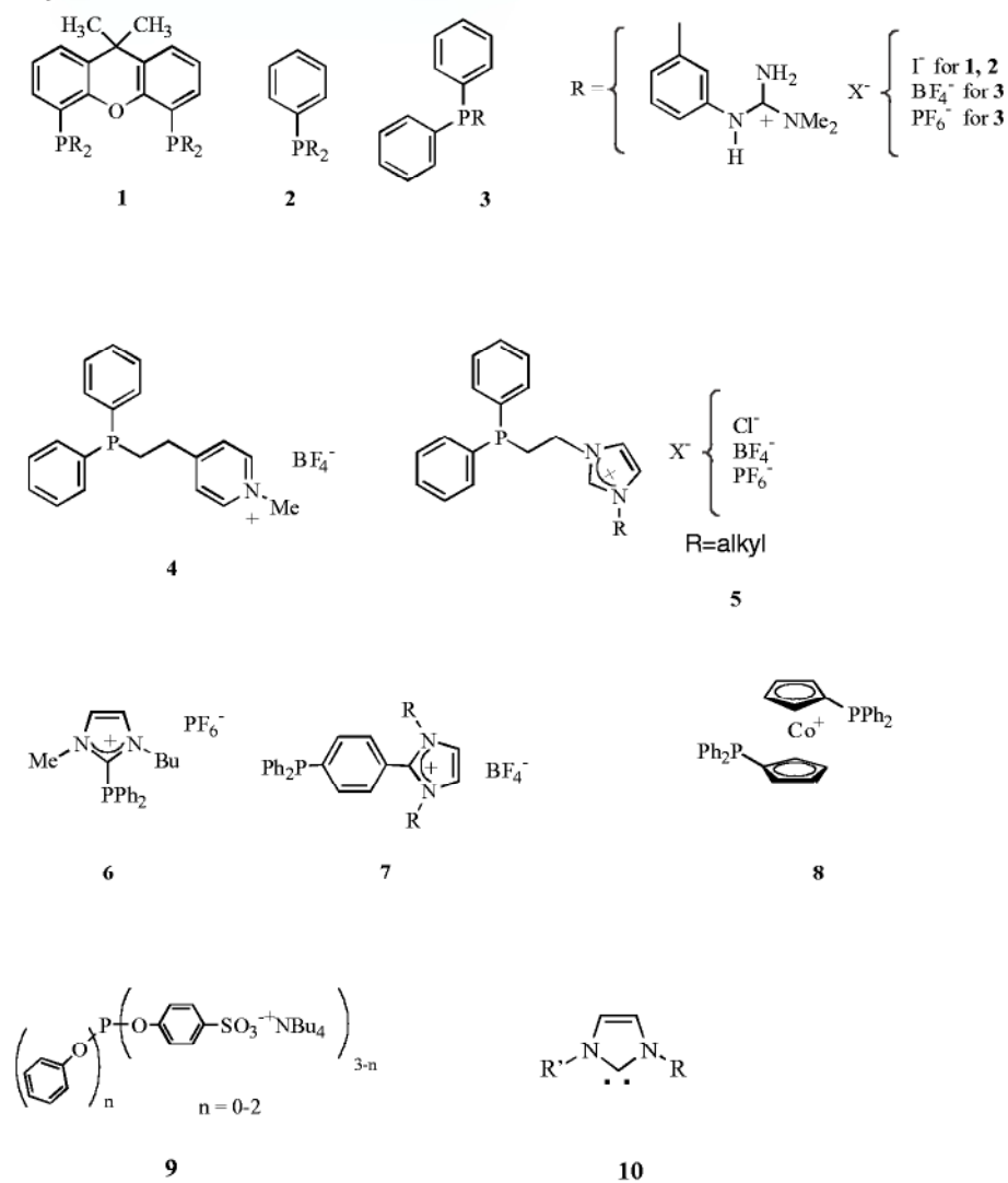
Scheme 5.3-1: Ligands 1-10.
