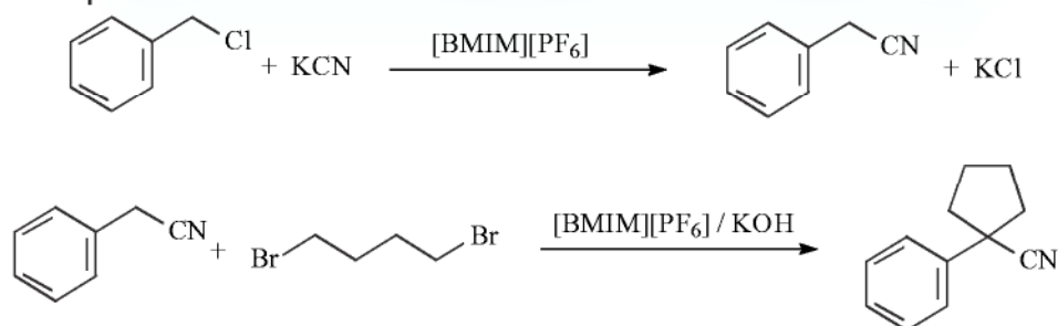
Scheme 5.1-23. The reaction of cyanide with benzyl chloride to produce 1-phenylacetonitrile, and subsequent treatment with 1,4-dibromobutane.
