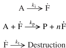
Fig. 3.2 Explosion in branching chain reactions.
