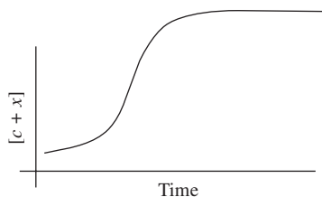
Fig. 1.5 Plot of (c + x) versus time.
