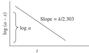
Fig. 1.3 The \log [conc.] versus time plot for first-order reaction.
