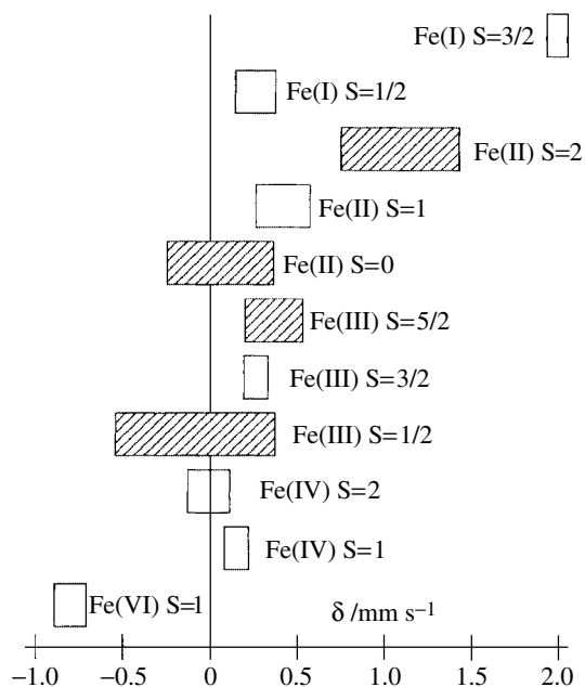
Figure 3.47 Ranges of isomer shift ( \delta ) values observed for iron compounds, coordination species, and polymers relative to metallic iron. S = spin quantum number. From Gütlich and Enslin, op cit., p 181, © 1999, John Wiley and Sons.
