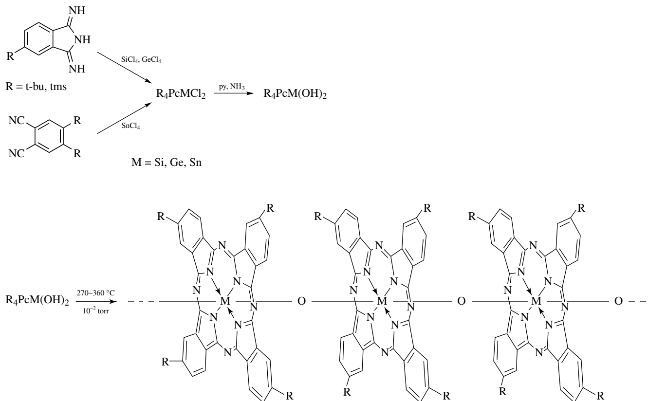
Figure 2.4 The synthesis of solubilized [\text{MPcO}]_n where M = \text{Si, Ge, Sn} ; \text{Pc} = \text{tetra-}t\text{-butylphthalocyanato} (6); and n = \sim 25 [J. W. Buchler, Metal Complexes with Tetrapyrrole Ligands II , Springer-Verlag: Berlin, 1991, pp 41-146].
