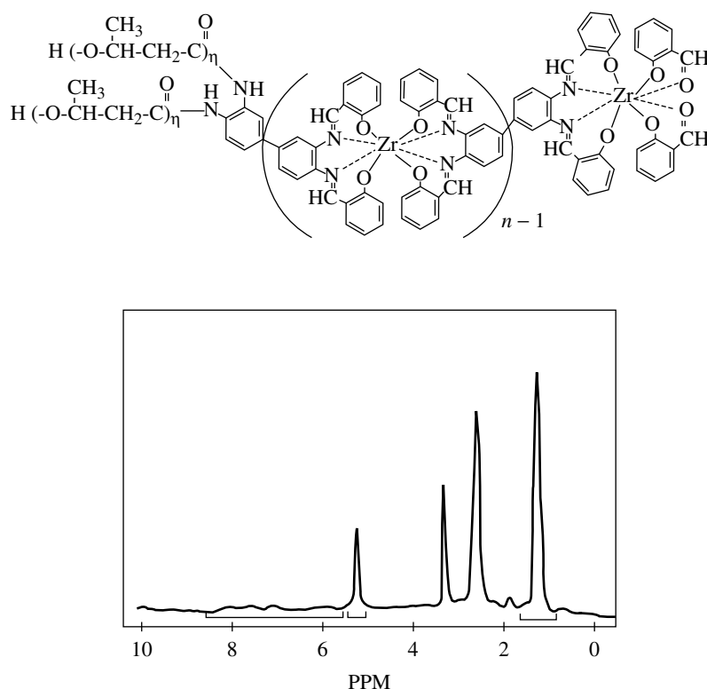
Figure 3.31 The copolymerization reaction between Zr(\text{tsdb})_n and (\pm)\beta -butyrolactone and the proton NMR spectrum of the product. (Spectrum taken by B. Wang.)
