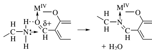
Figure 2.17 The schematic representation of the enhancement of a Schiff-base reaction between an aldehyde and an amine by a highly charged metal center.
