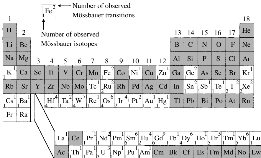
Figure 3.48 Periodic table of the elements for which the Mössbauer effect has been observed (in white) and those for which such an effect has not been observed (in gray). From Gütlich and Enslin, op cit., p 163, © 1999, John Wiley and Sons.
