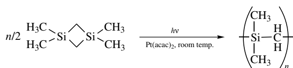
Figure 2.40 The photocatalyzed ring-opening polymerization of a carbosilane.
