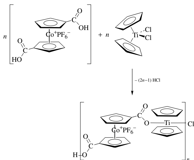
Figure 2.14 A mixed cobalticene/titanicene polymer synthesis.
