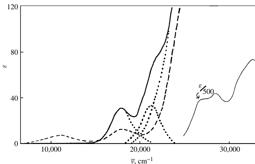
Figure 3.38 Absorption spectra for bis(1,1,1-trifluoro-4-pentene-2-ono)nickel(II): planar in dry benzene or chloroform (—) and octahedral in pyridine (----). A spectral band analysis of the visible bands for the planar complex is also shown (••••).
