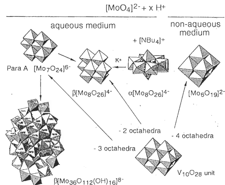
Figure 4.23 Structure of a few molybdc ions
