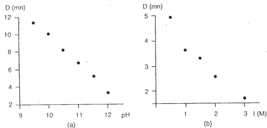
Figure 8.15 Average size of \text{Fe}_3\text{O}_4 particles formed (a) at various pH ( I = 0.5\text{M} ) and (b) at various ionic strengths ( \text{pH} = 12 ) after 8 day ageing at 25^\circ\text{C} . Reproduced with kind permission from Kluwer Academic Publishers from [43]
