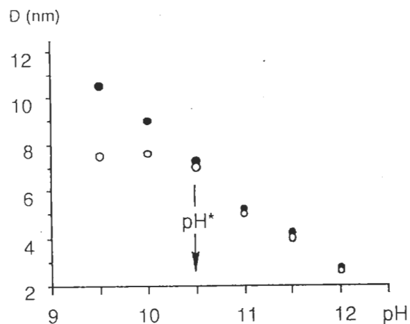
Figure 8.16 Average size of \text{Fe}_3\text{O}_4 synthesized at various pH, ( 25^\circ\text{C} , I = 0.5\text{M} ) immediately after precipitation ( \circ ) and after 8 day ageing ( \bullet ). Reproduced with kind permission from Kluwer Academic Publishers from [43]
