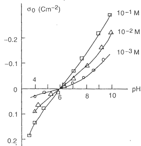
Figure 6.4 Variation in the surface charge of \text{TiO}_2 anatase as a function of the pH of NaCl solutions for several concentrations. Reproduced by permission of Academic Press from [17]
