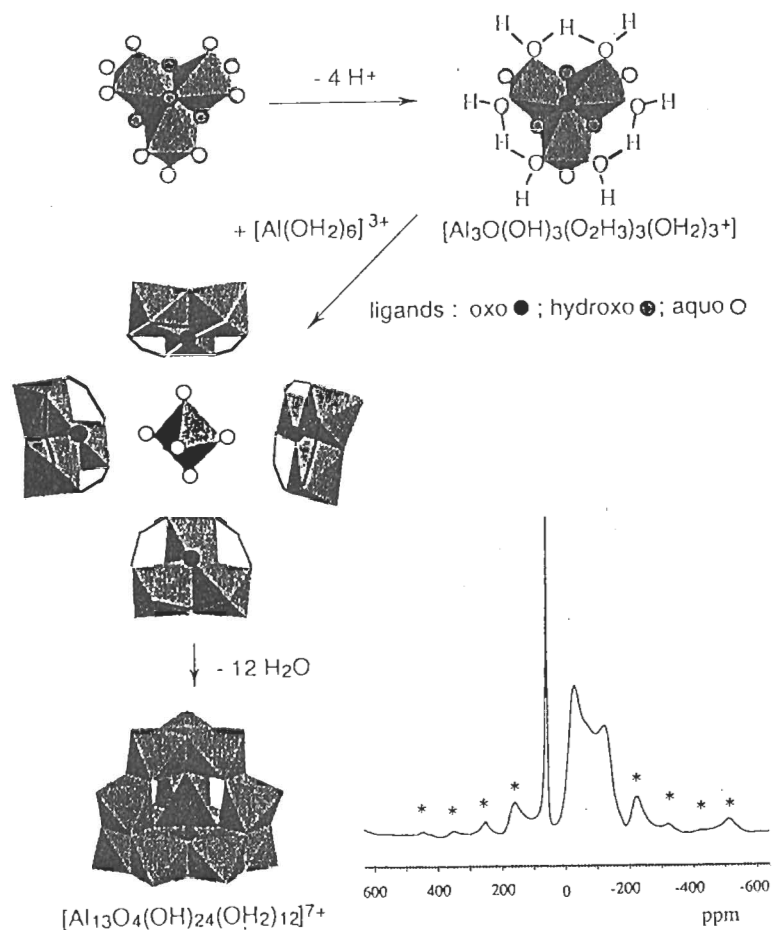
Figure 3.5 Possible formation mechanism of [Al_{13}O_4(OH)_{24}(OH_2)_{12}]^{7+} and ^{27}Al MAS-NMR spectrum of the sulfate salt of the polycation Al_{13} measured at 9.4 T, with spinning speed of 15 kHz; *spinning sidebands (J. Hernandez and J.P. Jolivet, unpublished results)
