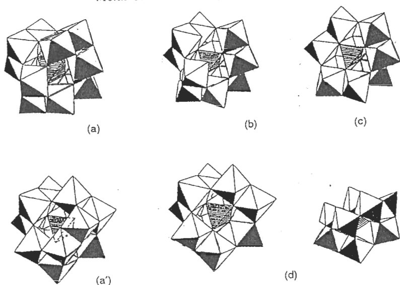
Figure 5.10 Structure of (a) \alpha -[PW 12 O 40 ] 3- (Keggin structure) and derivatives (b) \alpha -[PW 11 O 39 ] 7- and (c) A\alpha -[PW 9 O 34 ] 9- . (a') \gamma isomer of Keggin's polyanion (two W 3 O 13 groups have rotated 60°). From [37] by permission. (d) Vacancy compound [PW 10 O 36 ] 7- . Reprinted with permission from [42]. Copyright 1981 American Chemical Society
