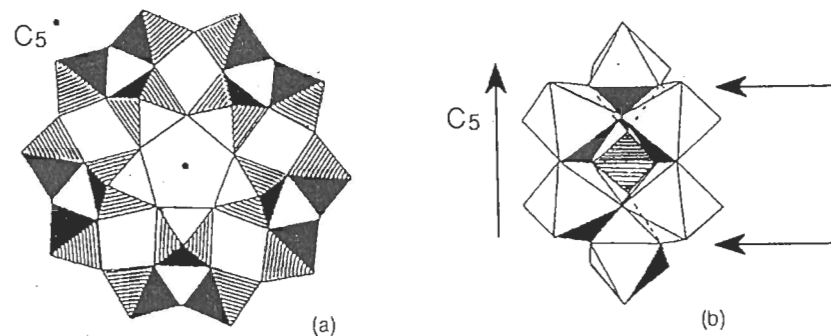
Figure 5.13 (a) Structure of [NaP 5 W 30 O 110 ] 14- . (b) PW 6 O 32 fragment shown parallel to the C 5 axis. The arrows perpendicular to the C 5 axis indicate the planes where sodium is located within the crown. Reprinted with permission from [49]. Copyright 1985 American Chemical Society
