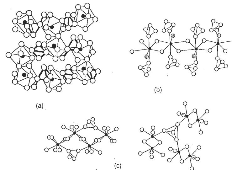
Figure 5.4 Structures of basic sulfates of zirconium: (a) \text{Zr}_2(\text{OH})_2(\text{SO}_4)_3(\text{OH}_2)_4 ; (b) \text{Zr}(\text{OH})_2(\text{OH}_2)(\text{SO}_4) ; (c) \text{Zr}(\text{OH})_2(\text{SO}_4)
