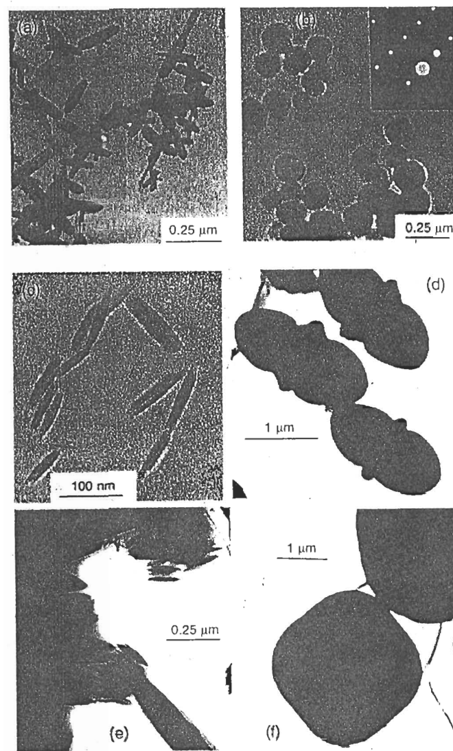
Figure 2.12 (a) Akaganeite particles formed by treatment of a solution of \text{FeCl}_3 ( 0.018 \text{ mol l}^{-1} ) and \text{HCl} ( 0.01 \text{ mol l}^{-1} ) at 100^\circ\text{C} for 12 h and (b) transformation into pseudospherical hematite particles after 1 week of heating; (c) akaganeite particles formed by heat treatment of a solution of \text{FeCl}_3 ( 0.018 \text{ mol l}^{-1} ) and \text{HCl} ( 0.05 \text{ mol l}^{-1} ) at 100^\circ\text{C} for 1 h and (d) transformation into double ellipsoidal hematite after 1 week of heat treatment; (e) aggregates of akaganeite particles obtained by heat treatment of a solution of \text{FeCl}_3 ( 0.45 \text{ mol l}^{-1} ) and \text{HCl} ( 0.01 \text{ mol l}^{-1} ) at 150^\circ\text{C} for 13 min and (f) transformation into particles of cubic hematite after 24 h of heat treatment. Reproduced by permission of Academic Press from [49]
