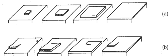
Figure 2.9 (a) Surface nucleation with two-dimensional growth of the nuclei. The hatched area represents the surface created by the formation of the nucleus. (b) Spiral growth around a defect
