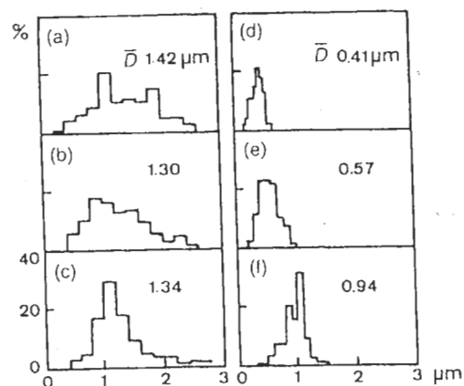
Figure 5.17 Particle size distribution of anatase as a function of the heating time at 95°C (a–c) in a sulfate medium \text{Na}_2\text{SO}_4 ( 0.48 \text{ mol l}^{-1} ) and (d–f) in a fluoride medium \text{NaF} ( 0.11 \text{ mol l}^{-1} ). Heat treatment time: (a), (d) 1 h; (b), (e) 3 h; (c), (f) 6 h. \text{HCl} 2.13 \text{ mol l}^{-1} , \text{Ti} 0.22 \text{ mol l}^{-1} . Reproduced from [72] by permission
