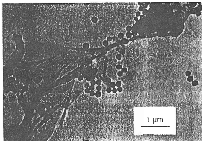
Figure 5.19 TEM micrograph of thermohydrolysis products at 75°C of \text{KCr}(\text{SO}_4)_2 ( 4 \times 10^{-4} \text{ mol l}^{-1} , initial pH 3.7, final pH 3.3). Reproduced by permission of Academic Press from [2b]
