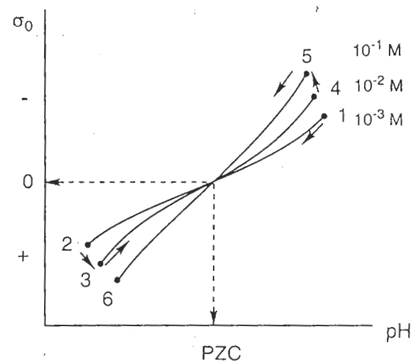
Figure 6.5 Proton titration curve of an oxide suspension for various electrolyte concentrations. Reproduced by permission of Academic Press from [18]
