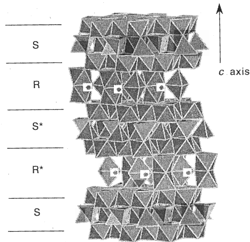
Figure 5.26 Structure of barium hexaferrite BaFe_{12}O_{19} . R and S blocks with an asterisk have rotated by 180° around the c axis
