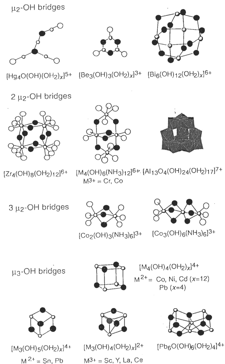
Figure 3.2 Several polycations with various modes of connection between coordination polyhedra
