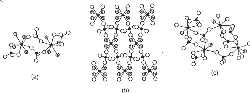
Figure 5.5 Structures of some zirconium sulfates: (a) Zr(SO_4)_2 \cdot 7H_2O ; (b) Zr(SO_4)_2 \cdot 4H_2O ; (c) Zr(SO_4)_2 \cdot H_2O
