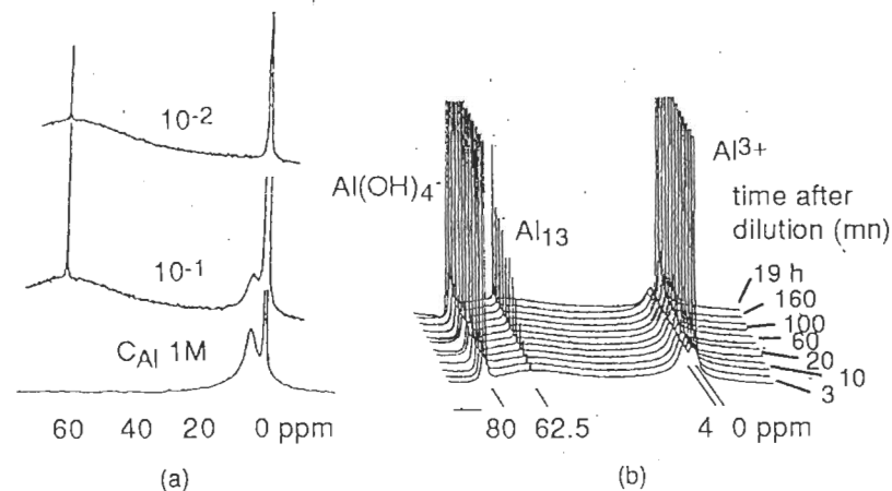
Figure 3.6 (a) ^{27}Al NMR spectra of AlCl_3 solutions hydrolyzed at h = 0.5 . The peak at around 4 ppm is due to oligomers (di-, tri- or tetramers). (b) ^{27}Al NMR spectra of a solution of AlCl_3 ( 1 \text{ mol l}^{-1} ) hydrolyzed at h = 1 and diluted 10 times rapidly with water. [Al(OH)_4]^- at 80 ppm is used as a reference. From [19] with permission
