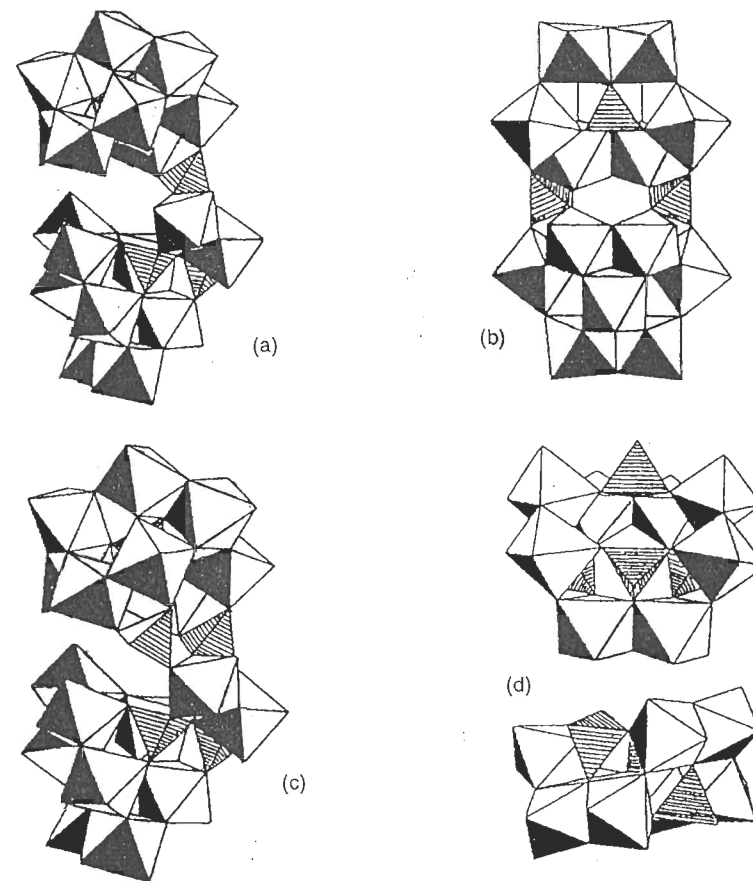
Figure 5.15 Structures of (a) [P_5W_{18}O_{75}(OH)_3]^{20-} (from [54] by permission) (b) [P_4W_{14}O_{58}]^{12-} (reprinted with permission from [55]. Copyright 1988 American Chemical Society), (c) [P_6W_{18}O_{79}]^{20-} (from [54] by permission) and (d) [P_4W_8O_{40}]^{12-} (reproduced from [56] by permission)
