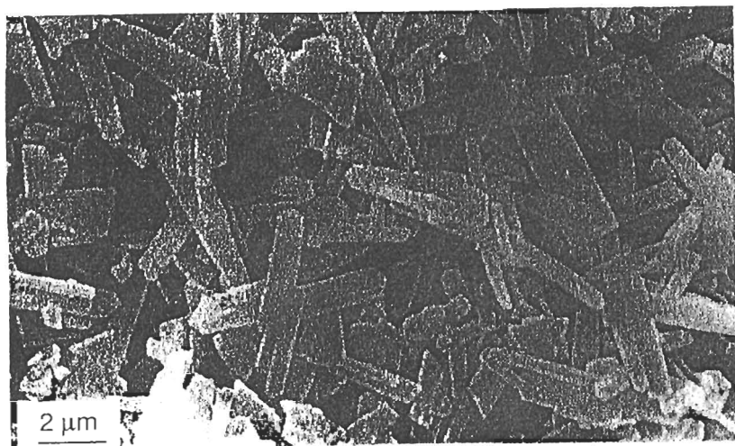
Figure 4.29 Particles of \text{MoO}_3 \cdot 1/3\text{H}_2\text{O} obtained by hydrothermal synthesis. Reproduced from [90] Copyright 1989 with permission from Elsevier Science Ltd, The Boulevard, Langford Lane, Kidlington OX5 1GB, UK
