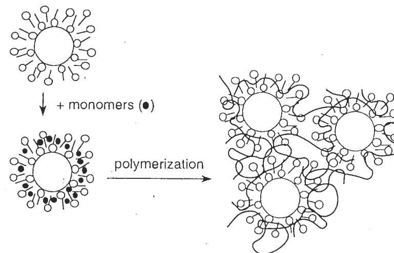
Figure 9.20 Encapsulation of oxide particles through monomer polymerization in a double layer
