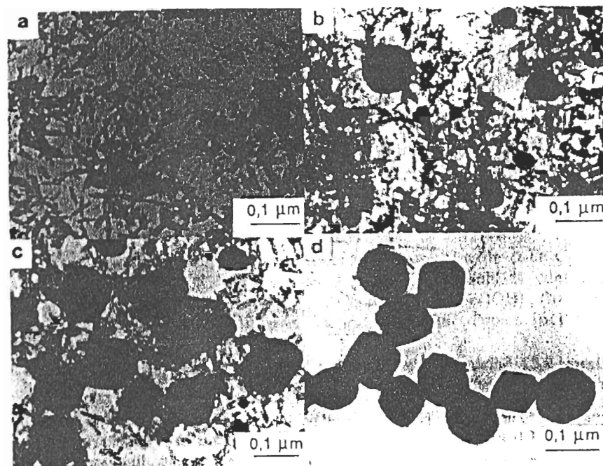
Figure 5.21 Formation steps of spherical particles of \alpha - \text{Fe}_2\text{O}_3 by the thermohydrolysis at 100^\circ\text{C} of \text{FeCl}_3 solutions ( 0.02 \text{ mol l}^{-1} ): (a) onset of turbidity ( \beta - \text{FeOOH} ); (b) after 5 h; (c) after 1 day; (d) after 2 days. Reproduced from [61] by permission
