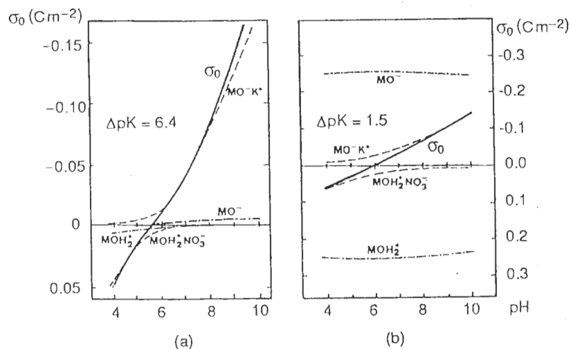
Figure 7.12 TiO_2-10^{-1} mol l^{-1} KNO_3 system. Constituents of the charge, calculated with the triple-layer model, with constants obtained by (a) graphic extrapolation ( \Delta pK = 6.4 , pK^+ = 2.6 , pK^- = 9 , pK_C = 7.1 , pK_A = 4.6 ) and (b) numerical optimization ( \Delta pK = 1.5 , pK^+ = 5.1 , pK^- = 6.6 , pK_C = 5.1 , pK_A = 6.6 ). Reproduced by permission of Academic Press from [17]
