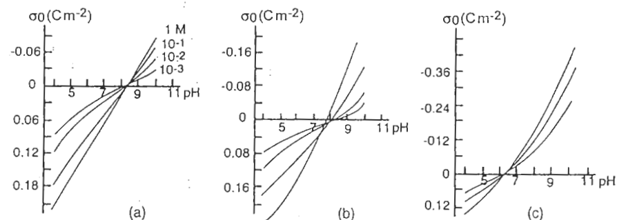
Figure 6.6 PZC for hematite, \alpha\text{-Fe}_2\text{O}_3 , as a function of the electrolyte: (a) KCl, (b) LiCl, (c) \text{Ca}(\text{NO}_3)_2 . The PZC shift is more pronounced with \text{Ca}^{2+} since it is more strongly adsorbed than \text{Li}^+ . From [19] by permission
