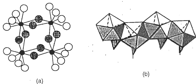
Figure 5.3 Structures of (a) \text{ZrOCl}_2 \cdot 8\text{H}_2\text{O} and (b) \text{Zr}(\text{OH})_2(\text{NO}_3)_2 \cdot 4.7\text{H}_2\text{O}
