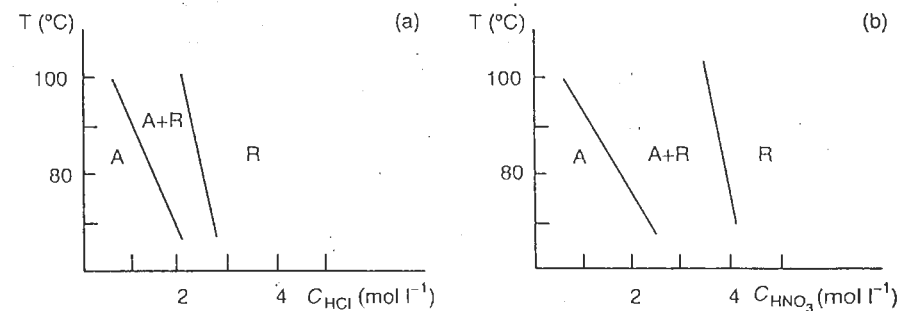
Figure 3.19 Precipitation of \text{TiO}_2 rutile R and anatase A as a function of medium acidity and temperature (a) With \text{HCl} ; (b) with \text{HNO}_3 . From [93]
