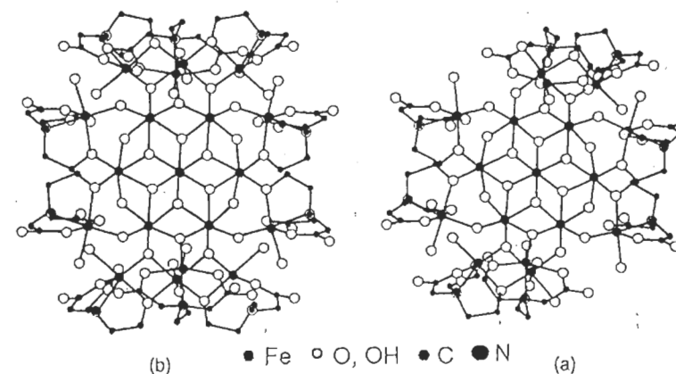
Figure 3.8 Structure of (a) [\text{Fe}_{17}(\mu_3\text{-O})_4(\mu_3\text{-OH})_6(\mu_2\text{-OH})_{10}(\text{L})_8(\text{H}_2\text{O})_{12}]^{3+} and (b) [\text{Fe}_{19}(\mu_3\text{-O})_6(\mu_3\text{-OH})_6(\mu_2\text{-OH})_8(\text{L})_{10}(\text{H}_2\text{O})_{12}]^+ , where \text{L} = \text{N}(\text{CH}_2\text{COOH})_2(\text{CH}_2\text{CH}_2\text{OH}) . From [50] with permission
