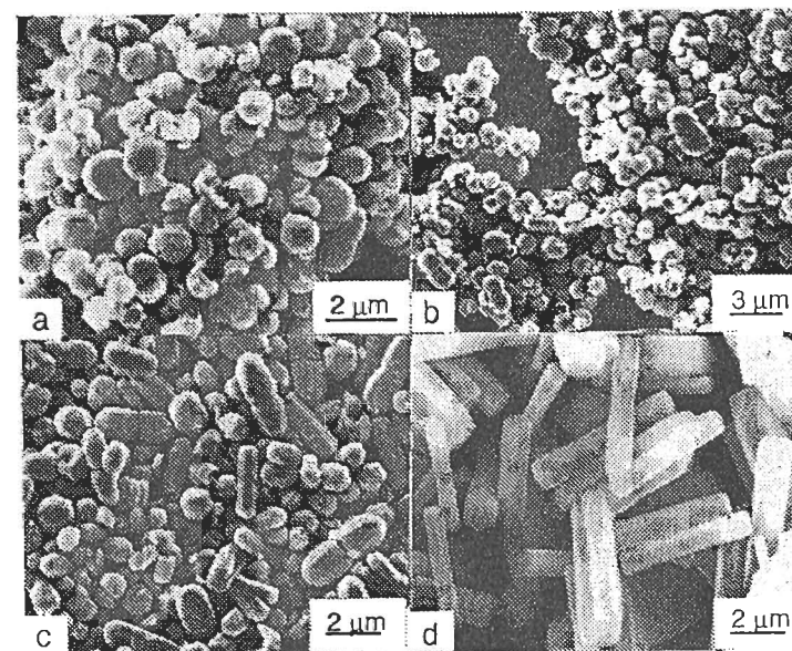
Figure 5.24 Change in the morphology of \text{ZnO} single crystals formed in a solution of \text{Zn}(\text{NO}_3)_2 ( 0.05\text{ mol l}^{-1} ) and hexamethylenetetramine ( 0.05\text{ mol l}^{-1} ) heated at 100^\circ\text{C} : (a) onset of turbidity; (b) after 3 min; (c) after 7 min; (d) after 30 min. Reproduced from [82] with permission
