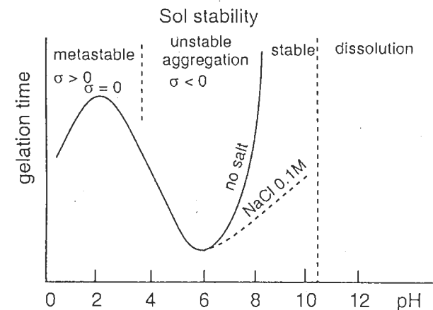
Figure 4.3 Gelation time and stability range for 'silica' sols as a function of pH. From [4] with permission
