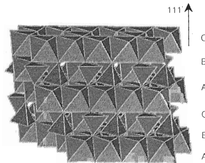
Figure 5.25 Spinel structure. A, B and C are conventional designations of the oxygen planes
