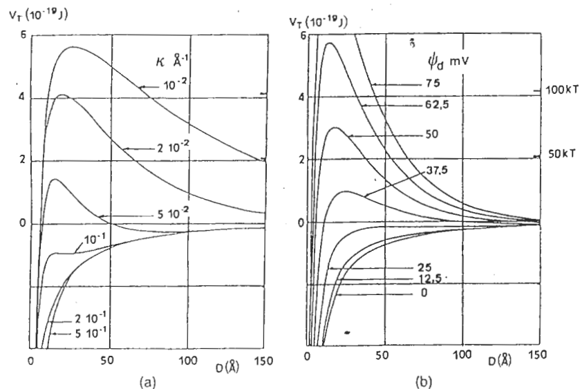
Figure 8.7 Interaction energy V_T between two spherical particles of radius a = 100 nm with T = 298 K and z = 1 as a function of (a) electrolyte concentration through the term \kappa ( \psi_d = 50 mV) and (b) potential \psi_d ( \kappa = 3 \times 10^8 m ^{-1} ). Hamaker constant 6.1 \times 10^{-20} J, \epsilon = 78.5 . V_R and V_A are calculated from equations (8.4) and (8.5). Reproduced by permission of Butterworth-Heinemann Publishers, a division of Reed Educational & Professional Publishing Ltd from [9]
