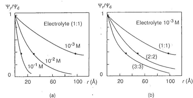
Figure 7.6 Variation in the potential in the diffuse layer, as a function of distance, calculated from the OHP (weak potential approximation). Influence of (a) electrolyte concentration (1:1) and (b) charges of ions in the electrolyte ( z : z ). Marker \bullet indicates the distance \kappa^{-1} . Data from [18]
