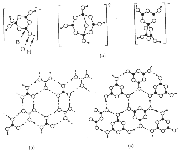
Figure 4.10 Structures of (a) polyborates, (b) boric acid and (c) metaboric acid
