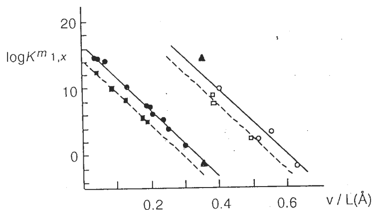
Figure 7.2 Protonation constants of hydroxo and oxo monomer complexes as a function of the bond-valence/M-H distance ratio. ● is for the protonation of neutral hydroxo complexes of metals with a rare gas configuration ( \log K_{1,2}^m ); ○ is for the protonation of oxo forms of the same elements ( \log K_{1,1}^m ). Constants \log K_{1,1}^m and \log K_{1,2}^m of d^{10} elements are denoted by ■ and □, and those of water (OH and H 2 O) are labeled ▲; L values are estimated from ionic radii. Reproduced by permission of Academic Press from [1]
