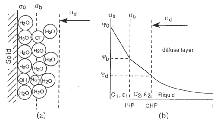
Figure 7.8 Oxide-solution interface with (a) the position of charged species on ideal planes and (b) the decrease in the potential starting from the surface. Reproduced by permission of Academic Press from [26]
