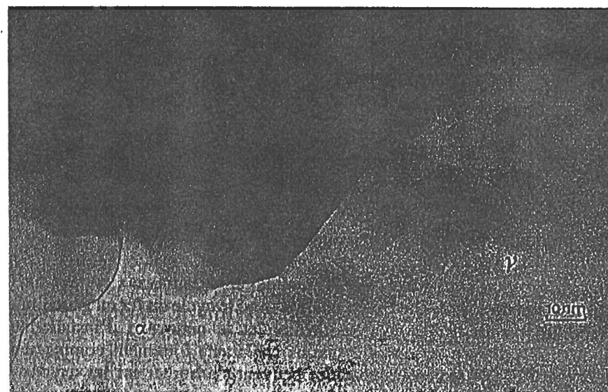
Figure 9.15 Hematite particles formed via thermal conversion of small \gamma\text{-Fe}_2\text{O}_3 particles [61]
