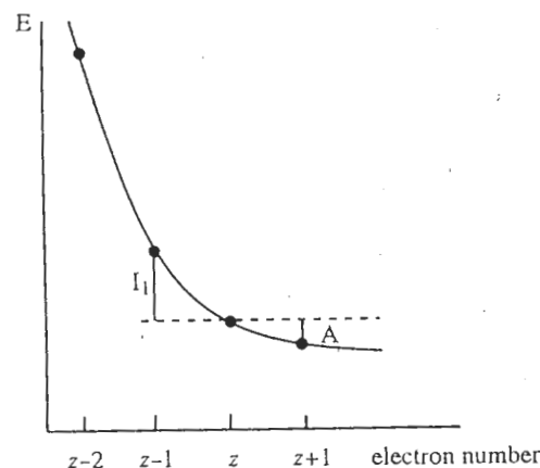
Figure A.1 Total energy of an atom (atomic number Z ) as a function of the number of electrons. From [12]
