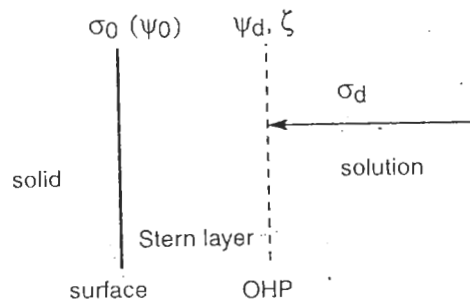
Figure 6.3 Oxide-aqueous solution interface
