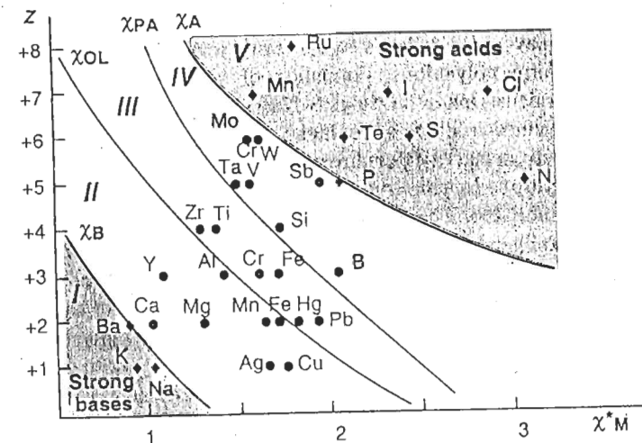
Figure 2.5 Charge-electronegativity diagram drawn using equations (A.15) to (A.18), showing five classes of behavior for the zero-charge MO_NH_{2N} form of a M^{z+} cation. In domains I and V, the element remains monomeric and soluble. Elements in domain II condense by olation only, and those in field IV by oxolation. Both condensation processes may be simultaneous for elements in field III
