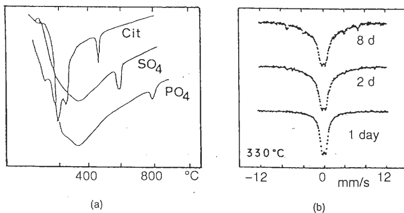
Figure 9.14 (a) Differential thermal analysis of \gamma\text{-Fe}_2\text{O}_3 particles (10 nm). The endotherm shows the \gamma \rightarrow \alpha\text{-Fe}_2\text{O}_3 transition. (b) Mössbauer spectra of \gamma\text{-Fe}_2\text{O}_3 particles heated at 330 °C for various times, after decomposition of the adsorbed citrate. The sextuplet of hematite appears at 330 °C after 8 days of heat treatment. Reproduced with kind permission from Kluwer Academic Publishers from [60a]
