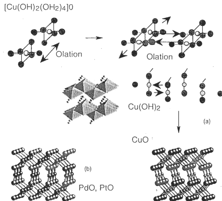
Figure 3.18 (a) Possible reaction mechanism of the formation of copper hydroxide \text{Cu}(\text{OH})_2 isostructural to boehmite. In \text{CuO}_6 octahedra highly distorted by the Jahn–Teller effect, there are four Cu–OH bonds of 1.94 Å and two of 2.63 Å. (b) Structure of \text{CuO} tenorite and of \text{PdO} and \text{PtO}
