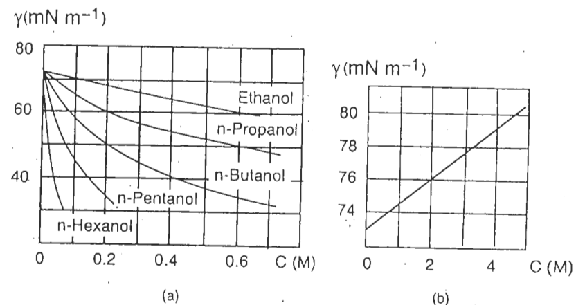
Figure 8.13 Surface energy of aqueous solutions as a function of concentration in (a) alcohol and (b) sodium chloride at 20^\circ\text{C} . Reproduced by permission of Butterworth-Heinemann Publishers, a division of Reed Educational & Professional Publishing Ltd from [9]
