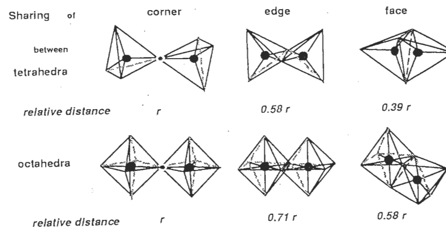
Figure 2.3 Relative distances between cations in octahedral and tetrahedral environments sharing a corner, an edge or a face
