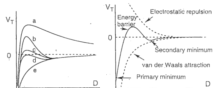
Figure 8.6 Interaction energy V_T = V_A + V_R as a function of distance: (a) the surfaces repel each other strongly; (b) the surfaces are in stable equilibrium in the secondary minimum if it is sufficiently deep; (c), (d) the surfaces in unstable equilibrium cause limited aggregation and slow flocculation of the particles; (e) the surfaces are strongly attracted to one another and the particles flocculate rapidly
