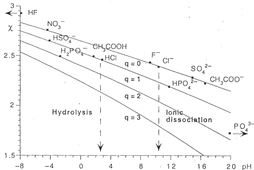
Figure A.2 Electronegativity versus pH diagram for the complexation of \text{Al}^{3+} by monodentate anions. For example, the acidity range for complexation by chloride ions is determined by the values of \chi(\text{Cl}^-) and \chi(\text{HCl})
