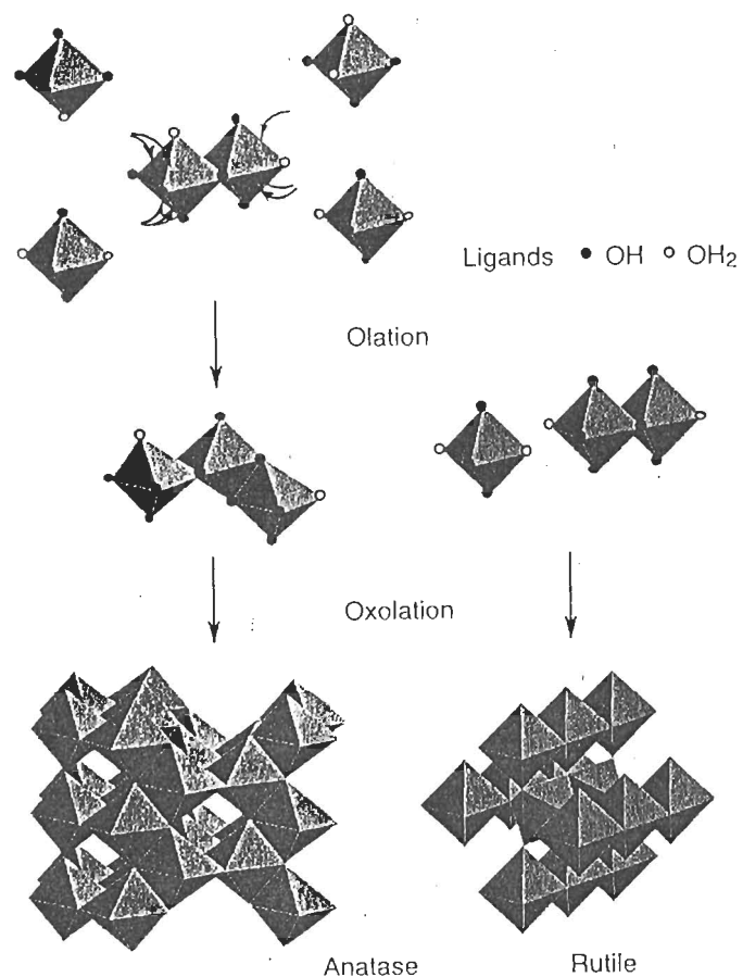
Figure 3.20 Possible formation mechanisms of TiO 2 rutile and anatase from aqueous solutions
