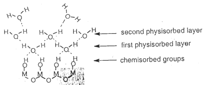
Figure 6.2 Adsorption of water on an oxide surface. From [6] by permission
