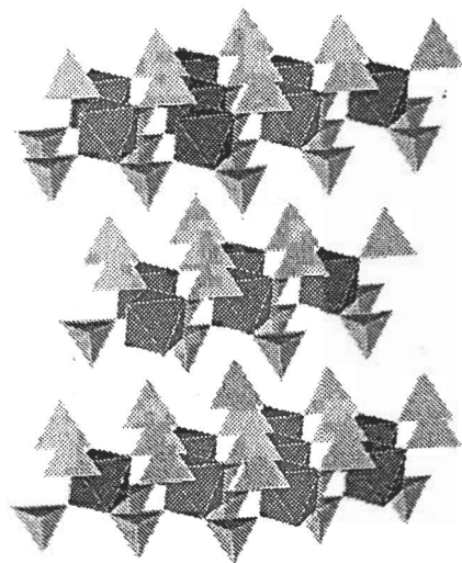
Figure 5.7 Structure of \alpha -Zr(HPO 4 ) 2 ·H 2 O
