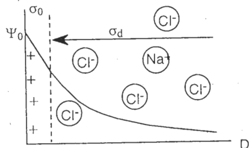
Figure 7.7 Two-layer model and the variation in the potential through the interface
