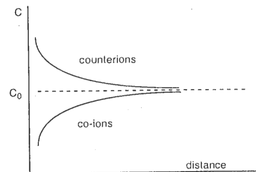
Figure 6.7 Concentration profile of the constituents to the surface countercharge near the PZC
