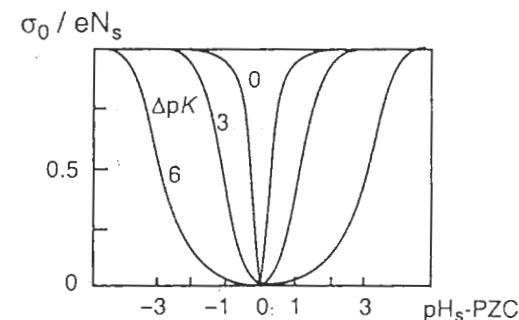
Figure 8.3 Surface charge \sigma_0 as a function of surface pH [equation (7.23)] for various values of \Delta\text{pK} . Reproduced from [5] by permission
