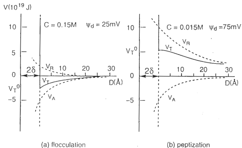
Figure 8.9 Total interaction energy V_T for (a) flocculation and (b) peptization. Thickness of the Stern layer d = 2 \text{ \AA} ; radius of the particles a = 500 \text{ \AA} ; effective Hamaker constant A = 5 \times 10^{-20} \text{ J} ; the concentration c of a [1 : 1] electrolyte and the diffuse layer potential \psi_d are shown on the figure. Reproduced by permission of Academic Press from [23]
