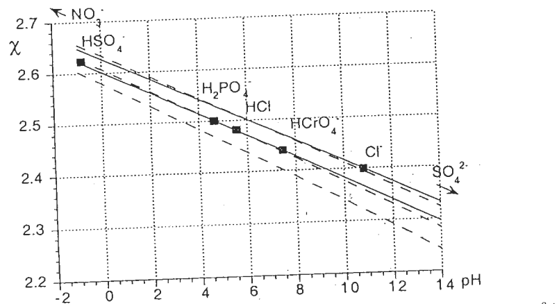
Figure 5.2 Electronegativity-pH diagram for the complexation of [\text{Zr}_4(\text{OH})_8(\text{OH}_2)_{16}]^{8+} by monodentate anions (solid lines) or bidentate anions (dotted lines)
