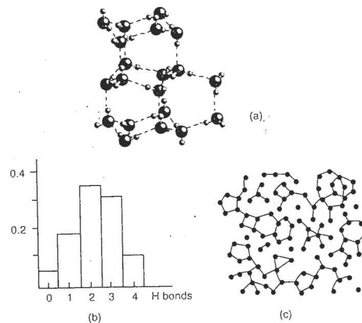
Figure 1.2 (a) Structure of hexagonal ice (bond length O \cdots H \cdots O 2.76 \text{ \AA} , O-H 1 \text{ \AA} , O \cdots H 1.75 \text{ \AA} , angles H-O-H 109.5^\circ [4]), (b) fraction of the molecules involved in various numbers of H bonds in liquid water at 10^\circ C [5] and (c) hydrogen bond network in liquid water (molecules are shown as points). Reprinted with permission from [5]. Copyright 1973 American Chemical Society
