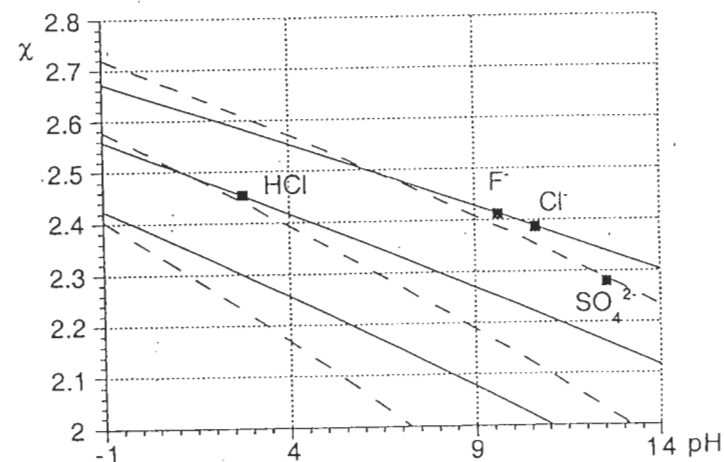
Figure 5.18 Electronegativity–pH diagram for the complexation of \text{Ti(IV)}
