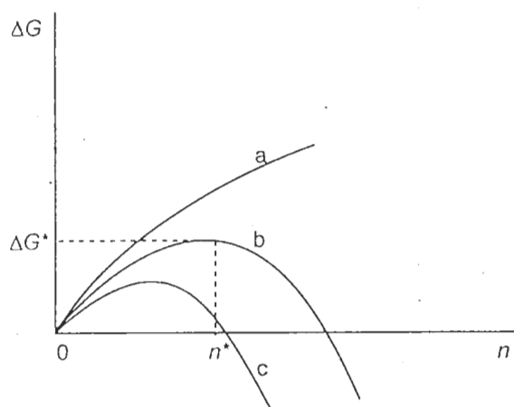
Figure 2.8 Variation in the free enthalpy of formation of nuclei as a function of the number of precursor molecules n associated in the nucleus. Curve a for a solution that is not supersaturated ( S < 1 ); curves b and c are for a supersaturated solution, with S_c > S_b > 1
