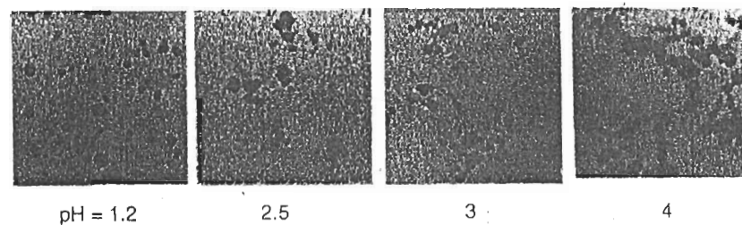
Figure 8.8 TEM micrographs showing the aggregation of iron oxide particles ( \gamma\text{-Fe}_2\text{O}_3 , average diameter 90 Å, \text{PZC} = 8 ) in a cationic sol at various pH. Polyvinyl alcohol introduced in the sol prior to drying allows the preservation of the dispersion on the grid [22]
