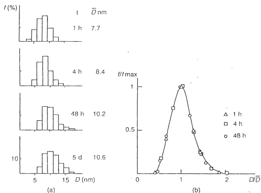
Figure 2.11 (a) Particle size distribution of \text{Fe}_3\text{O}_4 magnetite during aging and (b) Size distribution normalized for various times. From [39]
