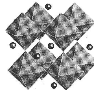
Figure 5.27 Perovskite structure \text{ABO}_3
