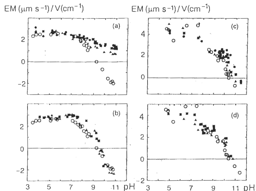
Figure 9.5 Electrophoretic mobility (EM) of goethite particles ( 20 \text{ m}^2/\text{l} ) adsorbed at various concentrations (solid markers): (a) Mg(II), (b) Mn(II); boehmite ( 20 \text{ m}^2/\text{l} ) having adsorbed (c) Mg(II) and (d) Mn(II). Open markers indicate the electrophoretic mobility of both solids measured in the presence of \text{NaClO}_4 . Reproduced by permission of Academic Press from [23]
