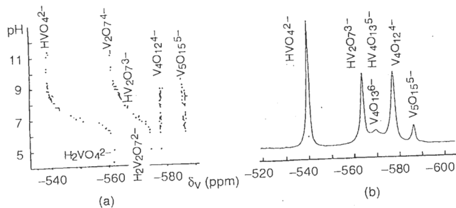
Figure 4.14 (a) ^{51}V NMR chemical shifts of the main vanadium species as a function of pH and (b) ^{51}V NMR spectrum of a solution at pH 8.3 ( C_V = 10^{-2} \text{ mol l}^{-1} ). Reproduced from [54] with permission
