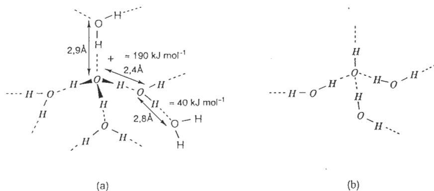
Figure 1.3 Probable structure of hydrated ions: (a) [\text{H}_9\text{O}_4]^+ ; (b) [\text{H}_7\text{O}_4]^- . From [14]
