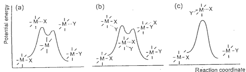
Figure 2.1 Reaction paths for nucleophilic substitution reactions: (a) dissociative; (b) associative; (c) direct displacement
