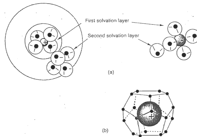
Figure 1.4 Hydration schemes (a) of hydrophilic cations and anions in aqueous solution and (b) of hydrophobic cations
