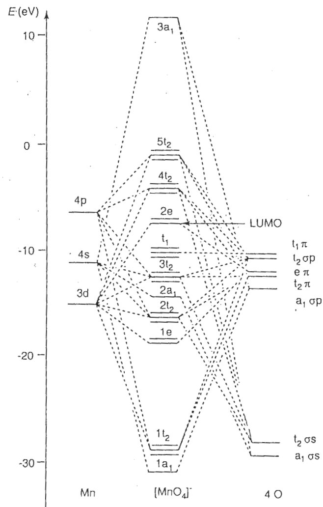
Figure 4.11 Molecular orbital diagram for [\text{MnO}_4]^- . From [49]
