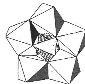
Figure 5.11 Structure of the [P 2 W 5 O 23 ] 6- anion. Reproduced with permission from [42]. Copyright 1981 American Chemical Society
