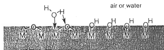
Figure 6.1 Water chemisorption on an oxide surface
