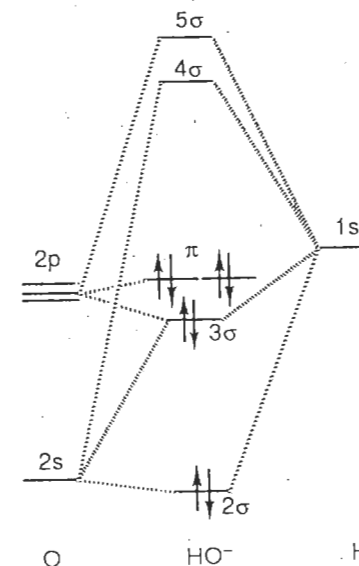
Figure 2.2 Molecular orbital diagram for the \text{HO}^- ion
