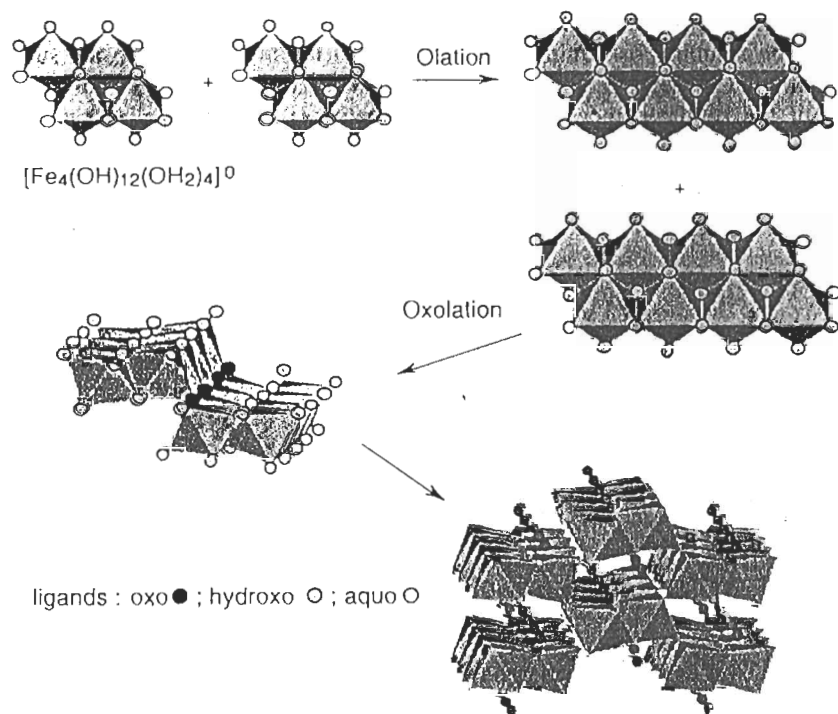
Figure 3.12 Possible formation mechanism of goethite \alpha -FeOOH in solution, via ageing or thermohydrolysis
