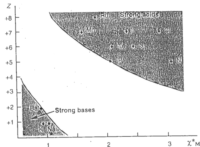
Figure 1.7 Charge–electronegativity diagram obtained from (A.19) and (A.20), showing the strong acidic or basic behavior of elements
