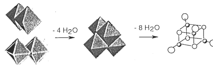
Figure 3.17 Tetrameric polycations formed by [\text{M}_2(\text{OH})_2(\text{OH}_2)_8]^{2+} dimers
