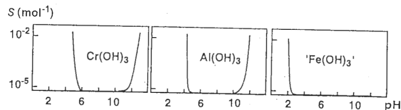
Figure 3.3 Precipitation of Cr(III), Al(III) and Fe(III). From [29a]
