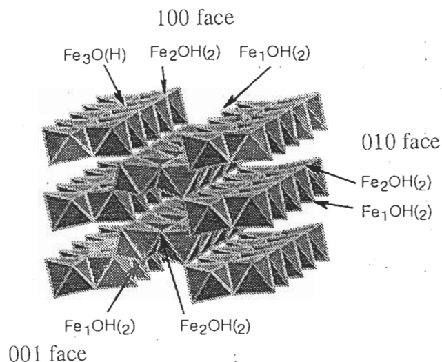
Figure 7.4 Crystal of goethite showing the surface structure of faces 100, 001 and 010
