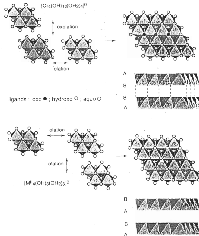
Figure 3.16 Possible reaction mechanism for the formation of chromium oxyhydroxide \alpha -CrOOH and hydroxides M(OH)_2 of brucite structure
