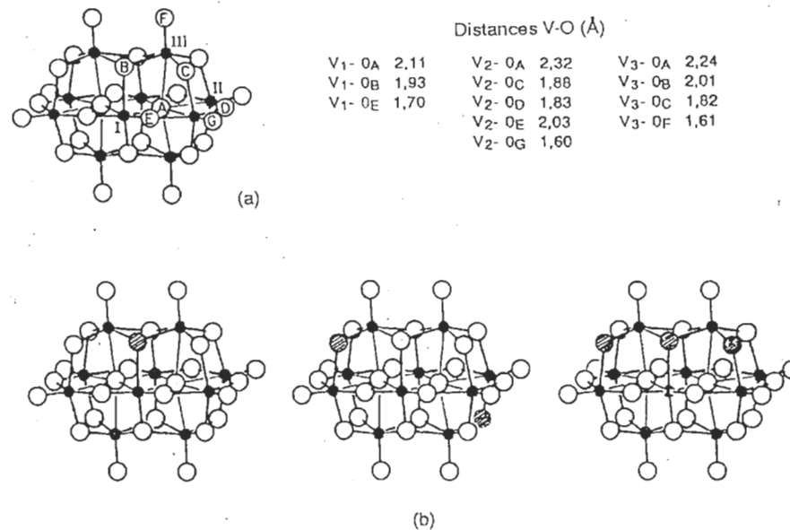
Figure 4.15 (a) Structure of the [V_{10}O_{28}]^{6-} ion and bond lengths and (b) protonation sites for [HV_{10}O_{28}]^{5-} and [H_2V_{10}O_{28}]^{4-} in water and for [H_3V_{10}O_{28}]^{3-} in H_2O/CH_3CN . Reprinted with permission from [56]. Copyright 1987 American Chemical Society
