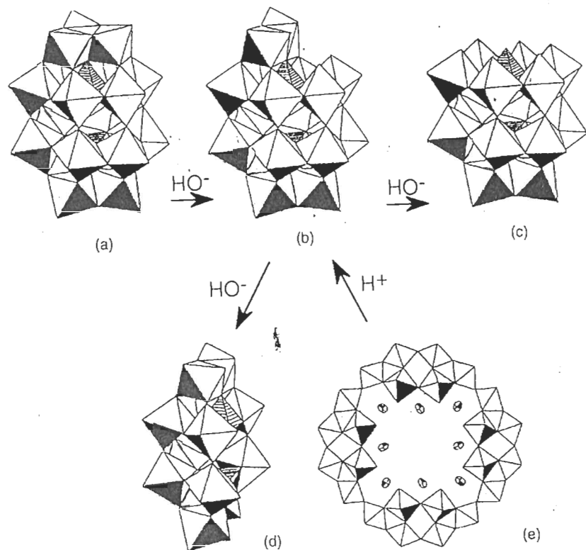
Figure 5.12 Structures of (a) \alpha -[P 2 W 18 O 62 ] 6- (Dawson's structure) and of the vacancy compounds (b) \alpha -[P 2 W 17 O 61 ] 10- , (c) \alpha -[P 2 W 15 O 56 ] 12- , (d) [H 2 P 2 W 12 O 48 ] 12- and (e) [P 8 W 48 O 184 ] 40- (potassium ions within the crown are shown as ellipsoids). Reprinted with permission from [47]. Copyright 1985 American Chemical Society
