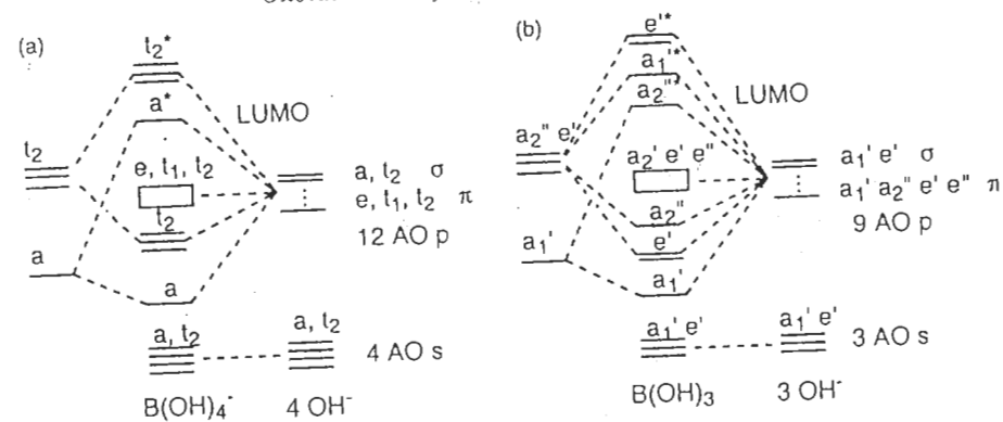
Figure 4.8 MO diagram for (a) [\text{B}(\text{OH})_4]^- and (b) \text{B}(\text{OH})_3 . The diagrams are drawn by analogy with the diagrams of \text{BX}_4^- and \text{BX}_3 respectively. From [41].
