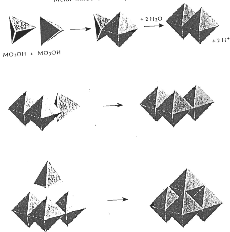
Figure 4.12 Tetrahedra addition with formation of chains and rings
