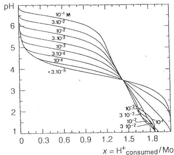
Figure 4.22 Protometric titration of [\text{MoO}_4]^{2-} for different molybdenum concentrations. Reproduced by permission of John Wiley & Sons from [2]
