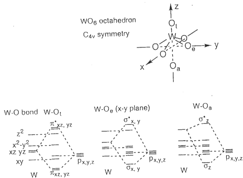
Figure 4.25 Simplified molecular orbital diagram for a C_{4v} WO_6 complex in a tungstic polyanion
