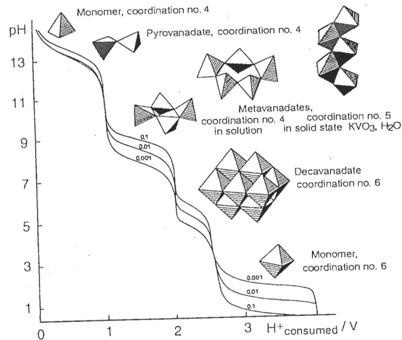
Figure 4.13 Titration curves of vanadate solutions for various vanadium concentrations. Reproduced by permission of John Wiley & Sons from [2]
