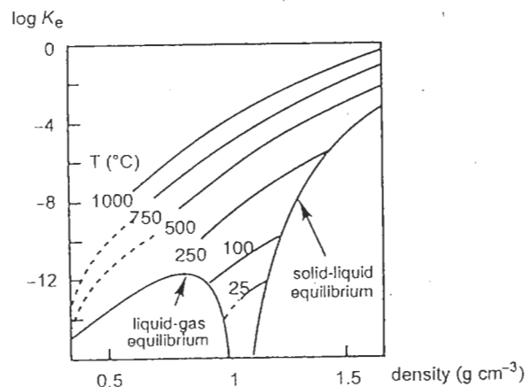
Figure 1.9 Ionic product of water as a function of temperature and density of the liquid. Reproduced with permission from [42]
