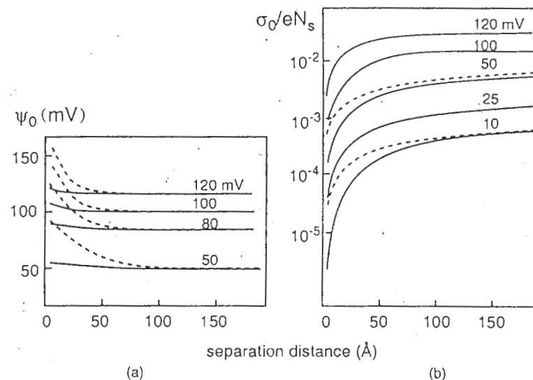
Figure 8.2 Variation in the potential \psi_0 (a) and in the charge \sigma_0 (b) as a function of the distance between two surfaces of \text{PZC} = 7 and \Delta\text{pK} = 3 (solid lines) and 6 (dotted lines). Electrolyte concentration 10^{-3} \text{ mol l}^{-1} ( \kappa^{-1} = 96 \text{ \AA} ). The potentials are given for an infinite separation distance. Reproduced from [5] by permission
