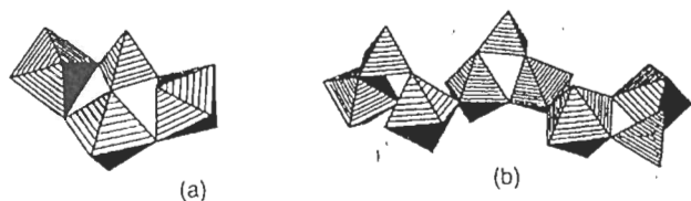
Figure 5.8 Configurations of phosphoantimonic anions: (a) [\text{Sb}_3(\text{OH})_{11}\text{O}_2(\text{PO}_4)]^{3-} formed at \text{pH} > 7 ; (b) [\text{Sb}_6(\text{OH})_{20}\text{O}_5(\text{PO}_4\text{H})_3]^{6-} formed at \text{pH} < 4 . From [30] and [31]
