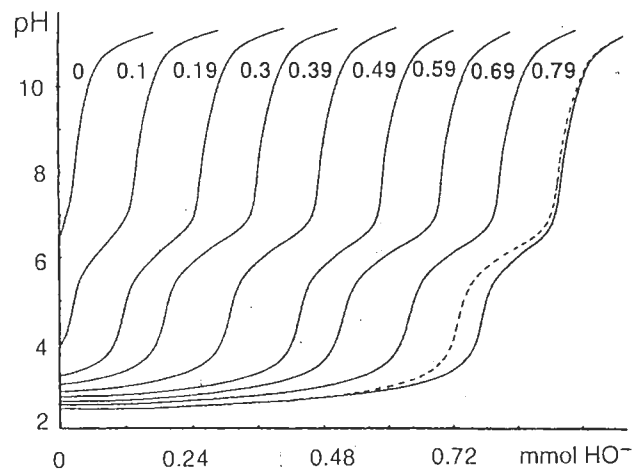
Figure 9.6 Titration of \text{Fe}_3\text{O}_4 + \text{HClO}_4 by \text{N}(\text{CH}_3)_4\text{OH} . The ratios [\text{H}^+]_{\text{added}}/\text{Fe(II)}_{\text{initial}} are indicated on the curves. Titrations are carried out 5 min after acidification. Dashed line: titration 45 min after acidification. Reproduced by permission of Academic Press from [35]
