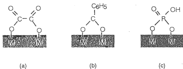
Figure 9.11 Coordination (a) of oxalate, (b) of benzoate and (c) of phosphate on the surface of oxides or hydroxides
