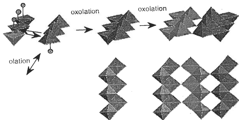
Figure 4.17 Possible formation mechanism of a V_2O_5 \cdot nH_2O gel from the neutral precursor VO(OH)_3(OH_2)_2
