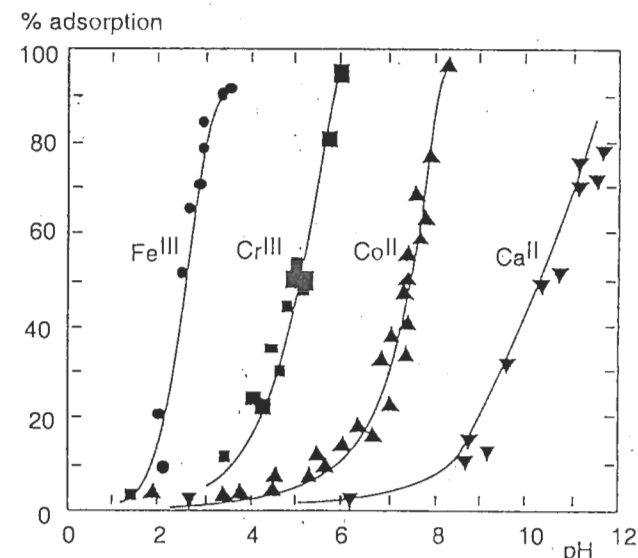
Figure 9.1 Adsorption isotherms at 25 °C for Fe(III) ( 1.2 \times 10^{-4} M), Cr(III) ( 2 \times 10^{-4} M), Co(II) ( 1.2 \times 10^{-4} M) and Ca(II) ( 1.4 \times 10^{-4} M) on \text{SiO}_2 as a function of pH. Reproduced by permission of Academic Press from [11]
