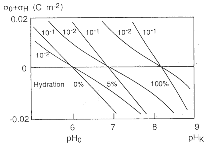
Figure 7.17 Relationship between the IEP and the hydration of an oxide surface. The system constants are those listed in Figure 7.16 using values of 0, 0.1 and 0.2 \text{ C m}^{-2} for \sigma_T . The ionic strength is indicated on the figure. Reproduced by permission of John Wiley & Sons from [25]
