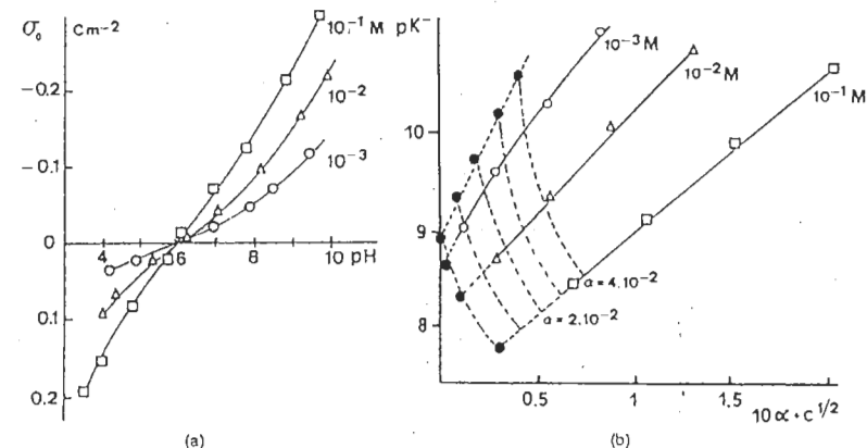
Figure 7.10 (a) Variation in the surface charge of \text{TiO}_2 anatase with NaCl concentration and (b) determination via double extrapolation of the affinity ratio \text{pK}^- . Extrapolations are the dashed lines and filled markers. Reproduced by permission of Academic Press from [28]
