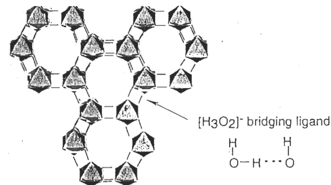
Figure 3.13 Planes of chromium hydroxide Cr(OH)_3(OH_2)_3 . [Cr(OH)_3(OH_2)_3] octahedra are connected by the bridging ligand [H_3O_2]^-
