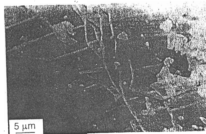
Figure 4.26 SEM micrograph of a tungstic gel of WO_3 \cdot H_2O formed by acidification of sodium tungstate on a resin. From [92]
