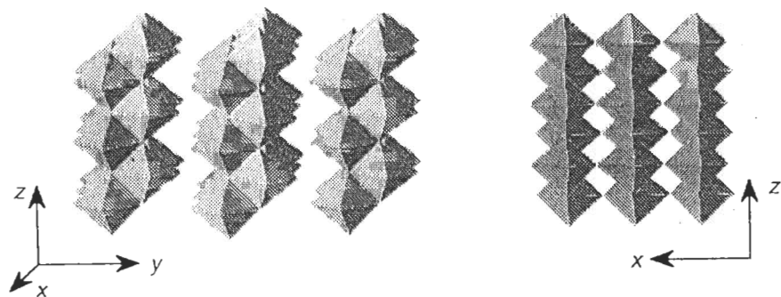
Figure 4.30 Structure of orthorhombic \text{MoO}_3
