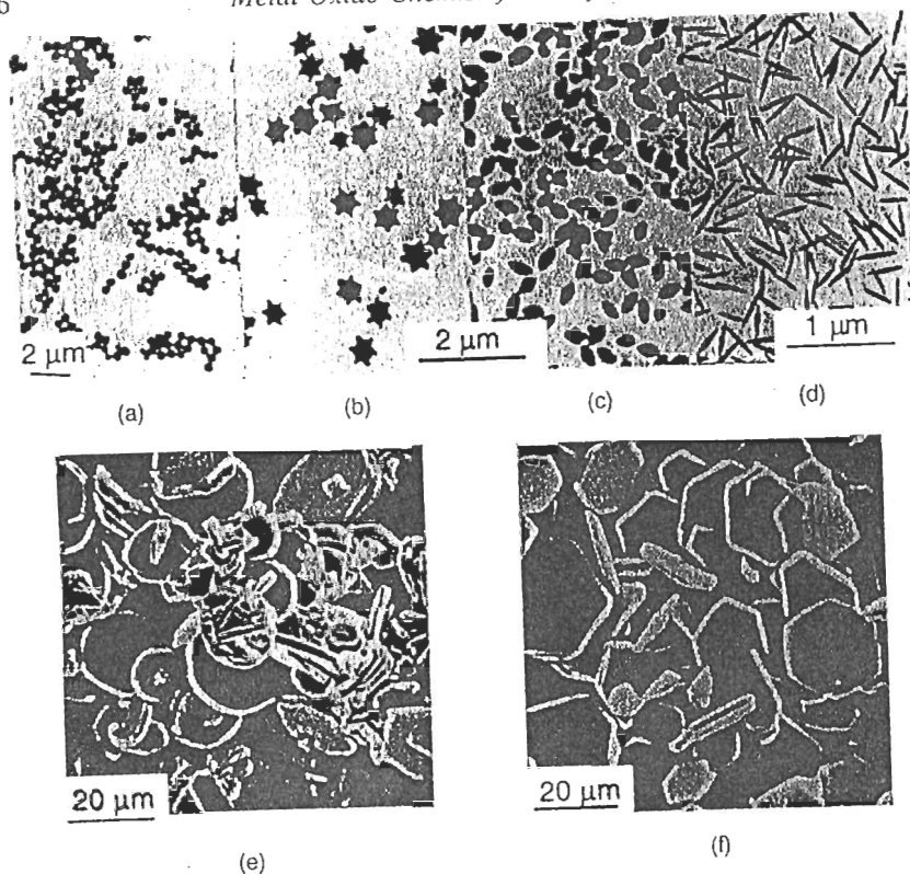
Figure 5.20 \alpha - \text{Fe}_2\text{O}_3 particles formed by the thermohydrolysis of acidic solutions of \text{Fe(III)} ( 100^\circ\text{C} , pH 0.5–2.5) in the presence of ions (a) \text{Cl}^- , (b) \text{ClO}_4^- , (c) \text{NO}_3^- and (d) \text{H}_2\text{PO}_4^- , and by the thermohydrolysis of alkaline solutions of \text{Fe(III)} –triethanolamine chelates ( 250^\circ\text{C} , \text{NaOH } 1.2 \text{ mol l}^{-1} ) in media (e) \text{ClO}_4^- and \text{H}_2\text{O}_2 and (f) \text{NO}_3^- and \text{CH}_3\text{COO}^- . Reproduced by permission of E. Matijevic
