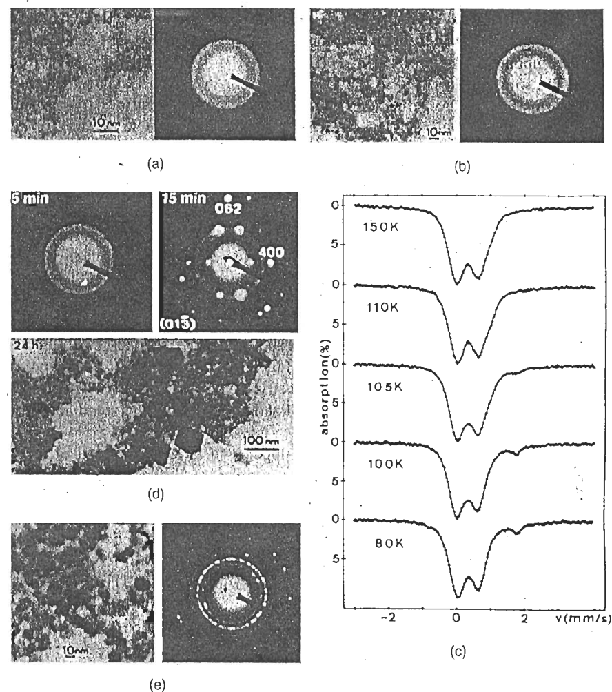
Figure 3.23 Micrographs and electron diffraction patterns of suspensions x = \text{Fe(II)/Fe(III)} for various reaction times (a) x = 0 , t = 5 min (ferric ferrihydrite); (b) x = 0.15 , t = 1 min; (c) Mössbauer spectra at various temperatures for x = 0.15 and t = 1 min; (d) x = 0.15 , t = 5 min, t = 15 min, t = 24 h; (e) x = 0.5 , t = 1 min. Reprinted with permission from [106]. Copyright 1992 American Chemical Society
