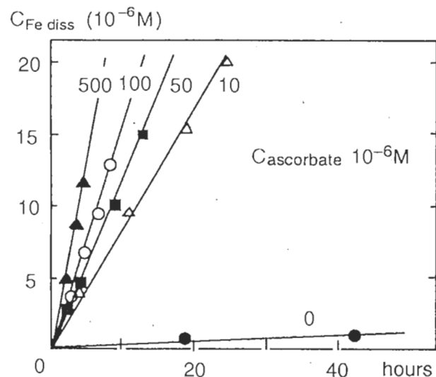
Figure 9.16 Dissolution of hematite in the presence of ascorbate at pH 3. In the absence of ascorbate, Fe(III) concentration. Reprinted with permission from [67]. Copyright American Chemical Society
