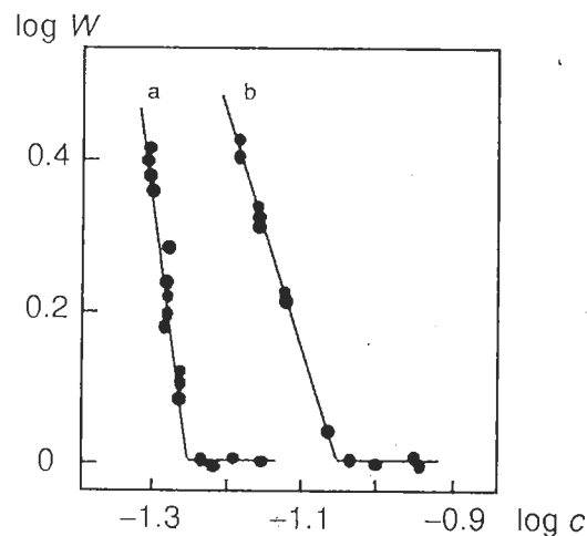
Figure 8.10 Influence of the electrolyte concentration on the flocculation rate of hematite particles ( \alpha - \text{Fe}_2\text{O}_3 ) of average diameter 47.5 nm and \text{PZC}=8.2 (a) at pH 11.8 with counterions \text{K}^+ and (b) at pH 4 with counterions \text{ClO}_4^- . Reproduced from [28] by permission
