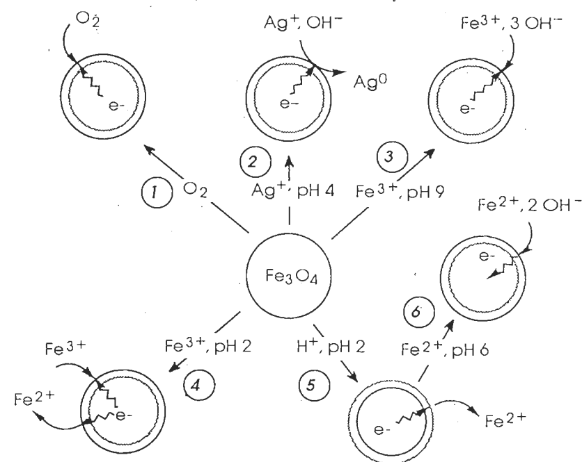
Figure 9.10 \text{Fe}_3\text{O}_4 \rightarrow \gamma\text{-Fe}_2\text{O}_3 transformations induced by adsorption of various species. Dashed circles represent the initial size of the colloid in each transformation. In each case, adsorption is assisted by outward electron transfers within the particle, which renew the reactive chemical species on the surface ( \text{Fe}^{2+} ions). The surface may be oxidized in situ (steps 1 to 3) or desorbed (steps 4 and 5) depending on the physicochemical characteristics of the medium. In all steps, electron transfers are associated with migration of \text{Fe}^{3+} from the octahedral sublattice towards the surface of the particle, causing formation of cation vacancies. Step 5 is apparently reversible. Adsorption of \text{Fe}^{2+} and \text{HO}^- (step 6) is also assisted by electronic and ionic ( \text{H}^+ ) inward transfers, but without appreciable Fe migration. This results in the epitaxial growth of an \text{Fe}_3\text{O}_4 layer
