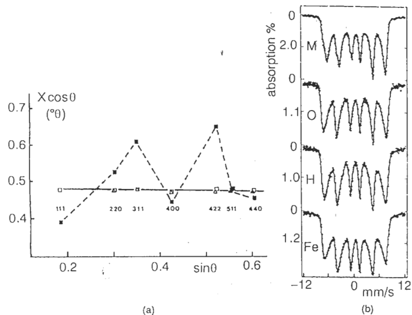
Figure 9.7 (a) Variation in the width L of XRD peaks and (b) Mössbauer spectra (300 K) of freshly prepared colloidal magnetite (average particle diameter 8 nm): \Delta , M; treated with \text{HClO}_4 : \square , H; treated with \text{Fe}(\text{NO}_3)_3 : \blacksquare , Fe; and oxidized in air: \circ , (diffraction data for particles oxidized in air and treated in an acidic medium are indistinguishable). Reproduced by permission of Academic Press from [35]
