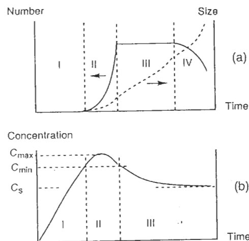
Figure 2.6 Change (a) in the number and sizes of particles formed in solution and (b) in the concentration C of the soluble precursor of the solid phase [23] during precipitation. The condensation rate, which is zero for C < C_{min} , becomes infinite for C \geq C_{max} . C_s is the solubility of the solid phase
