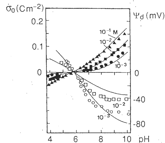
Figure 7.9 Surface charge and diffuse layer potential for \text{TiO}_2 as a function of pH and for several electrolyte concentrations. The continuous lines are derived from the model. Reproduced by permission of Academic Press from [26]
