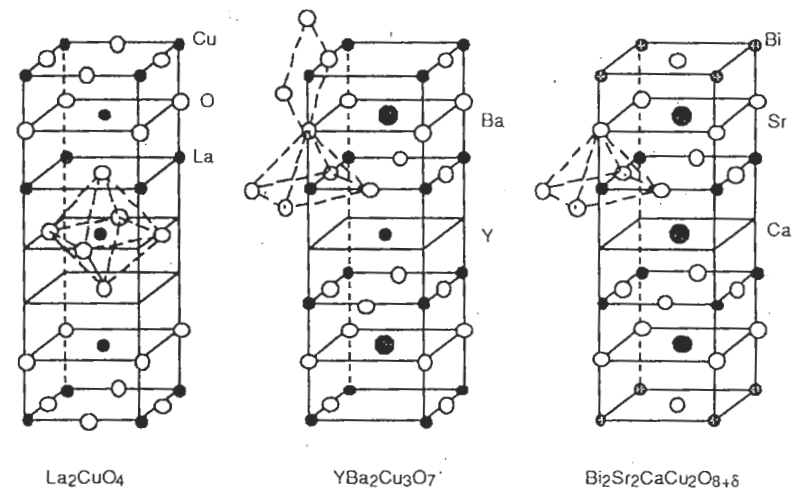
Figure 5.28 Structures of three copper-based superconductors
