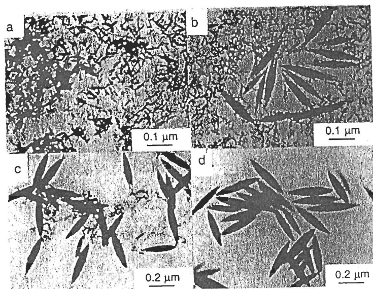
Figure 5.23 1 Formation steps of ellipsoidal particles of \alpha\text{-Fe}_2\text{O}_3 by the thermohydrolysis at 100^\circ\text{C} of \text{FeCl}_3 solutions ( 0.02\text{ mol l}^{-1} ) containing \text{KH}_2\text{PO}_4 ( 4.5 \times 10^{-4}\text{ mol l}^{-1} ): (a) onset of turbidity ( \beta\text{-FeOOH} ); (b) after 2 days; (c) after 4 days; (d) after 6 days. From [61] by permission
