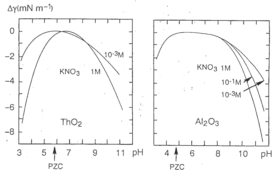
Figure 8.14 Surface energy as a function of pH, calculated from \sigma = f(\text{pH}) curves, for \text{ThO}_2 and \text{Al}_2\text{O}_3 at various ionic strengths. Reprinted with permission of from [40]. Copyright 1969 American Chemical Society
