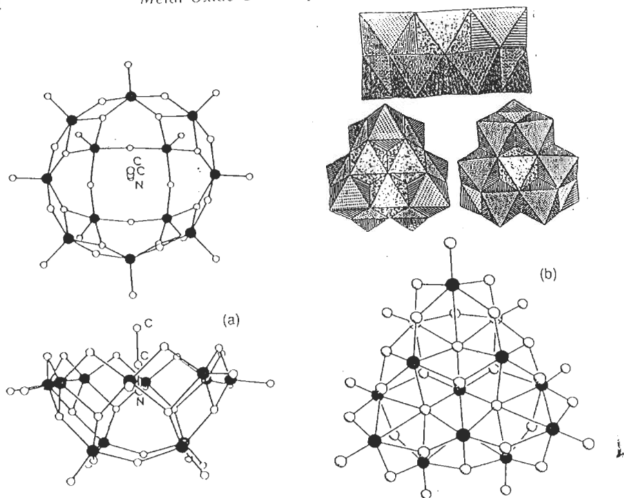
Figure 4.18 (a) Structure of [V_{12}O_{32}]^{4-} (the vanadium atoms are shown as filled circles). Reprinted with permission from [66]. Copyright 1989 American Chemical Society from [66]. (b) Structure of [V_{13}O_{34}]^{3-} . Reprinted with permission from [67]. Copyright 1992 American Chemical Society from [67]
