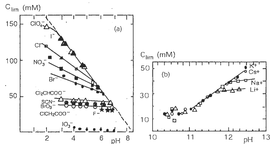
Figure 8.11 Critical flocculation concentrations for hematite particles as a function of pH for anions (a) and cations (b). Reproduced from [28] by permission
