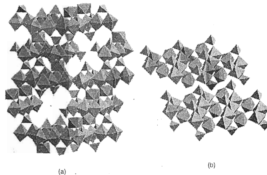
Figure 5.9 Structure of (a) \text{K}_5\text{Sb}_5\text{O}_{12}(\text{PO}_4)_2 and (b) \text{K}_3\text{Sb}_3\text{O}_6(\text{PO}_4)_2 from data in [34] and [36]
