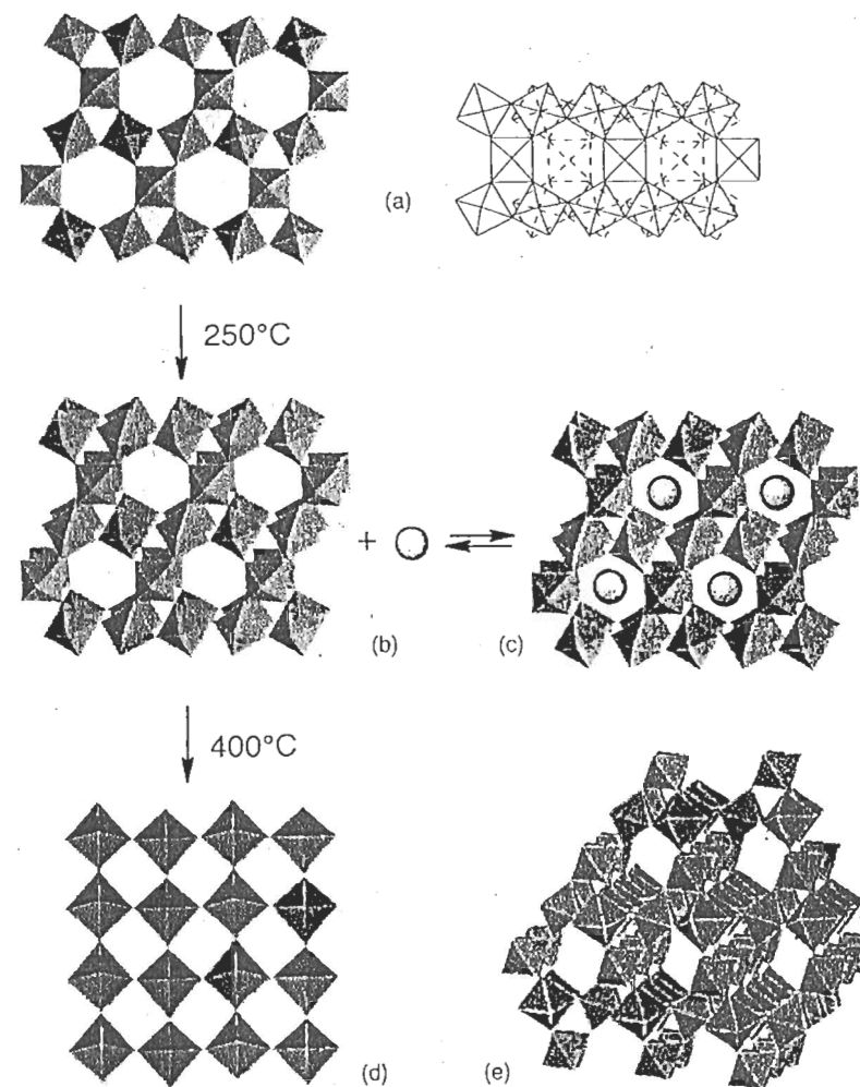
Figure 4.28 Structures of tungstic hydrates and oxides: (a) \text{WO}_3 \cdot 1/3\text{H}_2\text{O} (001) plane and connection between 001 planes; (b) hexagonal \text{WO}_3 with one-dimensional channels along the c axis; (c) hexagonal bronze \text{M}_x\text{WO}_3 ; (d) monoclinic \text{WO}_3 ; (e) pyrochlore \text{WO}_3 (111 planes)
