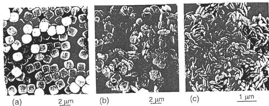
Figure 2.13 Hematite particles obtained by addition of sodium hydroxide to an \text{FeCl}_3 solution (final Fe concentration 1 \text{ mol l}^{-1} ): (a) pseudocubic particles obtained after heat treatment at 100^\circ\text{C} for 8 days of a suspension of (\text{OH}^-/\text{Fe} = 5.4) ; (b) platelets obtained after heat treatment at 180^\circ\text{C} for 2 h of a suspension of (\text{OH}^-/\text{Fe} = 8) ; (c) spindle-shaped particles obtained by heat treatment at 100^\circ\text{C} for 2 days of a solution of 2 \times 10^{-2} \text{ mol l}^{-1} in \text{FeCl}_3 and 3 \times 10^{-4} \text{ mol l}^{-1} in \text{NaH}_2\text{PO}_4 . Reproduced by permission of Academic Press from [50]
