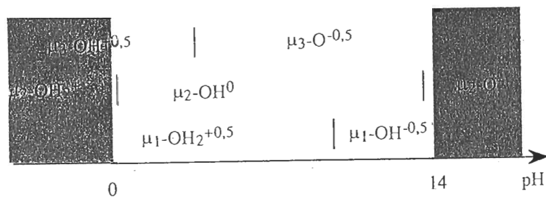
Figure 7.5 Protonation range of various groups on the surface of goethite
