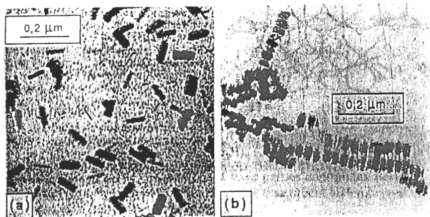
Figure 3.7 (a) Sol ( \text{Fe}^{3+} 6.25 \times 10^{-3} \text{ mol l}^{-1} ) after 1 year of ageing ( \text{pH} = 1.95 ), containing 20–40 Å colloids and goethite particles. (b) In a more concentrated medium ( \text{Fe}^{3+} 6 \times 10^{-2} \text{ mol l}^{-1} , \text{pH} = 1.50 ), the particles aggregate as tactoids. Reproduced by permission of Elsevier Science Ltd from [49]
