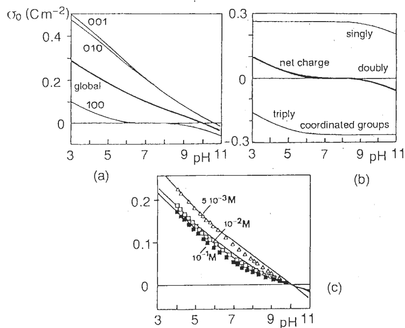
Figure 7.14 (a) \sigma_0 = f(\text{pH}) curves calculated for the 001, 010 and 100 faces of goethite ( \text{NaNO}_3 0.1 \text{ mol l}^{-1} , Stern layer capacitance 1.54 \text{ F m}^{-2} , \text{p}K_C = \text{p}K_A = 0.75 , specific surface area of the three types of face 5, 45 and 50 \text{ m}^2/\text{g} respectively). (b) Calculated contributions of several types of site to the charge of 100 faces with the same parameters as for (a). (c) Global \sigma_0 = f(\text{pH}) curve for various \text{NaNO}_3 concentrations. The calculated curves are shown in solid lines, experimental data points are shown using markers. Reproduced by permission of Academic Press from [2]
