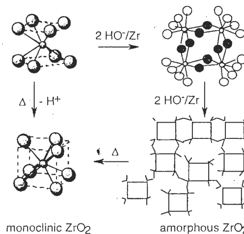
Figure 3.22 Formation of solid phases of zirconium oxides from solution, with the corresponding coordination polyhedra
