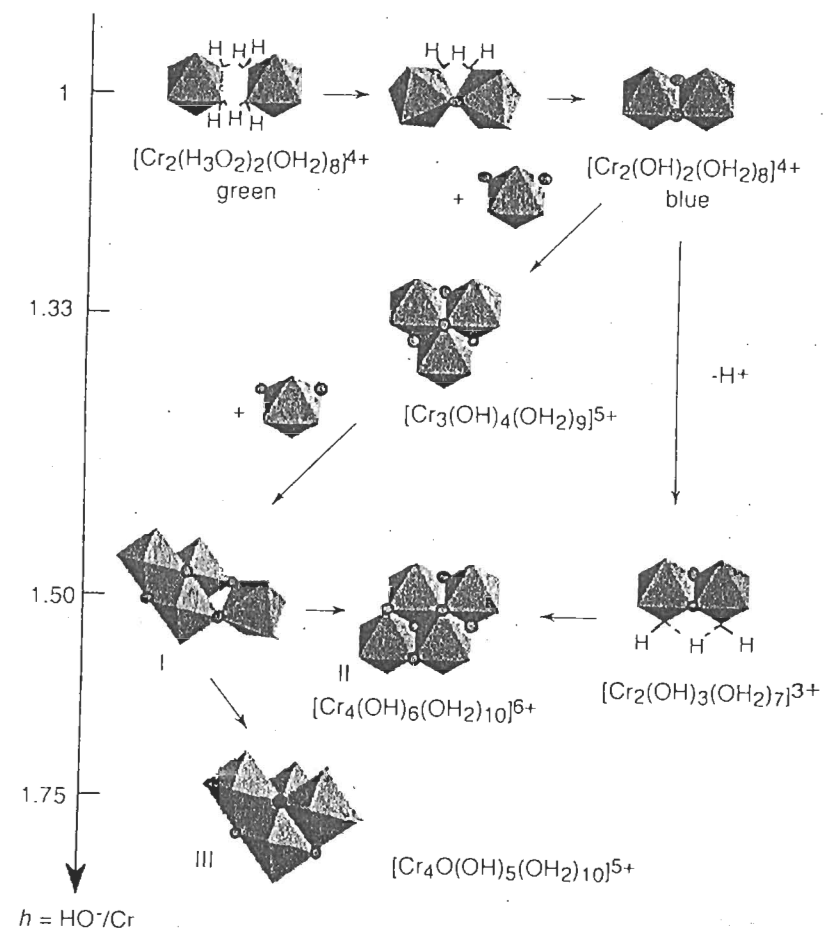
Figure 3.4 \text{Cr}(\text{III}) polycations in aqueous solution
