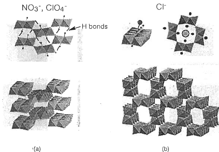
Figure 5.16 Structures of (a) goethite \alpha -FeOOH and (b) akaganeite \beta -FeOOH
