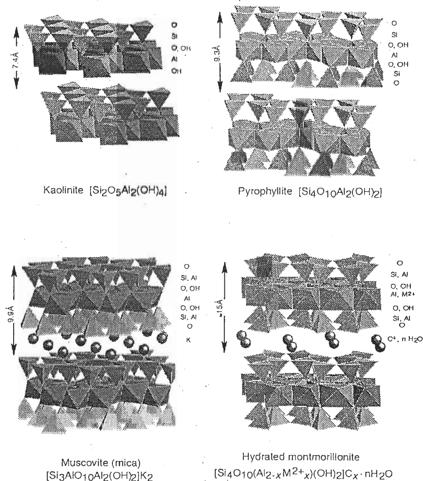
Figure 4.4 Structures of a few clays
