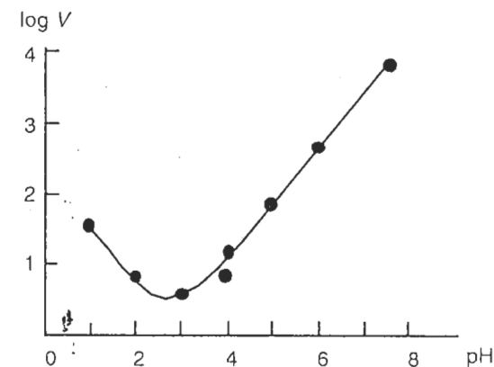
Figure 4.2 Rate of disappearance of the monomer at various pH (Si concentration 6 g/l in \text{SiO}_2 , temperature 20^\circ\text{C} ). From [21]
