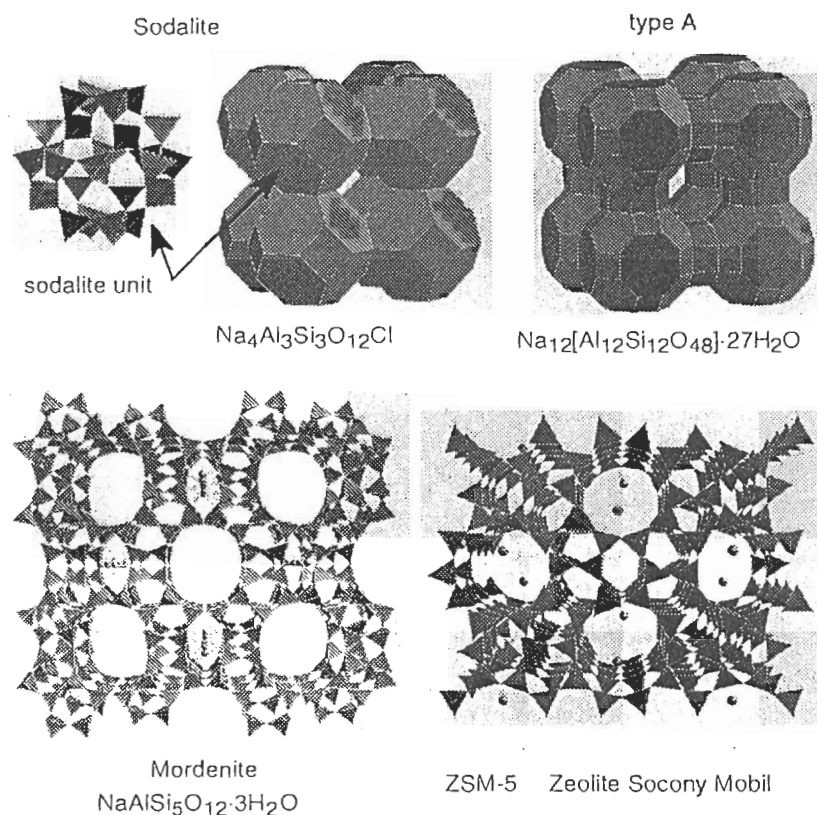
Figure 4.5 Structure of a few zeolites. These structures are based on corner-sharing \text{SiO}_4 and \text{AlO}_4 tetrahedra forming various motifs such as the sodalite unit (6.6 Å in diameter) shaped as a cuboctahedron. This unit contains 2.2 Å wide openings on hexagonal faces. The structure of the zeolite is formed by stacking such cuboctahedra to form small cubic or hexagonal prismatic voids. These voids may be connected to one another directly (sodalite) or through prismatic channels (zeolites of type A, for example). The large voids contain the charge-compensating cations and account for about 20–50% of the total volume of the crystal. Mordenite, the most silica-rich natural zeolite, contains large parallel channels formed by cycles of twelve tetrahedra (9.5 Å in diameter) and smaller channels (8-tetrahedra channels) trapping water molecules. The channels are connected by other perpendicular channels formed by 5- or 6-tetrahedra channels. In the ZSM-5 zeolite, a synthetic zeolite widely used as a catalyst, the Si/Al ratio is higher than 20. The larger the Si/Al ratio, the lower is the number of exchangeable cations and the network becomes hydrophobic
