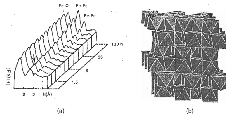
Figure 3.11 (a) Radial distribution function around Fe during crystallization of a ferric gel into hematite at 92 °C. The arrow indicates the appearance of the shoulder characteristic of Fe–Fe distances of 2.86 Å. (Reproduced from [62] 1990 by permission of Elsevier Science Ltd The Boulevard, Langford Lane, Kidlington OX5 1GB, UK (b) Structure of hematite α-Fe 2 O 3
