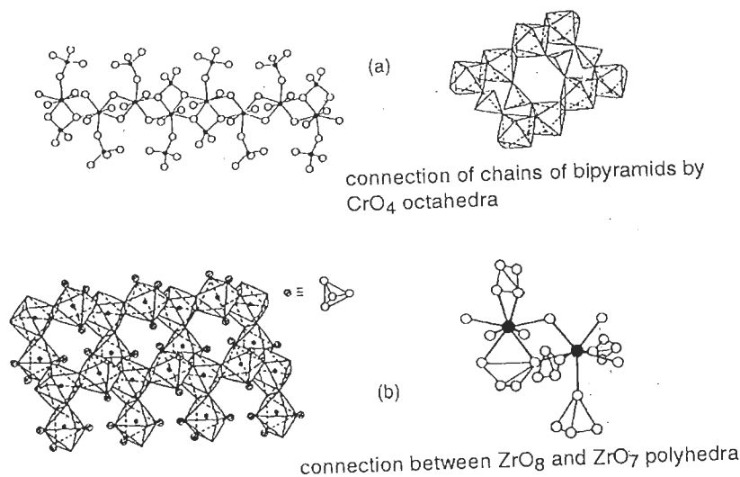
Figure 5.6 Structures of basic zirconium chromates: (a) Zr_8(OH)_{10}(CrO_4)_{11} \cdot 2H_2O ; (b) Zr(OH)_2(CrO_4)
