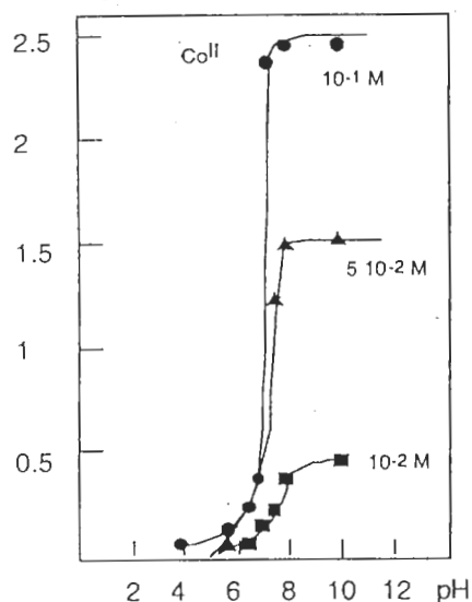
Figure 9.2 Adsorption of Co(II) on \alpha -FeOOH for various concentrations. (1 g solid in 200 ml solution). Reproduced by permission of Academic Press from [14]
