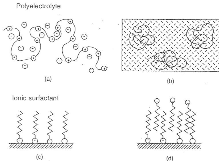
Figure 9.18 Polyelectrolyte (a) in solution and (b) adsorbed on a charged surface. Adsorption of an amphiphilic ionic surfactant, forming (c) a hydrophobic monolayer and (d) a hydrophilic double layer
