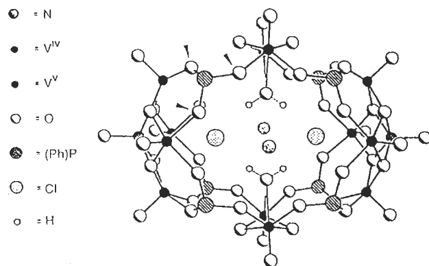
Figure 4.20 Structure of [V_{14}O_{22}(OH)_4(OH_2)_2(C_6H_5PO_3)_8]^{6-} . (Reproduced by permission of VCH from [74])
