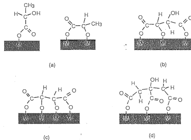
Figure 9.12 Coordination of (a) lactate, (b) l-tartrate, (c) mesotartrate and (d) citrate on oxide or hydroxide surfaces
