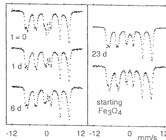
Figure 9.8 Evolution of Mössbauer spectra (300 K) for magnetite particles in the presence of ferric gel ( \text{Fe}(\text{OH})_3/\text{Fe}_3\text{O}_4=2.25 ) during ageing of the suspension. Reproduced by permission of Academic Press from [36]
