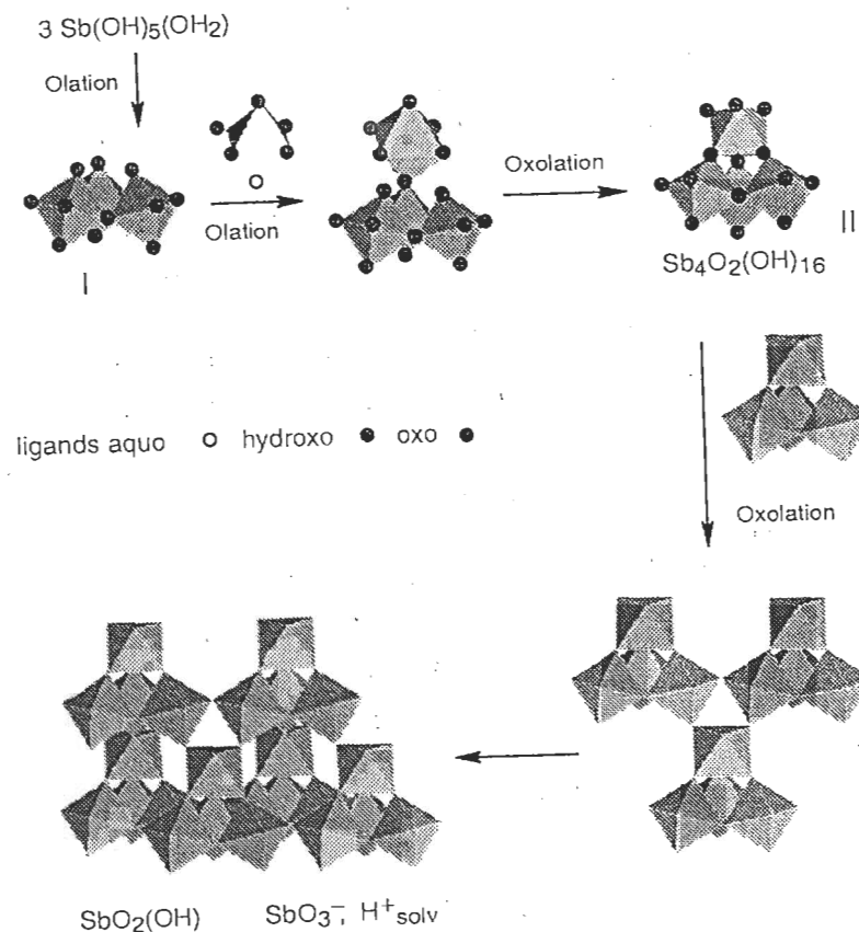
Figure 4.7 Possible reaction mechanism for the solution synthesis of antimonite acid (pyrochlore structure)
