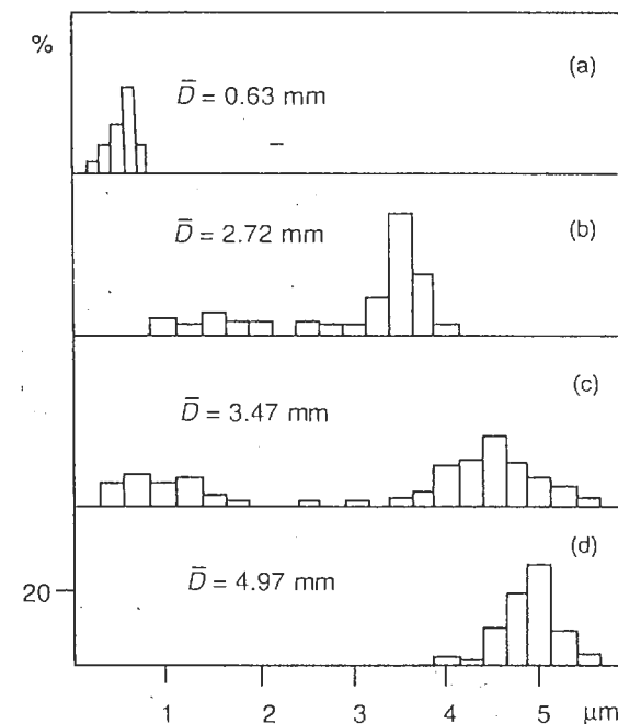
Figure 3.21 Size distribution of rutile particles as a function of the heating time at 95 °C. Duration (a) 0, (b) 1 h, (c) 3 h, (d) 6 h; (HCl 2.13 mol l -1 , Ti 0.22 mol l -1 ). From [94] by permission
