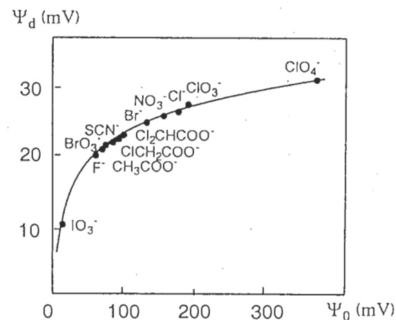
Figure 8.12 \psi_d as a function of \psi_0 at the specificity threshold for various anions adsorbed on \alpha -Fe 2 O 3 . Reproduced from [28] by permission
