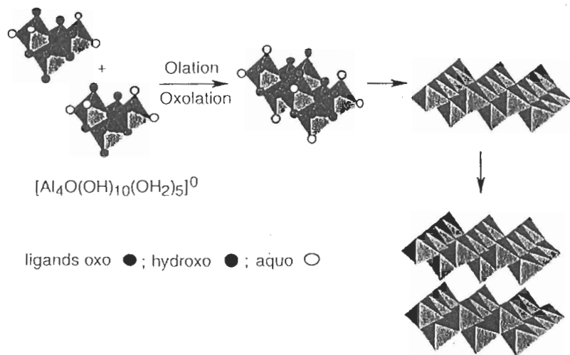
Figure 3.15 Possible formation mechanism of boehmite \gamma -AlOOH by thermolysis
