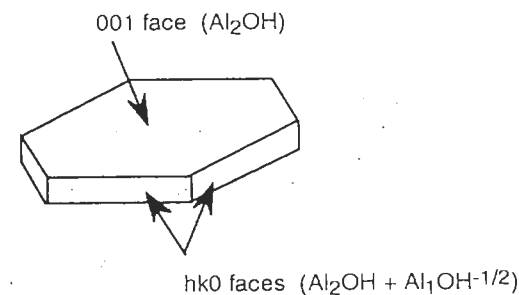
Figure 7.3 Gibbsite particle Al(OH) 3
