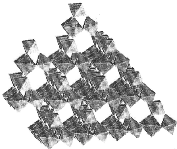
Figure 4.6 Pyrochlore structure of antimonite. \text{SbO}_6 octahedra are connected by oxo bridges (corner sharing). The solvated protons are distributed in the hexagonal channels of the structure
