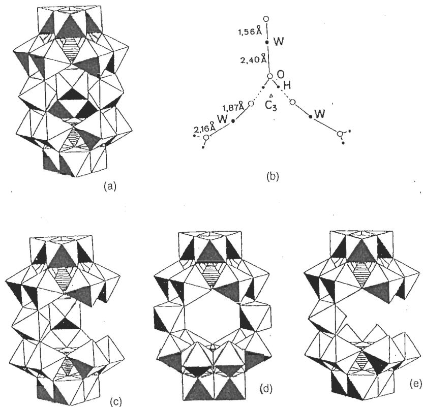
Figure 5.14 (a) Structure of the polyanion [P_2W_{21}O_{71}(OH_2)_3]^{6-} and (b) arrangement of tungsten and oxygen atoms and water molecules near the equatorial plane of the anion. From [50] by permission. Structure of vacancy compounds (c) [P_2W_{20}O_{70}(OH_2)_2]^{10-} and (d) [P_2W_{20}O_{72}]^{14-} . (e) Proposed structure for [P_2W_{19}O_{69}(OH_2)]^{14-} . Reproduced by permission of Conseil National de la Recherche du Canada from [40]
