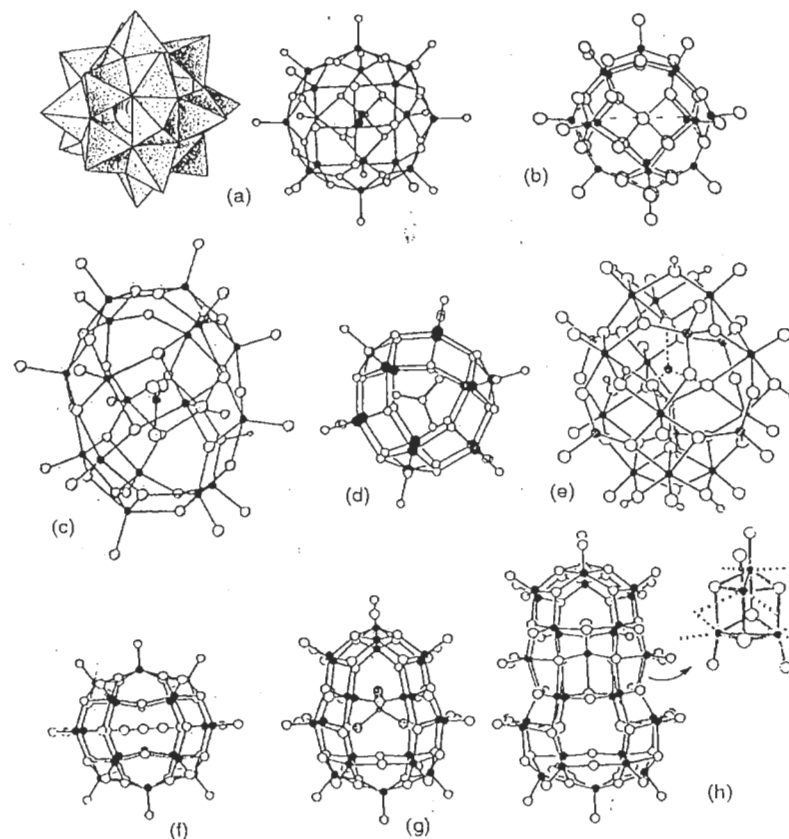
Figure 4.19 Cage structures of polyoxovanadate ions: (a) [V_{18}O_{42}(H_2O)]^{12-} (reproduced by permission of the American Chemical Society from [68]); (b) [H_4V_{18}O_{42}(X)]^{9-} ( X=Cl, Br, I ); (c) [HV_{18}O_{42}(NO_3)]^{10-} ; (d) [V_{15}O_{36}(CO_3)]^{7-} ; (e) [V_{19}O_{41}(OH)_9]^{9-} ; (f) [H_2V_{18}O_{44}(N_3)]^{5-} ; (g) [HV_{22}O_{54}(ClO_4)]^{6-} ; (h) [V_{34}O_{82}]^{10-} . (Reproduced by permission of VCH from [69,70,71,72])
