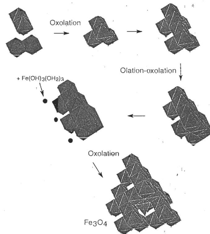
Figure 3.24 Possible reaction mechanism for the formation of the spinel lattice of \text{Fe}_3\text{O}_4 magnetite from a solution of ferric and ferrous ions
