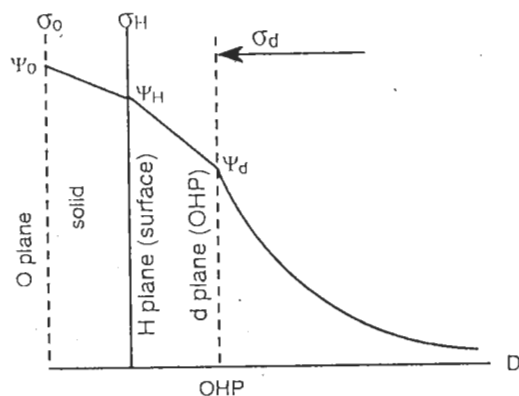
Figure 7.15 Charge distribution on ideal planes and decrease in the potential from the O plane. Reproduced by permission of John Wiley & Sons from [25]
