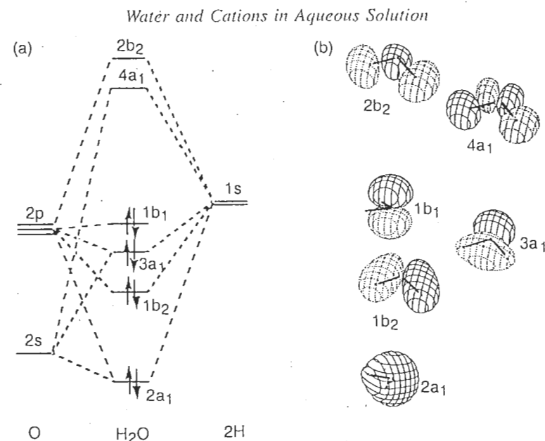
Figure 1.1 (a) Molecular orbital diagram of the water molecule and (b) electronic probability of presence. Reproduced by permission Academic Press from [2]
