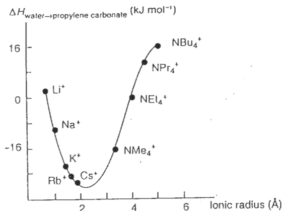
Figure 1.5 Transfer enthalpy for ions of various sizes from water towards propylene carbonate. Reprinted with permission from [19]. Copyright 1969 American Chemical Society
