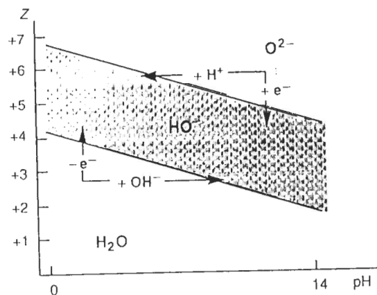
Figure 2.4 Possible initiation mechanisms for condensation reactions of metal cations in solution
