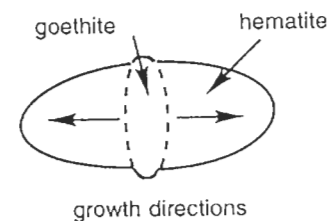
Figure 5.22 Anisotropic growth of hematite on a goethite nucleus. From [61b]
