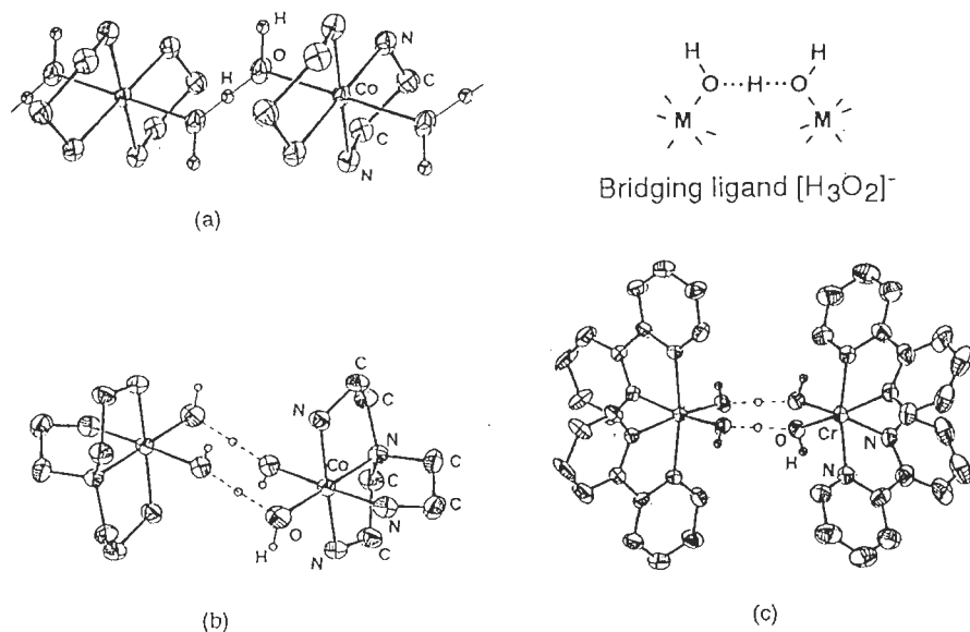
Figure 3.1 (a) Fragment of the chain of \text{trans-}[\text{Co}(\text{en})_2(\text{H}_3\text{O}_2)]_n^{2n+} \cdot 2n \text{ClO}_4^- bearing the [\text{H}_3\text{O}_2]^- ligand in which the proton appears approximately in the central position along the O-O axis (distances O-O 2.44 Å, O-H 1.22 Å, O-H non-bridging} about 0.95 Å). Crystal structures of (b) [(\text{tren})\text{Co}(\text{H}_3\text{O}_2)_2-\text{Co}(\text{tren})]^{4+} and (c) \text{cis-}[(\text{bipy})_2\text{Cr}(\text{H}_3\text{O}_2)_2\text{Cr}(\text{bipy})_2]^{4+} , where en = ethylenediamine, bipy = bipyridine and tren = triaminotriethylamine. From [5] with permission
