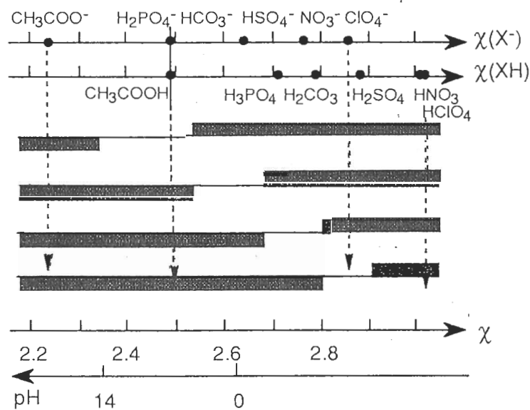
Figure 5.1 Complexation ranges of the hydrolyzed forms of Fe(III)
