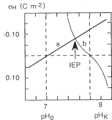
Figure 7.16 Graphic determination of the IEP using the intersection of (7.59) (a) and (7.60) (b). System parameters: K^+ = 10^7 , K^- = 10^{-11} , pH_0 = 7 , pH_K = 9 , C_0 = C_H = 1 \text{ F m}^{-2} , \sigma_T = 2 \text{ C m}^{-2} . Reproduced by permission of Academic Press from [40]
