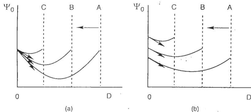
Figure 8.4 Surface potential as a function of the separation distance in the case of an interaction (a) at constant potential and (b) at constant charge. One of the surfaces is displaced from A towards C. \sigma_0 is indicated by the slope of the tangent at the origins of the potential variation with distance [ \sigma_0 = -\varepsilon(d\psi/dr)_{r=0} ]. In case (a) the decrease in the slope indicates a gradual decrease in the surface charge
