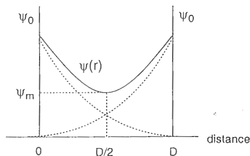
Figure 8.1 Variation in the potential (solid line) between two charged surfaces, resulting from the overlap of the diffuse layers (dotted lines)
