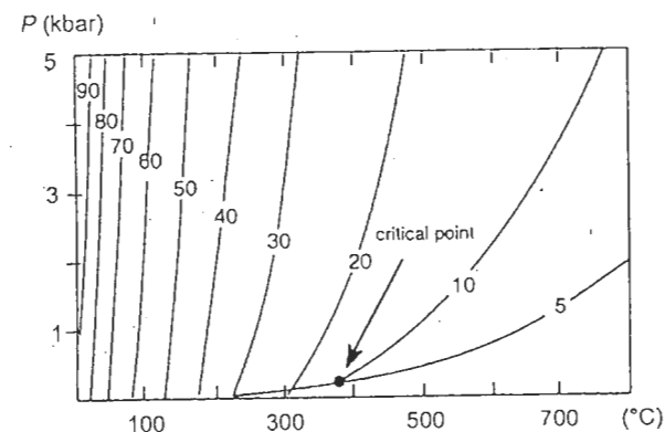
Figure 1.8 Change in the dielectric constant of water as a function of temperature and pressure. Reproduced by permission of Elsevier Science Ltd, The Boulevard, Langford Lane, Kidlington, OX5 1GB, UK from [40]
