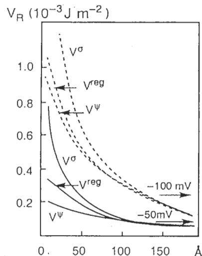
Figure 8.5 Electrostatic interaction energy V_R as a function of the separation distance for constant potential, constant charge interactions and under regulation conditions \Delta pK = 6 (dotted lines), \Delta pK = 3 (solid lines). Ionic strength 10^{-3} \text{ mol l}^{-1} . The potentials shown on each curve are for an infinite separation distance. Reproduced from [5] by permission
