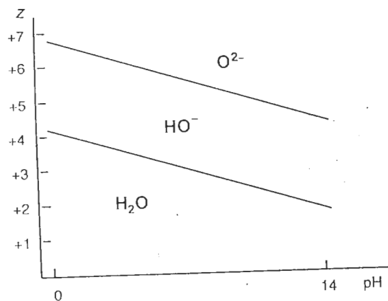
Figure 1.6 Nature of the ligands in the coordination sphere of a cation as a function of its formal charge z and the pH of the medium. Reproduced by permission of Academic Press from [2]
