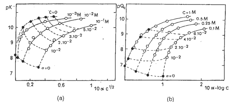
Figure 7.11 Calculation of affinity ratios \text{pK}^- (a) and \text{p}Q_C (b) by the double extrapolation method for \text{SiO}_2 -NaCl. Reproduced by permission of Elsevier Science Ltd from [29]
