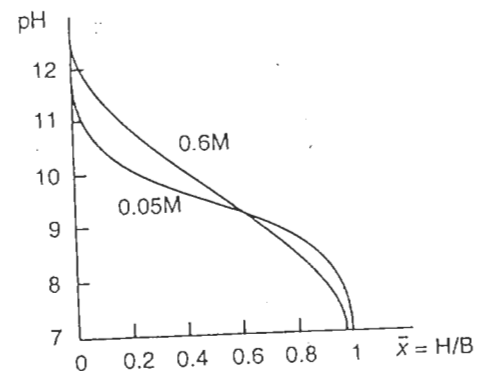
Figure 4.9 Protometric titration curves of borate for various concentrations, showing an intersection point corresponding to a maximum of condensation. Reproduced from [42]
