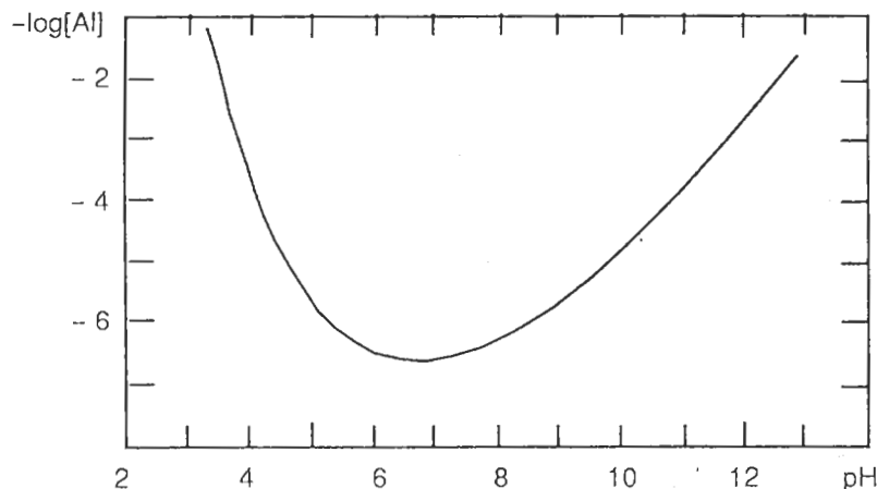
Figure 3.9 Solubility diagram of an amorphous aluminic gel (data obtained from [29b])
