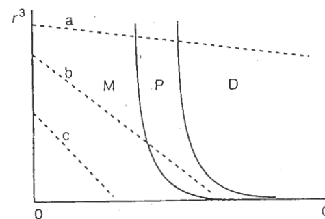
Figure 2.10 Domains of predominance of the main growth mechanisms: M mononuclear; P polynuclear; D diffusion. The evolution of r^3 (dashed lines) with concentration is approximately linear during precipitation initiated through mechanisms 1 (a), 2 (b) and 3 (c). From [22]
