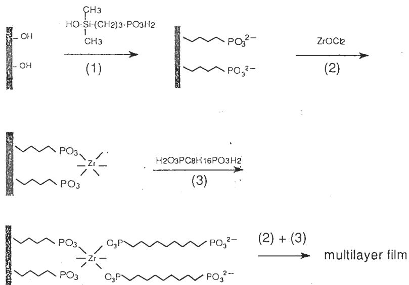
Figure 9.19 Formation of multilayer films on the surface of silica particles. Reprinted with permission from [99]. Copyright 1991 American Chemical Society
