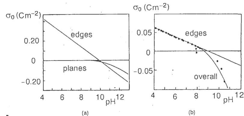
Figure 7.13 (a) \sigma_0 = f(pH) curves calculated for the large faces and the edges of gibbsite particles, for an NaCl concentration of 0.5 mol l^{-1} and a Stern layer capacitance fixed at 1.4 F m^{-2} . The adsorption constants of electrolyte ions are pK_A = pK_C = 0.1 . (b) Overall \sigma_0 = f(pH) curves calculated for gibbsite. The specific surfaces of the edges and the large faces are 3.4 and 16.4 m^2/g . The parameters used for the calculation are the same as in (a). The markers show experimental data. Reproduced by permission of Academic Press from [2]
