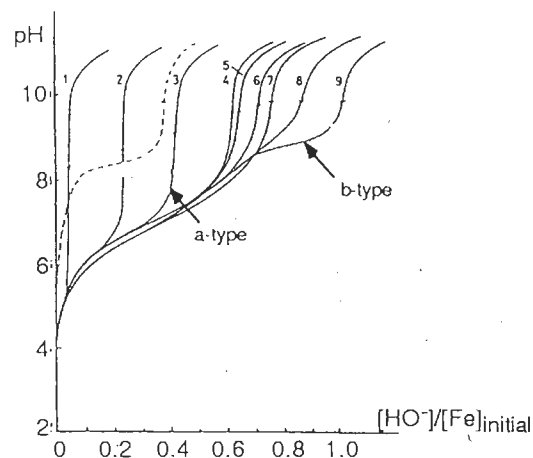
Figure 9.9 Titration of \gamma\text{-Fe}_2\text{O}_3 by \text{N}(\text{CH}_3)_4\text{OH} in the presence of ferrous ions. The ratio [\text{Fe}^{2+}]_{\text{added}}/[\text{Fe}^{3+}]_{\text{initial}} is shown on the curves. The dashed curve shows the titration of \text{Fe}^{2+} alone. Reproduced from [39], by permission
