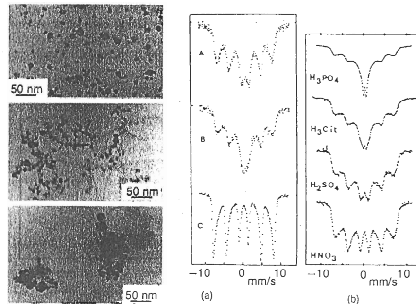
Figure 9.13 (a) SEM micrographs and Mössbauer spectra (300 K) of \gamma -Fe 2 O 3 colloids. The samples are sols stabilized using a polymer, containing aggregates of various sizes and morphology. They were obtained through modification of the surface charge. (b) Mössbauer spectra (290 K) of \gamma -Fe 2 O 3 particles (powder) flocculated with various acids. Reproduced by permission of Elsevier Science Ltd from [59]
