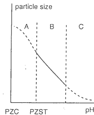
Figure 8.17 Variation in particle size as a function of precipitation pH ( \text{pH} \geq \text{PZC} , surface charge \leq 0 )
