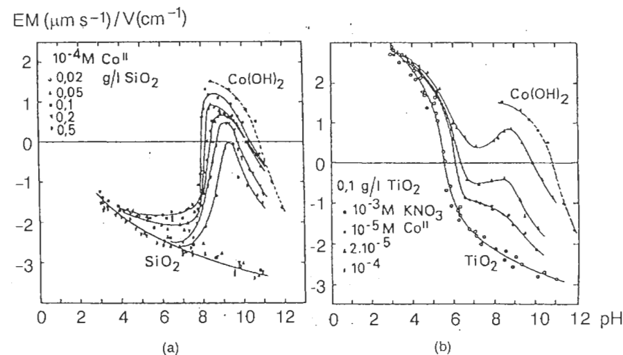
Figure 9.4 Electrophoretic mobility (a) for various \text{SiO}_2 amounts and (b) for \text{TiO}_2 in the presence of \text{Co}(\text{NO}_3)_2 . Reproduced by permission of Academic Press from [22]
