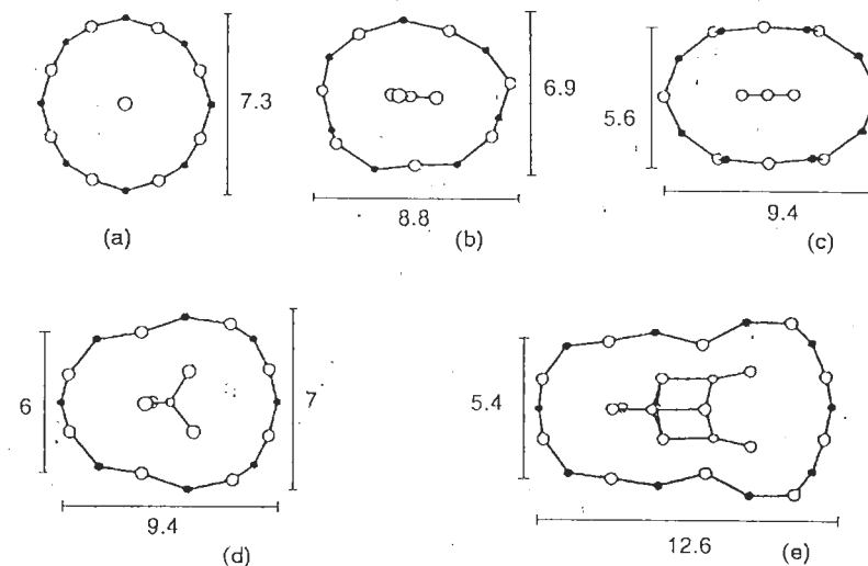
Figure 4.21 Simplified polyvanadic structures built by template effect (lengths in Å): (a) [H_4V_{18}O_{42}(X)]^{9-} ( X = Cl, Br or I ); (b) [HV_{18}O_{42}(NO_3)]^{10-} ; (c) [H_2V_{18}O_{44}(N_3)]^{5-} ; (d) [HV_{22}O_{54}(ClO_4)]^{6-} ; (e) [V_{34}O_{82}]^{10-} . Reproduced by permission of VCH from [72]
