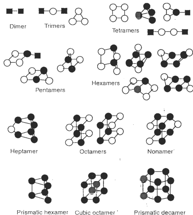
Figure 4.1 Main structures of silicates in aqueous solution (silicon concentration 1.5 \text{ mol l}^{-1} , \text{KOH/Si} = 1 , 22^\circ\text{C} ). \text{SiO}_4 tetrahedra, shown using different symbols, share 1 (■), 2 (○) or 3 (●) corners. The double cages are stabilized in solution by tetraalkylammonium cations. Reproduced from [7] with permission
