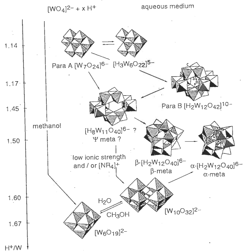
Figure 4.24 Structure of a few tungstic ions
