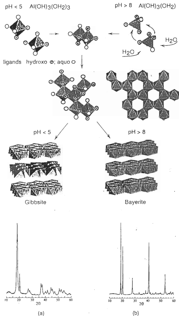
Figure 3.10 Possible reaction mechanisms for the formation of Al(OH) 3 (gibbsite, bayerite) during evolution of the aluminic gel at pH < 5 and pH > 8. XRD of the solids precipitated at pH 10 and aged (a) at pH 4.5 for 1 month (gibbsite) and (b) at pH 10 for 1 week (bayerite) (J. Hernandez and J.P. Jolivet, unpublished results)
