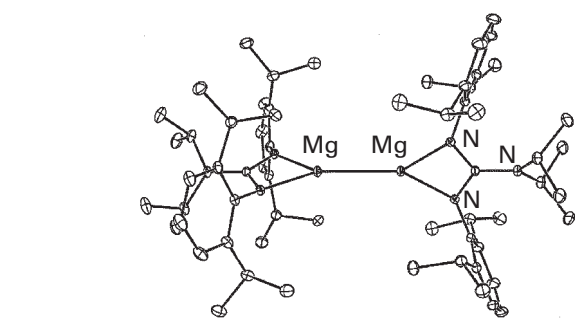
13 LMgMgL , L = [Ar(NC)(N^iPr_2)NAr]^- \cdot iPr = (CH_3)_2CH
