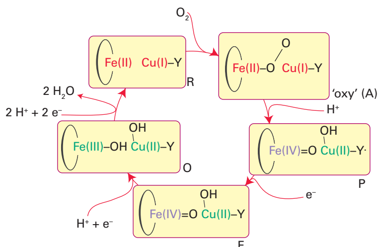
Figure 27.36 The catalytic cycle of cytochrome c oxidase. The intermediates are labelled according to current convention. Electrons are provided from the other haem and Cu_A . During the cycle, an additional four H^+ are pumped across the membrane.
