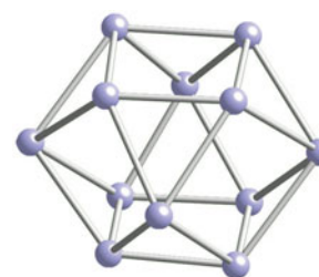
26 B_{12} cuboctahedron
