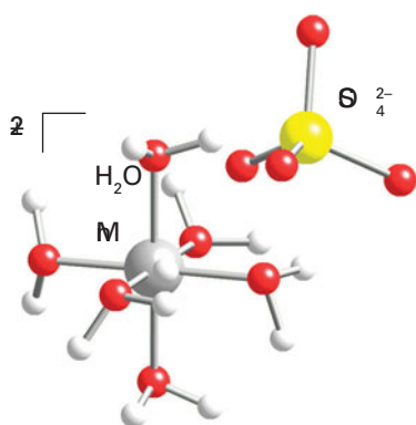
3 [\text{Mn}(\text{OH}_2)_6]\text{SO}_4
