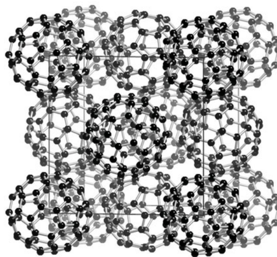
Fig. 3.16 The structure of solid C_{60} showing the packing of C_{60} polyhedra on an fcc unit cell.
