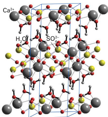
Figure 12.9 The structure of \text{CaSO}_4 \cdot 2\text{H}_2\text{O} highlighting the water molecules that are mainly lost on heating above 150^\circ\text{C} .
