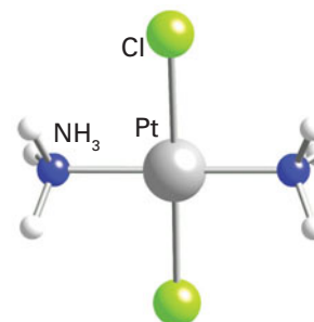
38 trans - [\text{PtCl}_2(\text{NH}_3)_2]
