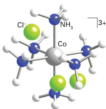
2 [\text{Co}(\text{NH}_3)_6]\text{Cl}_3
