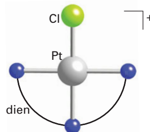
76 [\text{PtCl}(\text{dien})]^+
