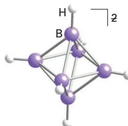
9 closo - [\text{B}_5\text{H}_6]^{2-}
