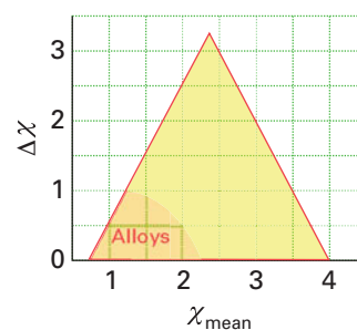
Fig. 3.25 The approximate locations of alloys in a Kettelaar triangle.
