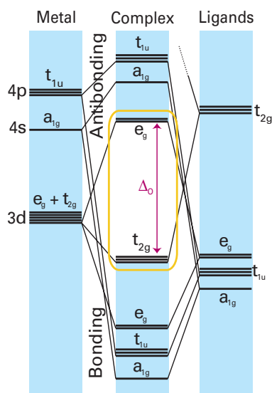
Figure 22.1 The energy levels of the orbitals of an octahedral complex with strong-field ligands.
