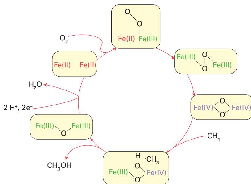
Figure 27.38 A plausible catalytic cycle for methane monoxygenase.
