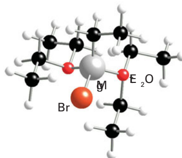
12 \text{MgBr}(\text{OEt})_2
