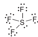
13 \text{SF}_4
