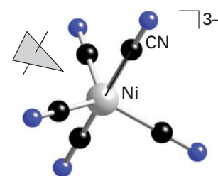
51 [\text{Ni}(\text{CN})_5]^{3-} , trigonal bipyramidal ( D_{3h} )
