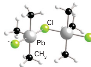
23 (\text{PbClMe}_3)_n
