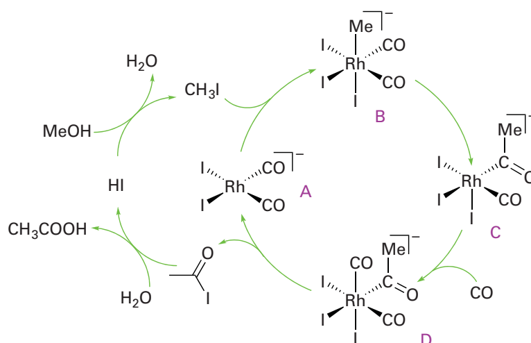
Figure 26.13 The catalytic cycle for the formation of ethanoic (acetic) acid with a rhodium-based catalyst. The oxidative addition step (A → B) is rate determining.
