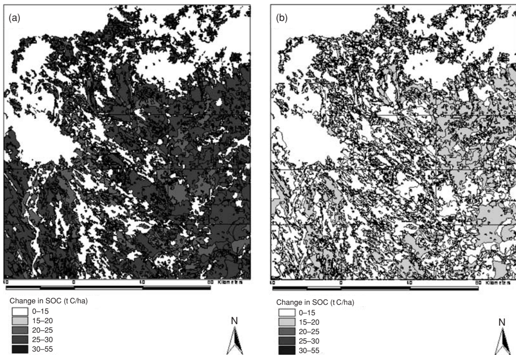
Figure 12.9 Predicted change in soil carbon over 100 years due to a land management change (application of 4.26\ t\ ha^{-1}\ y^{-1} cereal straw to all arable land) using (a) RothC model and (b) CENTURY model (after Falloon et al. , 2002).
