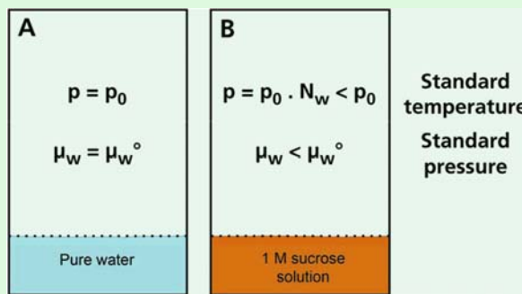
FIGURE 1. The difference in water potential between two systems. The system at the left is a sealed container with pure water at standard temperature and pressure; the partial water vapor pressure in this container is p_o and the chemical potential of water in this system is \mu_w^o . The system at the right is a container with a solution of 1 M sucrose at the
