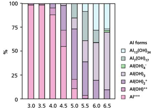
FIGURE 21. Calculated distribution of total inorganic Al concentration over various monomeric and polymeric forms as a function of pH. Calculations are based on parameters given by Nair & Prenzel (1978).
