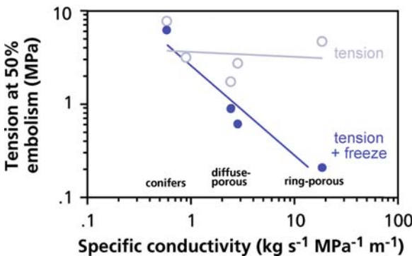
FIGURE 17. Tension at the time of 50% embolism as dependent on the size of the tracheids or vessels. The experiment was carried out with trees exposed to water stress (tension, open circles) and with trees exposed to a freeze-thaw cycle (tension + freeze, solid circles) (after Sperry & Sullivan 1992). Copyright American Society of Plant Biologists.
