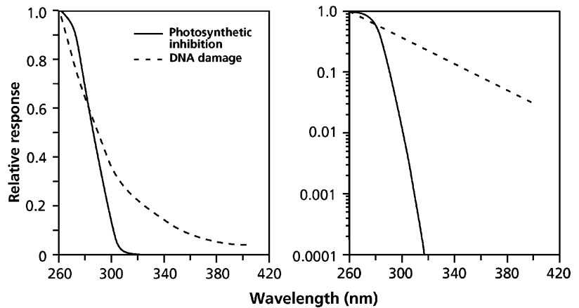
FIGURE 2. The damaging effect of UV on the dichlorophenol-indophenol reduction of chloroplasts isolated from Spinacia oleracea (spinach) (“photosynthetic inhibition”) and on DNA in microorganisms (“DNA damage”). The same data are plotted on a linear (left) and an exponential (right) scale, showing that DNA is very sensitive to UV radiation, compared with photosynthesis (Jones & Kok 1966, as cited in Caldwell 1981, and Sewtlow 1974).
