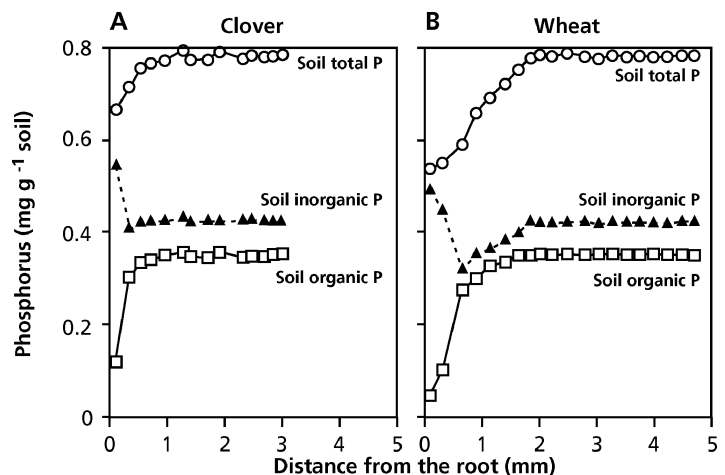
FIGURE 11. Distribution of total, inorganic and organic P in the rhizosphere of Trifolium alexandrinum (clover, 10 days old) and Triticum aestivum (wheat, 15 days old) grown in a silt loam (Tarafdar & Jungk 1987).
