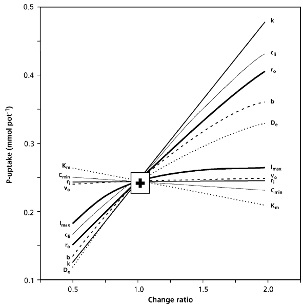
FIGURE 20. Effects of changing parameter values (from 0.5 to 2.0 times the standard value) on simulated P_i uptake by roots of Glycine max (soybean). k is the rate of root elongation, C_{ii} is the initial P_i concentration in solution, r_o is the root diameter, b is the buffer power of the soil, D_e is the diffusion coefficient of P_i in the soil, I_{max} is the maximum P_i inflow rate, v_o is the rate of transpiration, r_i is the spacing between individual roots, C_{min} is the lowest concentration at which P_i uptake is possible, and K_m is the P_i concentration at which the rate of P_i uptake is half of that of I_{max} (Silberbush & Barber 1983). With kind permission, from the Annual Review of Plant Physiology, Vol. 36, copyright 1985, by Annual Reviews Inc.
