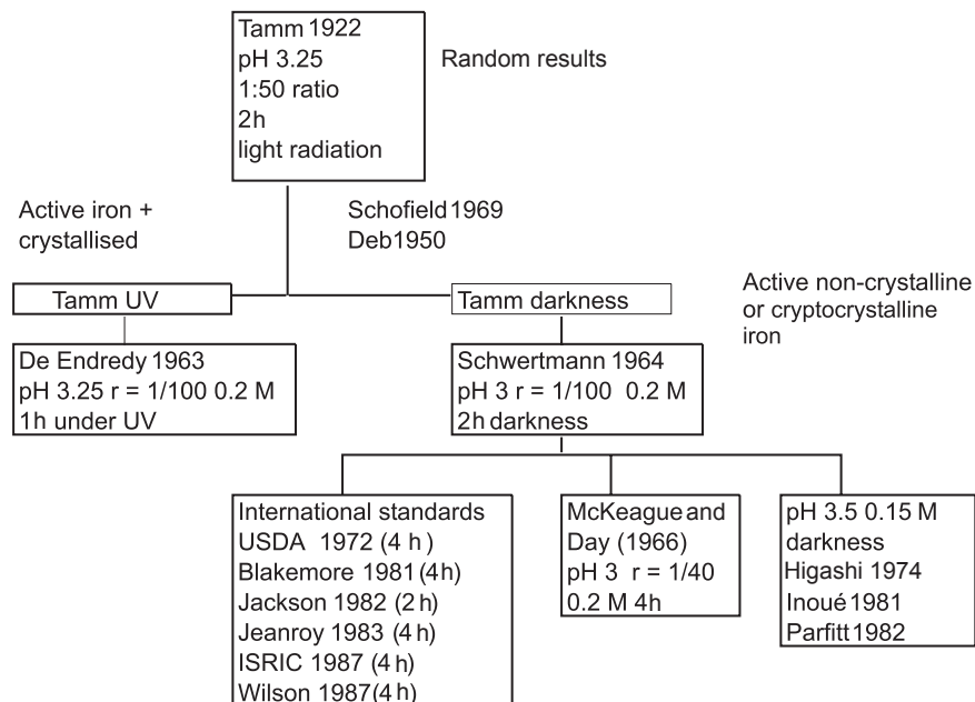
Fig. 6.5. Changes of the Tamm method using ammonium oxalate-oxalic acid reagent (basic procedures)
