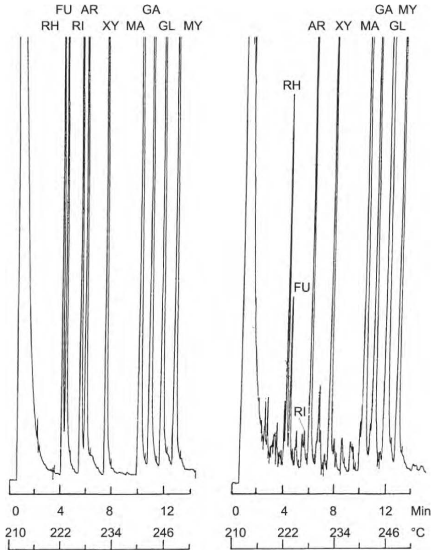
Fig. 13.1. Chromatograms of alditol acetates (conditions described in "Chromatographic conditions", RH, rhamnose; FU, fucose; RI, ribose; AR, arabinose; XY, xylose; MA, mannose; GA, galactose; GL, glucose; MY, myoinositol internal standard). On the left: standard mixture corresponding to the injection of 0.2 \mu\text{g} of each sugar. On the right: sugars of a strongly desaturated ferrallitic soil of the Niari valley (Congo). Hydrolysis according to the procedure described in "Attack Favouring the Measurement of Pentoses" earlier.
