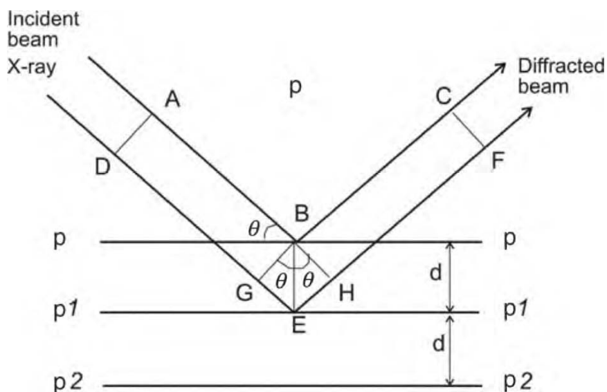
Fig. 4.2 Diffraction of an incidental beam by crystalline reticular planes. Lines p , p1 , p2 represent the parallel and equidistant reticular planes separated by space d . An X-ray beam striking the higher plane p will be reflected in the incidental angle \theta . To obtain a measurable reflection, all the rays reflected by planes p , p1 , p2 , etc, must be in phase. To achieve this, GE + EH , the path difference between radiations ABC and DEF must be equal to a whole number of the wavelength. As GE = EH = d \sin \theta , the condition is thus the law of Bragg (1).
