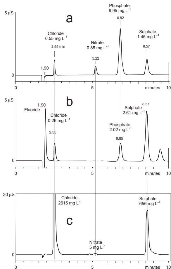
Fig. 18.2. Analysis of soluble anions of soils by ionic chromatography (Doubeau and Rochette, IRD Montpellier, France, unpublished data). (a) cold water extract (10 g 200 mL -1 , agitate for 4 h) of a Luvisol ( Hapludalf ) developed on loess, cultivated at Boigneville (France), injection without dilution (b) hot water extract of the a-Luvisol previously extracted with cold water (reflux boiling for 16 h), injection without dilution (c) 1:5 extract at 20°C of a surface horizon of a chloruro-sulphated Salisol ( Maison de la Nature , Latte, France), 1:50 dilution of the extract before injection. The contents are those of the undiluted extract.
