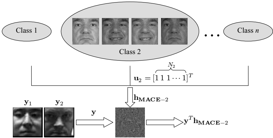
Fig. 3.7. The CFA algorithm; the filter response of y_1 and \mathbf{h}_{\text{MACE-2}} can be distinctive to that of y_2 and \mathbf{h}_{\text{MACE-2}} .
