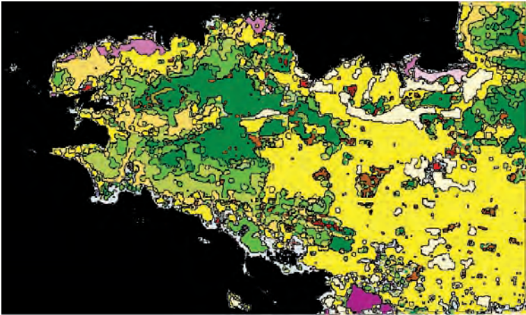
Fig. 30.2b Post-processing techniques applied to landscape classification (Phase 2) (See also Plate 41 in the Colour Plate Section)
