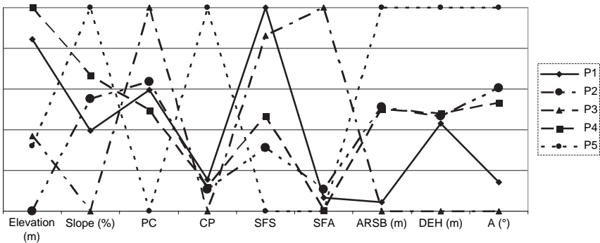
Fig. 32.2 Geomorphometric patterns of the five soilscales (the mean values for each variable were re-scaled between 0 and 1, for the proportion of the class with maximum mean value being 1 and with minimum mean value being 0, with the maximum indicated by the top of the figure)
