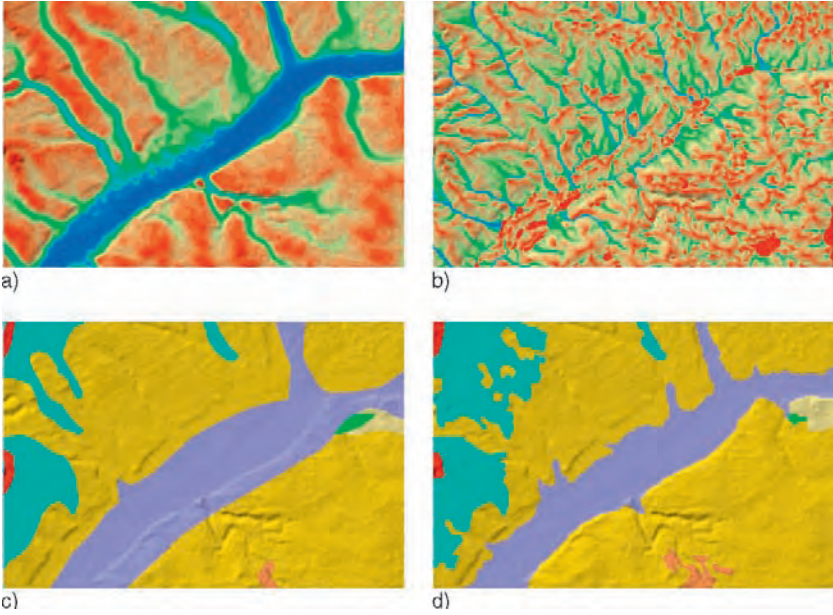
Plate 20 Comparison of flow-accumulation based on a Monte Carlo simulation using a single-flow approach (a) and a multiple-flow approach (b) for a section of the geological map of the Republic of Niger (c = original, d = corrected) (See also Figure 18.2 on page 216)
