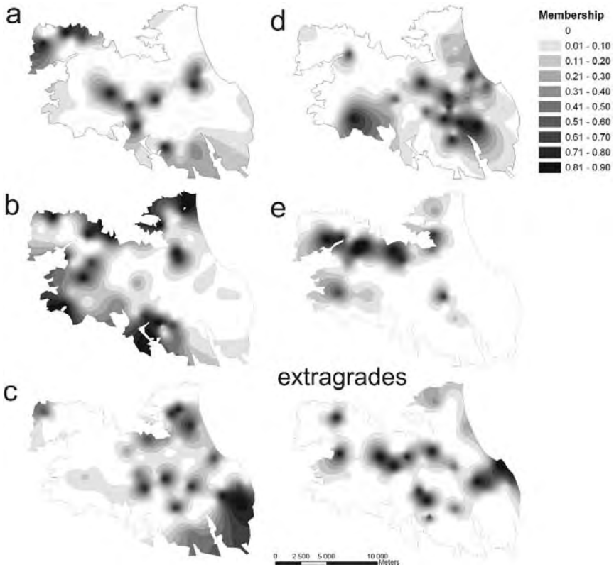
Fig. 26.2 Kriged maps of membership values for the five fuzzy classes (a–e) and extragrades
