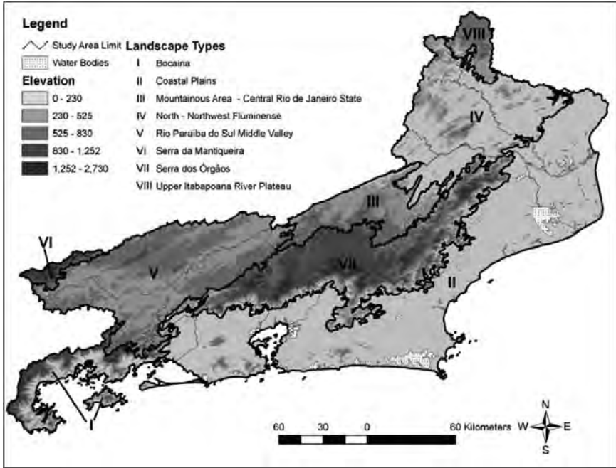
Fig. 34.2 Landscape types of Rio de Janeiro state
