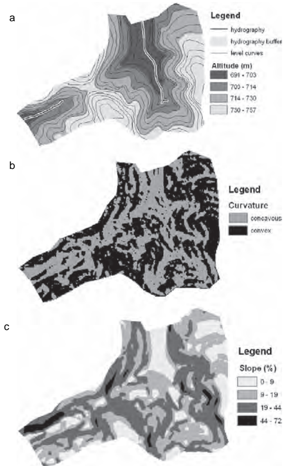
Fig. 31.2 Maps derived from DEM of CAPTA-Frutas, Jundiá, SP, Brazil. (a) altitude with level curves, hydrography and buffer; (b) curvature; (c) slope
