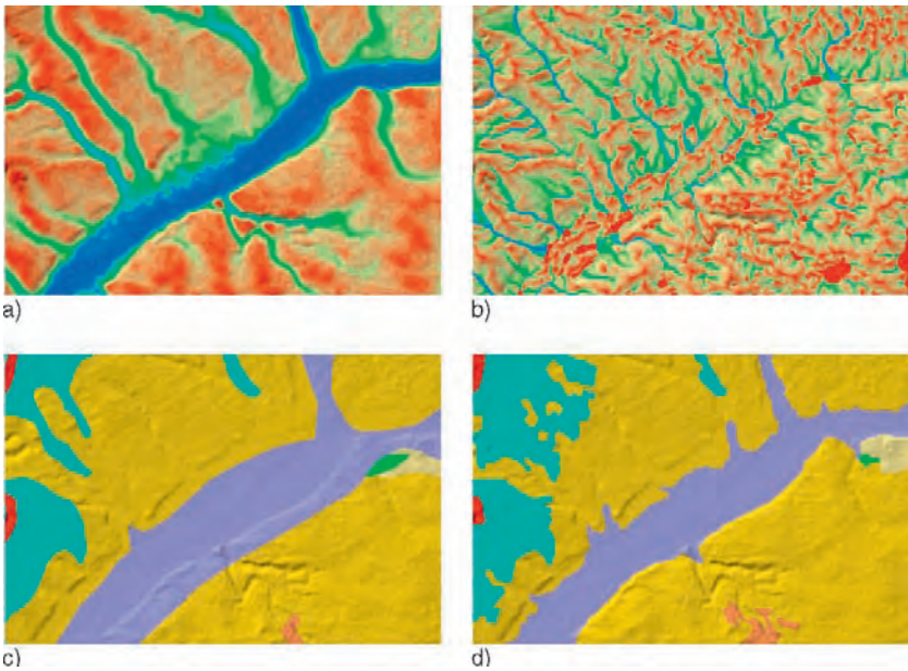
Fig. 18.2 Comparison of flow-accumulation based on a Monte Carlo simulation using a single-flow approach (a) and a multiple-flow approach (b) for a section of the geological map of the Republic of Niger (c = original, d = corrected). (See also Plate 20 in the Colour Plate Section)
