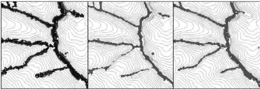
Fig. 28.3 Detail of delineation of alluvial soil by combination of drainage area and slope curvature (a), compound topographic index (b), combination of drainage area and height above watercourse (c)
