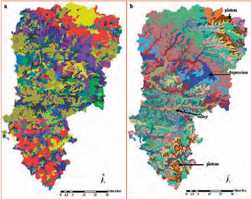
Fig. 17.2 Maps resulting from the bottom-up (a) and the top-down (b) approaches (See also Plate 18 in the Colour Plate Section)
