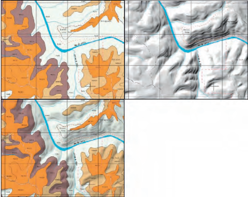
Plate 12 Soil map with conventional soil information, analytical DEM hill shading and fusion of the hill shading with the conventional soil map (See also Figure 9.5 on page 110)
