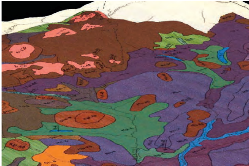
Plate 3 Perspective view, soil map draped on SRTM elevation model (See also Figure 6.1B on page 76)
