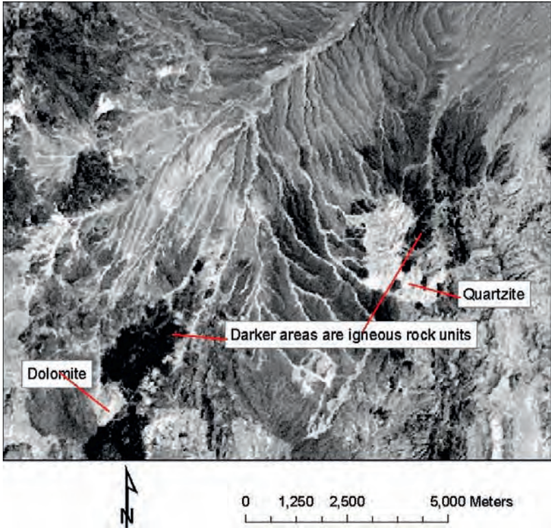
Fig. 16.2 Normalized difference ratio of Landsat 7 bands (5-2)/(5+2) clearly differentiates igneous rocks such as andesite ( darker areas ) from sedimentary rocks ( lighter areas ) such as dolomite and sandstone/quartzite at the northern edge of the Tonoquits Volcanic Field in the Basin and Range physiographic province, southwestern Utah
