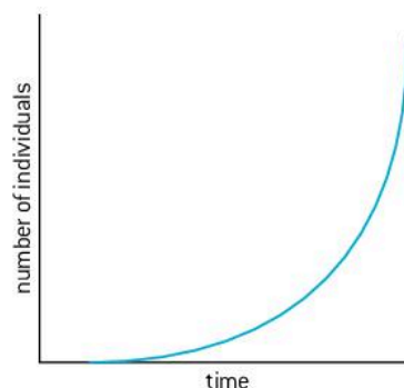
▲ Figure 2.1.11 J-shaped growth curve of a population
