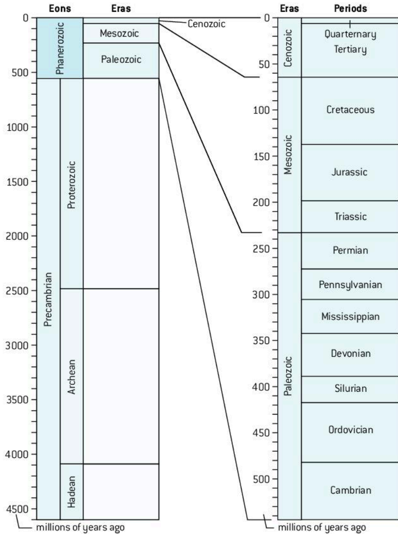
▲ Figure 3.2.10 The geological timescale
