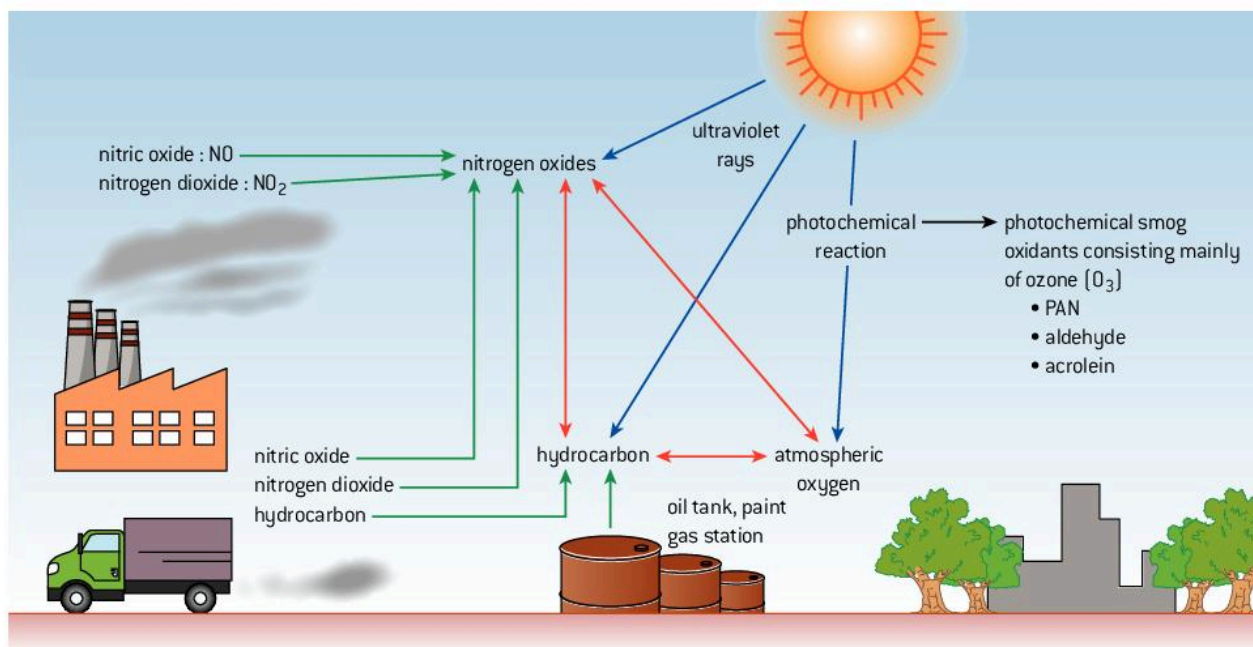
▲ Figure 6.3.3 Formation of photochemical smog
