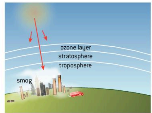
▲ Figure 6.2.1 Ozone in the atmosphere
