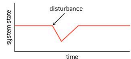
▲ Figure 1.3.10 Stable equilibrium
