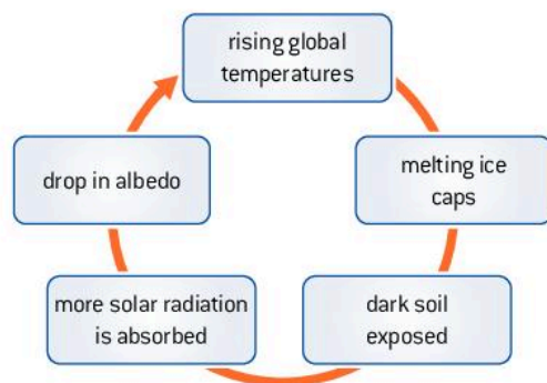
▲ Figure 1.3.14 Positive feedback in global warming
