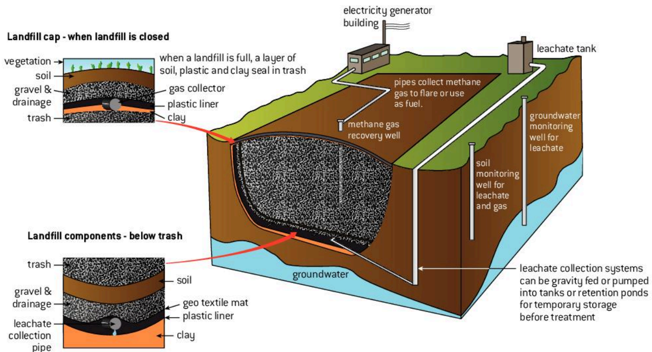
▲ Figure 8.3.12 The technology of a landfill site
