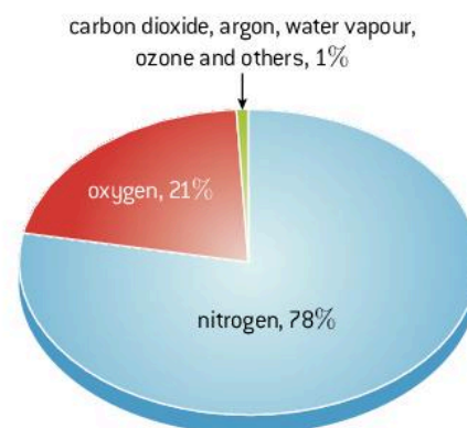
▲ Figure 6.1.1 Atmospheric composition
