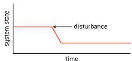
▲ Figure 1.3.11 Unstable equilibrium
