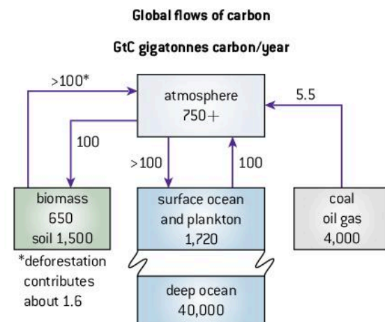
▲ Figure 2.3.7 The carbon cycle with flow values
