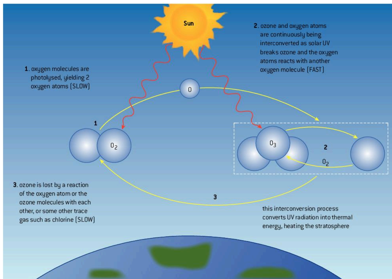
▲ Figure 6.2.5 The ozone cycle
