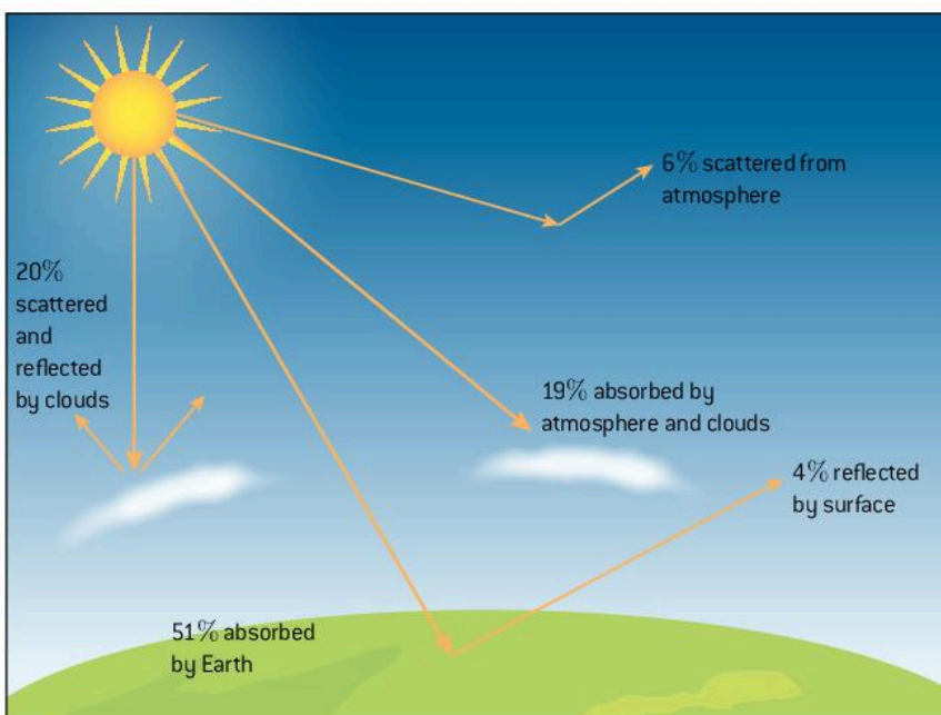
▲ Figure 7.2.8 The greenhouse effect showing percentages absorbed, reflected or scattered
