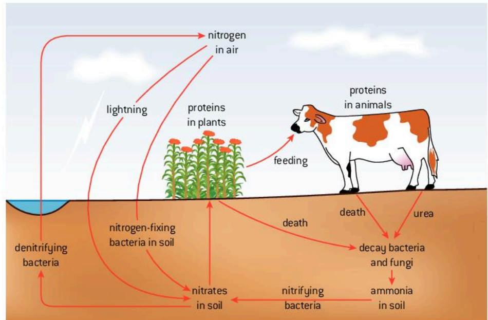
▲ Figure 2.3.8 The nitrogen cycle
