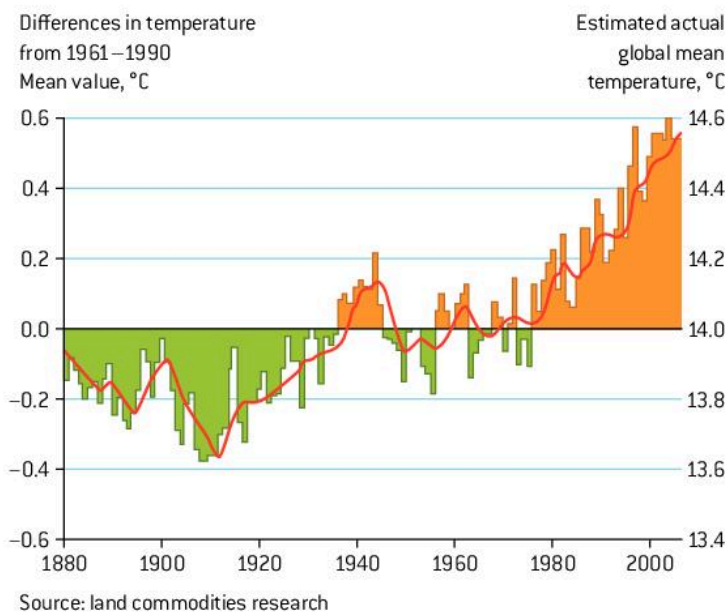
▲ Figure 7.2.1 Global average temperature 1860–2008
