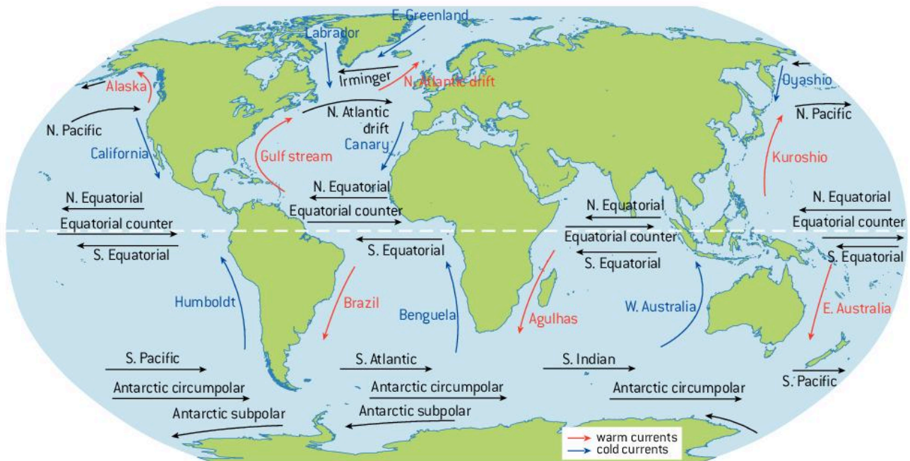
▲ Figure 4.1.5 The ocean currents
