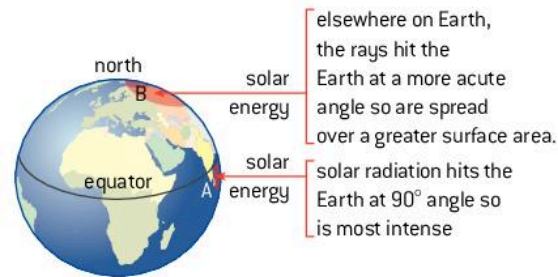
▲ Figure 2.4.2 Solar radiation hitting the Earth
