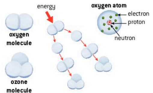
▲ Figure 6.2.2 Formation of ozone
