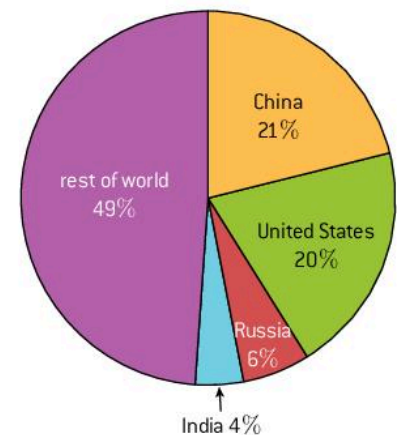
▲ Figure 7.1.7 World energy use
