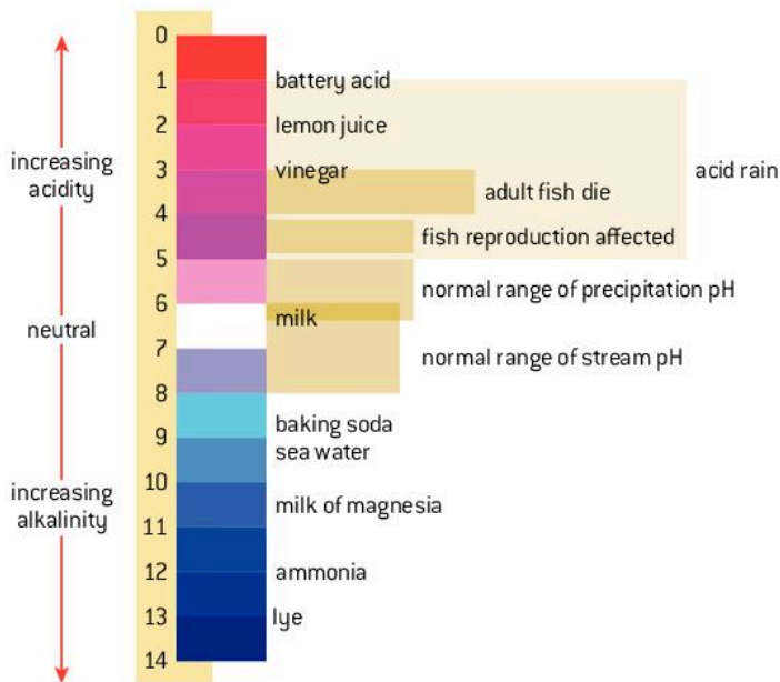
▲ Figure 6.4.1 The pH scale
