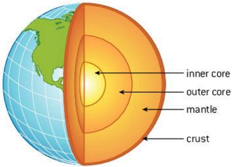
▲ Figure 3.2.5 Simplified diagram of the Earth
