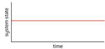
▲ Figure 1.3.8 Static equilibrium
