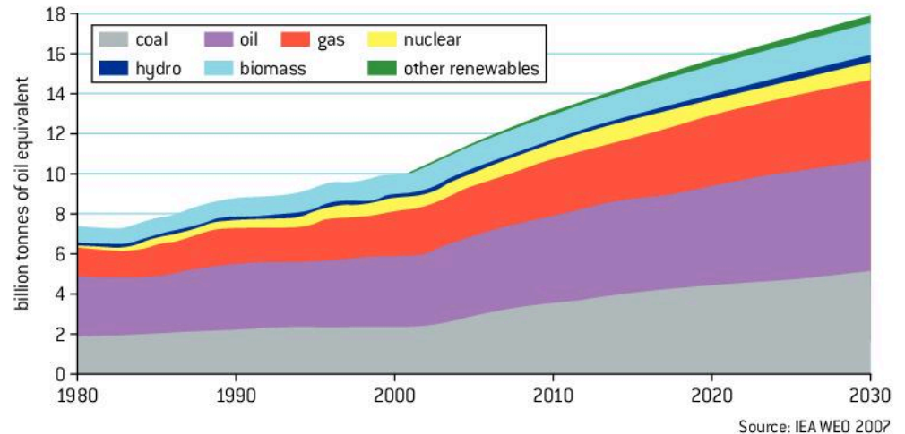
▲ Figure 7.1.2 Projected growth in global energy demand
