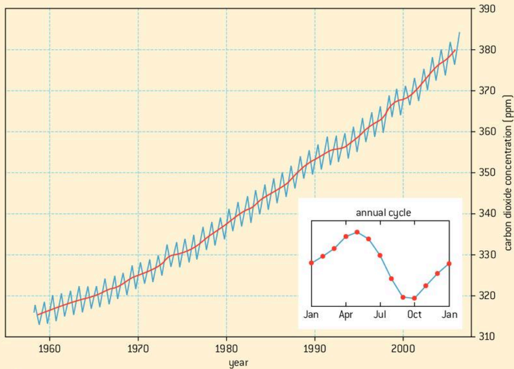
▲ Figure 7.2.15 Atmospheric CO 2 in ppm 1958–2007
