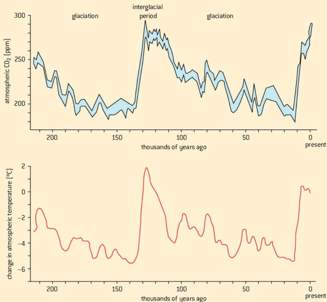
▲ Figure 7.2.14 CO 2 and temperature levels of the last 240,000 years
