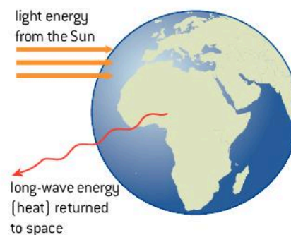
▲ Figure 1.2.7 A closed system – the Earth
