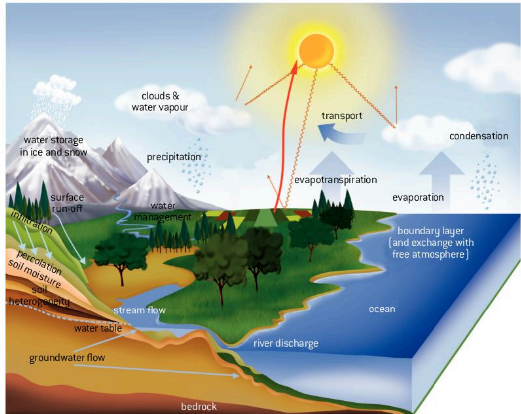
▲ Figure 4.1.3 The water cycle
