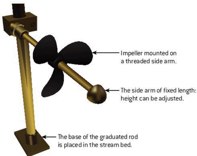
▲ Figure 2.5.7 Impeller
