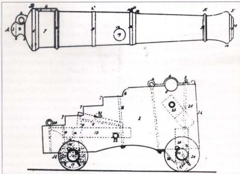
Diagram explaining the parts of a typical heavy cannon and carriage of the Napoleonic wars. Note the ring for the breeching rope on top of the cascabe, and the dispart sight on top of the reinforcing ring, immediately forward of the trunnion. (Author's collection)
