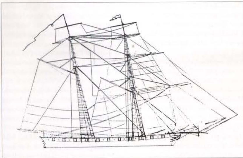
The sail plan of the American privateering schooner Prince de Neufchâtel in 1813. In October 1814 while under the command of the French-born Captain ' Ordranax her crew repulsed a boarding attempt by ship's boats from HMS Endymion . (Mel Fisher Maritime Museum, Key West, Florida)
