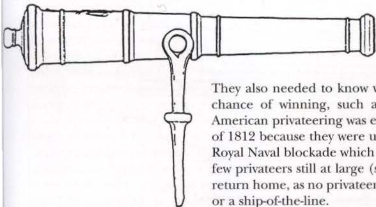
A swivel gun, an essential part of the armament of a privateer or pirate vessel during the 18th and early 19th centuries. Mounted on the ship's rail, they could sweep the enemy decks with a charge of musket balls or scrap metal immediately prior to boarding. (Author's collection)
