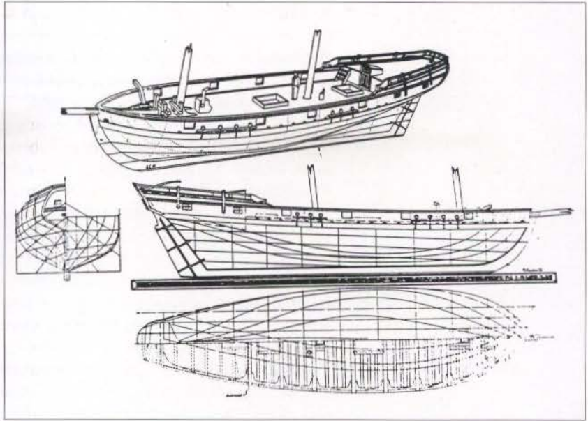
Profile, plan and isometric view of a former privateering schooner captured and purchased into the Royal Navy in 1780, when she was renamed the armed schooner Bernice . Although her original name and port are unknown, she was almost certainly an American vessel. (Mel Fisher Maritime Museum, Key West, Florida)
