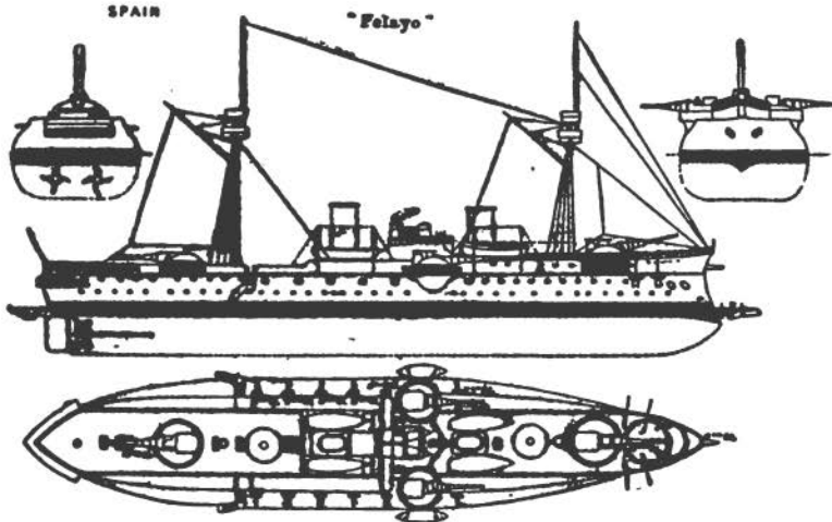
SPANISH BATTLESHIP "PELAYO."
