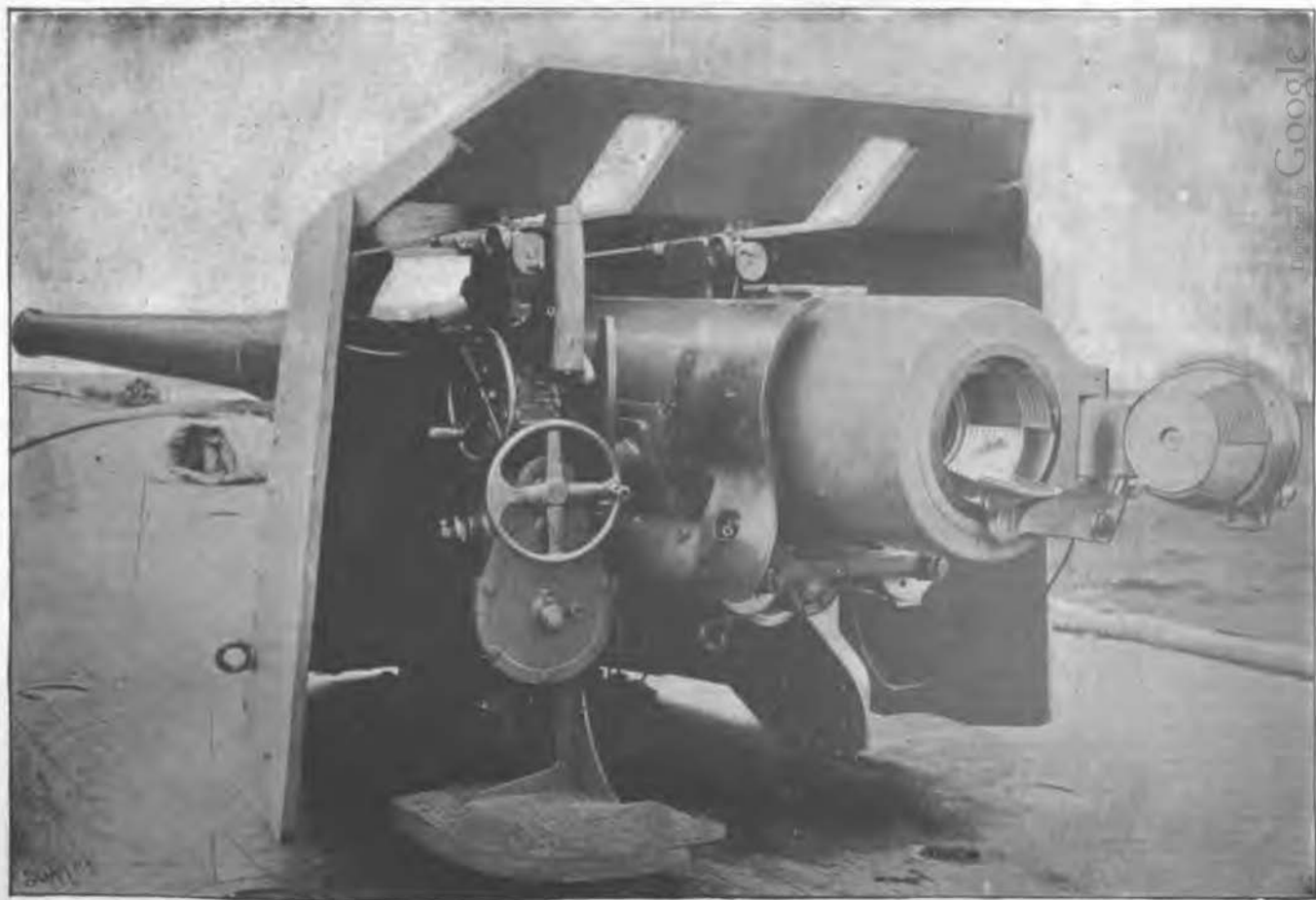
6-INCH RAPID-FIRE GUN OF U. S. CRUISER "NEW ORLEANS," MADE AT ELSWICK, ENG.
