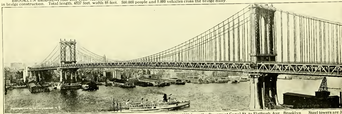
MANHATTAN BRIDGE —This is a double-deck suspension bridge, constructed 1901 to 1909 from the Bowery at Canal St. to Flatbush Ave., Brooklyn. Steel towers are 336 feet high, resting on masonry pedestals which are 92 feet below water line, the four cables weigh 6300 tons, length of bridge, 8655 feet, width 120 feet, total cost $13,400,000.
