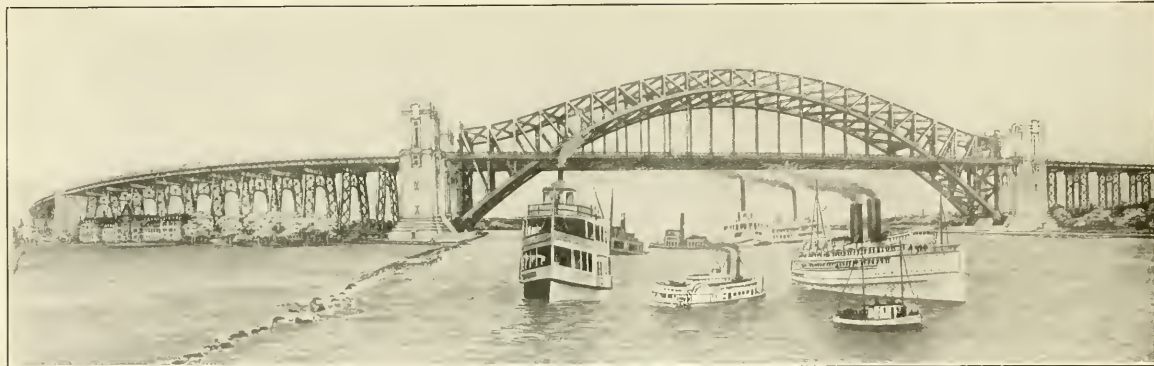
HELL GATE BRIDGE—This is the longest steel arch bridge in the world and crosses Hell Gate, Ward's Island and Randall's Island, from Bronx Hills to New York. Length of steel arch 1000 feet, height 200 feet, weight 80,000 tons, concrete towers, 200 feet high, cost $14,000,000.
