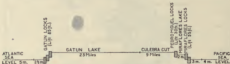
DIAGRAM SHOWING LOCK TYPE OF CANAL AT PANAMA.
