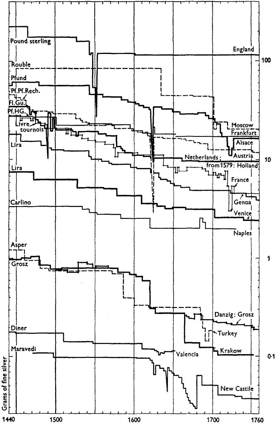
Fig. 4. Moneys of account in Europe, classified by their weights in grams of fine silver. (Pf. Pf. Rech.: Pfund Pfenning Rechengulden . Fl. Gu.: florin; from 1579, guilder. Pf. H. G.: Pfund Heller Gulden . Approximate values are given for the rouble and the asper .)
