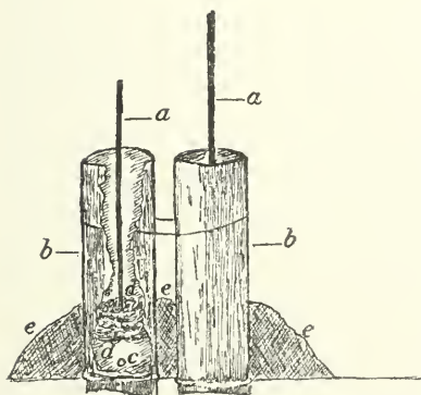
View of Sema smith's bellows from behind.
