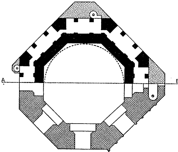
Fig. 3. Plan of mausoleum of Öljeitü at Sulṭāniyeh.
