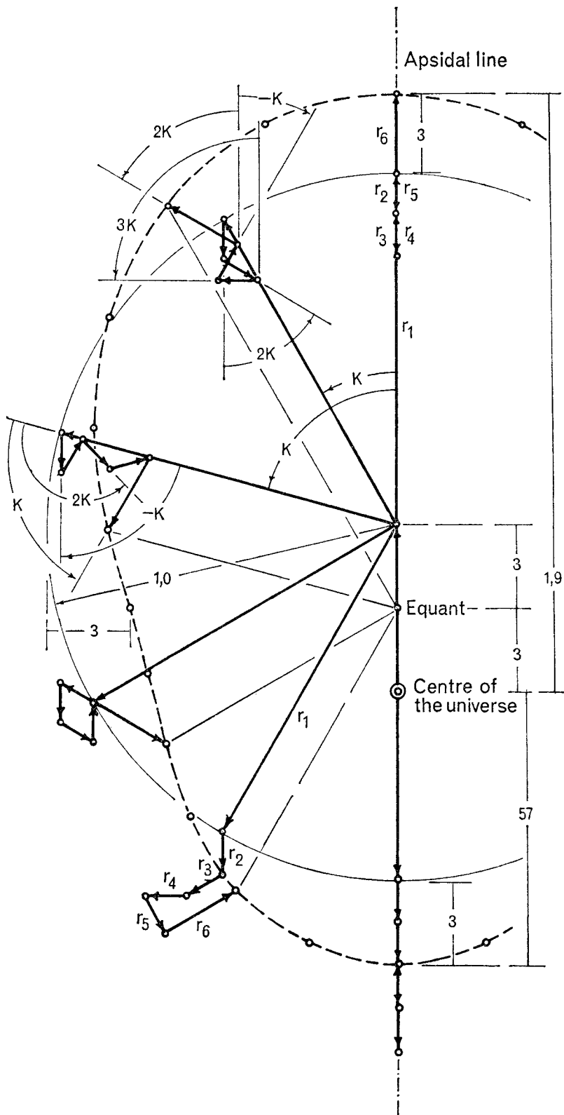
Fig. 4. Qutb al-Din's model for Mercury.
