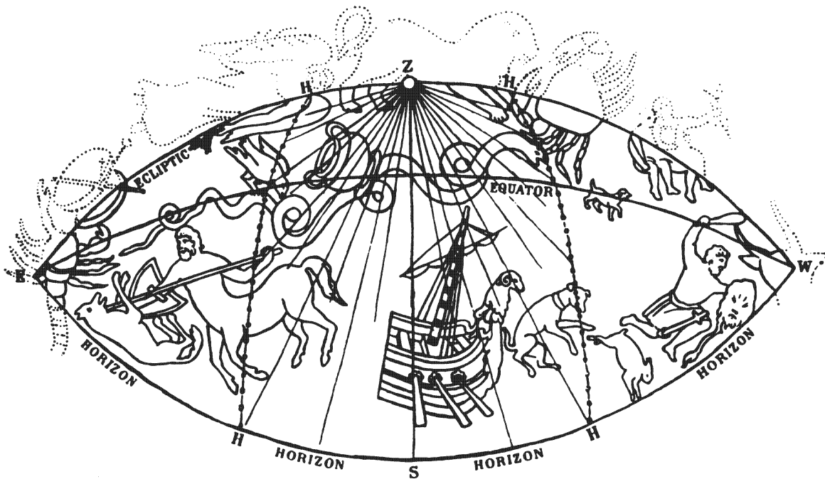
Portion of Sun at Summer Solstice, 3,000 B.C. Observer in Lat. 23^{\circ} N. Constellations between the lines H H Z and Z H H invisible all through the night of Summer Solstice.
