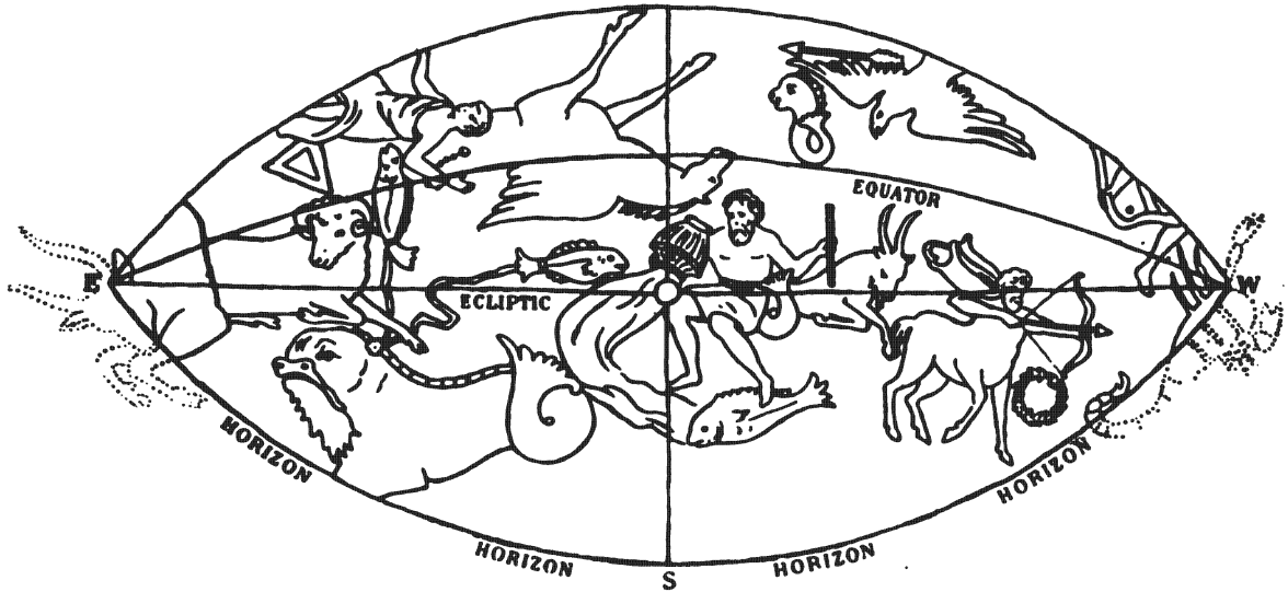
Position of Moon amongst the Constellations at Summer Solstice, and of the Sun at Winter Solstice, 3,000 B.C. Observer in Lat. 23° N.
