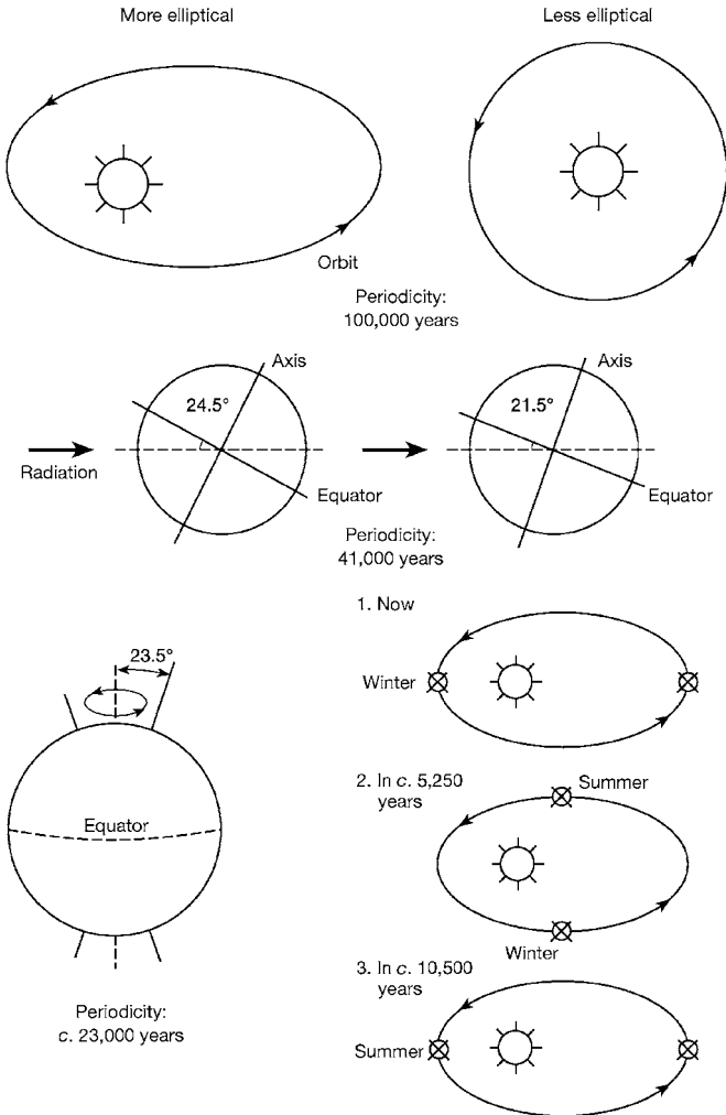
10. Milankovitch cycles control the timing of the ice ages; variations in the shape of the Earth's orbit around the Sun (top), changes in the tilt of the Earth's axis (middle), and precession about the Earth's axis (bottom)
