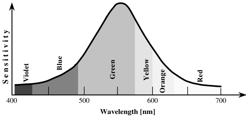
FIGURE 3.11 The spectral sensitivity of an average human eye.
