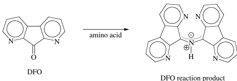
FIGURE 4.16 Suggested reaction between DFO and an amino acid to produce a luminescent product. (Wilkinson, D. [2000b], Study of the reaction mechanism of 1,8-diazafluoren-9-one with the amino acid l-alanine, Forensic Sci. Int. , 109, 87–103. With permission.)
