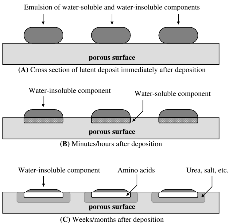
FIGURE 4.1 Aging of a latent fingerprint on a porous substrate (e.g., paper).
