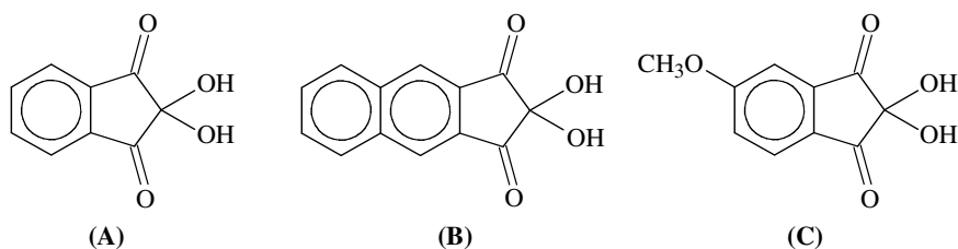
FIGURE 4.12 Chemical structures for (A) ninhydrin and the ninhydrin analogs, (B) benzoninhydrin, and (C) 5-methoxyninhydrin.
