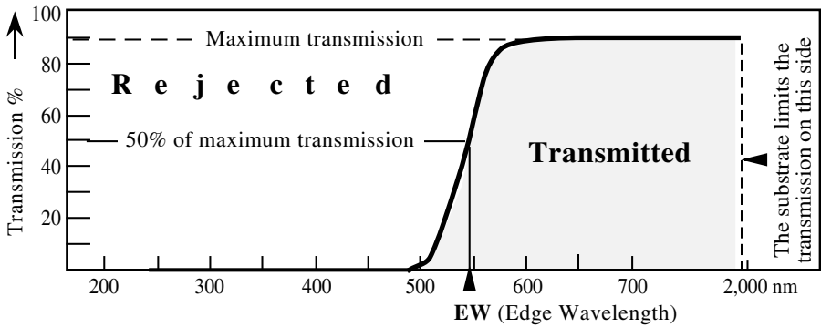
FIGURE 3.17 Typical transmission characteristics of a long pass filter.
