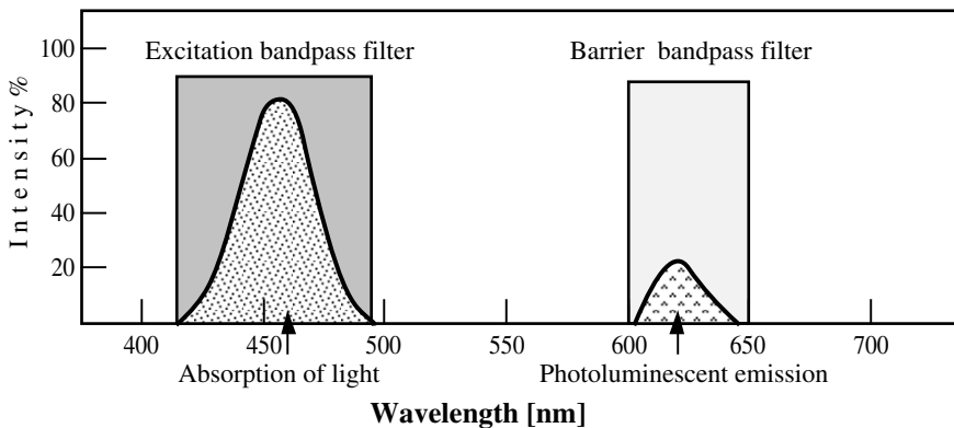
FIGURE 3.32 Absorption and emission curves for a theoretical photoluminescent material with choice of appropriate excitation and barrier filters.
