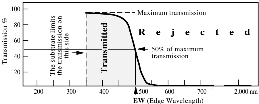
FIGURE 3.16 Typical transmission characteristics of a short pass filter.
