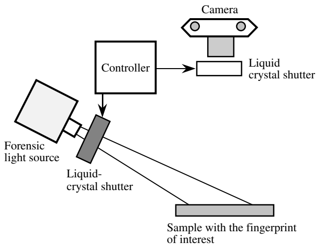
FIGURE 3.36 Two alternatively driven fast liquid-crystal shutters, one placed in front of the light source and the other in front of the camera, can be used to gather phosphorescence emission.
