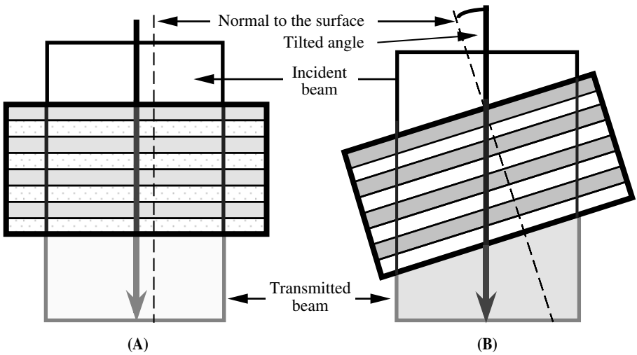
FIGURE 3.22 (A) Conventional use of an interference filter compared with (B) down-tuning, where the filter is tilted with respect to the incident beam. The light path through the filter layers becomes longer, resulting in a shift of the band toward shorter wavelengths.
