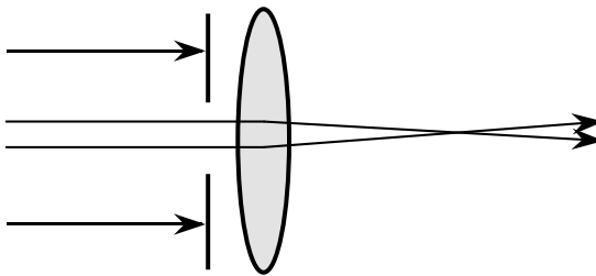
FIGURE 3.43 A diaphragm in front of the lens reduces the lens aperture, thus reducing the spherical aberration effect.
