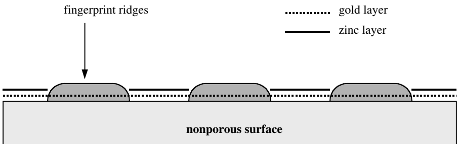
FIGURE 4.24 Principle of fingerprint development by vacuum metal deposition.
