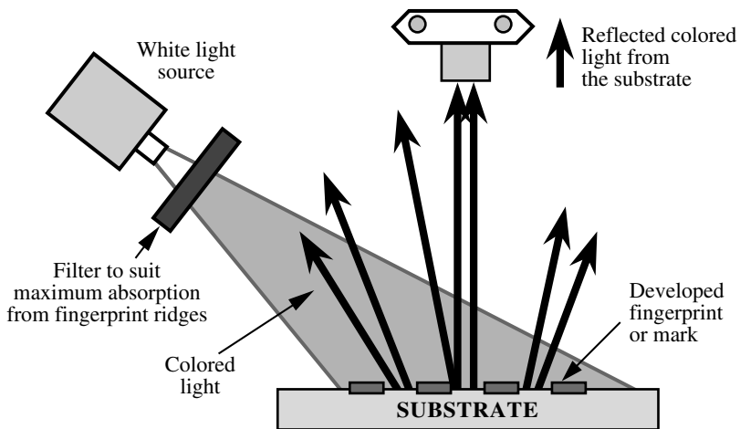
FIGURE 3.26 Schematic representation of the absorption mode with the appropriate filter in front of a light source. This method can be used only in dark or semidark situations.
