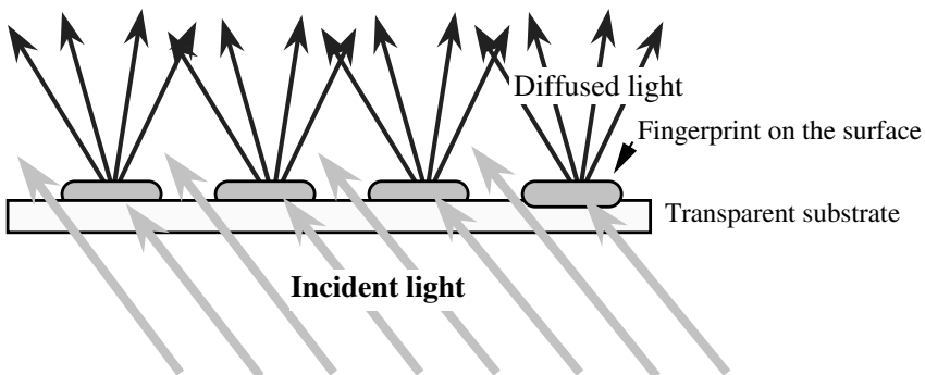
FIGURE 3.29 The diffused reflection mode as applied to a transparent substrate. Note that the incident light is directed at an angle from underneath the object.
