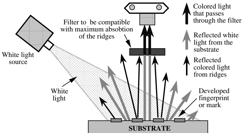
FIGURE 3.25 Schematic representation of the absorption mode with the appropriate filter used in front of the camera. This method can be used in all situations in the presence or absence of daylight or artificial light.
