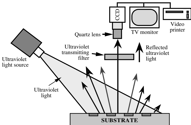
FIGURE 3.38 Implementation of the UV reflection mode.
