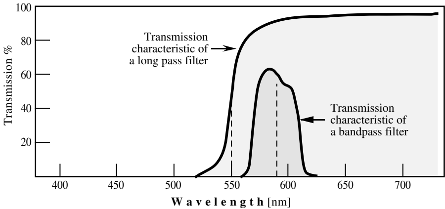
FIGURE 3.19 Transmission characteristics of a long pass filter (KV550) compared with transmission characteristics of a bandpass filter (IF590/40).
