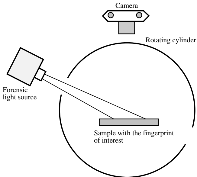
FIGURE 3.35 A phosphoroscope can be used for the recording of a phosphorescent fingerprint.
