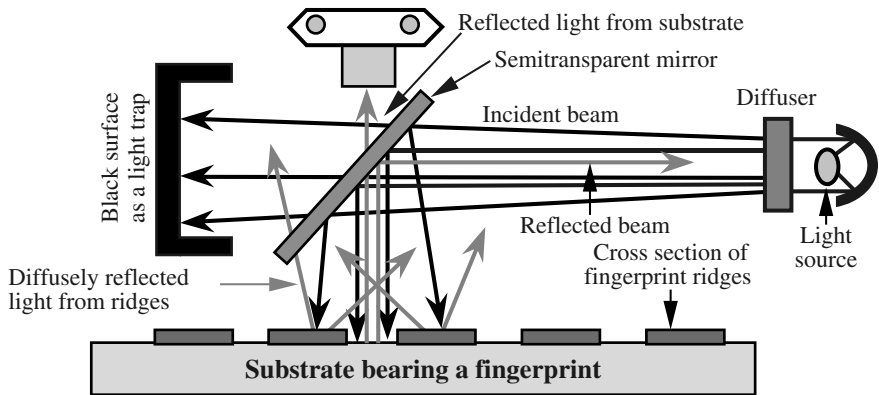
FIGURE 3.30 A schematic representation of episcopic coaxial illumination. (From Pfister, R. [1985], The optical revelation of latent fingerprints, Fingerprint Whorl , 10, 64–70. With permission.)
