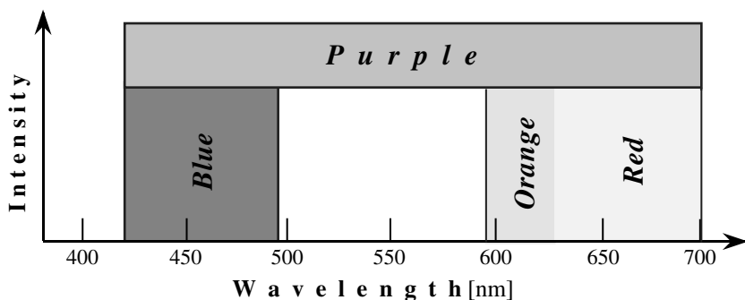
FIGURE 3.10 A blue band combined with an orange/red band will produce polychromatic light that will be perceived by the human eye as being purple in color.
