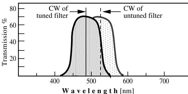
FIGURE 3.23 Tilting of an interference filter results in the shifting of its passband toward shorter wavelengths (wavelength down-tuning).
