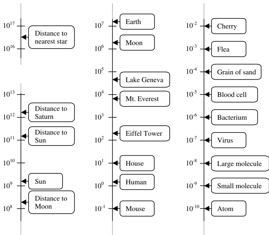
FIGURE 3.1 Scale of dimensions (in meters).
