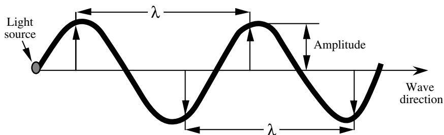
FIGURE 3.6 Wave theory. Schematic representation of a light wave. The distance between the two nearest points in the same phase is known as the wavelength \lambda .
