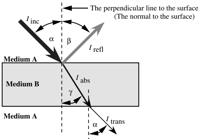
FIGURE 3.12 Transformation of incident light after irradiation of an object.
