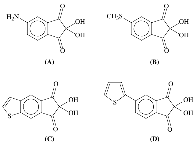
FIGURE 4.13 Chemical structures for the ninhydrin analogs (A) 5-aminoninhydrin, (B) 5-methylthioninhydrin, (C) thieno[f]ninhydrin, and (D) 5-(2-thienyl)-ninhydrin.
