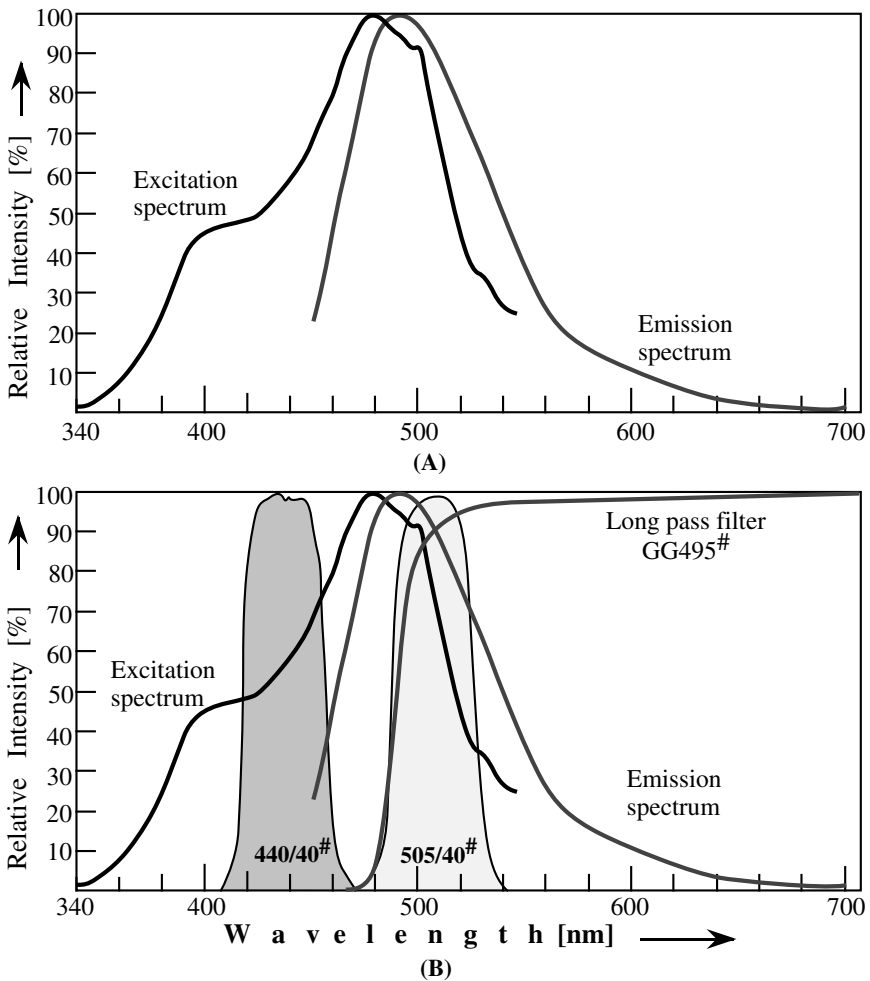
FIGURE 4.26 (A) Luminescence spectra for a DMAC-developed fingerprint; (B) Recommended filter combination for excitation (*) and observation (#).
