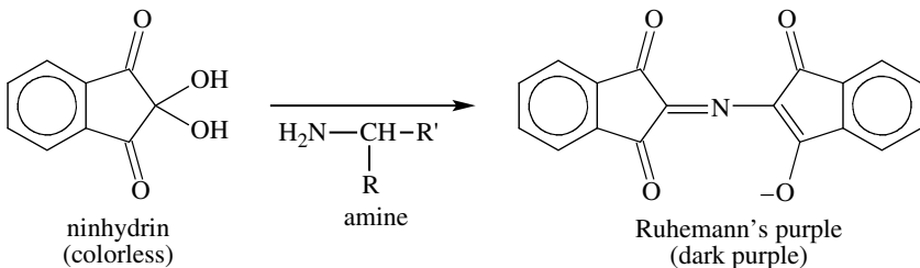
FIGURE 4.3 Chemical reaction between ninhydrin and a primary or secondary amine, resulting in the formation of a dark purple product known as Ruhemann's purple.
