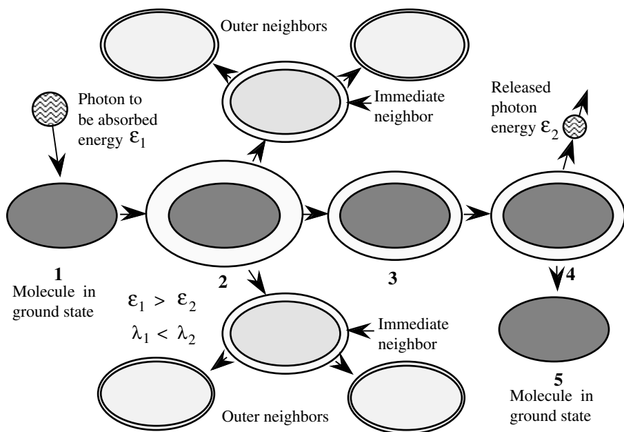
FIGURE 3.14 Absorption and emission of a photon — photoluminescence. (1) A molecule in its normal (ground) state just before absorption of a photon. (2) The molecule becomes excited by the amount of absorbed energy. It immediately shares some of its extra energy with its nearest neighbors. Shared energy spreads out to other molecules. (3) The molecule is less excited by the amount of the shared energy. (4) The molecule releases (emits) its extra energy in the form of a photon. (5) The molecule returns to its ground state.
