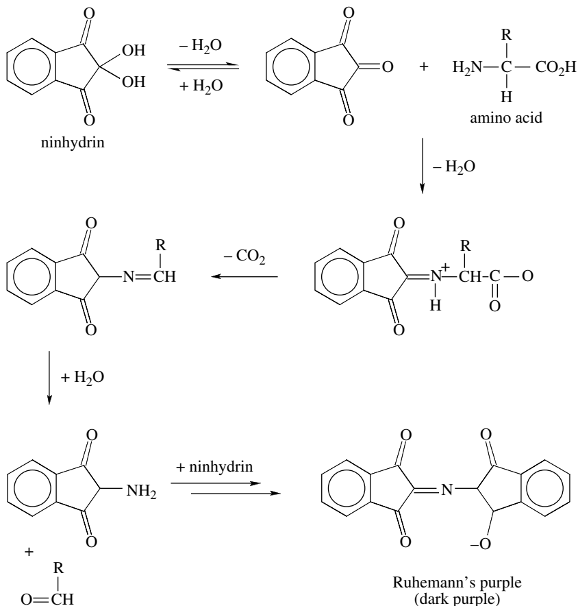
FIGURE 4.5 Mechanism for the reaction between ninhydrin and an amino acid.
