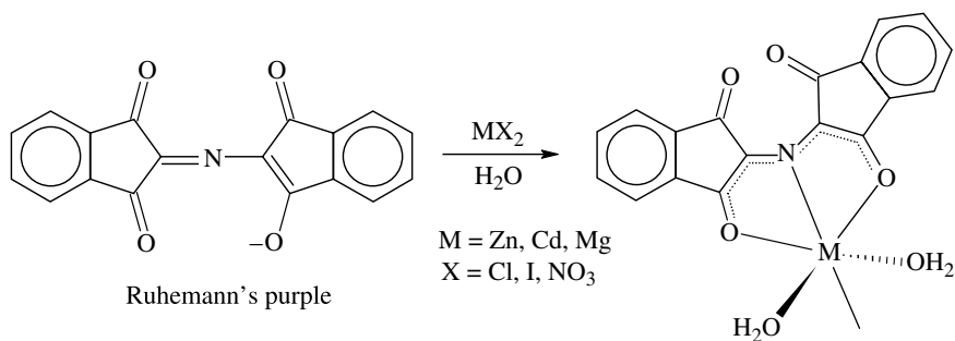
FIGURE 4.7 Treatment of Ruhemann's purple with certain metal salts results in the formation of a coordination complex. (From Lennard, C.J., Margot, P.A., Sterns, M., and Warrenner, R.N. [1987], Photoluminescent enhancement of ninhydrin developed fingerprints by metal complexations: structural studies of complexes formed between Ruhemann's purple and Group IIb metal salts, J. Forensic Sci. , 32, 597–605. With permission.)
