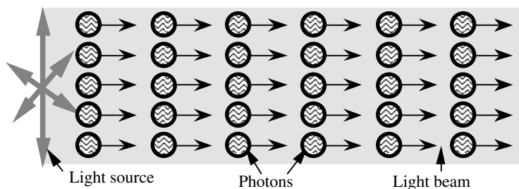
FIGURE 3.7 A beam of pure energy particles, called photons, traveling at the speed of light.
