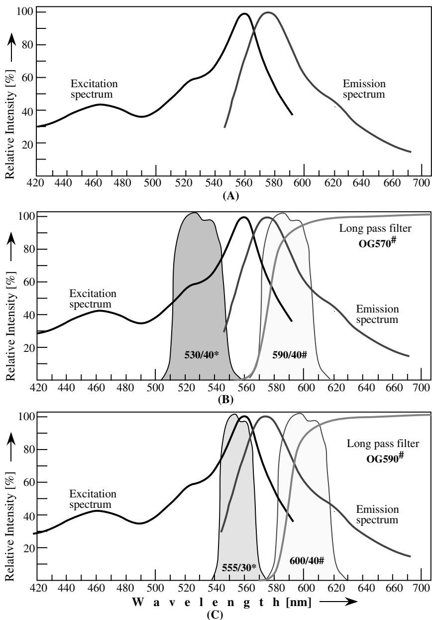
FIGURE 4.17 (A) Luminescence spectra for a DFO developed fingerprint on paper; (B, C) Recommended filters for excitation (*) and observation (#) in the luminescence.
