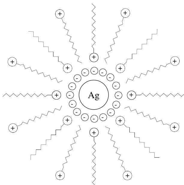
FIGURE 4.19 In the PD reagent, cationic surfactant molecules form positively charged micelles, each encapsulating a negatively charged silver colloid (silver colloid surrounded by negatively charged citrate ions). These positively charged micelles stabilize the reagent by repelling nearby silver ions and other micelles. (From: Cantu, A.A. [2001], Silver physical developers for the visualization of latent prints on paper, Forensic Sci. Rev. , 13, 29–64; and from Cantu, A.A. and Johnson, J.L. [2001], Silver physical development of latent prints, in Advances in Fingerprint Technology , 2nd ed., H.C. Lee and R.E. Gaensslen, Eds., Boca Raton, FL: CRC Press, pp. 242–247. With permission.)
