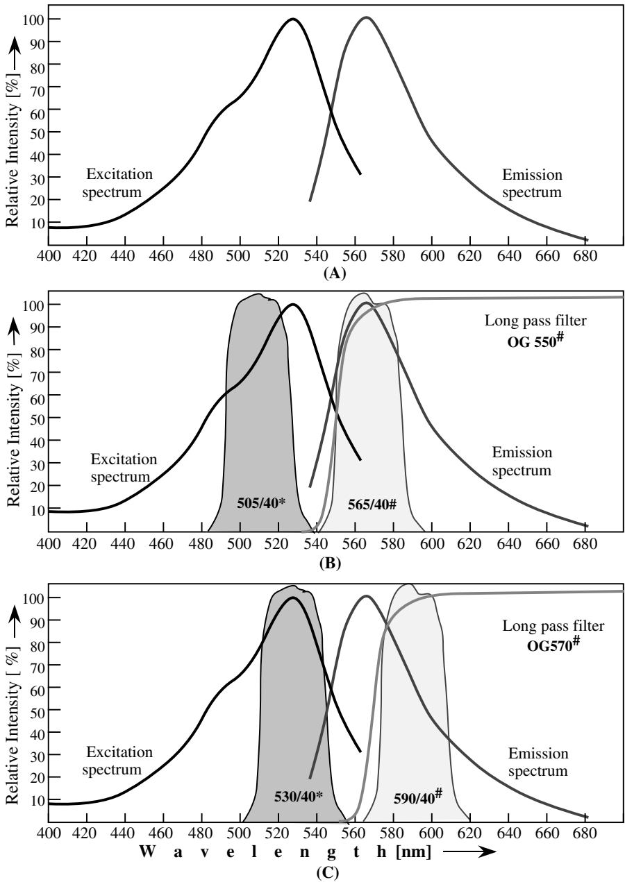
FIGURE 4.22 (A) Luminescence spectra for a cyanoacrylate-delivered fingerprint stained with rhodamine 6G; (B, C) recommended filter combinations for excitation (*) and observation (#) mode.
