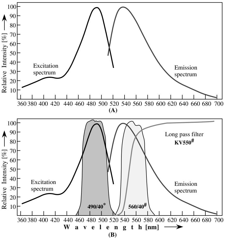
FIGURE 4.9 (A) Luminescence spectra recorded at liquid nitrogen temperature for a ninhydrin developed print post-treated with zinc nitrate; (B) Recommended filters for excitation (*) and observation (#) in the luminescence mode.
