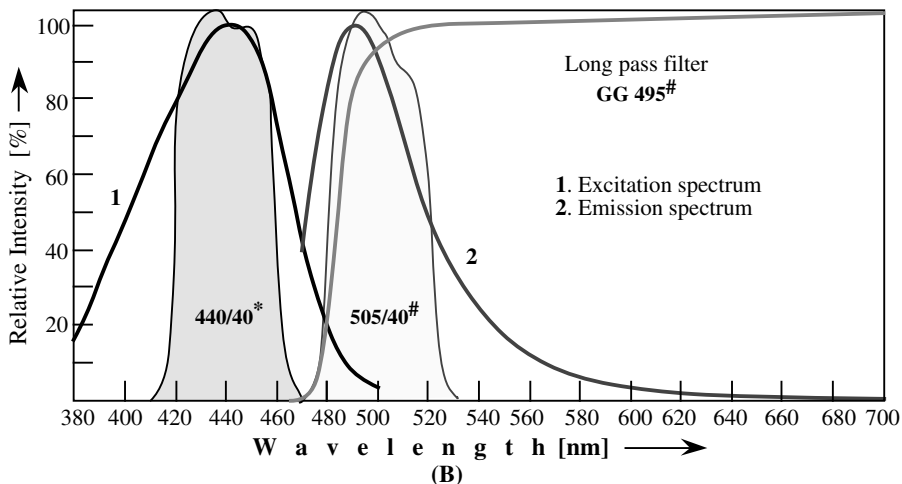
FIGURE 4.23 (A) Luminescence spectra for a cyanoacrylate-developed fingerprint stained with Basic Yellow 40; (B) Recommended filter combination for excitation (*) and observation (#).
