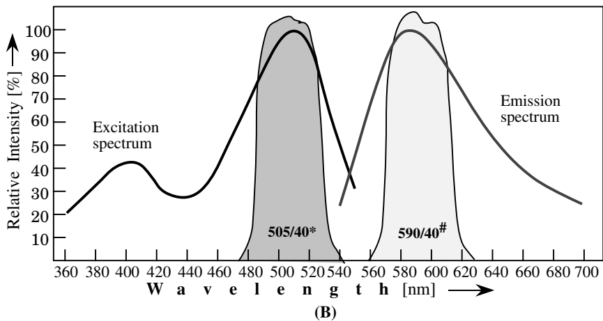
FIGURE 4.10 (A) Luminescence spectra recorded at liquid nitrogen temperature for a ninhydrin developed print post-treated with cadmium nitrate; (B) Recommended filters for excitation (*) and observation (#) in the luminescence mode.
