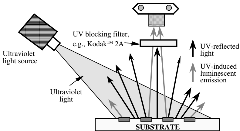
FIGURE 3.37 Typical setup for the photoluminescence mode with excitation in the UV region and observation in the visible region.
