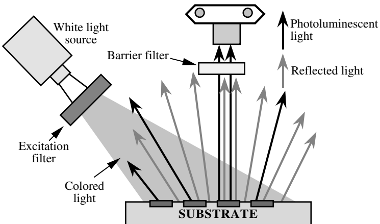
FIGURE 3.34 Arrangement for photoluminescence observation.
