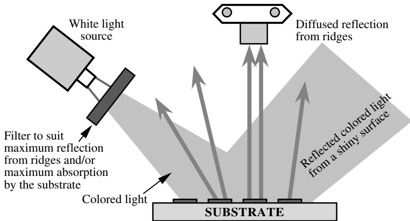
FIGURE 3.28 A schematic representation of the diffused reflection mode.
