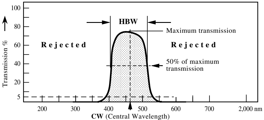
FIGURE 3.18 Typical transmission characteristics of a bandpass filter.
