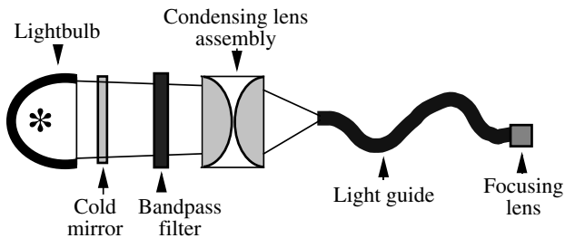
FIGURE 3.39 Schematic representation of a forensic light source.
