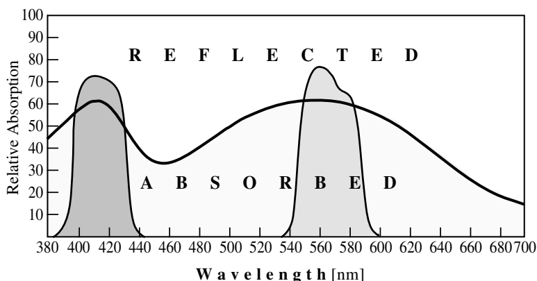
FIGURE 3.27 A typical absorption spectrum for a ninhydrin-developed fingerprint. There are two absorption bands: a narrow band with a maximum at around 410 nm (violet region) and a broad major band with a maximum at around 560 to 580 nm (green–yellow region).
