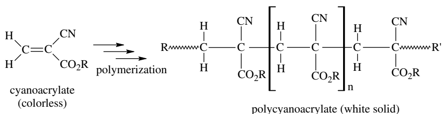
FIGURE 4.21 Cyanoacrylate polymerization reaction that results in the formation of a hard white polymer known as polycyanoacrylate.
