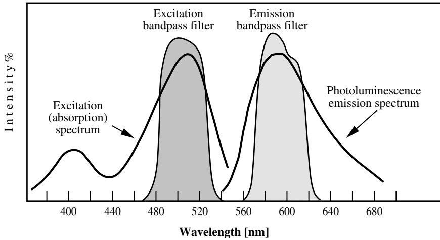
FIGURE 3.33 Excitation and emission spectra for a ninhydrin-developed latent fingerprint post-treated with cadmium nitrate (as an example) with the choice of appropriate filters for excitation and emission.
