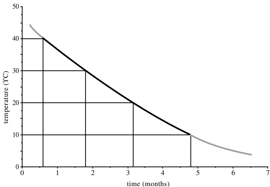
FIGURE 5.1 A typical fingerprint dehydration curve relating temperature to average drying time (in months) under controlled conditions (relative humidity = 50%).
