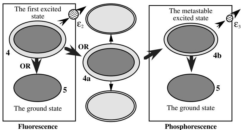
FIGURE 3.15 The molecule in stage 4 (first excited state) has two possibilities of returning to the ground state: directly, or indirectly by further sharing its extra energy. The latter process takes longer and leads to phosphorescence emission.
