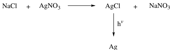
FIGURE 4.27 Silver nitrate reacts with chloride in the print deposit to form silver chloride. In the presence of light ( h^\nu ), silver chloride decomposes to silver metal.
