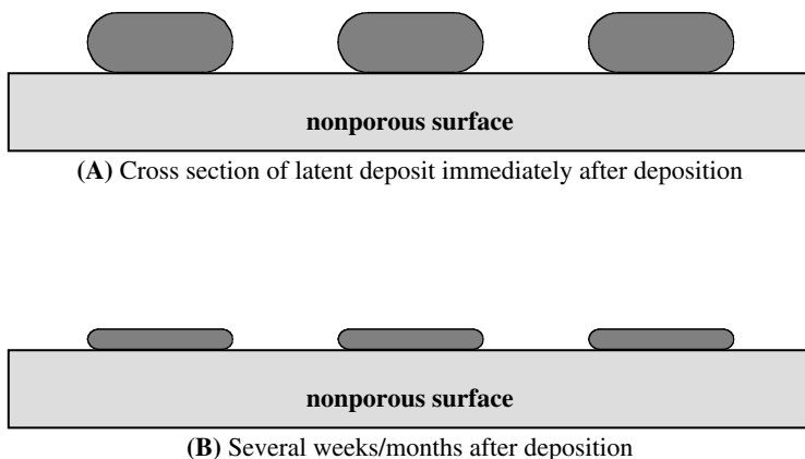
FIGURE 4.2 Aging of a latent fingerprint on a nonporous substrate (e.g., glass).
