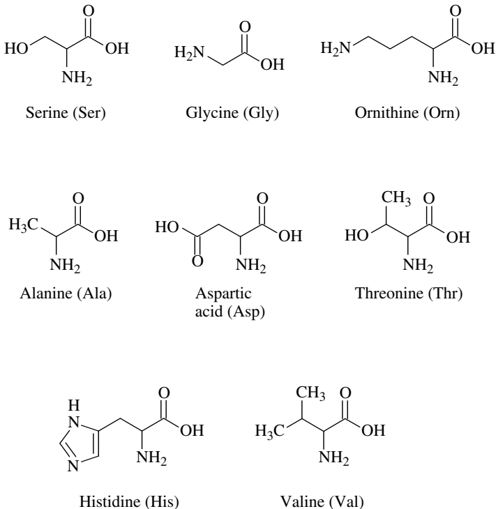
FIGURE 4.4 Structures of the major amino acids found in a typical latent fingerprint deposit.
