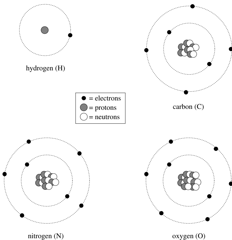
FIGURE 3.3 The atomic structures of hydrogen, carbon, nitrogen, and oxygen.
