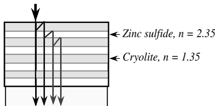
FIGURE 3.21 An interference filter is made from many alternate layers of zinc sulfide and cryolite. Beams with different light paths through the filter interfere with each other, which leads to only certain wavelengths appearing in the transmitted light.
