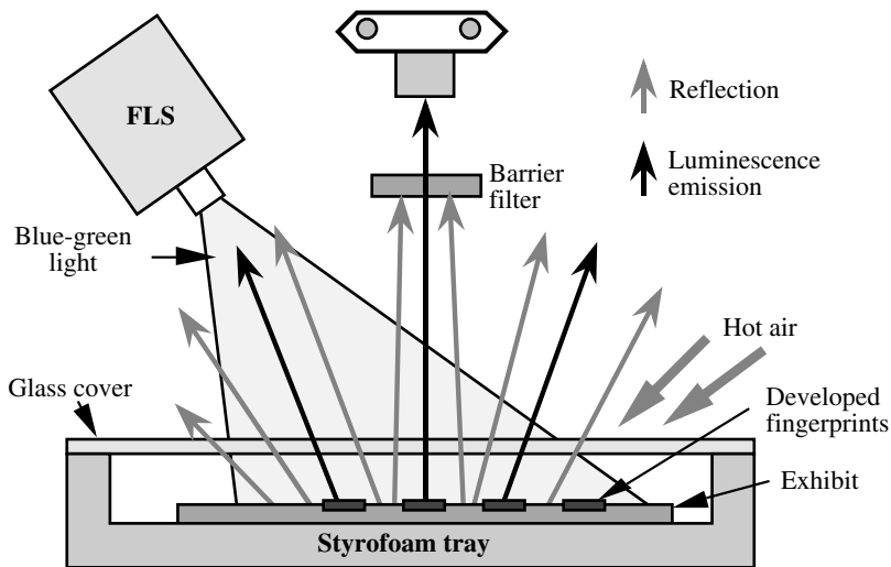
FIGURE 4.11 General luminescence mode set-up for the recording of ninhydrin developed prints post-treated with a metal salt (zinc or cadmium).
