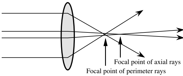
FIGURE 3.42 Schematic representation of spherical aberration.
