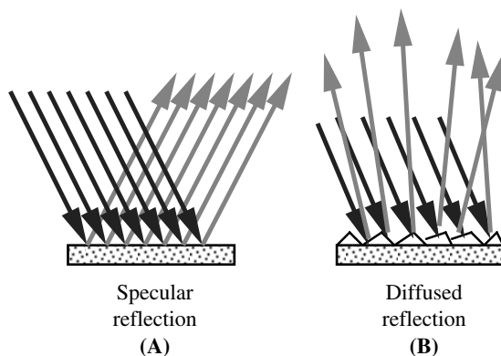
FIGURE 3.13 (A) Specular reflection from a flat surface. (B) Diffused reflection from a rough surface.
