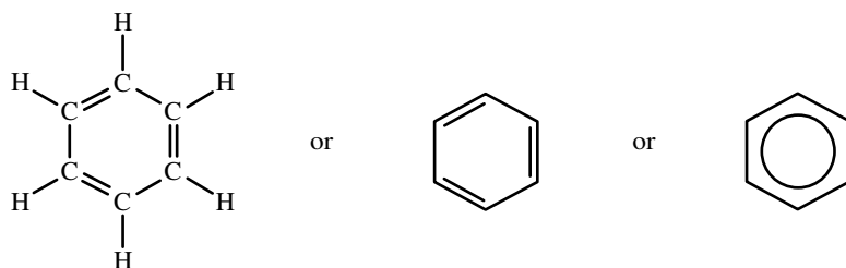
FIGURE 3.4 Different graphical representations for a benzene ring ( C_6H_6 ).
