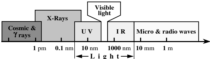
FIGURE 3.5 The electromagnetic spectrum. Light consists of three parts: ultraviolet (UV), visible, and infrared (IR). Visible light is a very small portion in this region.
