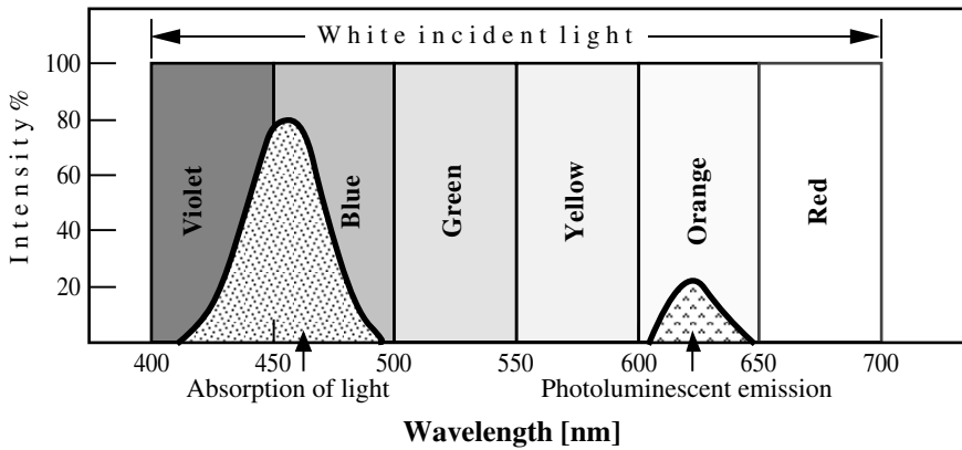
FIGURE 3.31 Absorption and emission curves for a theoretical photoluminescent material with white incident light.
