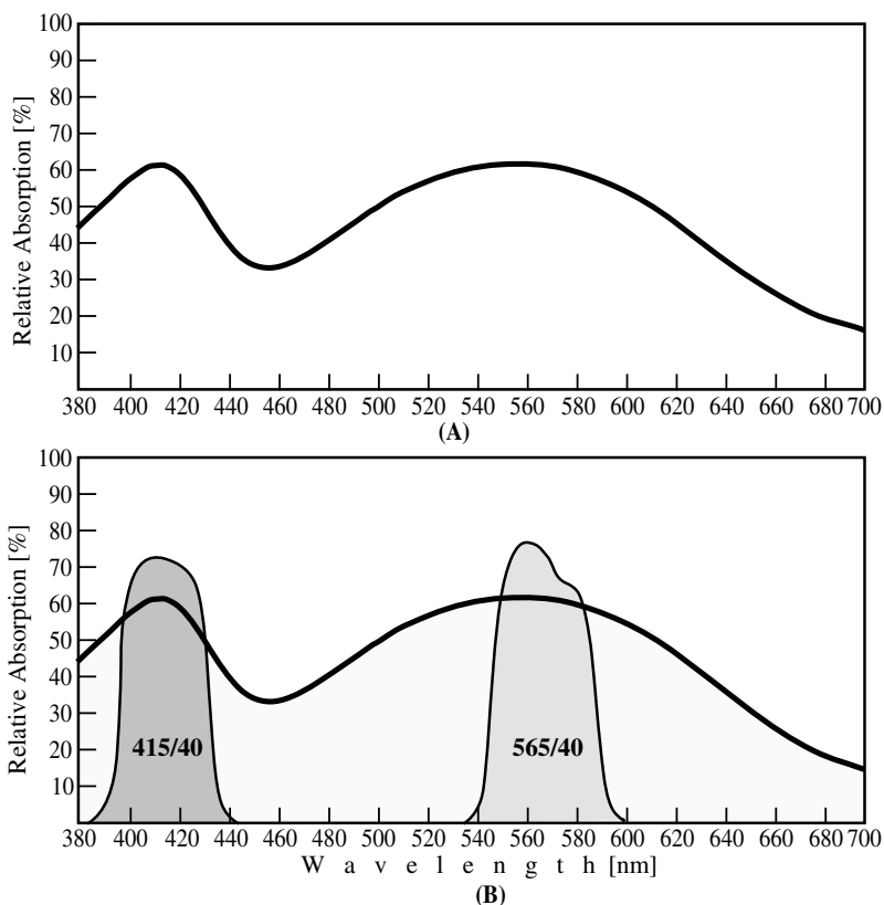
FIGURE 4.6 (A) Relative absorption of spectrum of a ninhydrin-developed fingerprint on paper; (B) Recommended bandpass filters for observation in the absorption mode.
