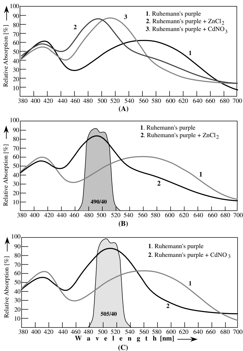
FIGURE 4.8 (A) Relative absorption spectra of Ruhemann's purple and its complexes with zinc and cadmium; (B) Recommended bandpass filter for observation in the absorption mode in the case of the zinc complex; (C) Recommended bandpass filter for observation in the absorption mode in the case of the cadmium complex.
