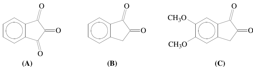
FIGURE 4.15 Chemical structures for (A) ninhydrin in its anhydrous form, (B) 1,2-indanedione, and (C) 5,6-dimethoxy-1,2-indanedione.
