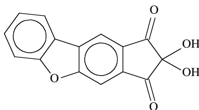
FIGURE 4.14 Structure of benzo[f]furoninhydrin.
