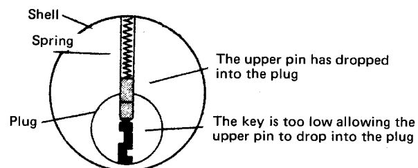
Fig. 5 Cylinder with Improper Key Cuts Too Low
