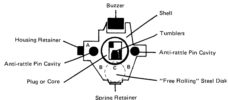
FRONT VIEW OF 76½-UP FORD IGNITION WITH "BUTTERFLY" REMOVED
