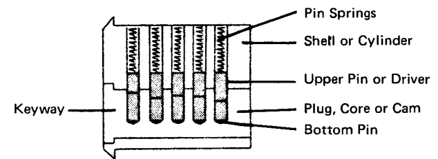
Fig. 1 Cylinder without Key
