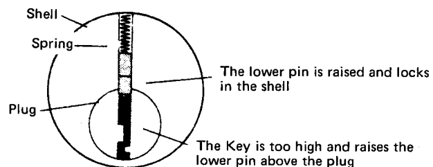
Fig. 4 Cylinder with Improper Key Cuts Too High
