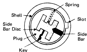
Fig. 9 Side Bar Cylinder - Proper Key
