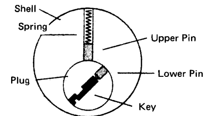
Fig. 2 Cylinder with Proper Key Front View
