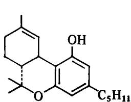
\Delta^1 -THC
