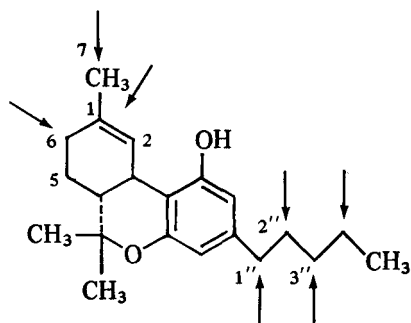
\Delta^1 -THC
