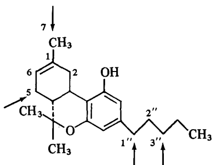
\Delta^6 -THC
