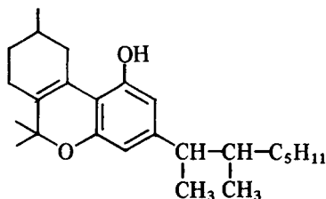
DMHP
