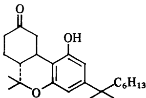
Nabilone (Lilly)
