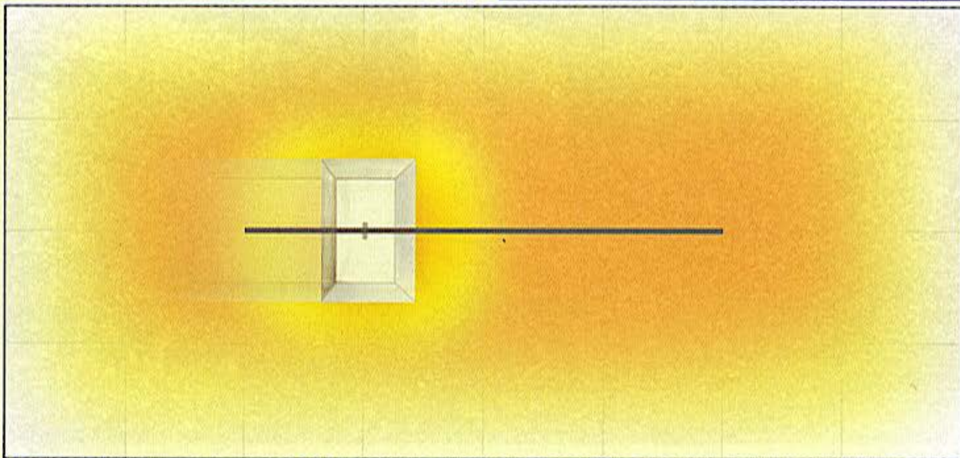
This is the approximate coverage of a linear light mover. Note the brightest light is close to the reflector.
