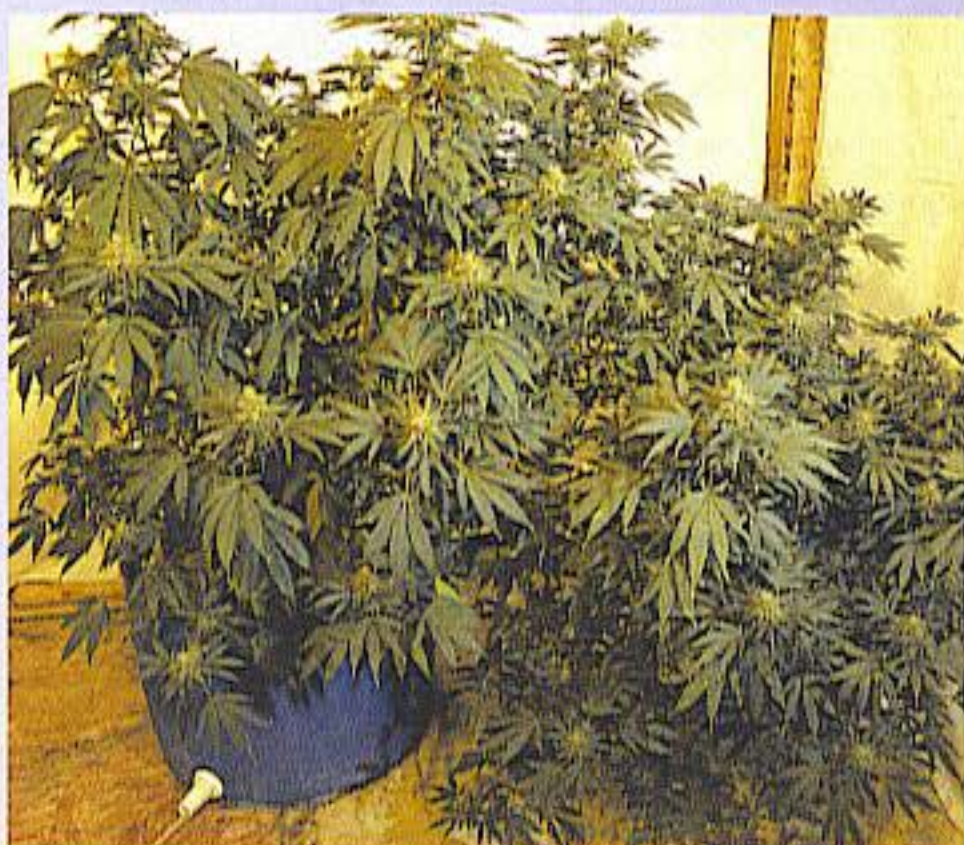
This ingenious DWC garden uses an air pump to aerate and agitate the nutrient solution.
