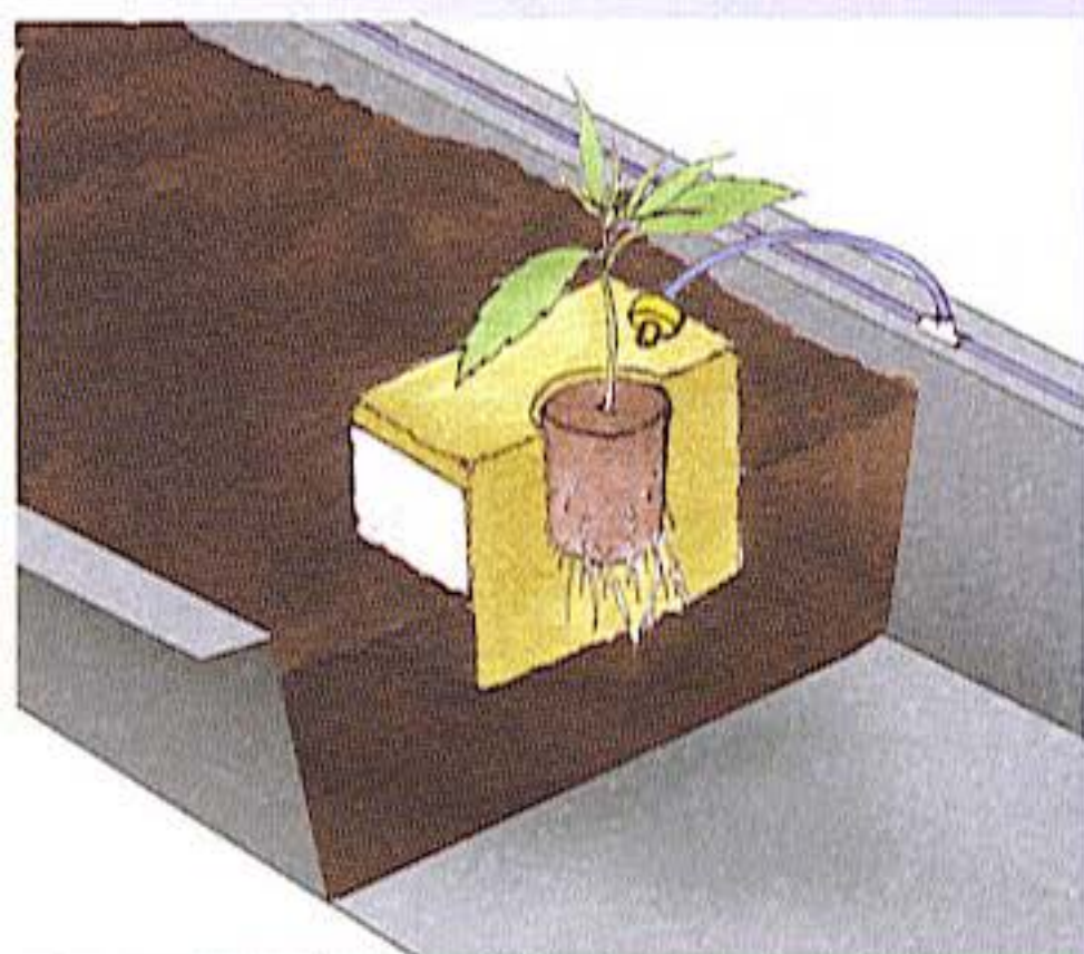
This cutaway drawing shows how nutrient delivery is simple and easy with a top-feed bat system. Aerated nutrient solution is metered via emitter onto a grow cube. Aerated solution percolates down through the medium. Channels in the bottom of the tray speed drainage back to the reservoir.
