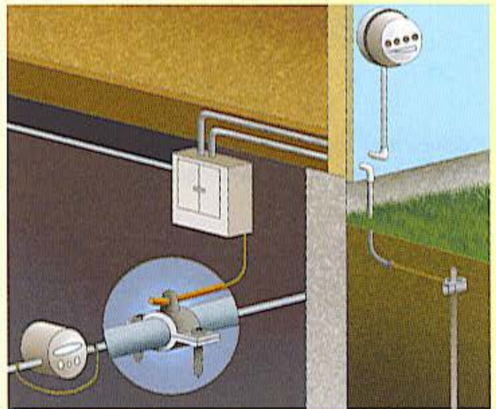
Electrical ground
