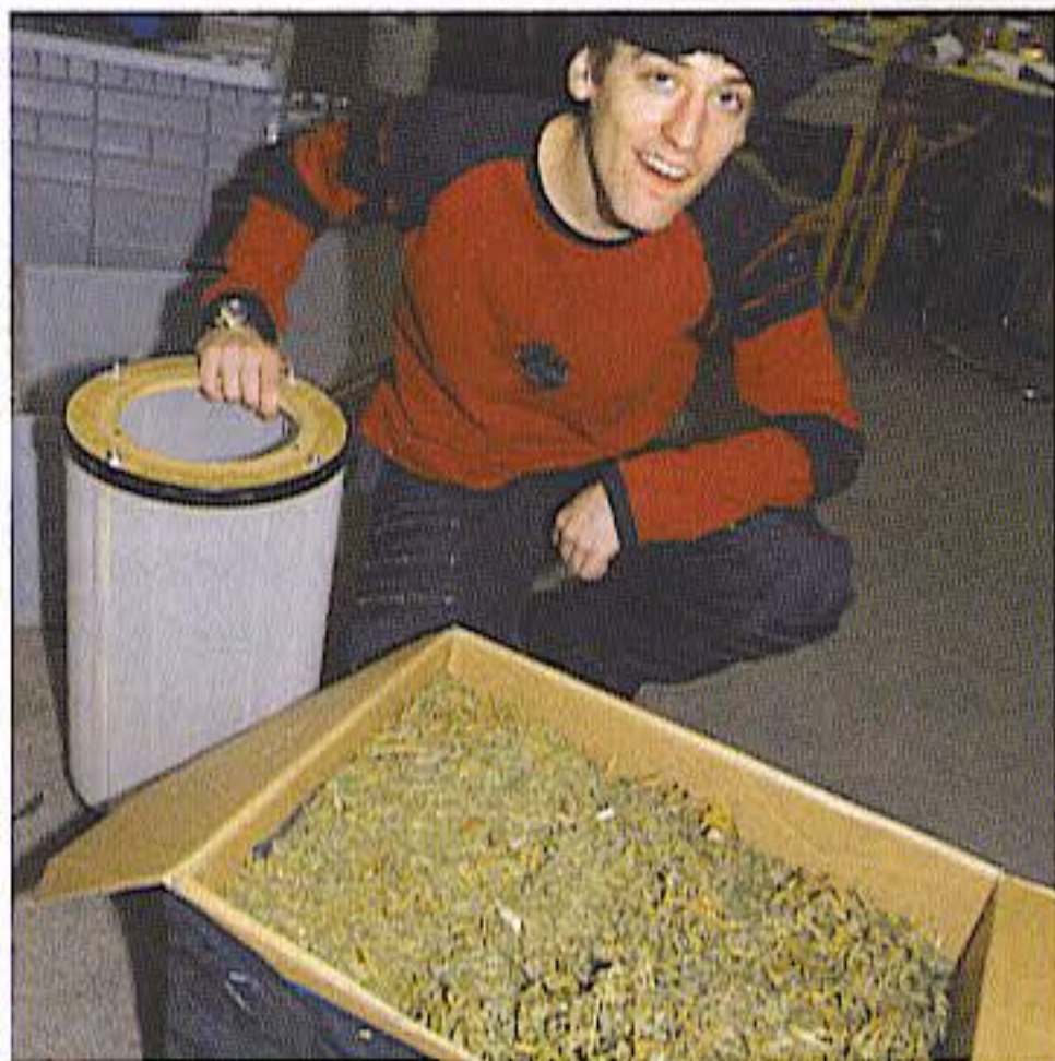
Open the lid of the Pollinator, and lift out the silkscreen drum. Pick up the drum and remove it from the containing box.
