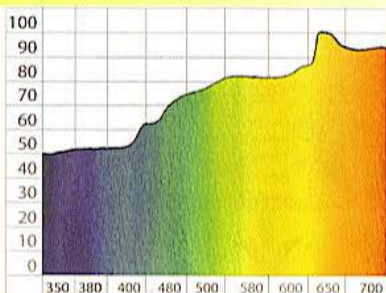
The light spectrum of an incandescent lamp will grow plants but is best suited to generating heat.
