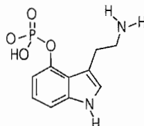
Figure 5. Norbaeocystin or 4-phosphoryloxytryptamine.
