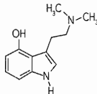
Figure 3. Psilocin or 4-hydroxy-N,N-dimethyltryptamine.
