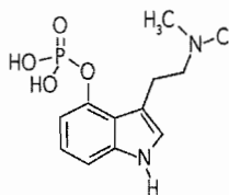
Figure 2. Psilocybin or 4-phosphoryloxy-N,N-dimethyltryptamine.
