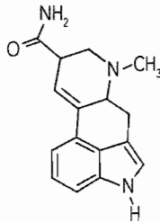
Figure 15. Lysergic Acid Amide.
