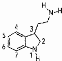
Figure 1. Tryptamine, showing numbering of the indole ring.
