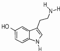
Figure 9. Serotonin or 5-hydroxytryptamine.
