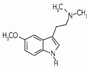
Figure 7. 5-methoxy-N,N-dimethyltryptamine or 5-MeO-DMT.
