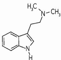
Figure 6. N,N-dimethyltryptamine or DMT.
