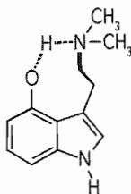
Figure 11A. Possible hydrogen bonding interaction in psilocin.
