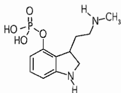
Figure 4. Baeocystin or 4-phosphoryloxy-N-methyltryptamine.
