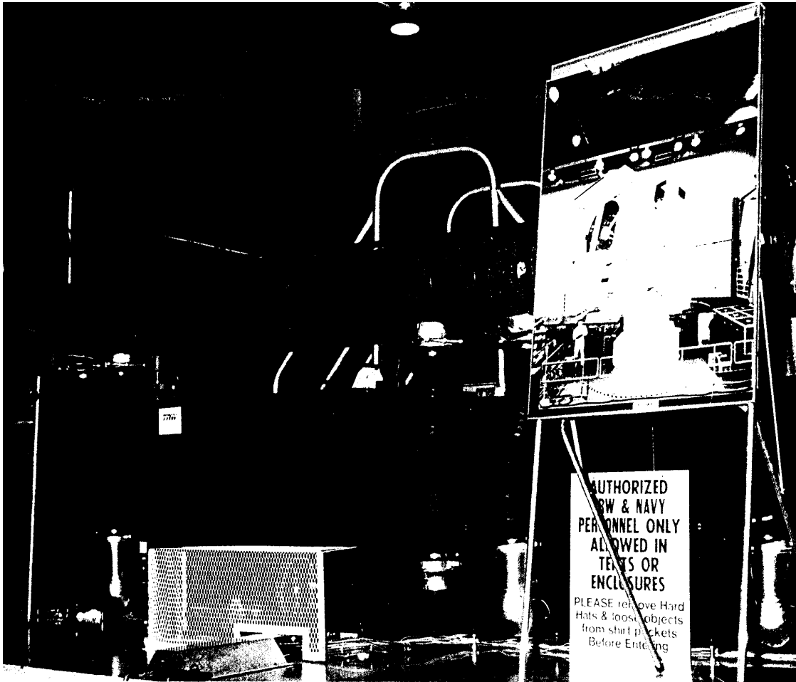
Opposite page: The US Navy's Hughes Aircraft-manufactured High Energy Laser Beam Director (HEL) . Immediate left: This is a closeup of the HEL's mirror arrangement. Above: The TRW Defense and Space Systems Group laser, built for use with the HEL ( in mirror ).
