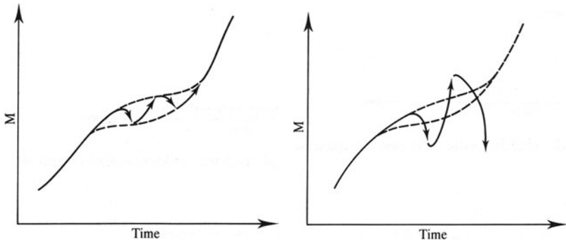
3.8 Local Turbulence
