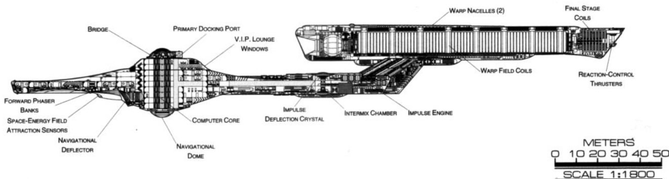
CROSS SECTION
