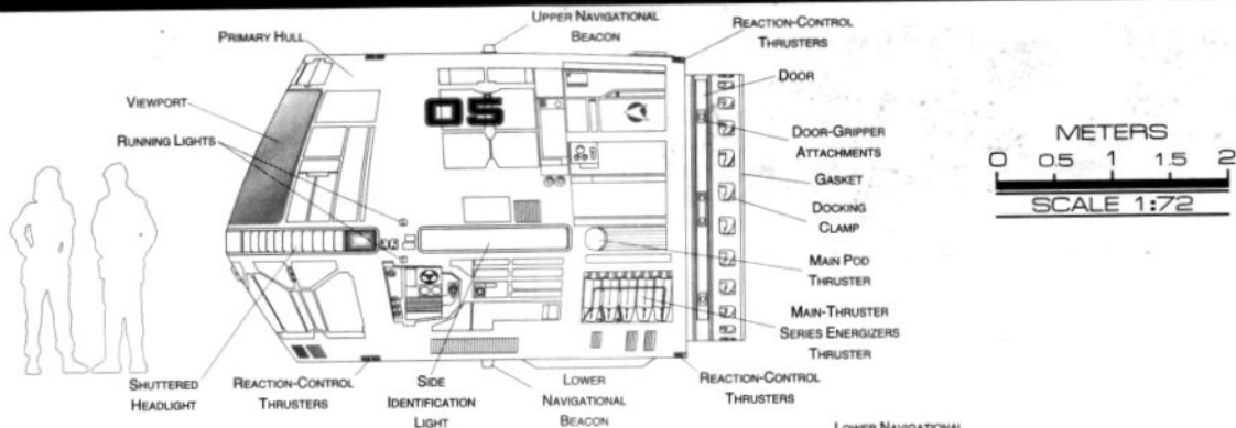
PORT PROFILE
