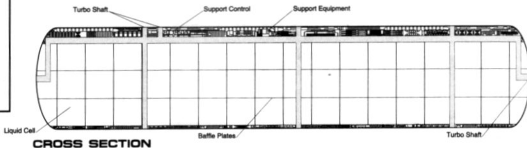
CROSS SECTION
