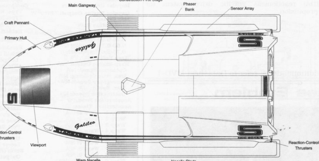
TOP PROFILE
