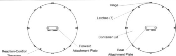
FRONT PROFILE
