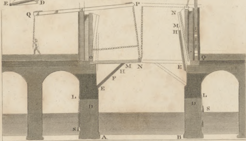
DRAW BRIDGE.
