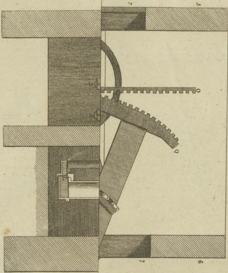
Watt's STEAM ENGINE.
