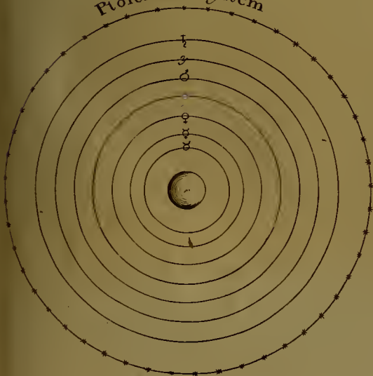
Fig. 150 Ptolemaic System
