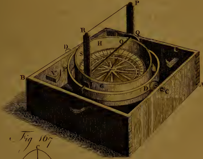
AZIMUTH Compass
