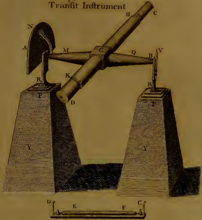
Fig. 222. Compound Transit Instrument.
