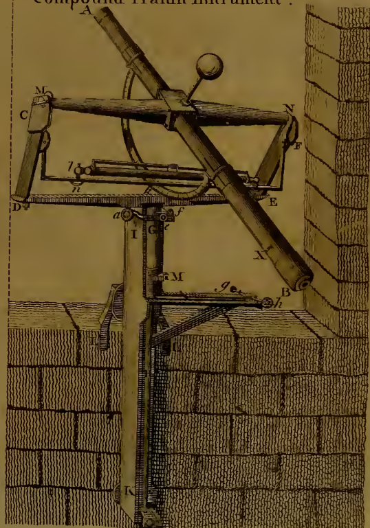
Fig. 222. Compound Transit Instrument.
