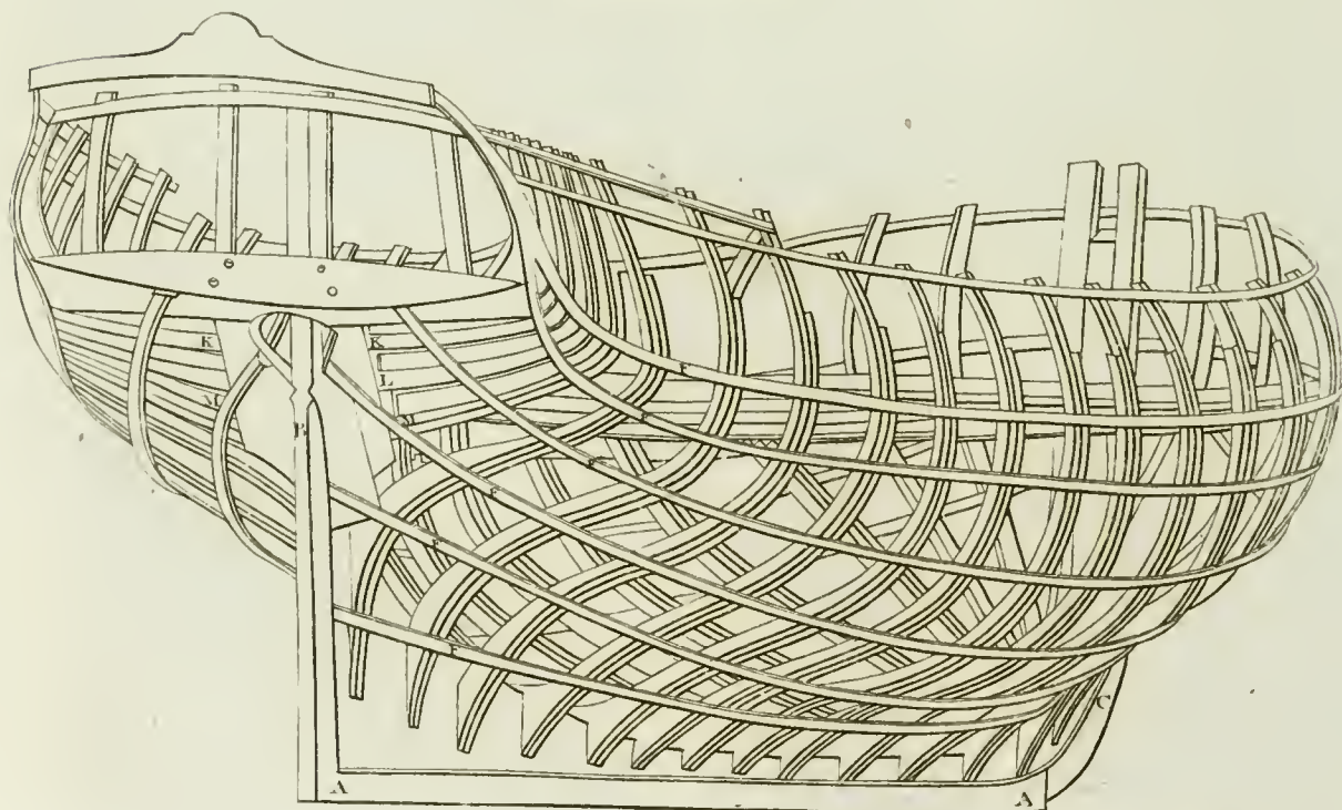
FRAMES of a SHIP.
